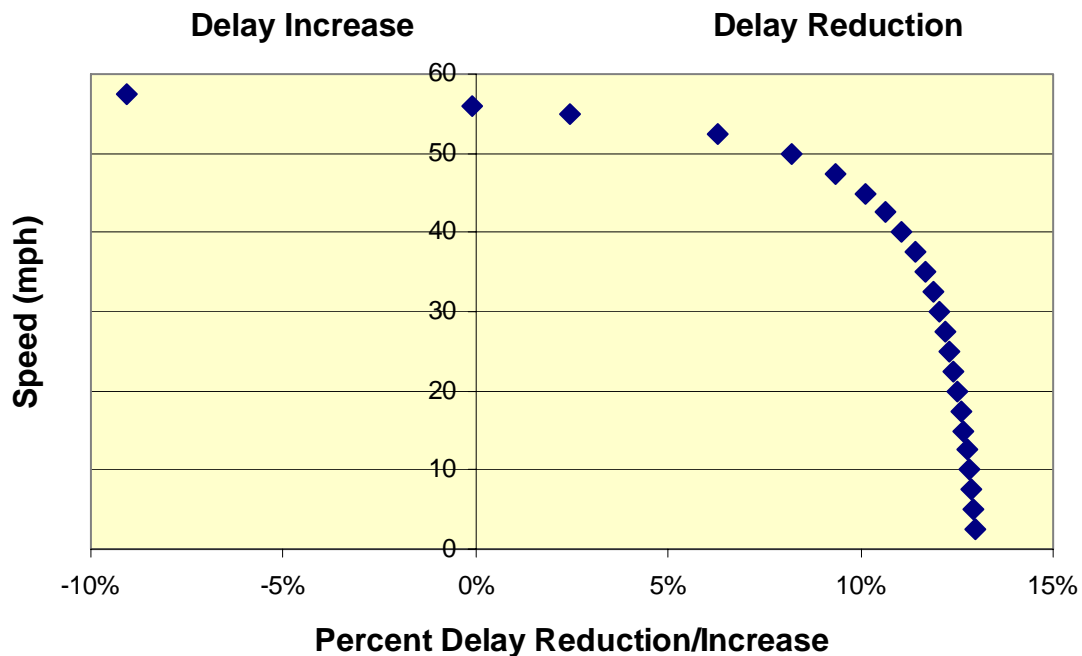
Exhibit 2. Ramp Metering Effects – Speed versus Delay Savings
