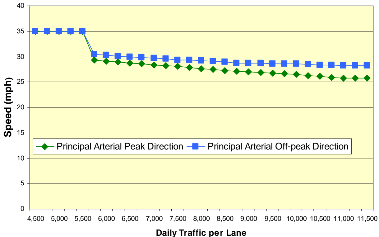
Exhibit 9. Principal Arterial Speed Estimation
