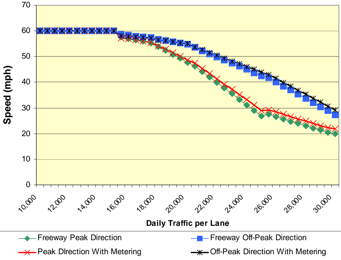
Exhibit 3. Freeway Speed Curves
