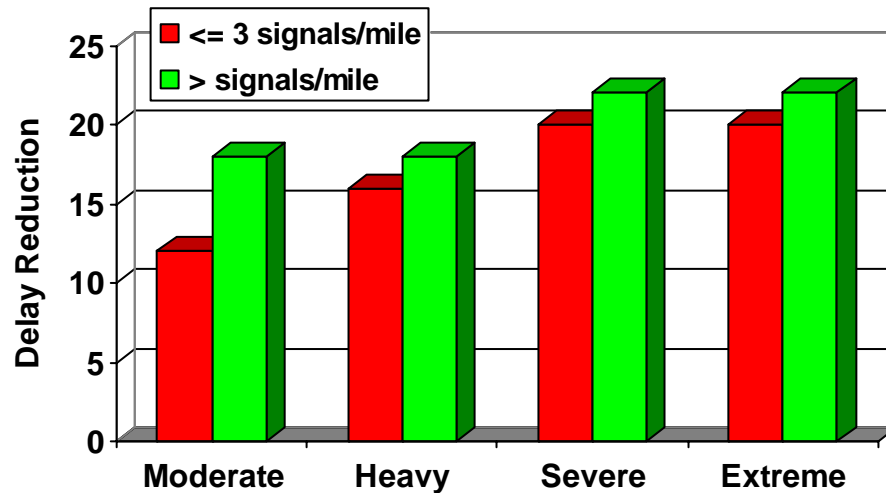
Exhibit 19. Access Management Incident Delay Effects
