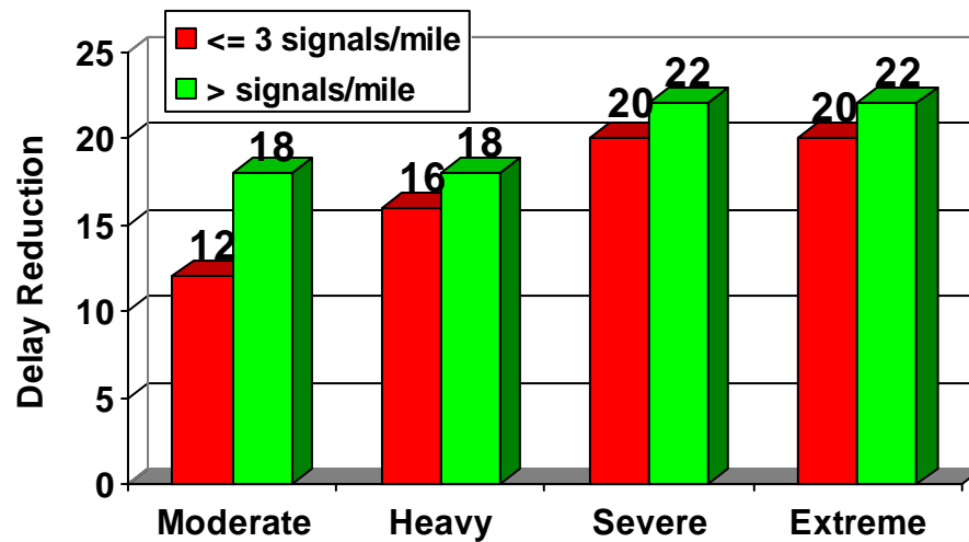
Exhibit 29. Access Management Incident Delay Effects
