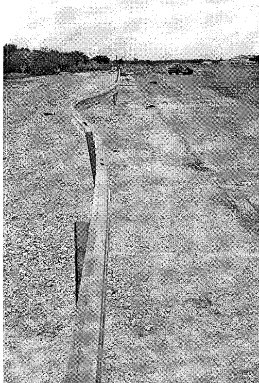
Figure 6. Vehicle trajectory after test 473750-4.
