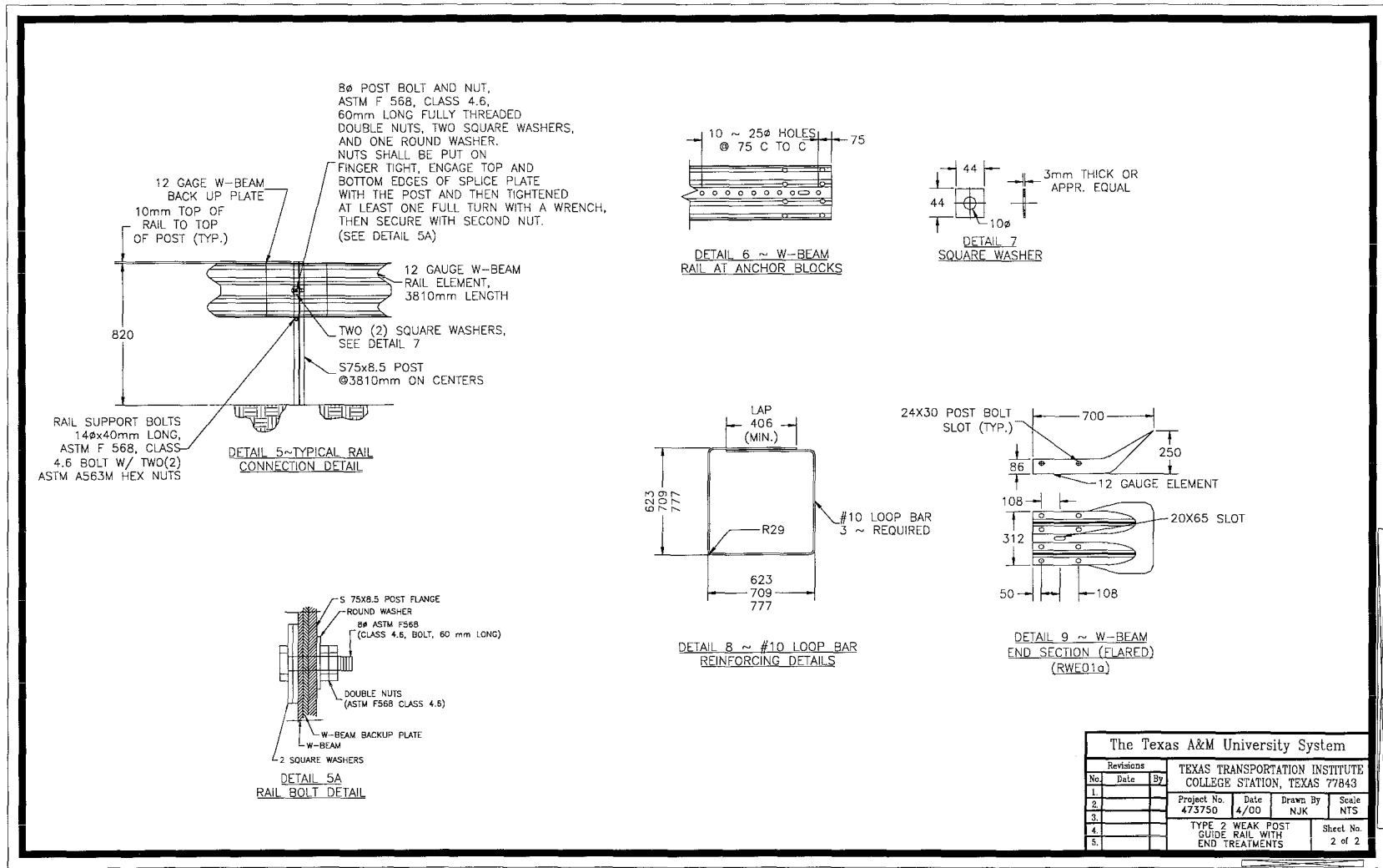
Figure 1. Details of the PennDOT Type 2 guide rail for test 473750-4 (continued).
