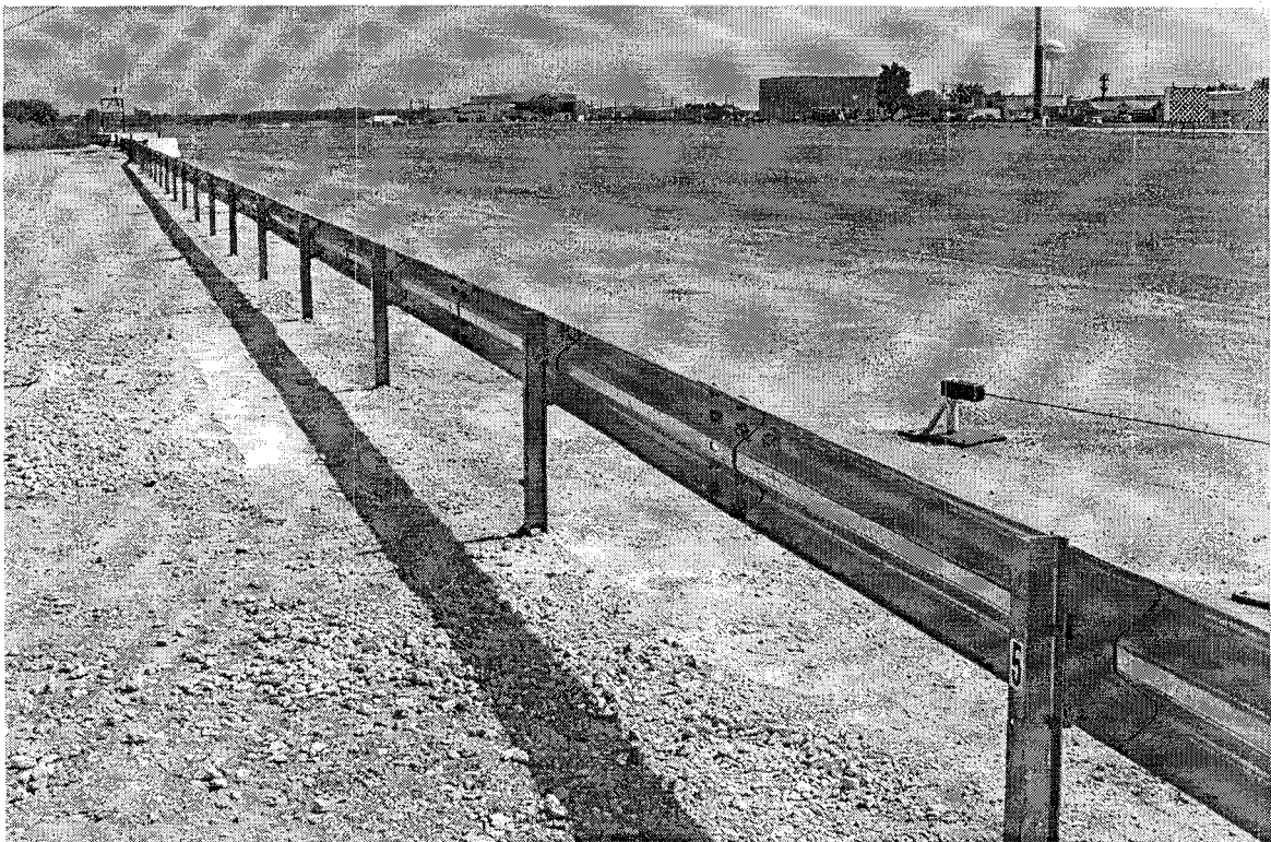
Figure 2. PennDOT Type 2 guiderrail prior to test 473750-4.
