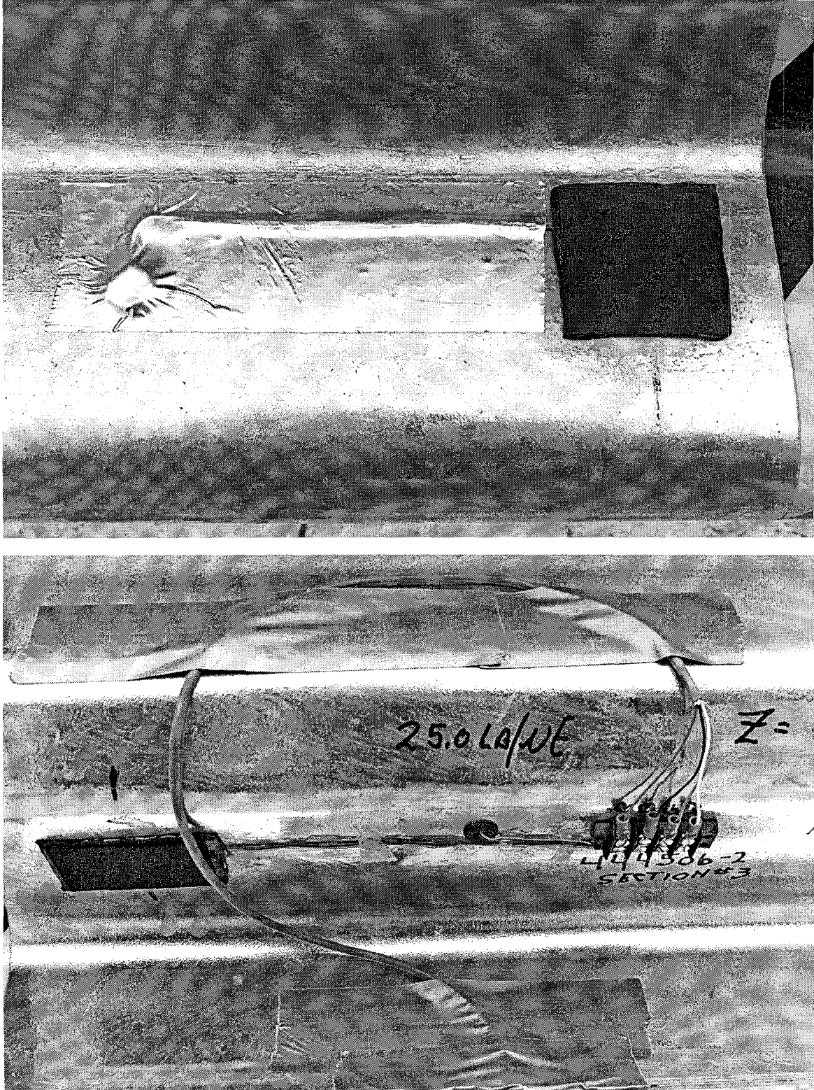
Figure 11. Strain gage installation on W-beam rail for test 473750-4.
