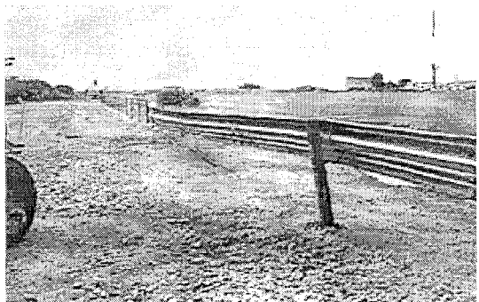
Figure 14. Sequential photographs for test 473750-4 (rear view).
