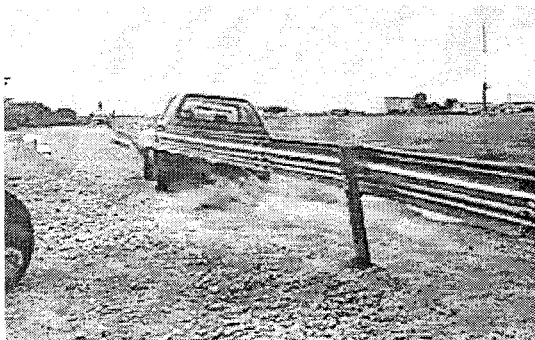
Figure 14. Sequential photographs for test 473750-4 (rear view).
