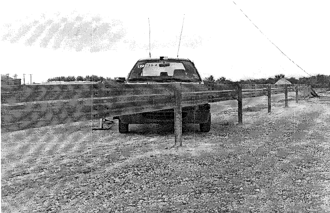
Figure 4. Vehicle/installation geometrics for test 473750-4.
