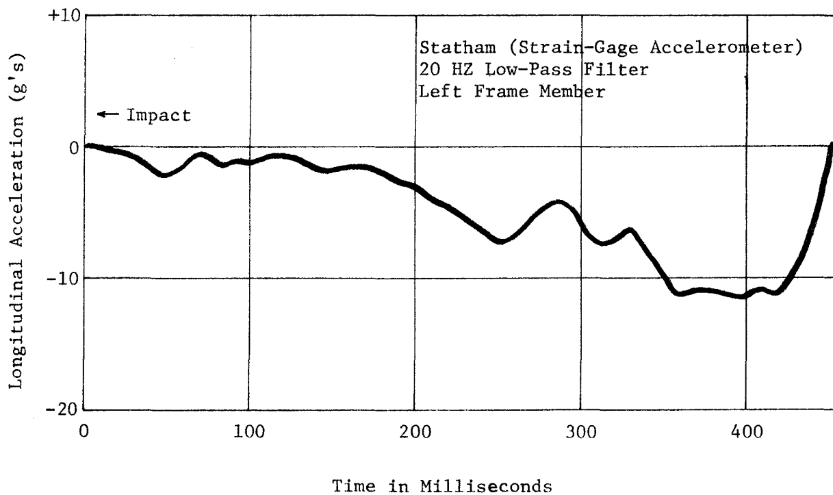
Figure A8, Longitudinal Accelerometer Data, Test 505 B-D.
