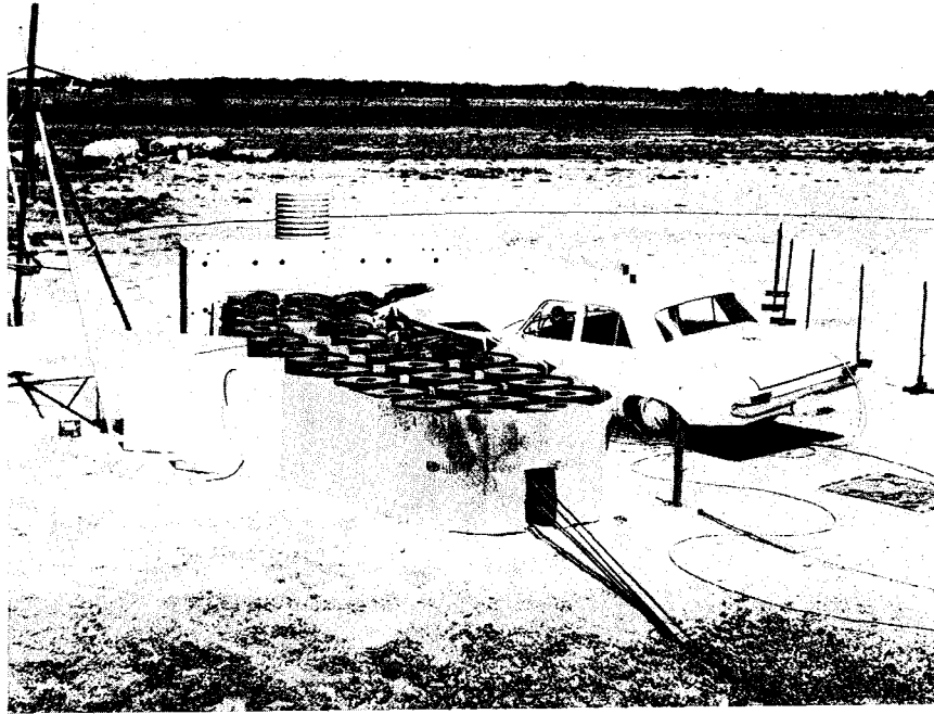
Figure 9, Crash Area After Test 505 B-A.
