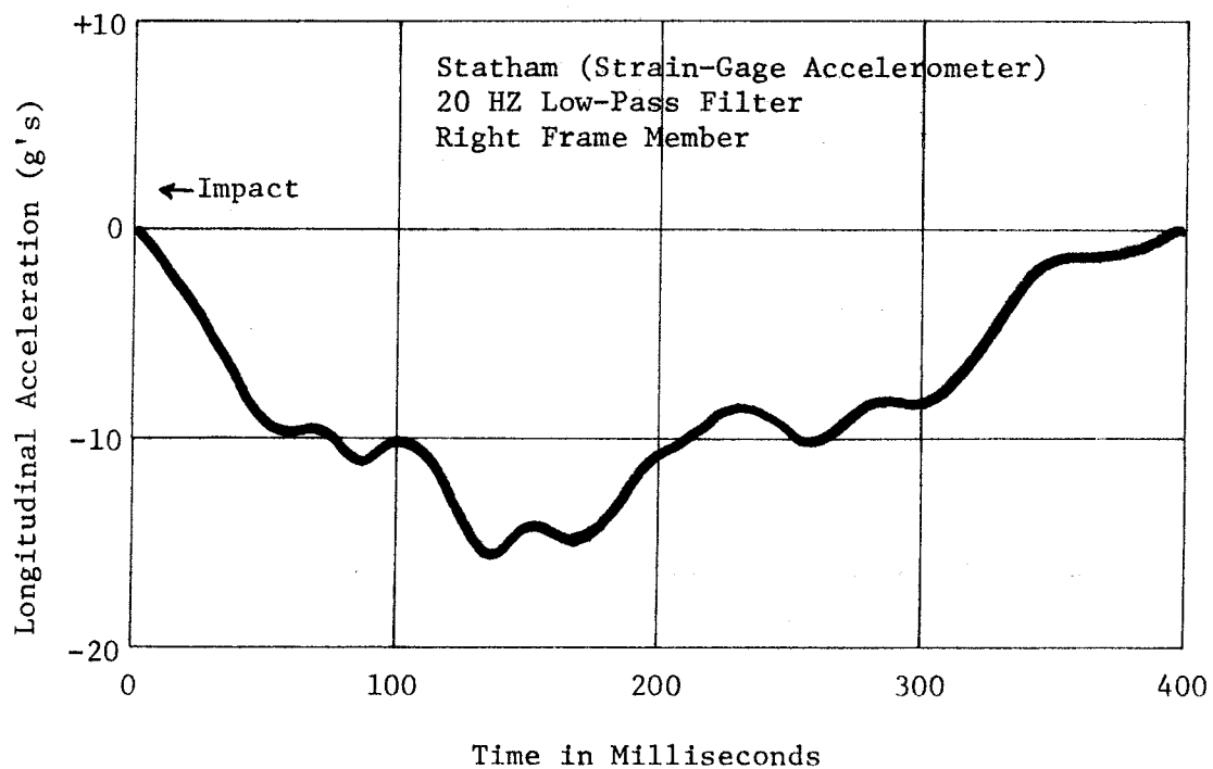
Figure A10, Longitudinal Accelerometer Data, Test 505 B-E.
