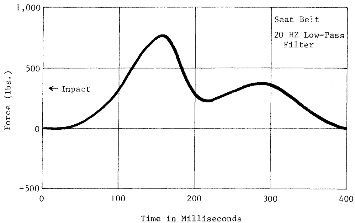
Figure A11, Seat Belt Data, Test 505 B-E.
