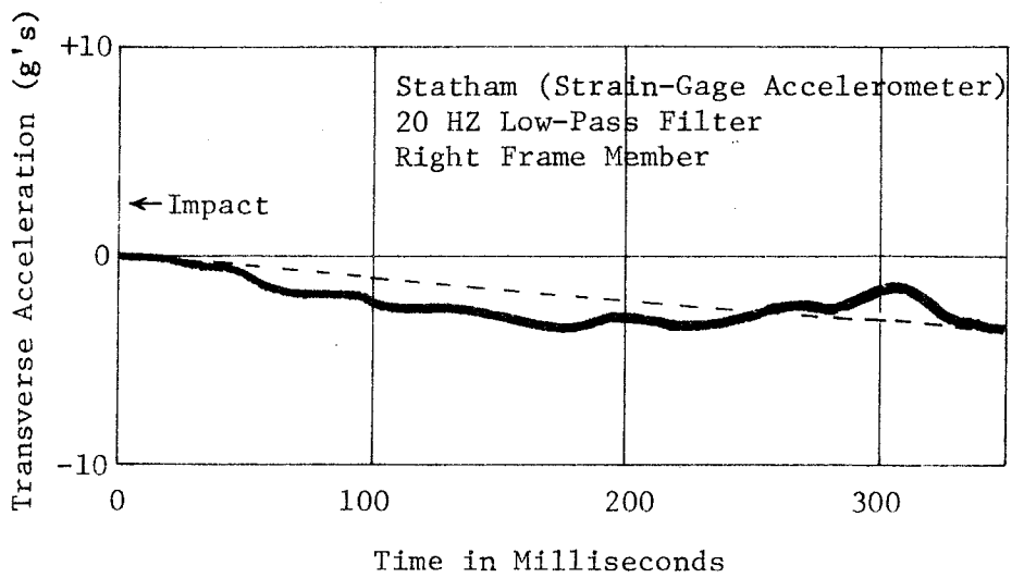
Figure A3, Transverse Accelerometer Data, Test 505 B-A.
