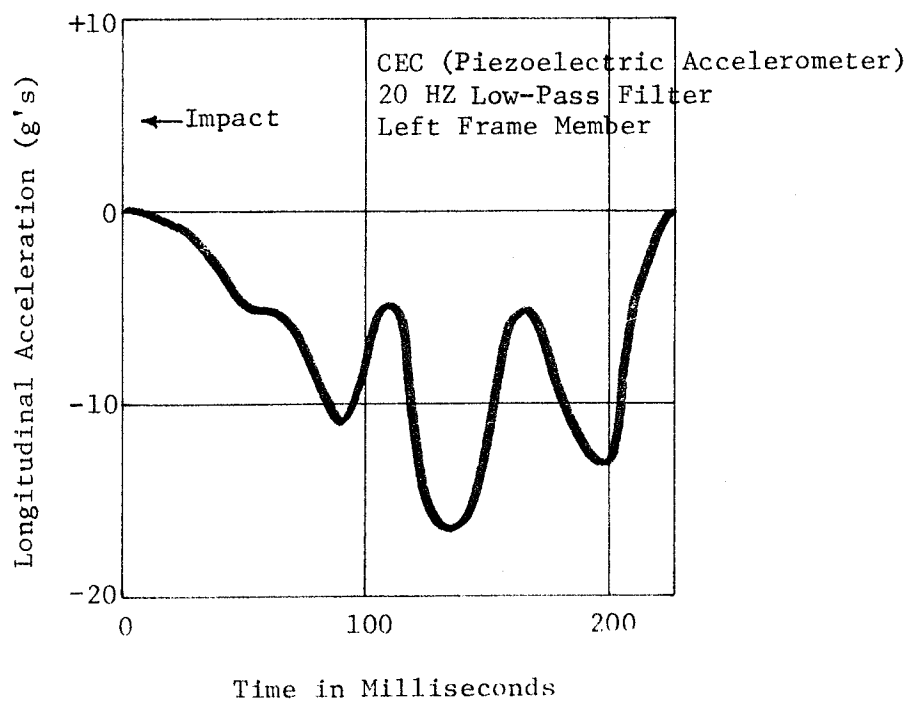
Figure A5, Longitudinal Accelerometer Data, Test 505 B-B.
