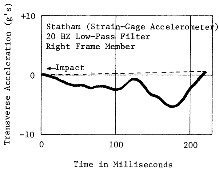
Figure A6, Transverse Accelerometer Data, Test 505 B-B.
