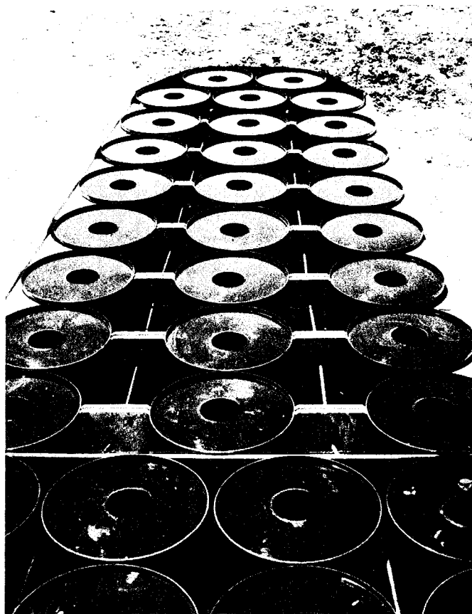
Figure 4, Modular Crash Cushion Before Test 505 B-A.
