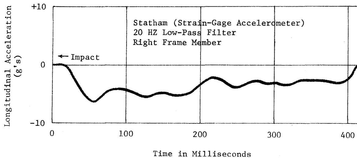
Figure A7, Longitudinal Accelerometer Data, Test 505 B-C.
