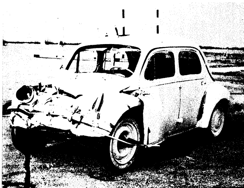
Figure 29, Vehicle After Test 505 B-E.
