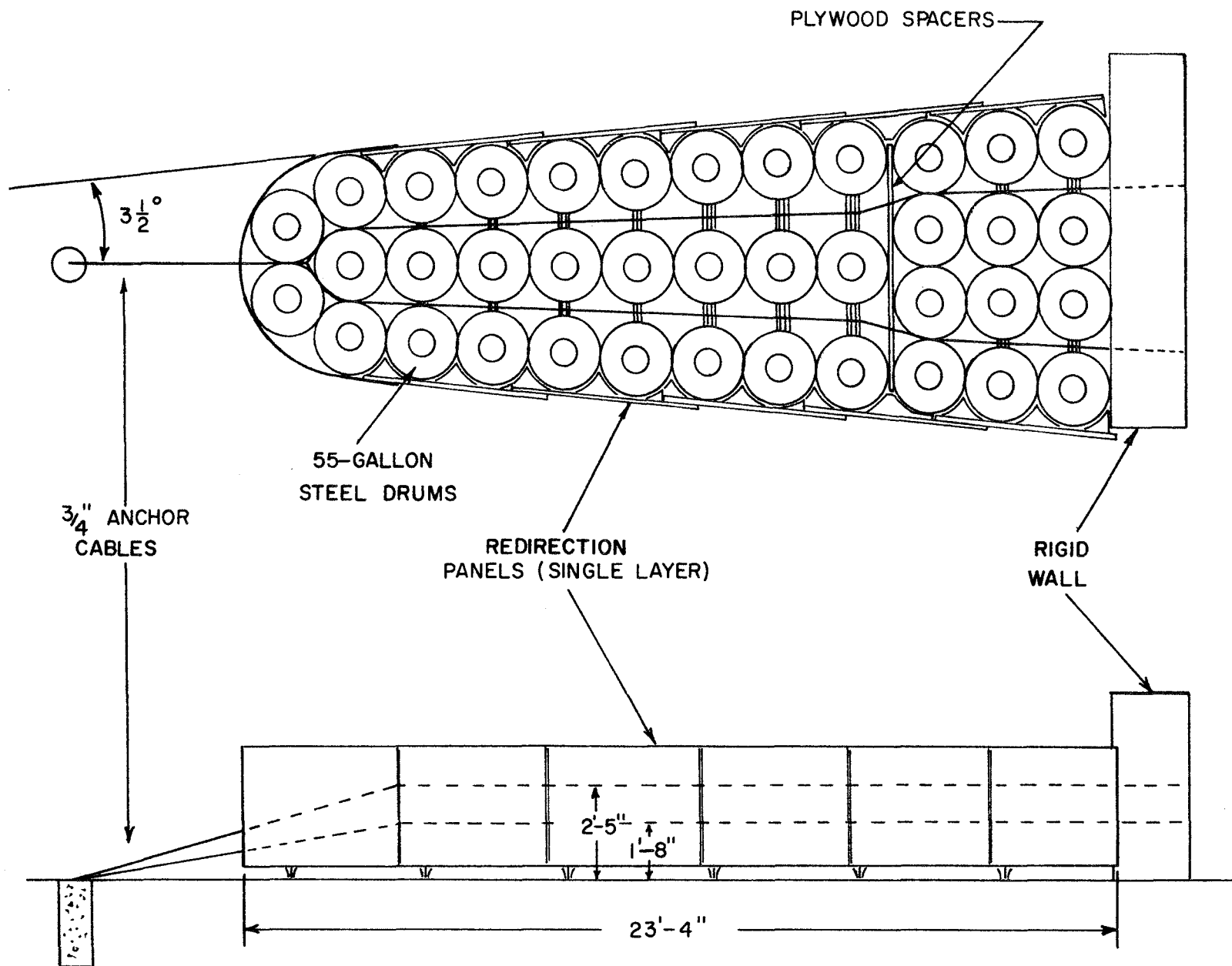
FIGURE I, CONFIGURATION USED IN TEST 505B-A (BARRIER TYPE I)
