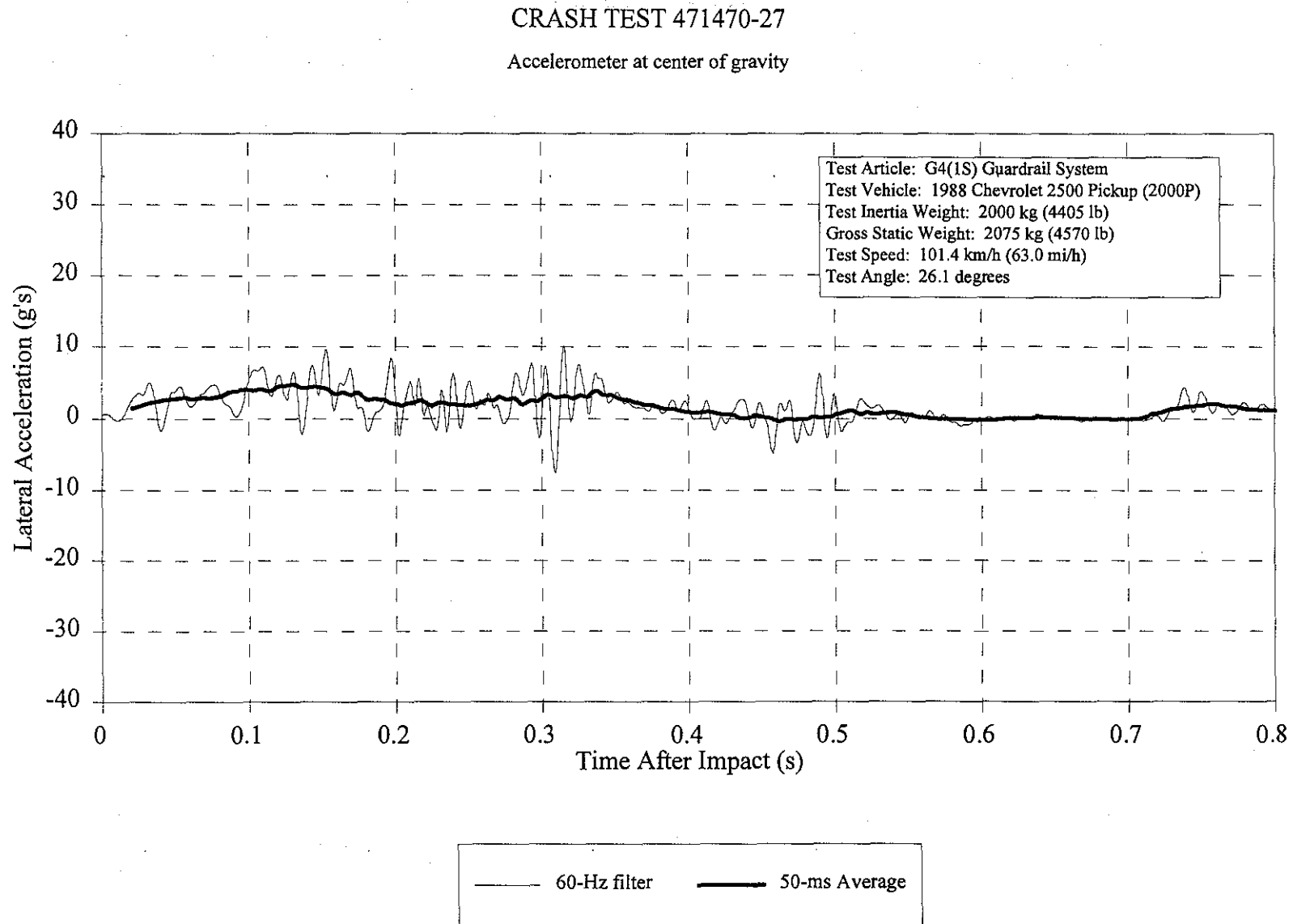
Figure 97. Vehicle lateral accelerometer trace for test 471470-27.
