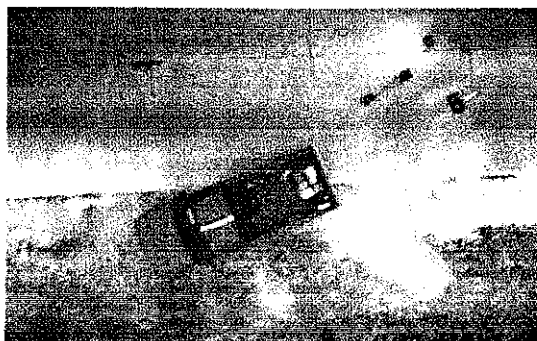
Figure 14. Sequential photographs for test 471470-28 (overhead and frontal views).
