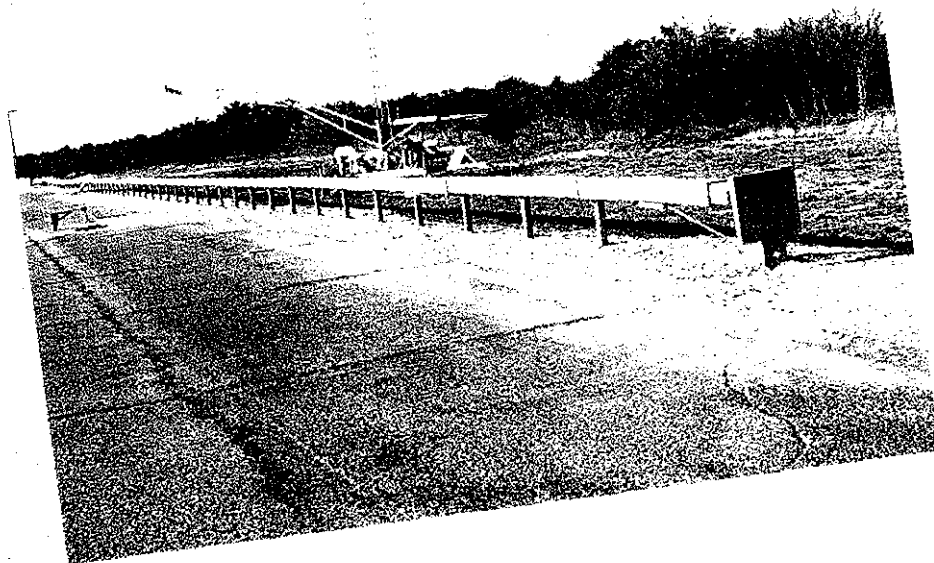
Figure 52. Box-beam (G3) guardrail installation used for test 471470-33.
