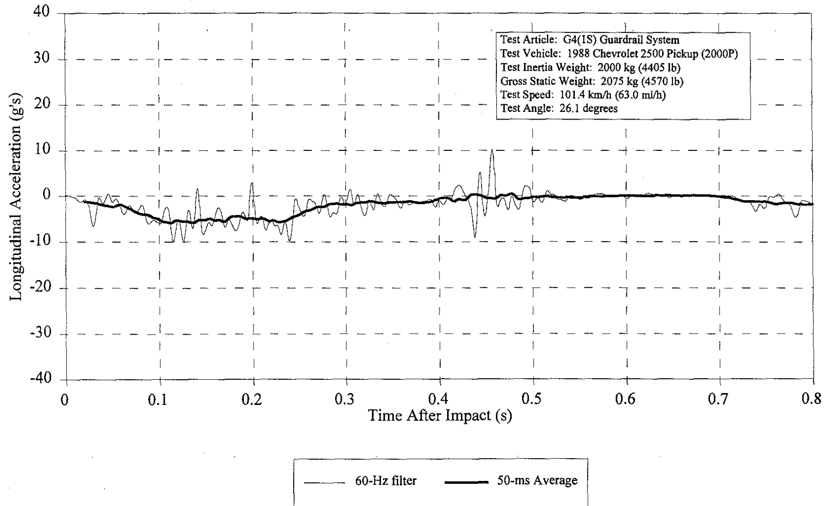
Figure 96. Vehicle longitudinal accelerometer trace for test 471470-27.
