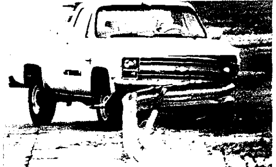
Figure 29. Sequential photographs for test 471470-21 (overhead and frontal views).
