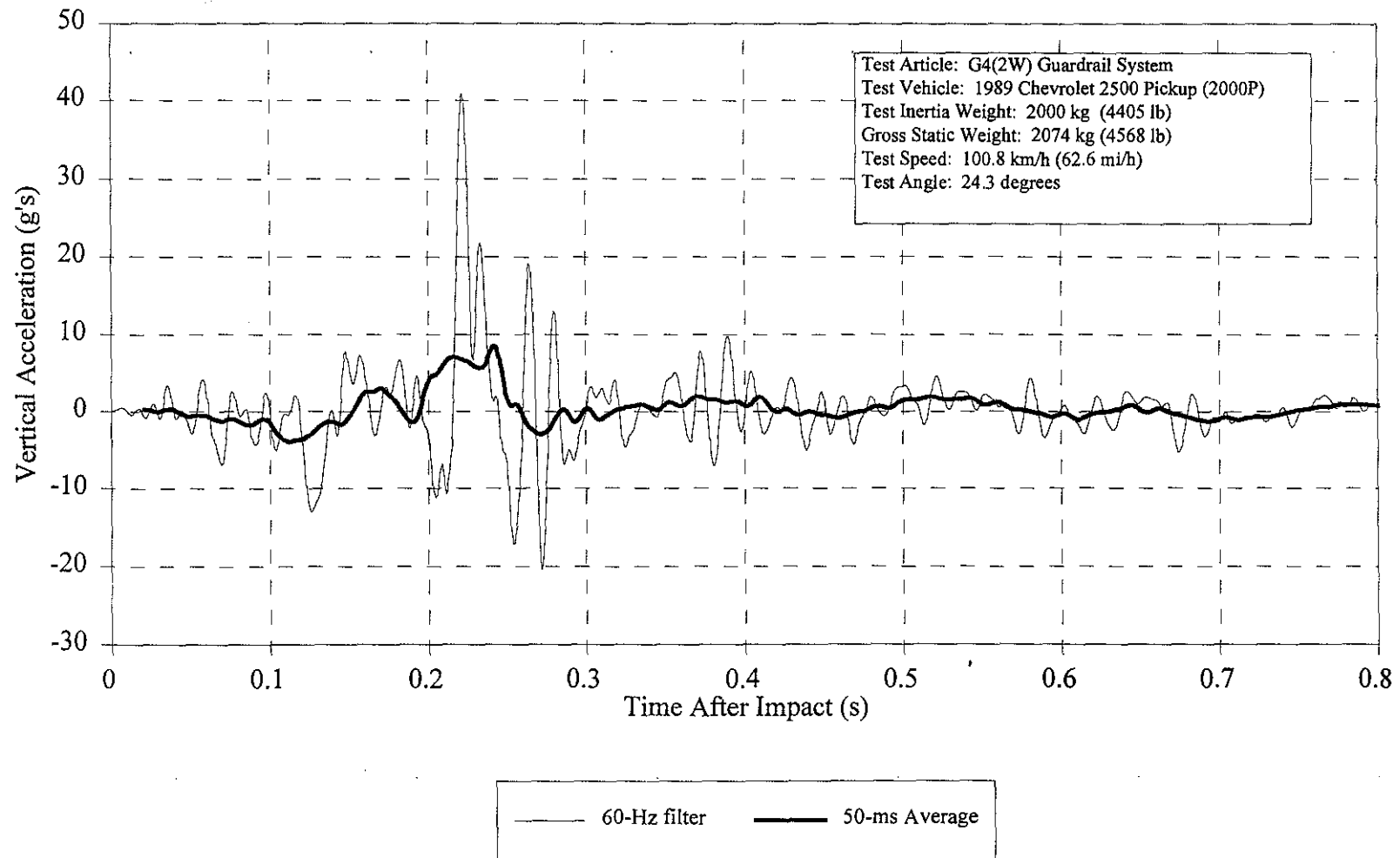
Figure 82. Vehicle vertical accelerometer trace for test 471470-26.
