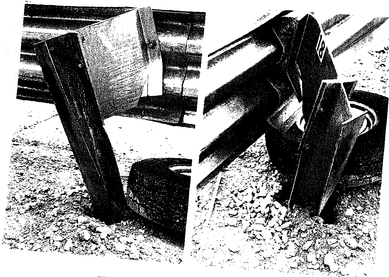
Figure 128. Damage at post 18, test 471470-30.
