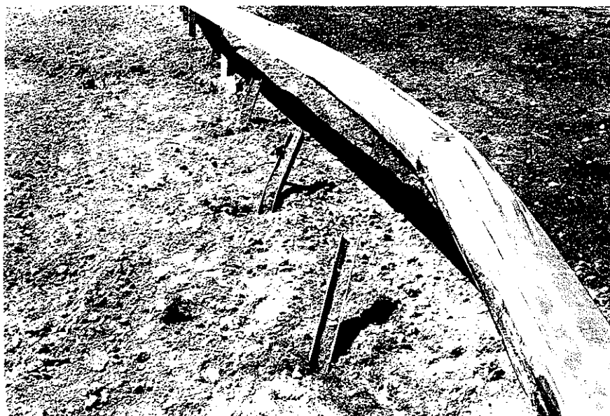
Figure 61. Damage at post 16, test 471470-33.
