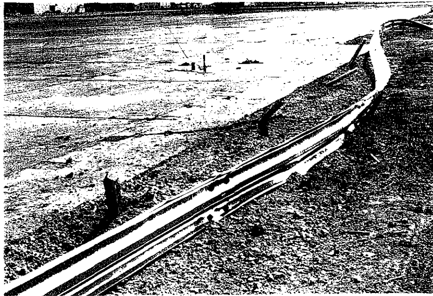
Figure 31. W-beam, weak-post (G2) guardrail after test 471470-21.
