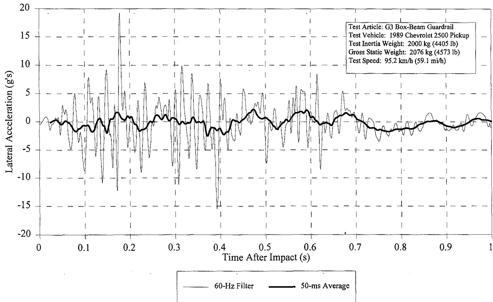
Figure 66. Vehicle lateral accelerometer trace for test 471470-33.
