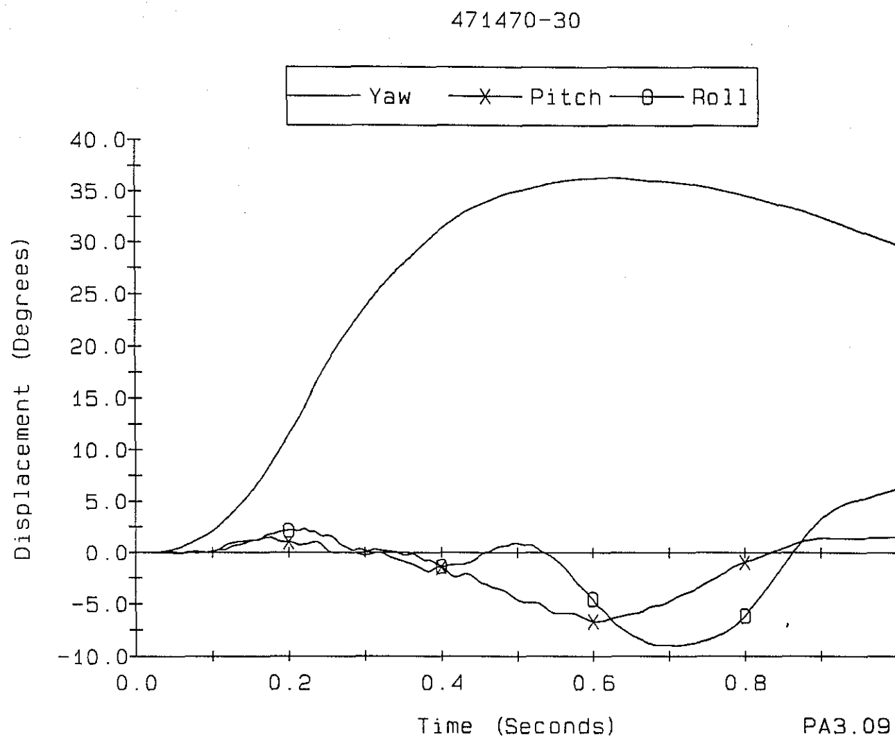
Figure 131. Vehicle angular displacements during test 471470-30.
