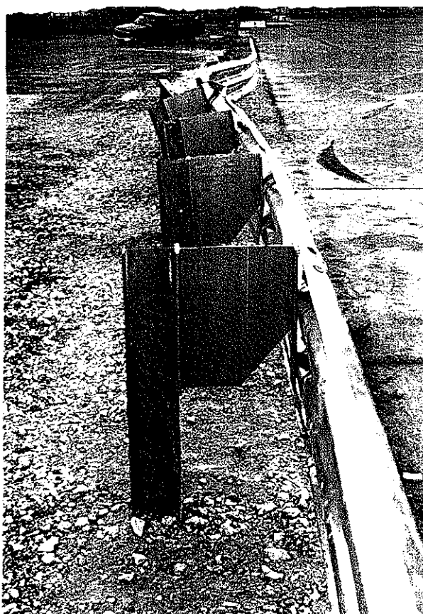
Figure 124. Modified thrie-beam guardrail after test 471470-30.
