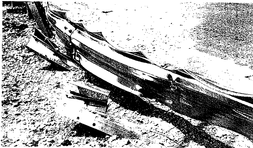
Figure 91. Damage at posts 14 through 17, test 471470-27.
