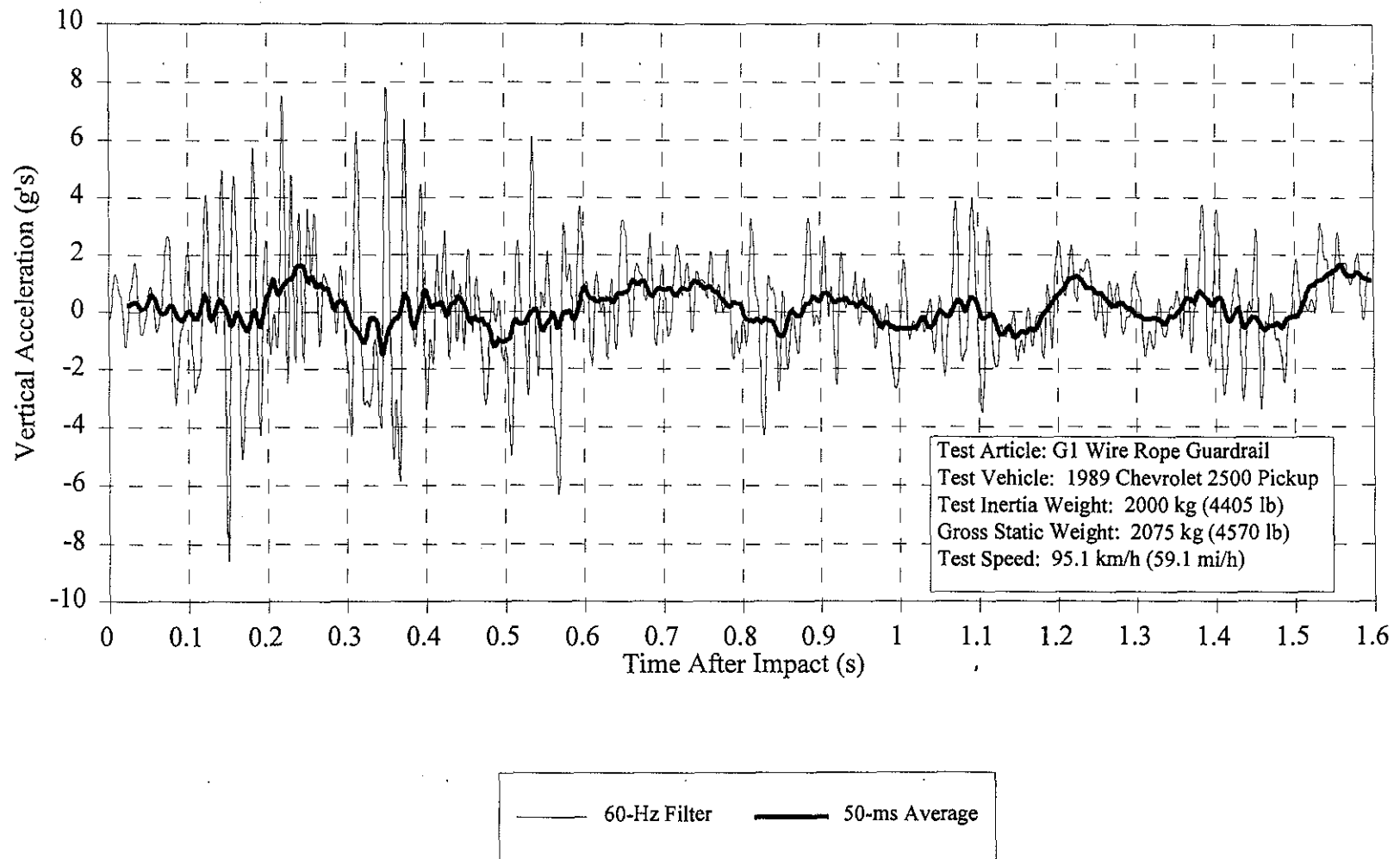
Figure 23. Vehicle vertical accelerometer trace for test 471470-28.
