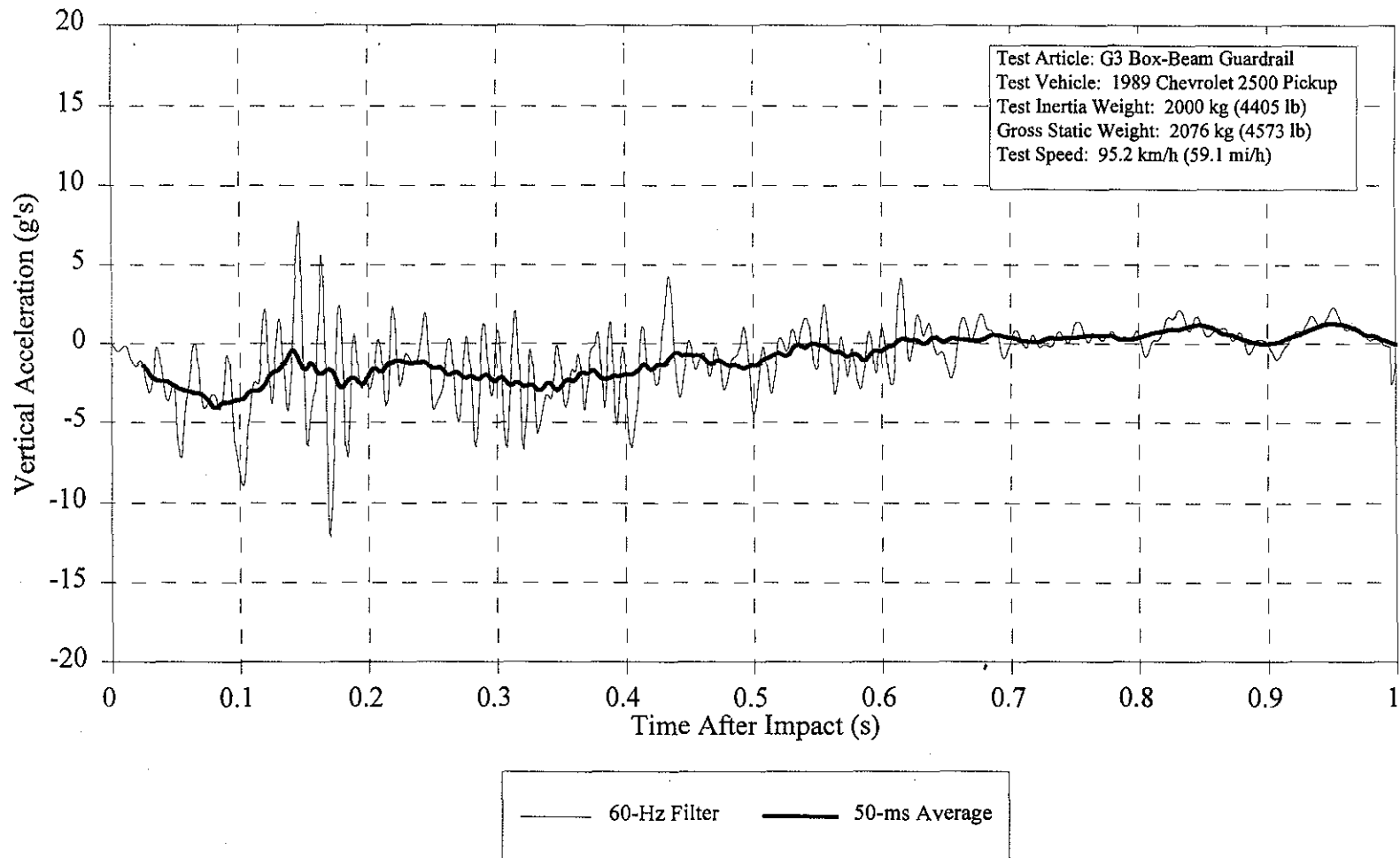
Figure 67. Vehicle vertical accelerometer trace for test 471470-33.
