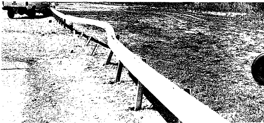
Figure 59. Box-beam (G3) guardrail after test 471470-33.
