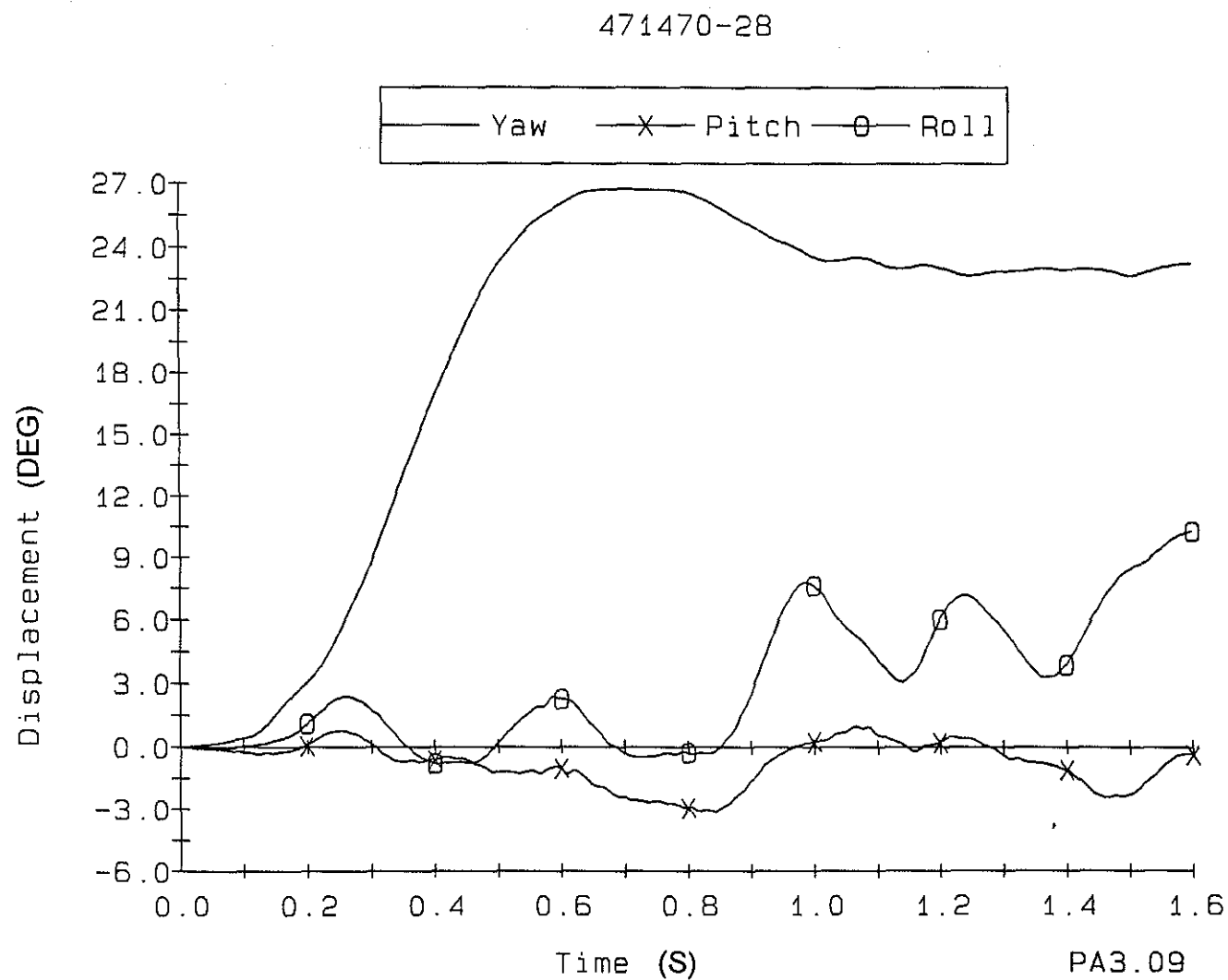
Figure 20. Vehicle angular displacements during test 471470-28.
