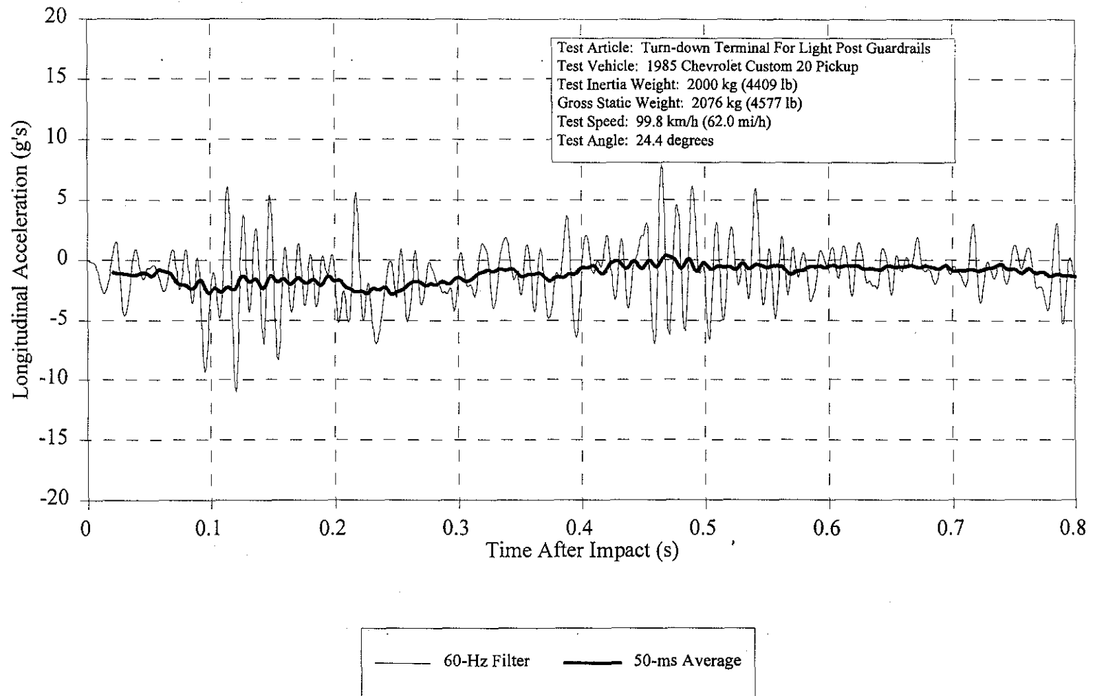
Figure 35. Vehicle longitudinal accelerometer trace for test 7147-21.
