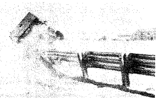
Figure 106. Sequential photographs for test 471470-31 (rear and interior views) (continued).
