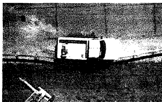
Figure 57. Sequential photographs for test 471470-33 (overhead and frontal views).
