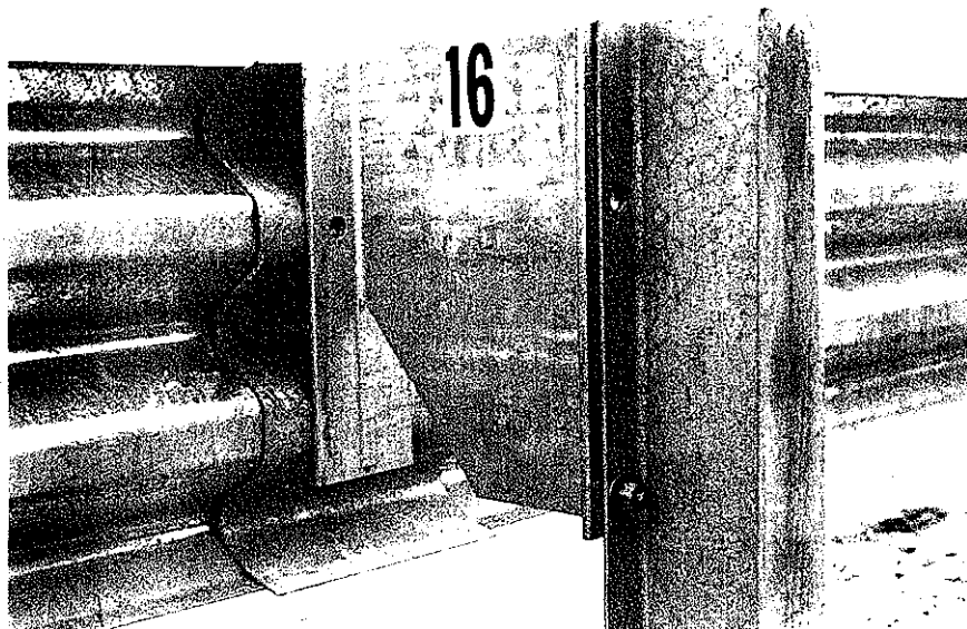
Figure 118. Modified three-beam guardrail section before test 471470-30.
