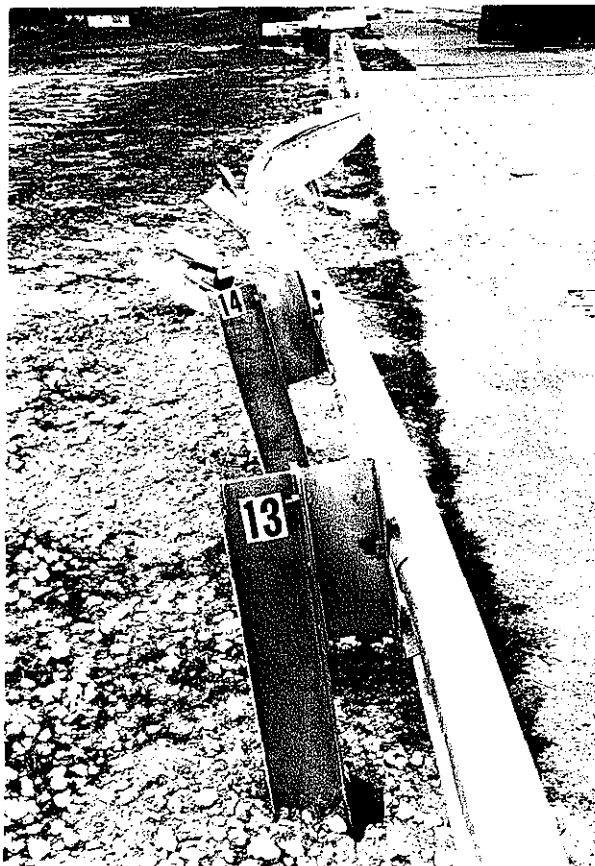
Figure 90. W-beam, steel-post (G4(1S)) guardrail installation after test 471470-27.
