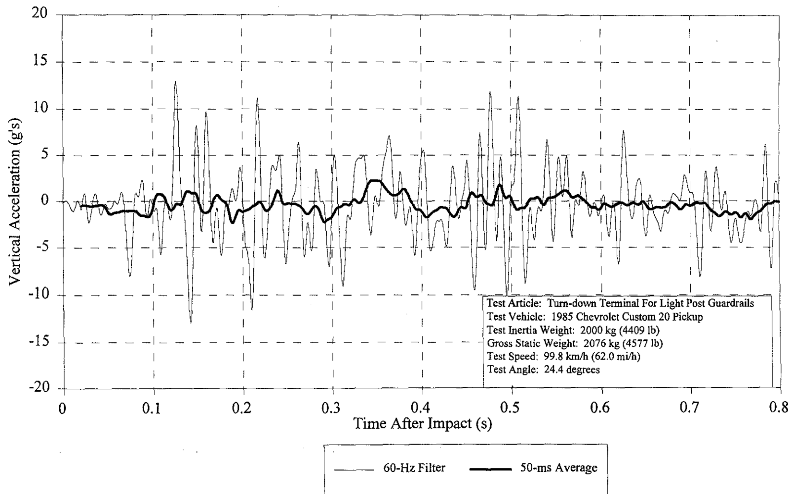
Figure 37. Vehicle vertical accelerometer trace for test 7147-21.
