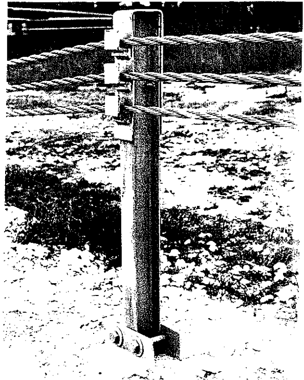
Figure 10. Anchor for the cable (G1) guardrail before test 471470-28.
