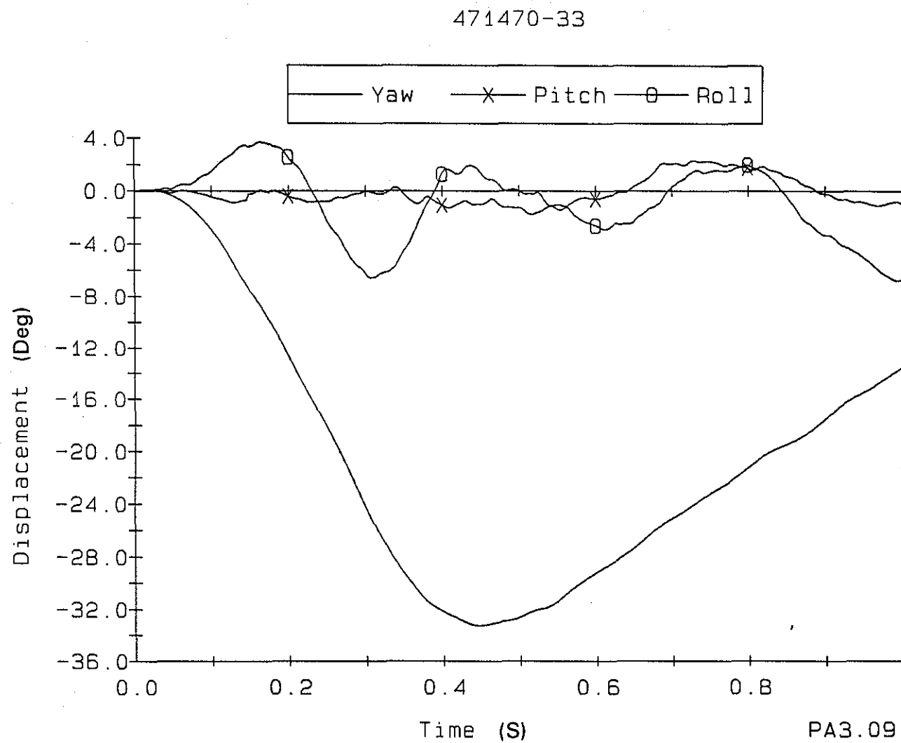
Figure 64. Vehicle angular displacements during test 471470-33.
