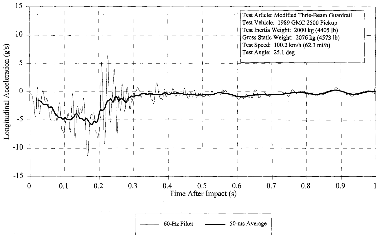
Figure 132. Vehicle longitudinal accelerometer trace for test 471470-30.
