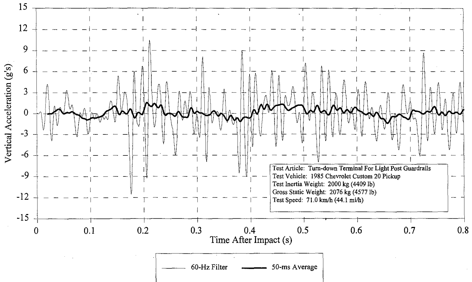
Figure 50. Vehicle vertical accelerometer trace for test 7147-22.
