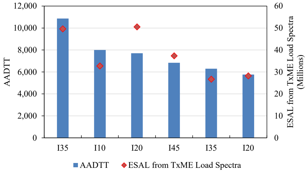
Figure 5. Comparison of AADTT for IHs.
