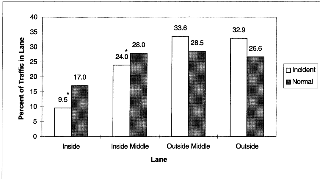
FIGURE C-11. Lane Distribution at Morningside (6/8/95)
