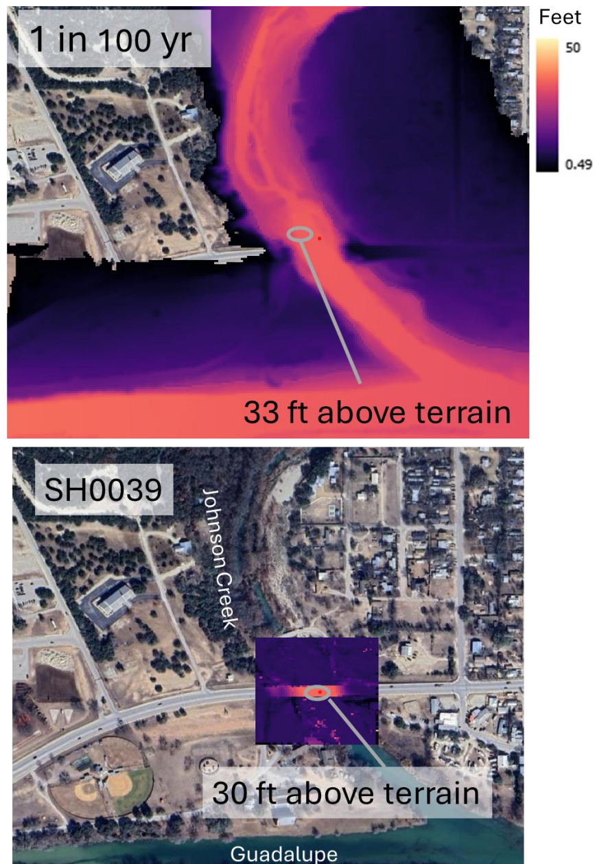
Figure 50. Example Flood Depth and LIDAR Data Integration Used to Assess Risk.
