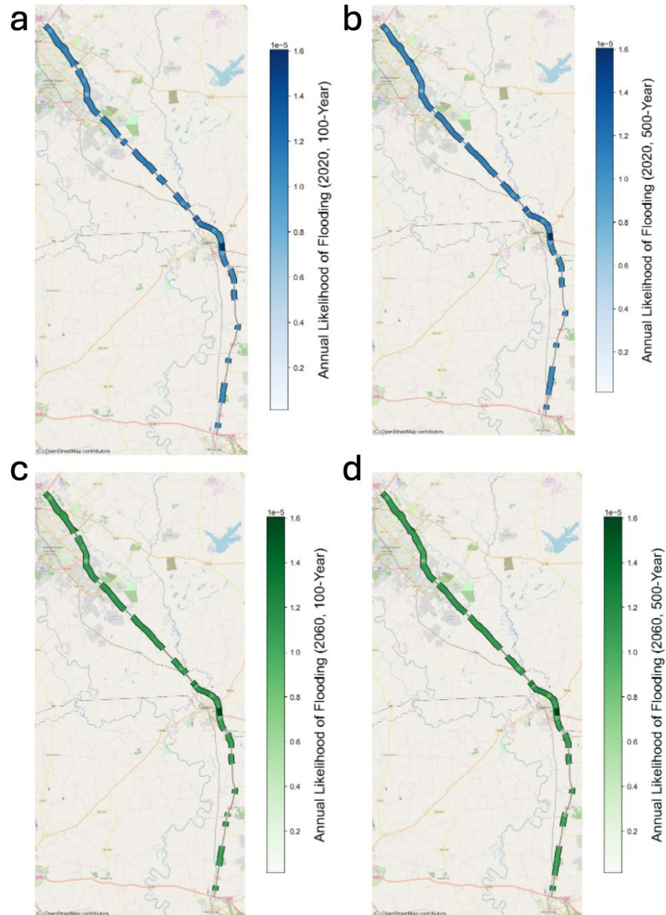
Figure C-10. Annual Likelihood of Flooding for the SH0006—Bryan/College Station to Hempstead US290 Case Study: (a) 100-Year Return Period and 2020 Scenario, (b) 500-Year Return Period and 2020 Scenario, (c) 100-Year Return Period and 2060 Scenario, and (d) 500-Year Return Period and 2060 Scenario.
