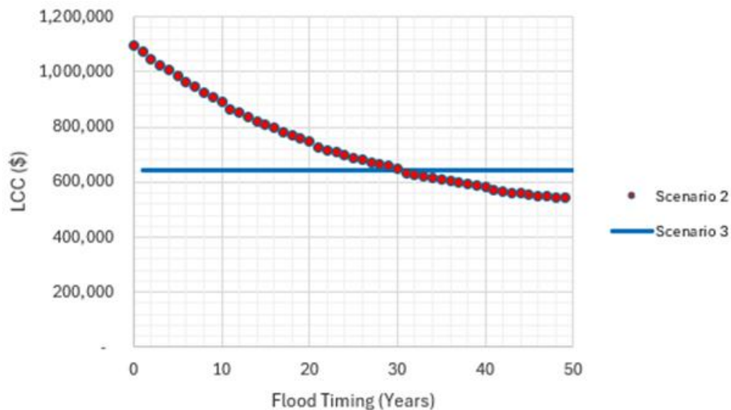
Figure 42. LCC per Lane-Mile Versus Flood Timing for a 50-Year Flood.
