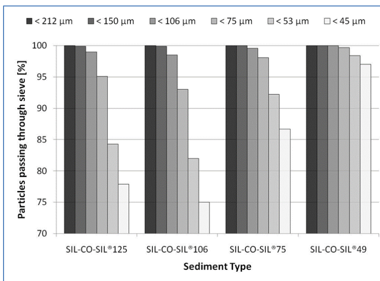
Figure 3. Particle Size Distributions.
