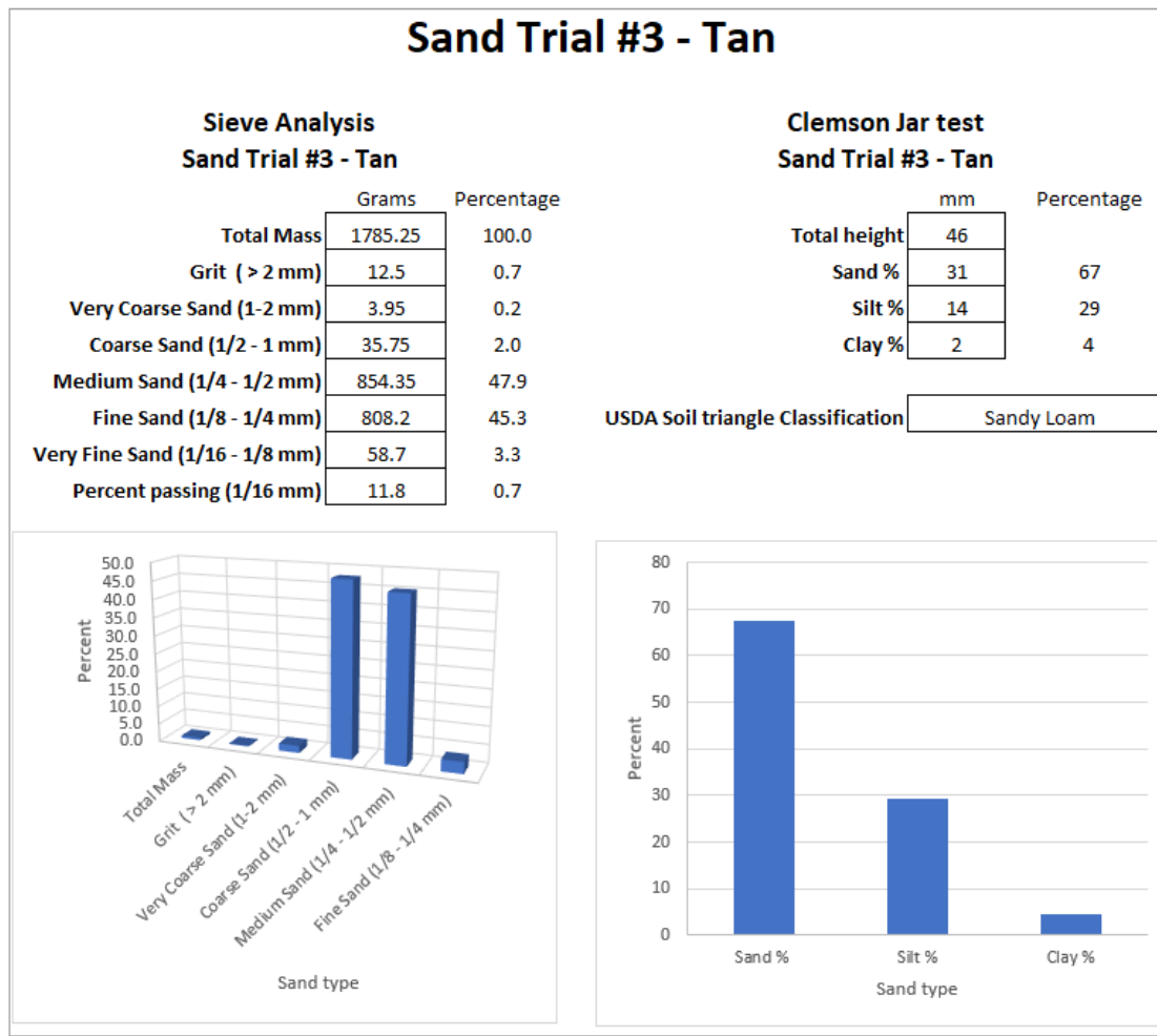
Figure 5. Test Results for Selected Sand (Sand Trial #3-Tan).
