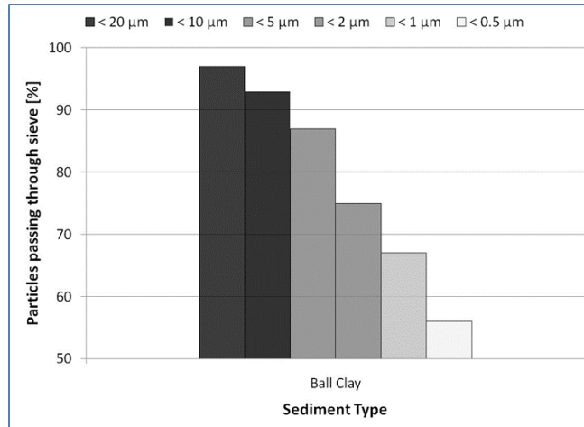
Figure 4. Ball Clay PSD.
