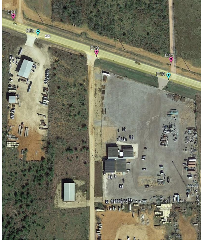
Figure 12. FM 468 August 2022 One-Lane Section near Driveways 18 and 20.
