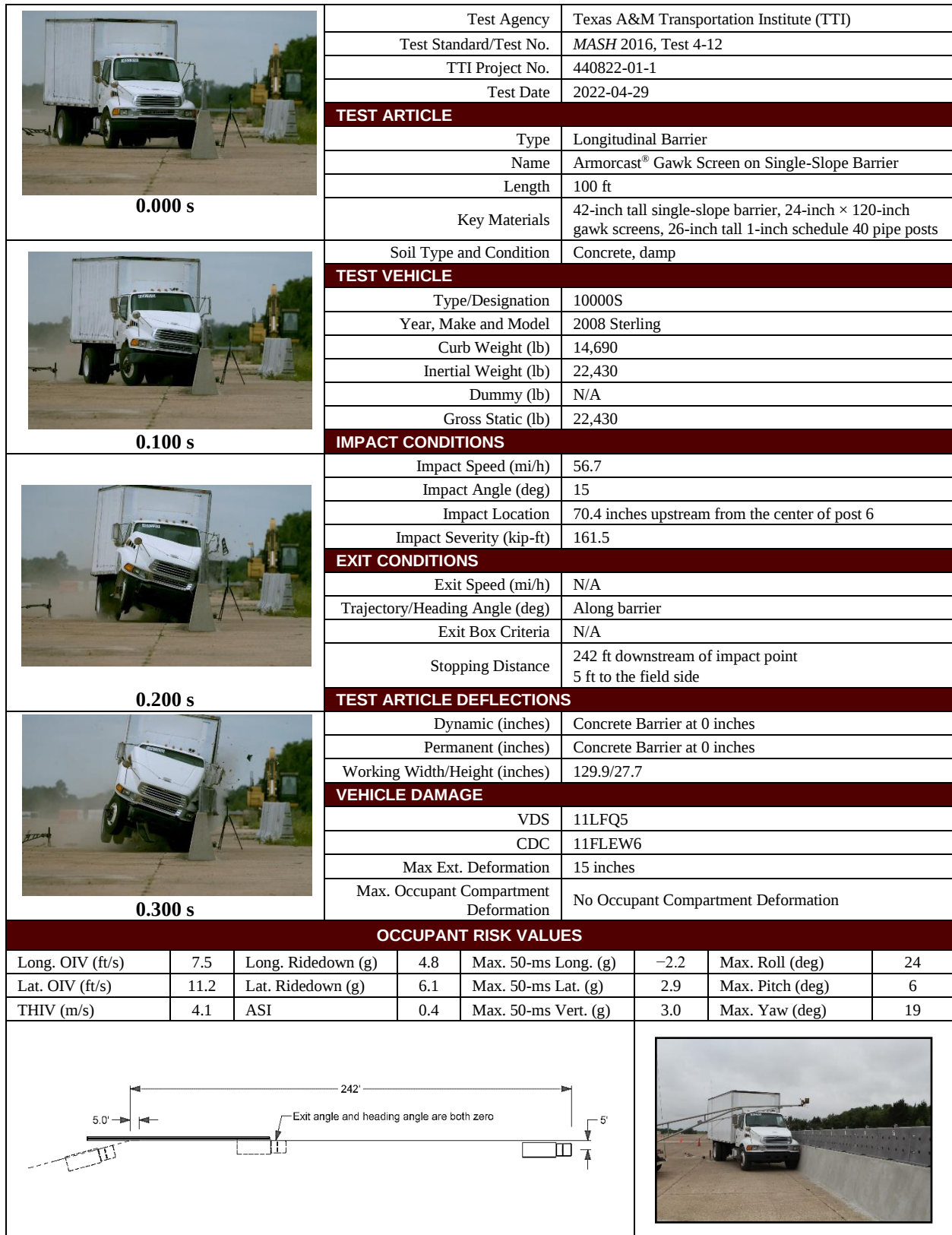
Figure 6.1. Summary of Results for MASH Test 4-12 on Armorcast® Gawk Screen on Single-Slope Barrier.
