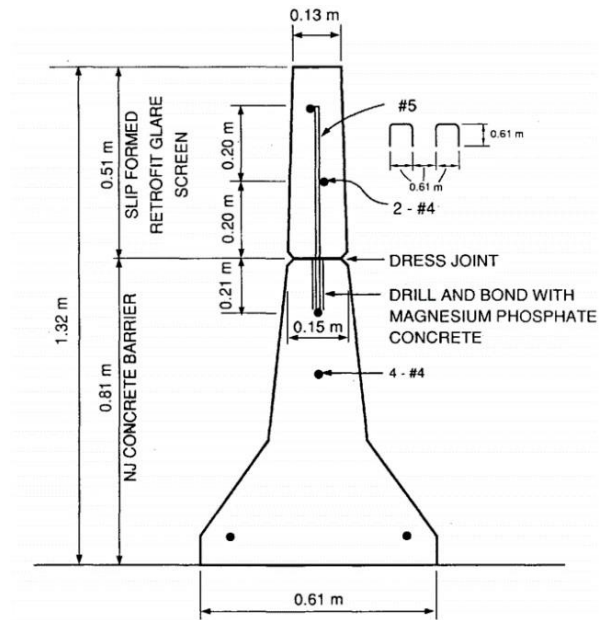
Figure 2.6. Reinforced Concrete Glare Screen.
