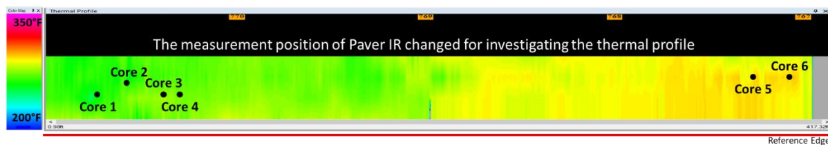
Figure 74. SH 105 Thermal Plot with Core Locations.
