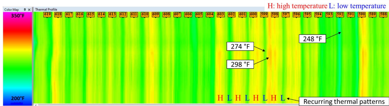
Figure 51. US 183 Thermal Profile.
