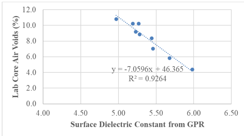
Figure 31. GPR Results from US 69 Cores.
