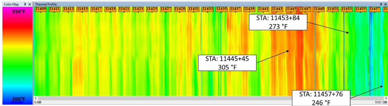
Figure 26. US 69 Thermal Profile.
