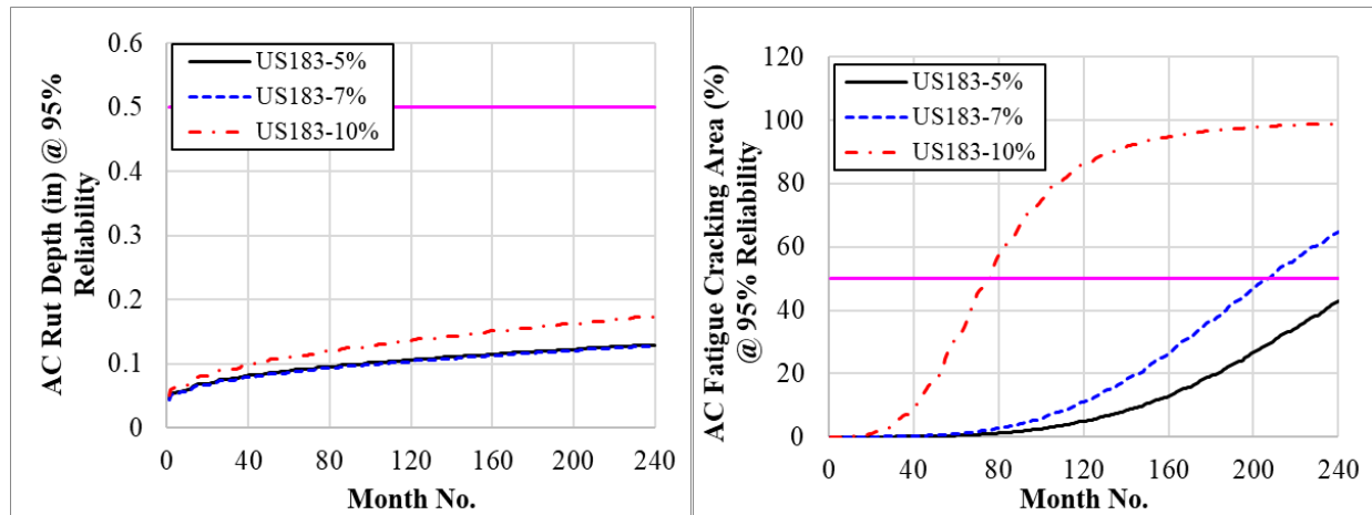
Figure 92. TxME Analysis Results—US 183 for Different AVs.
