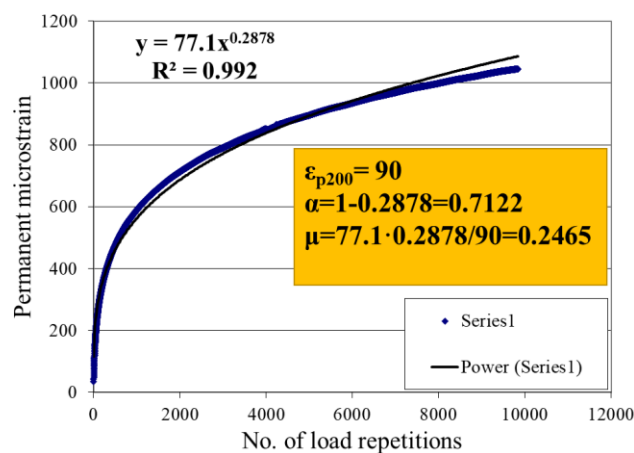
Figure 91. Permanent Deformation Curve and Data Calculation Example.
