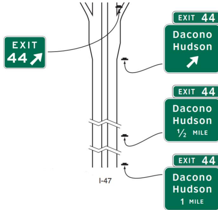
Figure 1. Interchange Exit Ramp Sign Sequence from TMUTCD (1).
