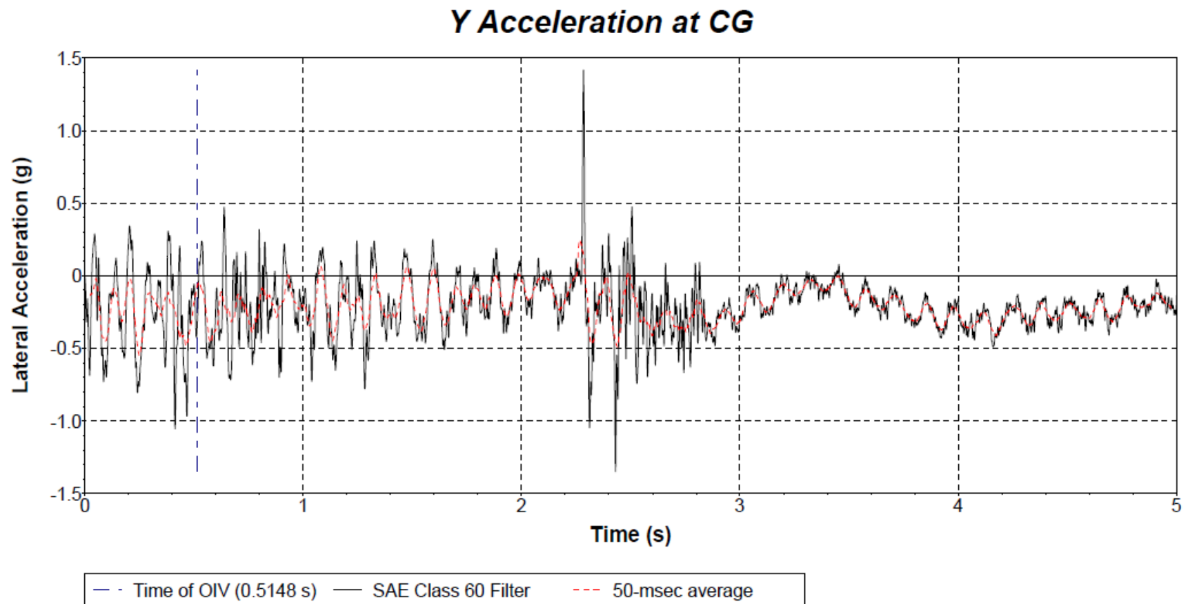
Figure F.7. Vehicle Lateral Accelerometer Trace for Test 440211-01-5 (Accelerometer Located at Horizontal Center of Gravity).
