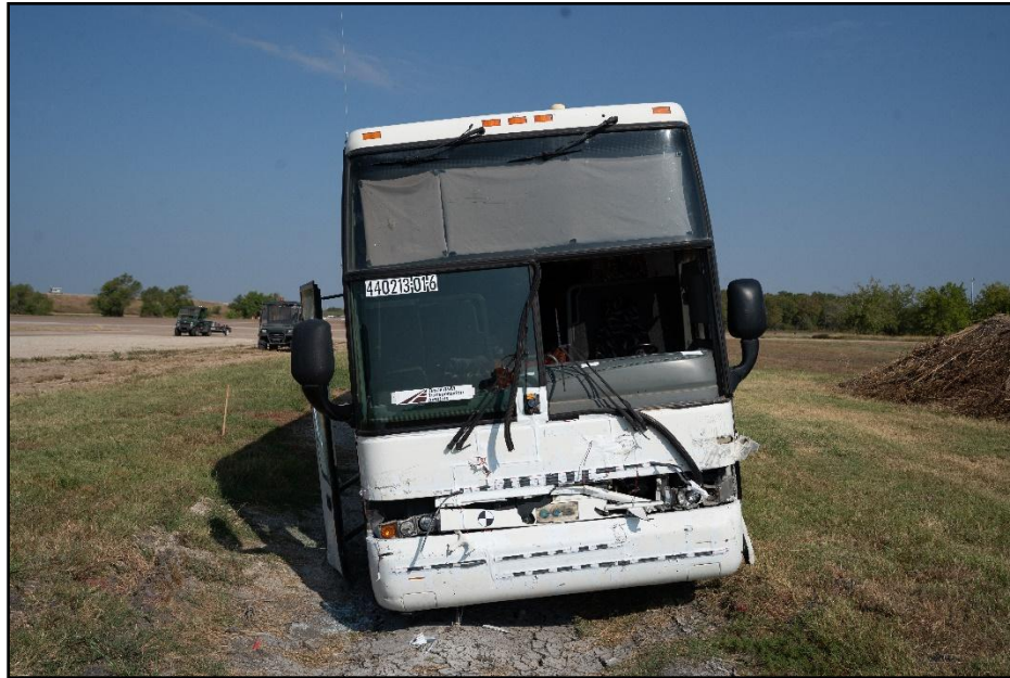
Figure 12.3. Front of Test Vehicle after Test 440213-01-6.
