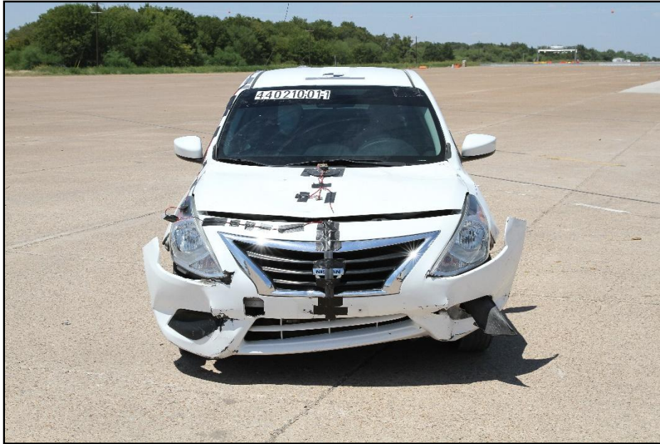
Figure 7.7. Test Vehicle after Test 440210-01-1.
