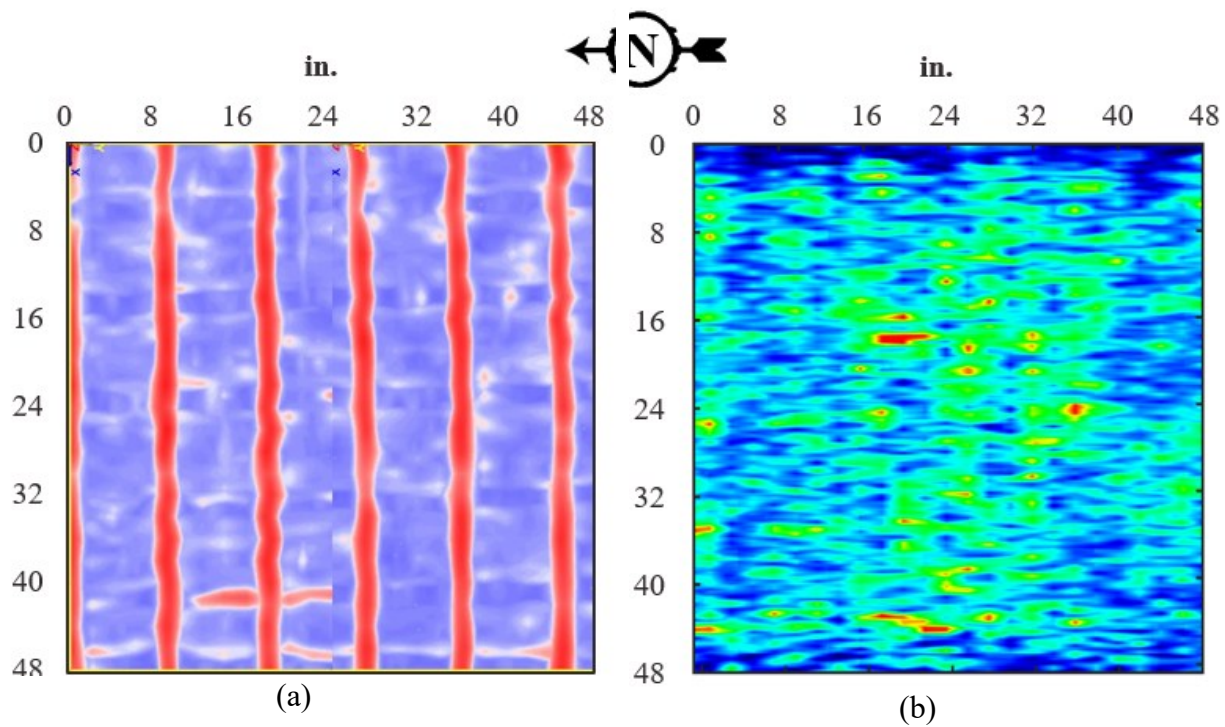
Figure 4.58. LUB4 results for the primary NDE area for (a) GPR and (b) UST of top longitudinal reinforcement at depth 2.73 in.
