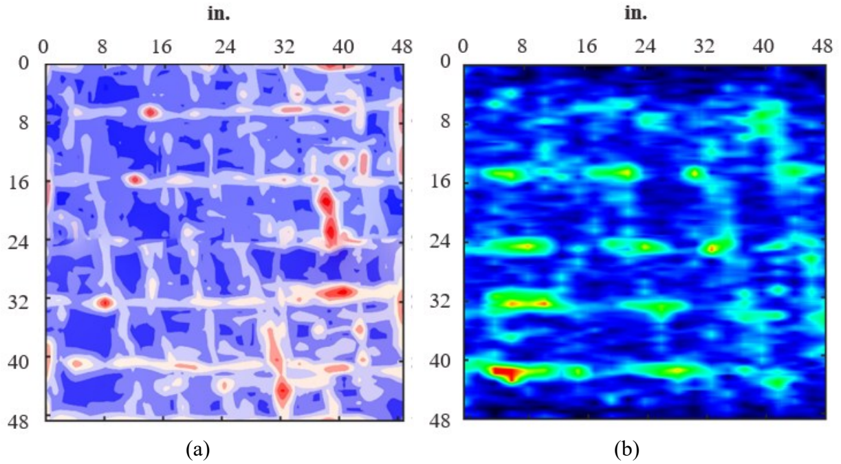
Figure 4.15. ATL2 results for (a) GPR and (b) UST of bottom longitudinal reinforcement at depth 7.23 in.
