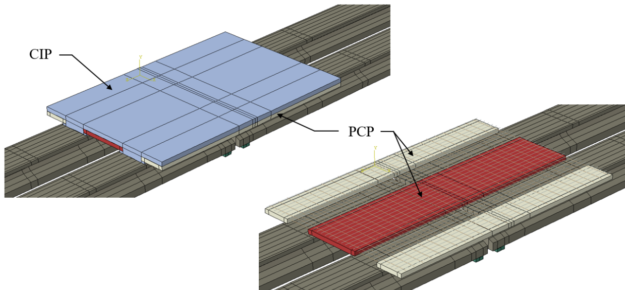
Figure 8.6. Double-girder continuous precast panel model, showing the CIP topping slab (left) and without the CIP concrete, revealing the continuous PCPs and reinforcement beneath (right).
