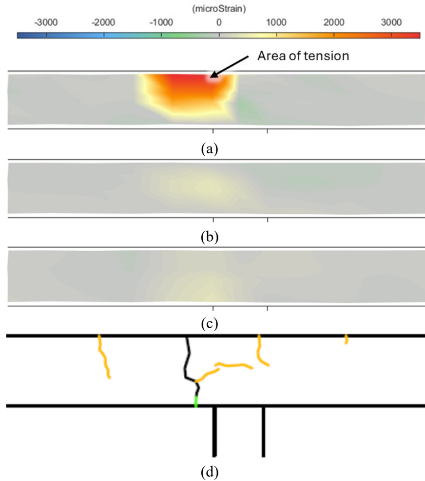
Figure 10.26. Optotrak strains for PBJ-OP2 Pattern All: (a) horizontal, (b) vertical, (c) shear strain, and (d) crack pattern.
