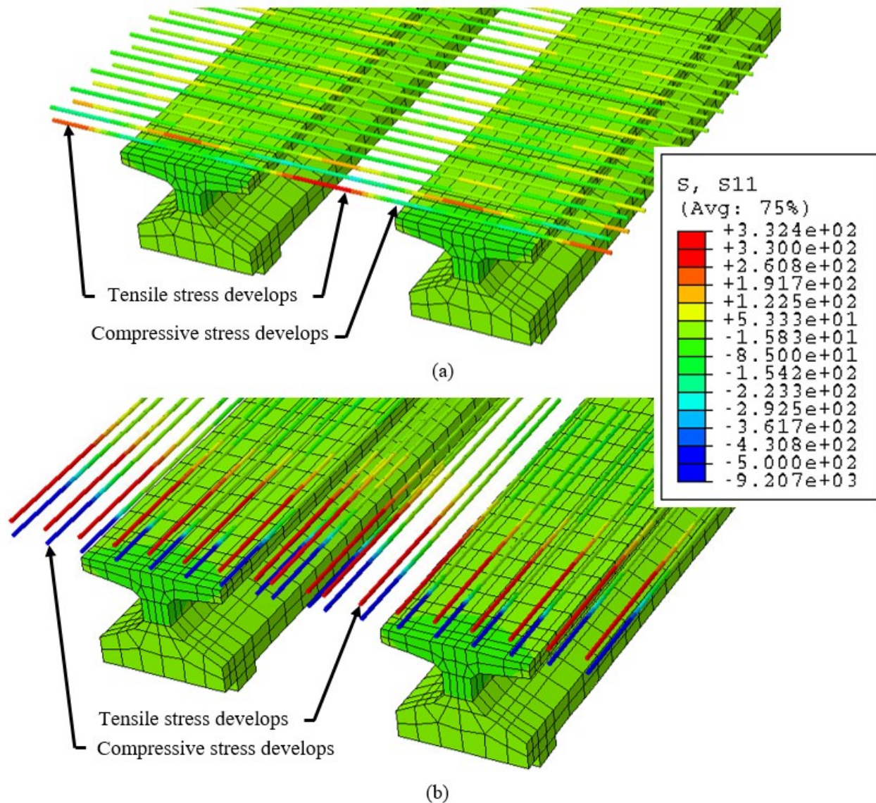
Figure 8.23. Longitudinal stresses in reinforcement (psi) for (a) transverse bars and (b) longitudinal bars at the onset of cracking.
