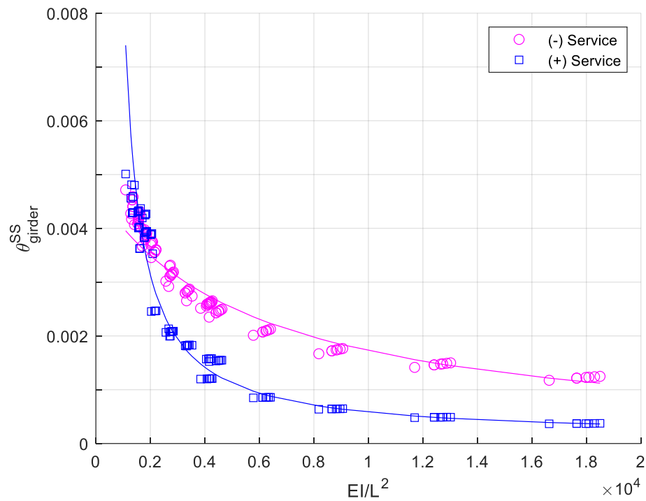
Figure 7.3. Girder end rotations for service load combinations.
