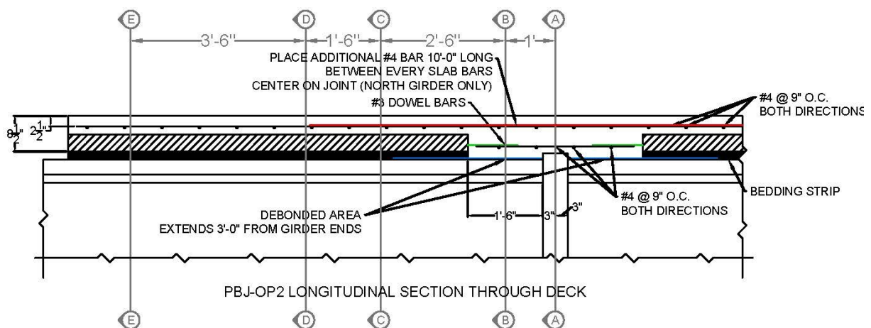
Figure 9.12. PBJ-OP2 elevation view.
