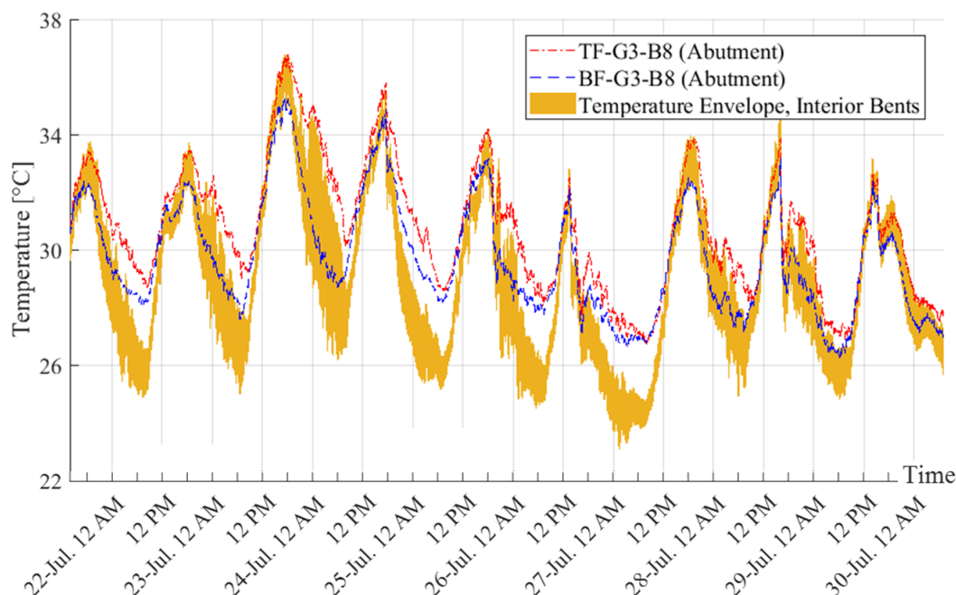
Figure 5.16. Temperature envelope for BRY3.
