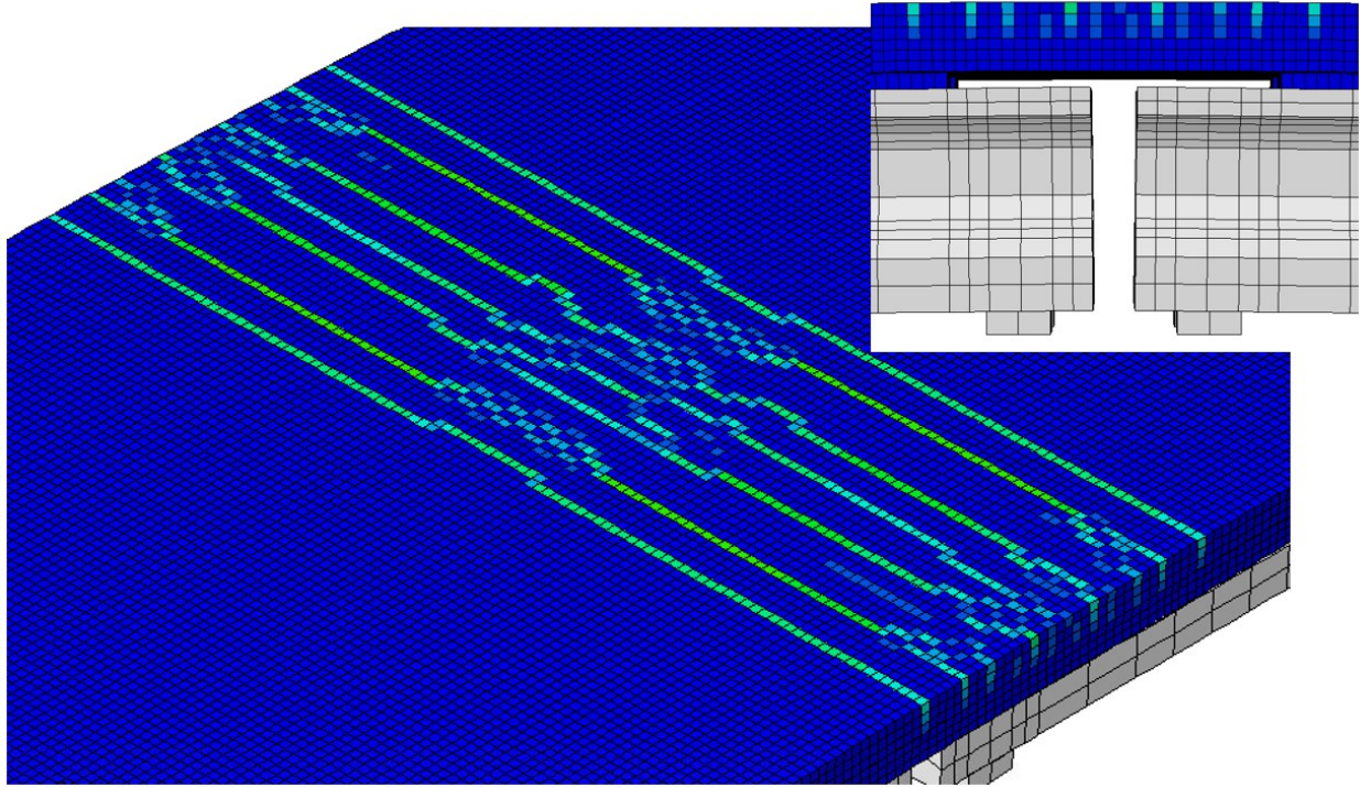
Figure 8.47. Cracking pattern for an offset precast panel model, debonded for 18 in. with a vertical gap along the debonded length, and squared ends of the debonded region.
