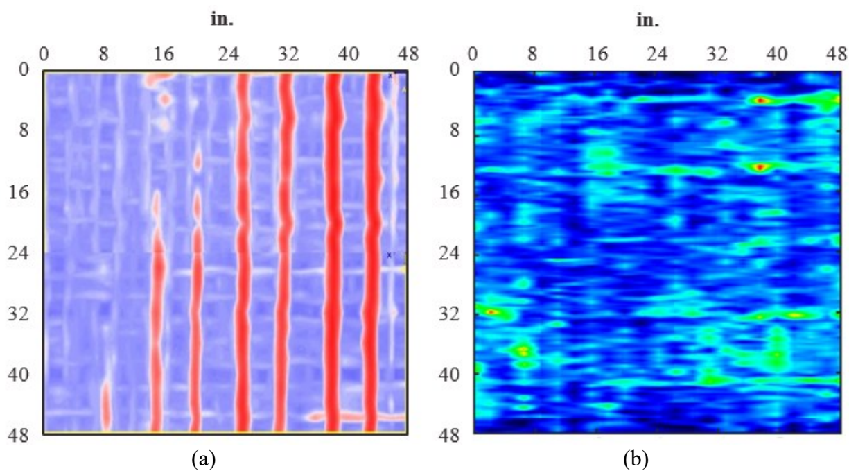
Figure 4.7. ATL1 results for (a) GPR and (b) UST of top transverse reinforcement at depth 2.23 in.
