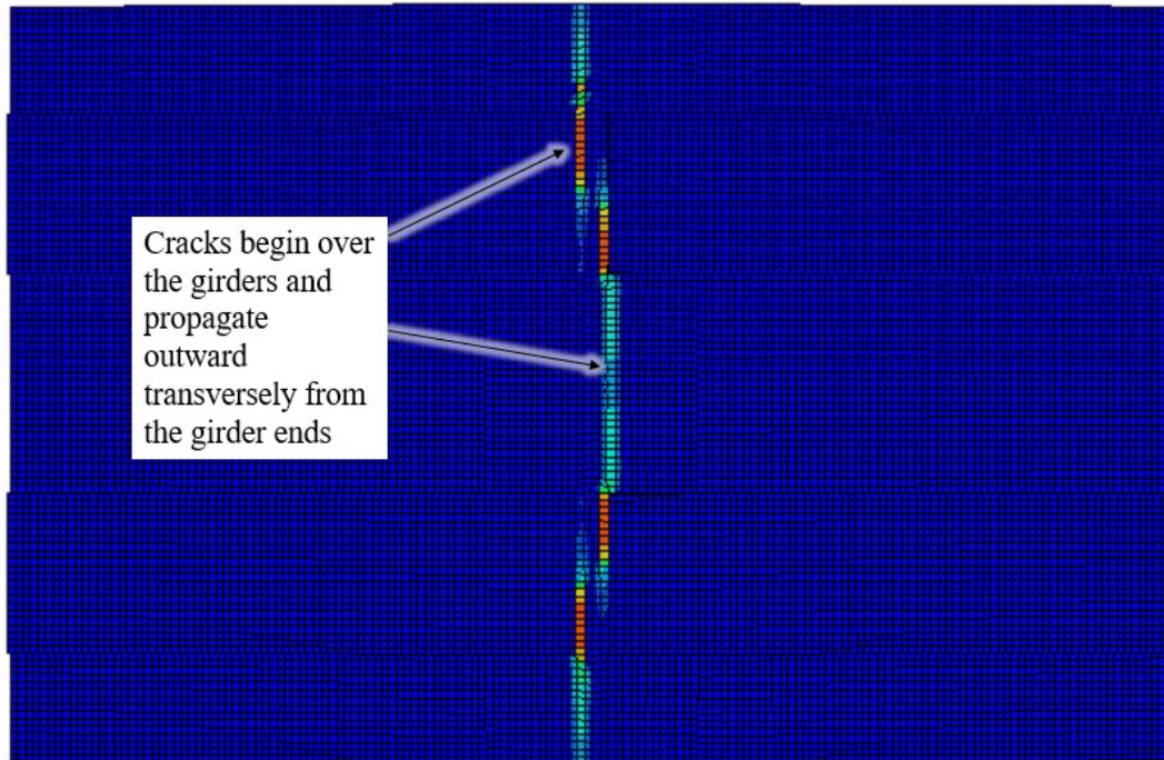
Figure 8.62. The crack pattern in the bottom of the slab for an offset precast panel model loaded with negative temperature gradient.
