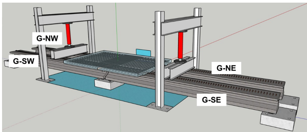
Figure 9.2. Schematic overview of test setup.
