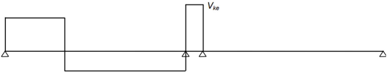
Shear force diagram due to a concentrated load P applied at distance X_F (also representative of the case where the uniform load w is applied in one span)
