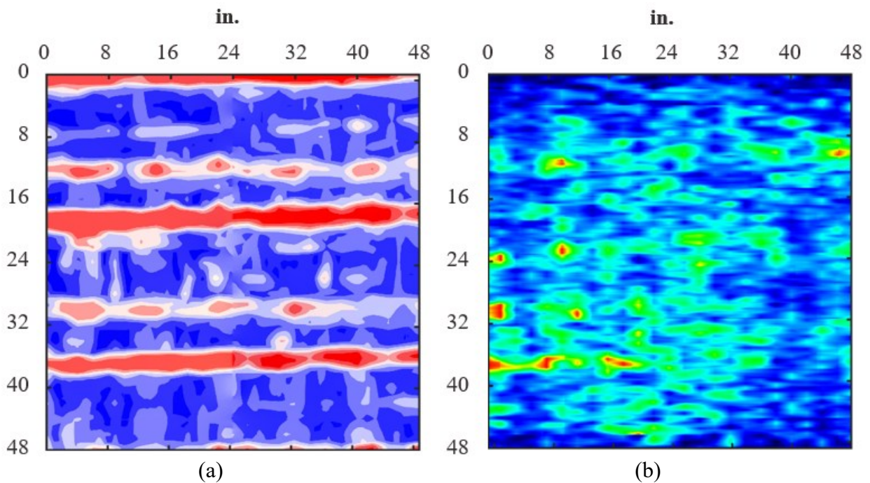
Figure 4.61. LUB4 results for the primary NDE area for (a) GPR and (b) UST of PMDF at depth 8.5 in.
