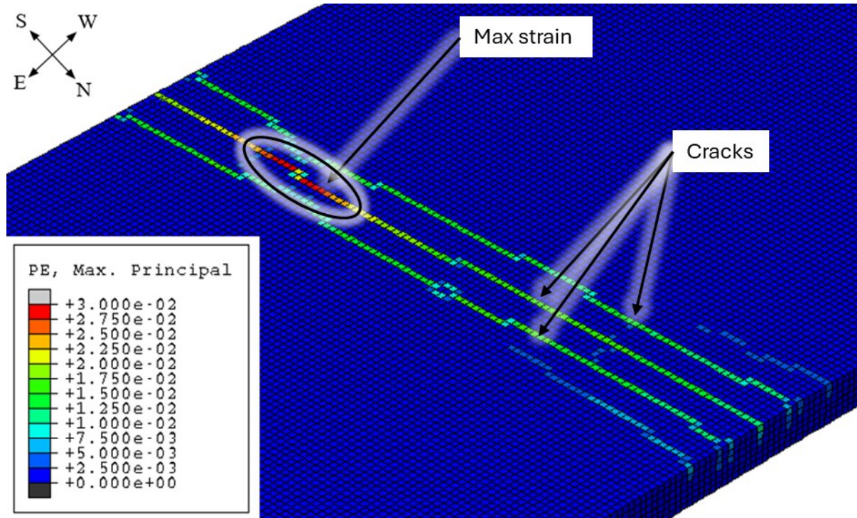
Figure 8.51. Cracking pattern for a model simulating PBJ-OP2, with added longitudinal reinforcement in the north half of the deck.
