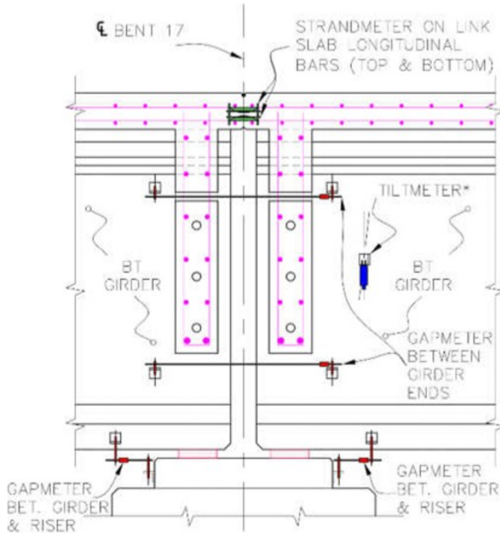
Figure 2.9. Field monitoring instrumentation setup, reprinted from Canales Jr. (2019).
