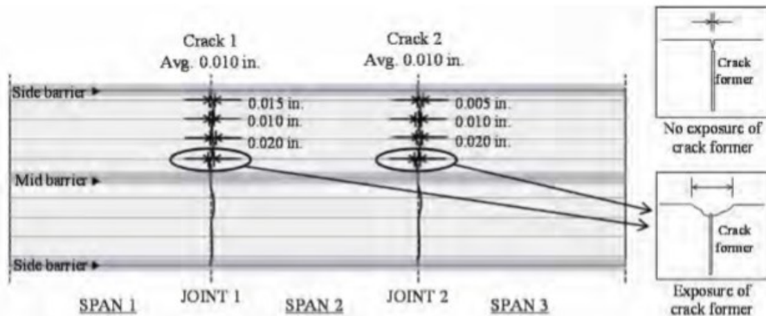
Figure 2.26. Crack widths found in the second inspection of the Wharton-Weems Overpass, reprinted from Bayrak et al. (2013).
