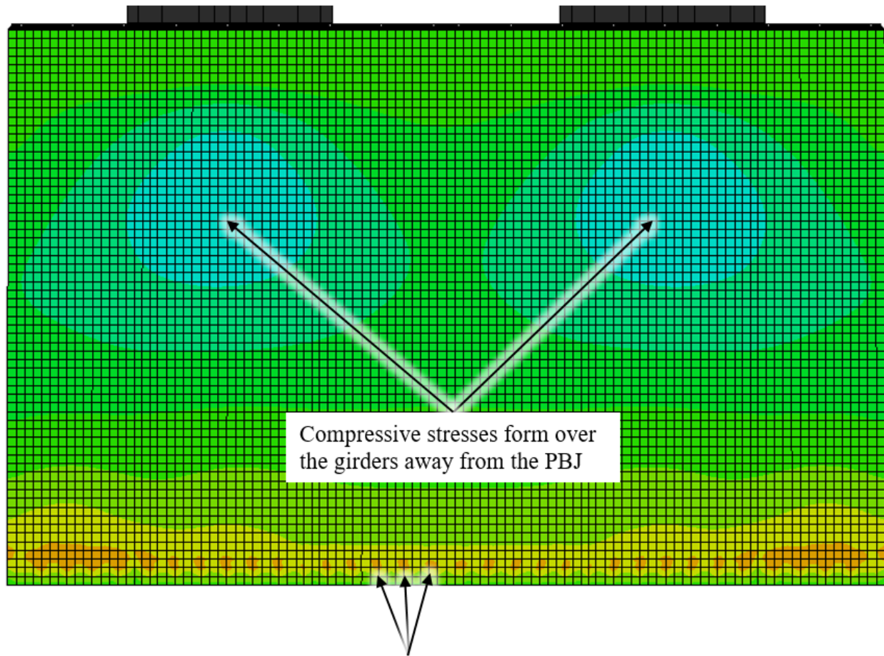
Figure 8.29. Longitudinal stresses form near the PBJ at the locations of longitudinal reinforcing bars, while compressive forces form away from the PBJ over the girder lines.
