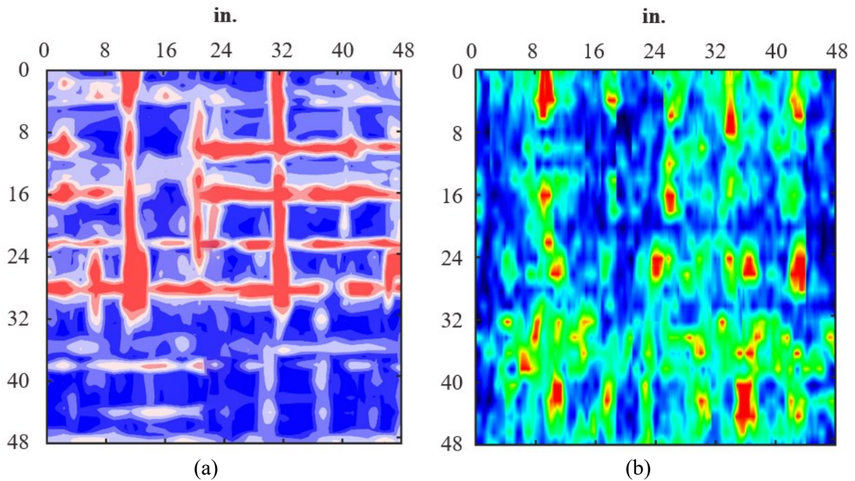
Figure 4.30. ATL4 results for (a) GPR and (b) UST of bottom reinforcement between the girders at depth 8.48 in.
