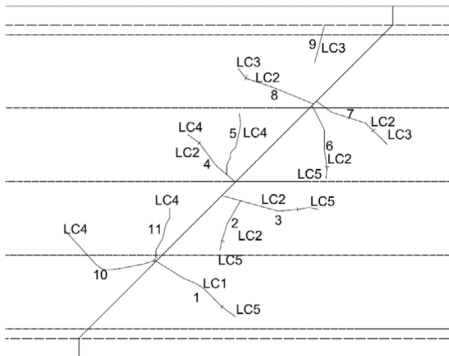
Figure 2.37. Crack propagation from crack former, reprinted from Munsterman (2017).
