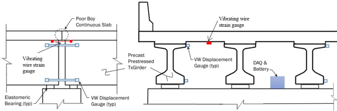
Figure 5.2. General layout of instrumentation at girder ends.
