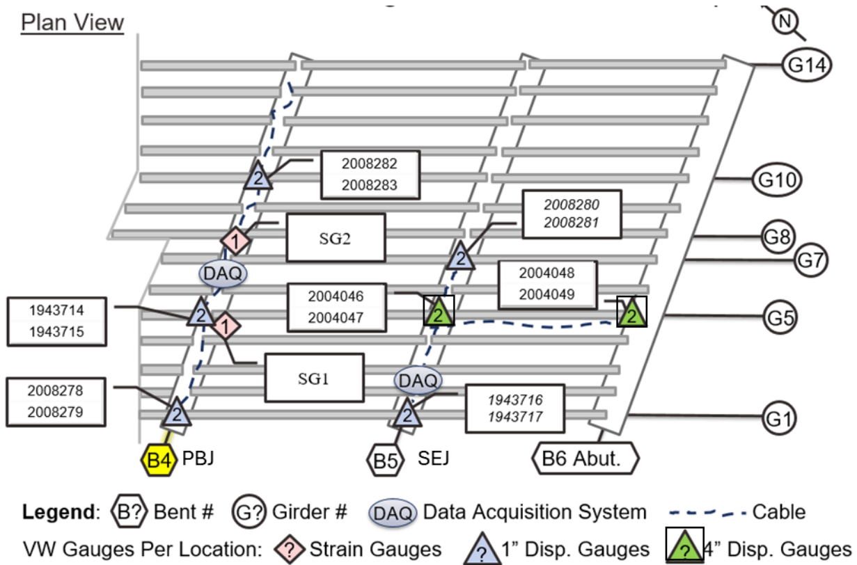
Figure 5.7. Instrumentation plan for Bridge BRY1 (SH 6 over Peach Creek).
