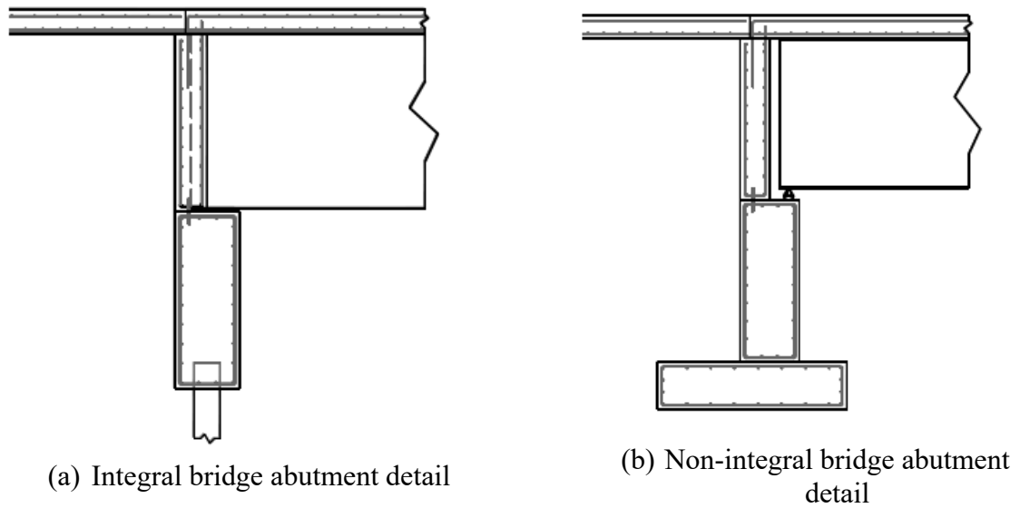
Figure 2.75. Abutment details: (a) integral and (b) non-integral; reprinted from Stringer and Burgueño (2012).
