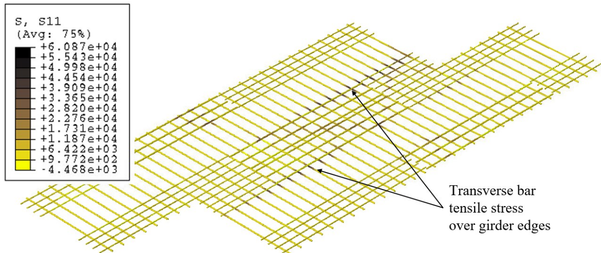
Figure 8.79. Stress in the bottom longitudinal and transverse bars for the skewed model, showing maximum tensile stresses forming in the transverse reinforcement over the girder edges.
