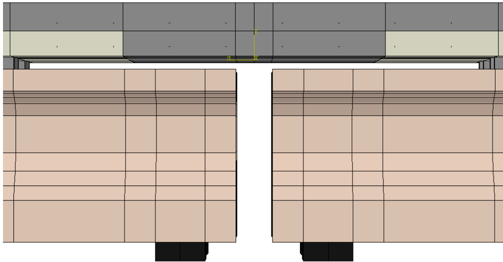
Figure 8.44. Debonded offset panel model with the girder haunch removed, creating a 2-in. vertical gap between the girder and the bottom of the slab.
