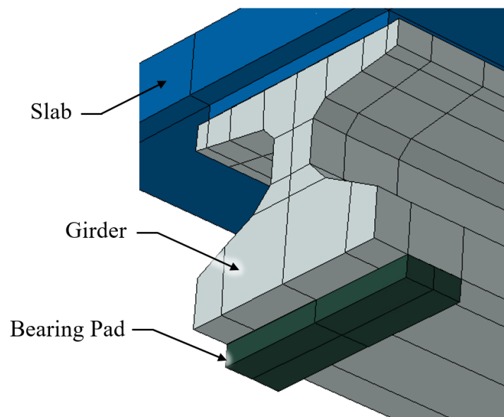
Figure 8.17. Bearing pad location at girder end.
