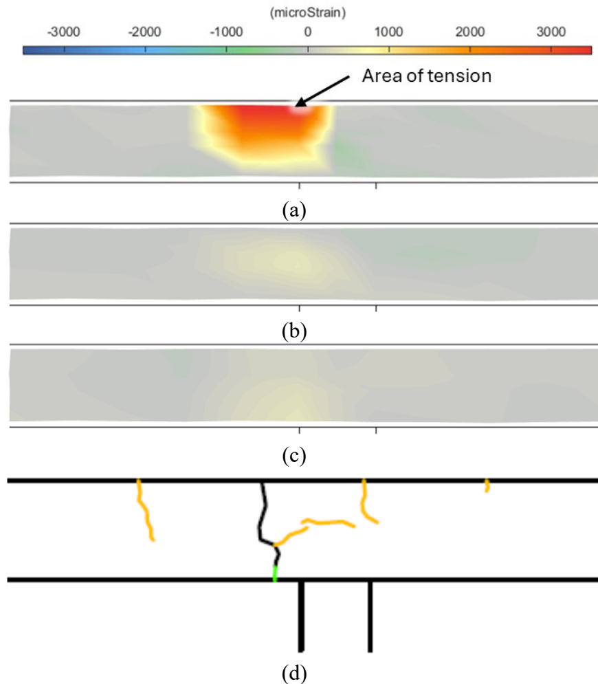
Figure 10.31. Optotrak strains for PBJ-OP2 Pattern All-Yield: (a) horizontal, (b) vertical, (c) shear strain, and (d) crack pattern (cracks formed during the load pattern are shown as yellow lines).
