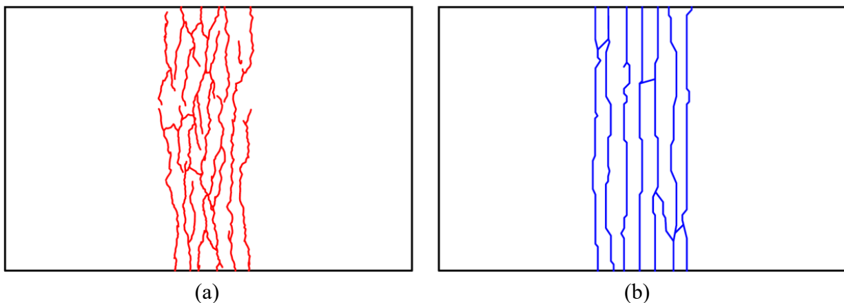
Figure 8.96. Crack patterns of model CP1 for (a) the experimental test and (b) the FEM.
