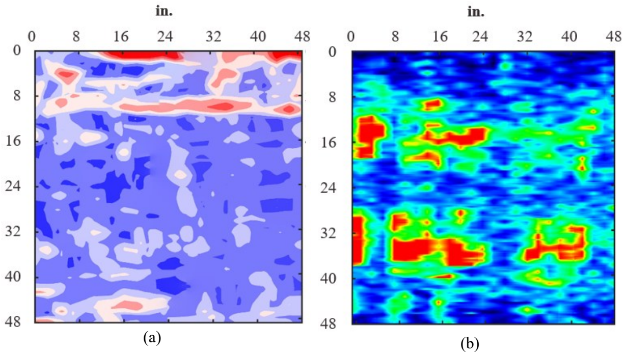
Figure 4.46. LUB2 results for (a) GPR and (b) UST of PMDF at depth 8.5 in.
