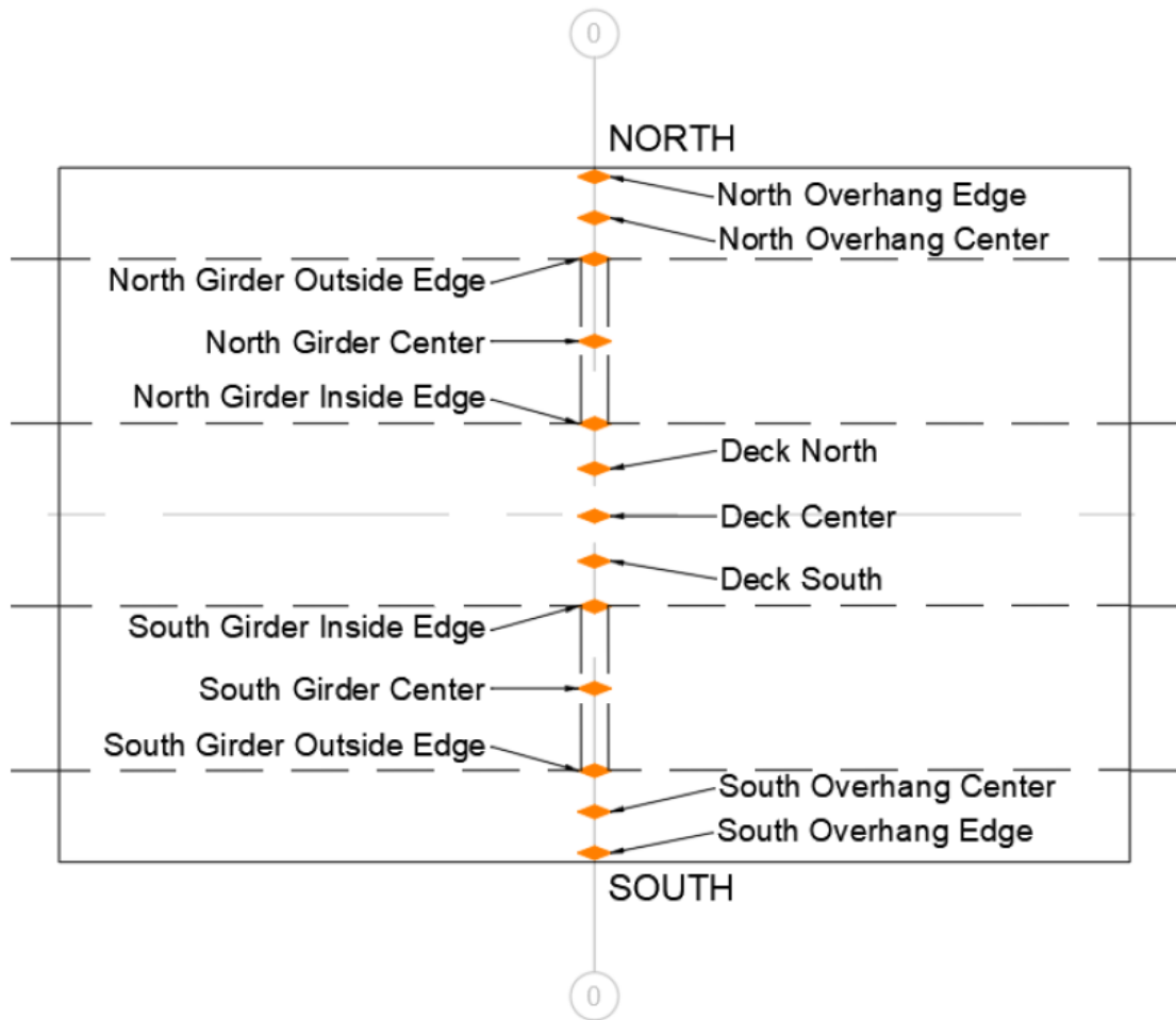
Figure 9.43. Locations of crack width measurements on top of deck.
