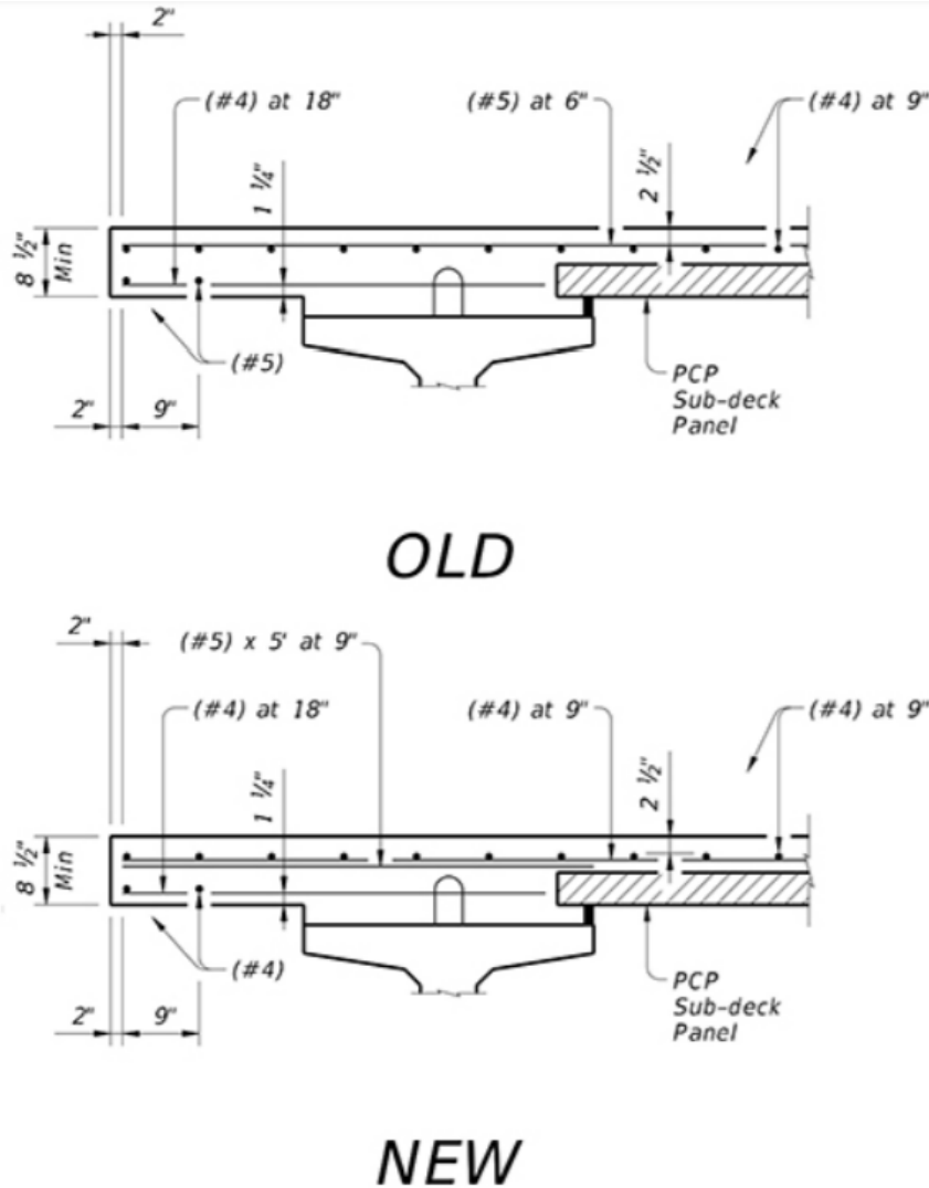
Figure 2.30. Old and new deck reinforcement detail with precast panels, reprinted from Holt and Smith (2014).
