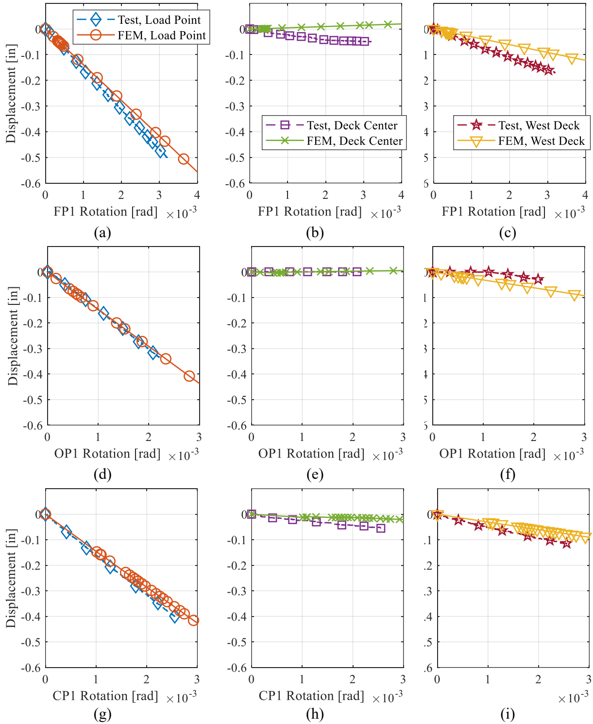
Figure 8.91. Comparison of vertical displacement beneath the loading point of the girder, the deck center beneath the PBJ, and the deck center 3 ft west of the PBJ for tests FP1, OP1, and CP1.
