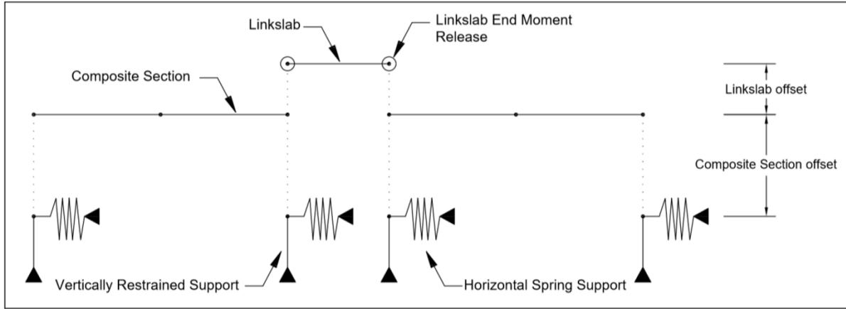
Figure 2.7. Finite element model, reprinted from Canales and Okeil (2019).
