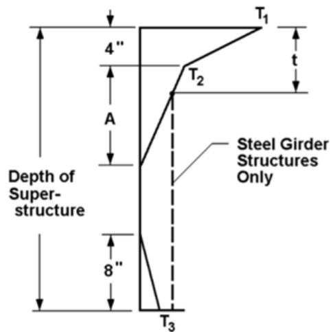
Figure 7.1. Temperature gradient from AASHTO LRFD specification.
