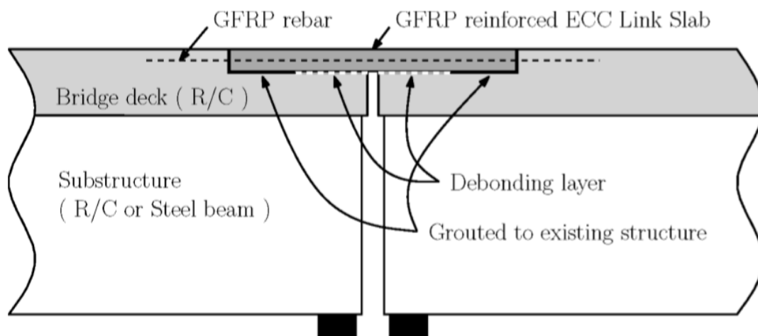
Figure 2.71. Prefabricated ECC link slab concept with GFRP reinforcement, reprinted from Lárusson et al. (2013).
