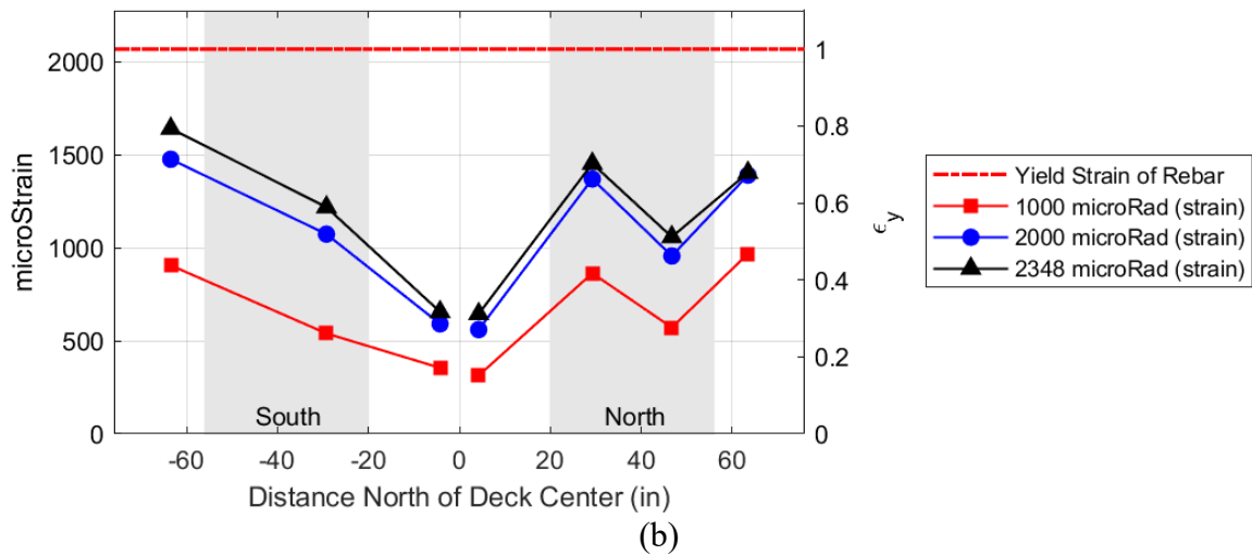
Figure 10.10. PBJ-OP2: Pattern All comparison of (a) crack width profiles and (b) strain width profiles.
