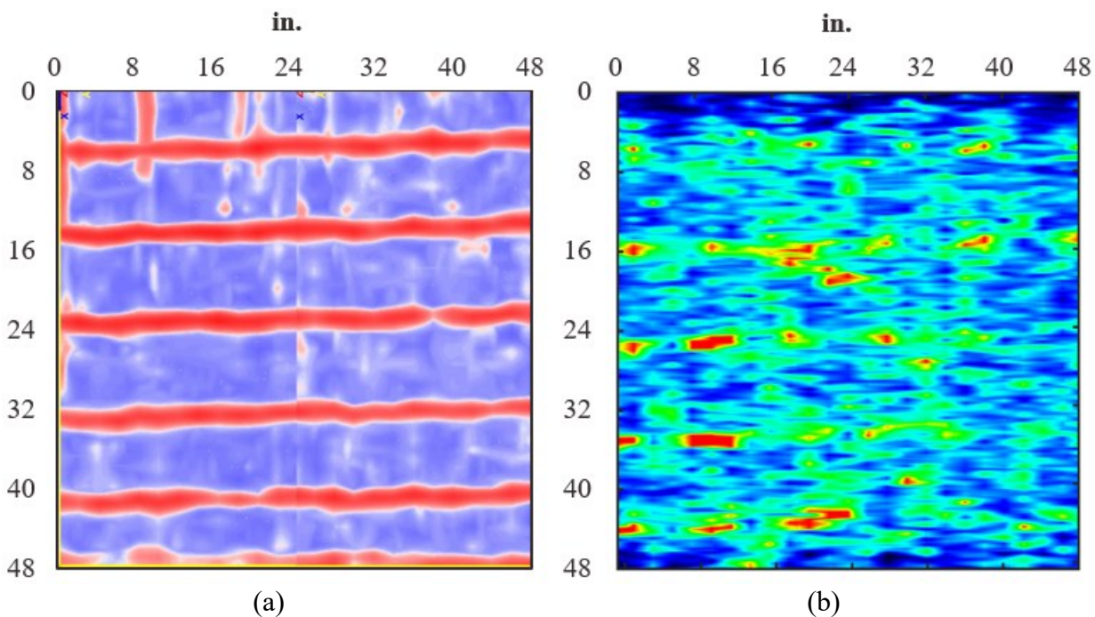
Figure 4.59. LUB4 results for the primary NDE area for (a) GPR and (b) UST of top transverse reinforcement at depth 3.5 in.
