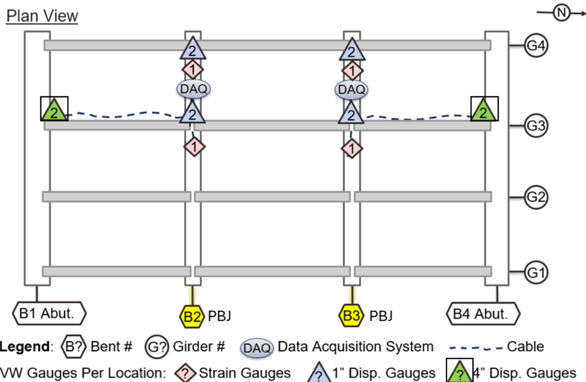
Figure 5.13. Instrumentation plan for Bridge BRY4 (FM 3090 at Spring/Holland Relief).
