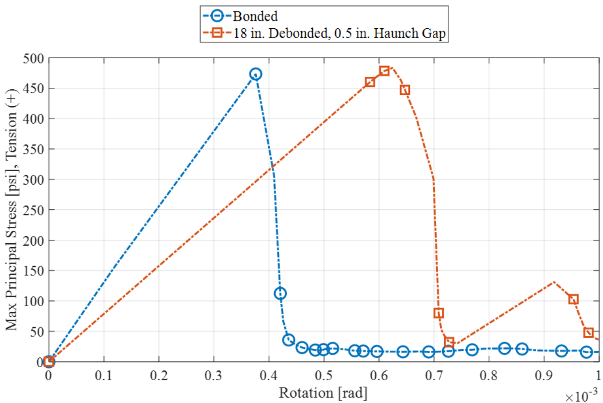
Figure 8.85. Bonded and debonded comparison of dual-girder skewed models, showing maximum principal stress at the location of first cracking in each deck.
