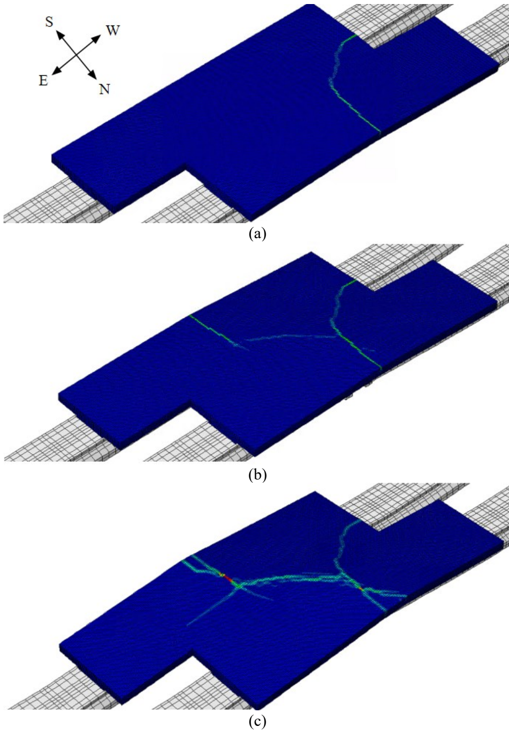
Figure 8.76. Crack propagation in the dual-girder skewed model with offset panels for loading progressing from the (a) northwest girder, (b) southwest girder, and (c) southeast and northeast girders.
