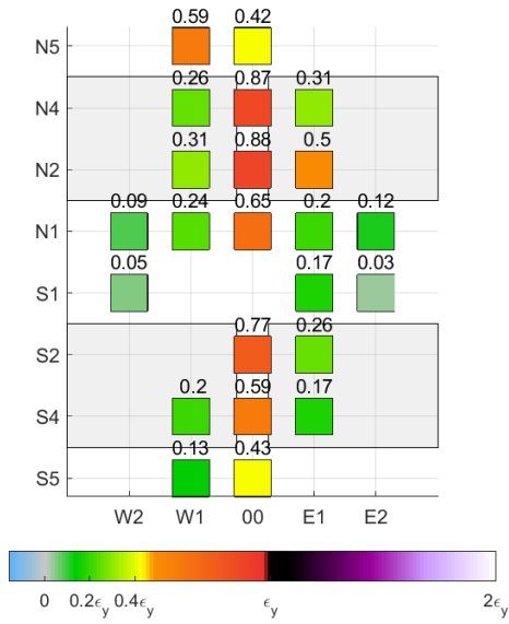
(a) PBJ-FP1 (3294 microradians)
