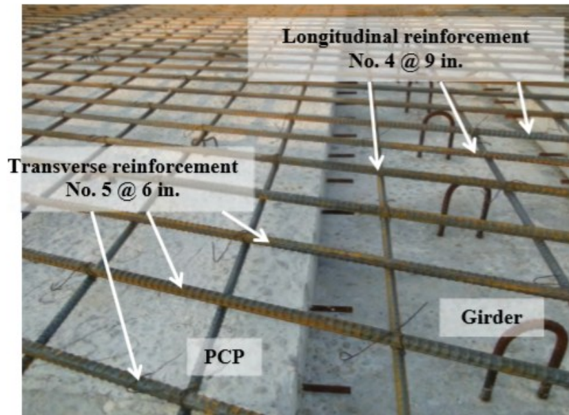
Figure 2.28. Deck reinforcement placement on Lampasas River Bridge, reprinted from Bayrak et al. (2013).
