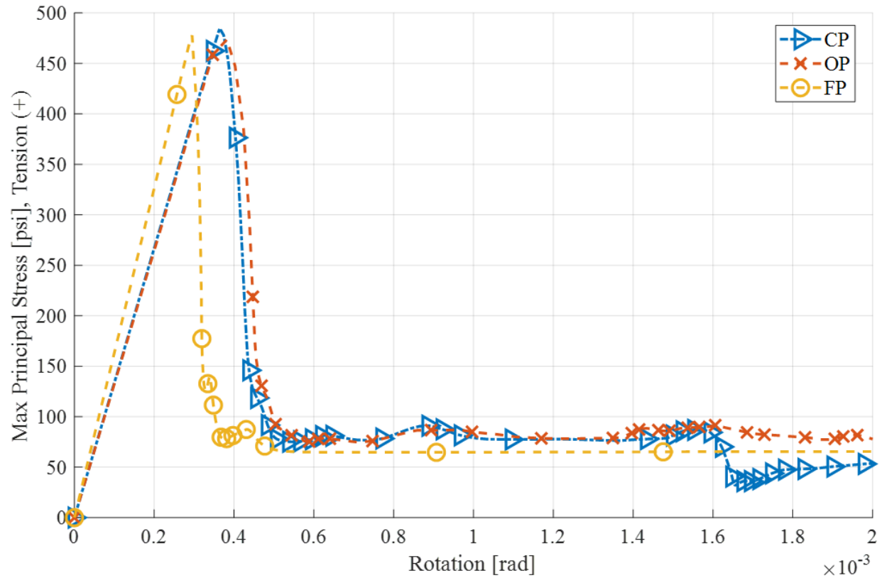
Figure 8.55. Maximum principal stress in the concrete at the point of first cracking for the continuous panel model, compared to the bonded offset panel and flush panel models.
