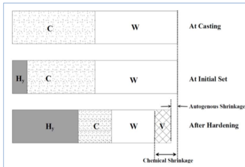
Figure 2.10. Chemical changes and shrinkage during the concrete curing process, reprinted from Holt (2001).
