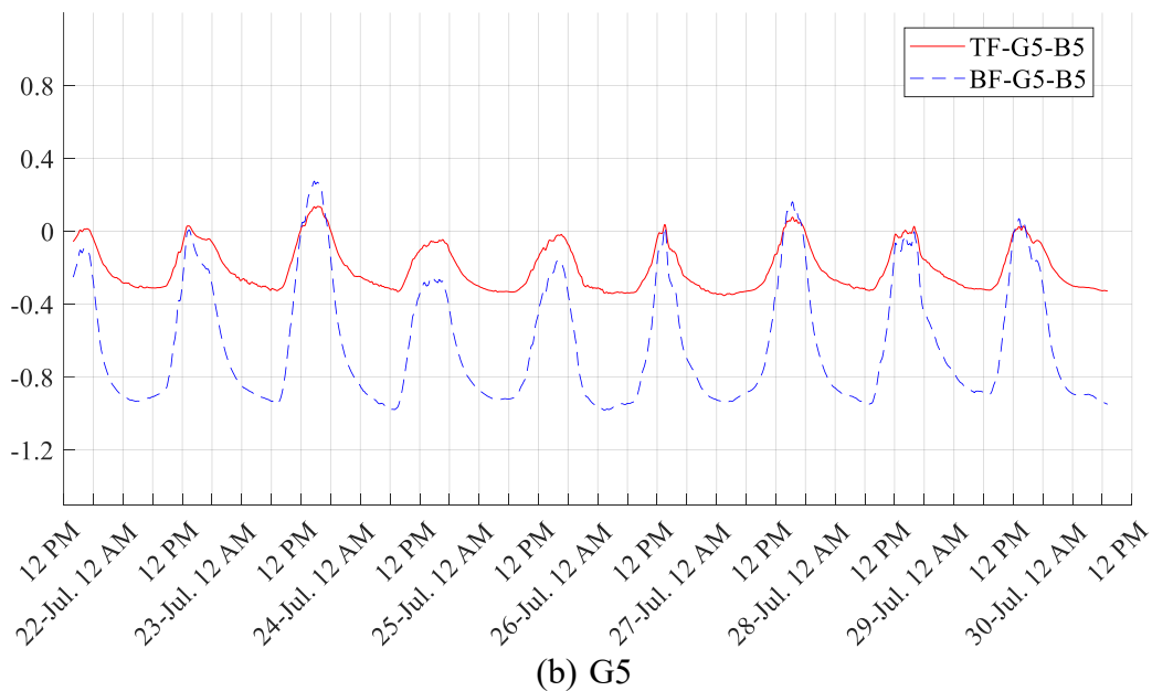
Figure 5.17. Thermal deformations of gages in BRY3 at PBJs at B5.
