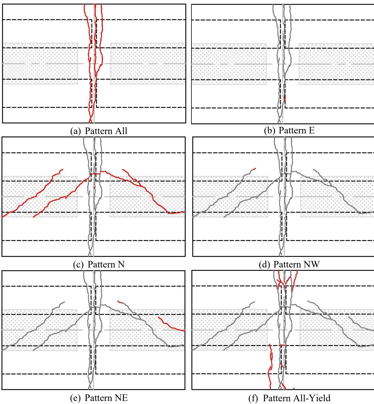
Figure 9.56. PBJ-OP2: Cracks for all load patterns.
