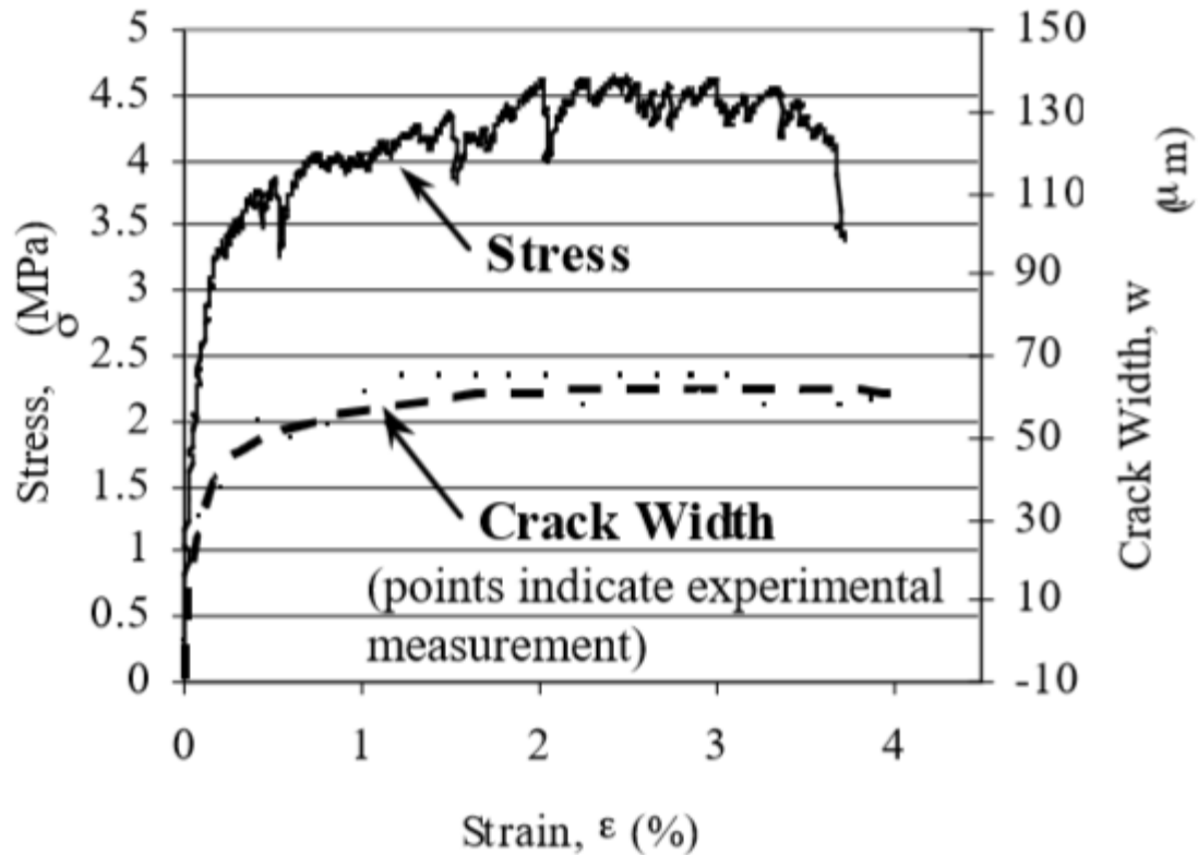
Figure 2.64. ECC stress-strain plot and corresponding crack width, reprinted from Lepech and Li (2005).
