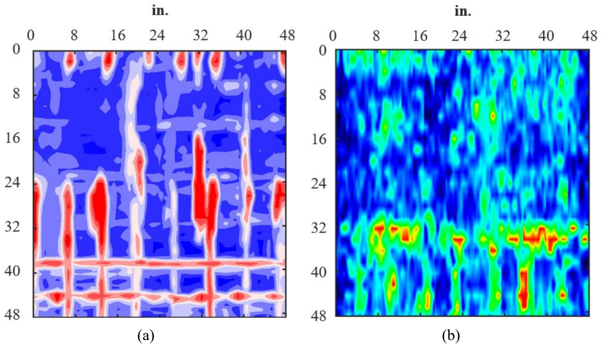
Figure 4.31. ATL4 results for (a) GPR and (b) UST of bottom reinforcement between the girders at depth 7.48 in.
