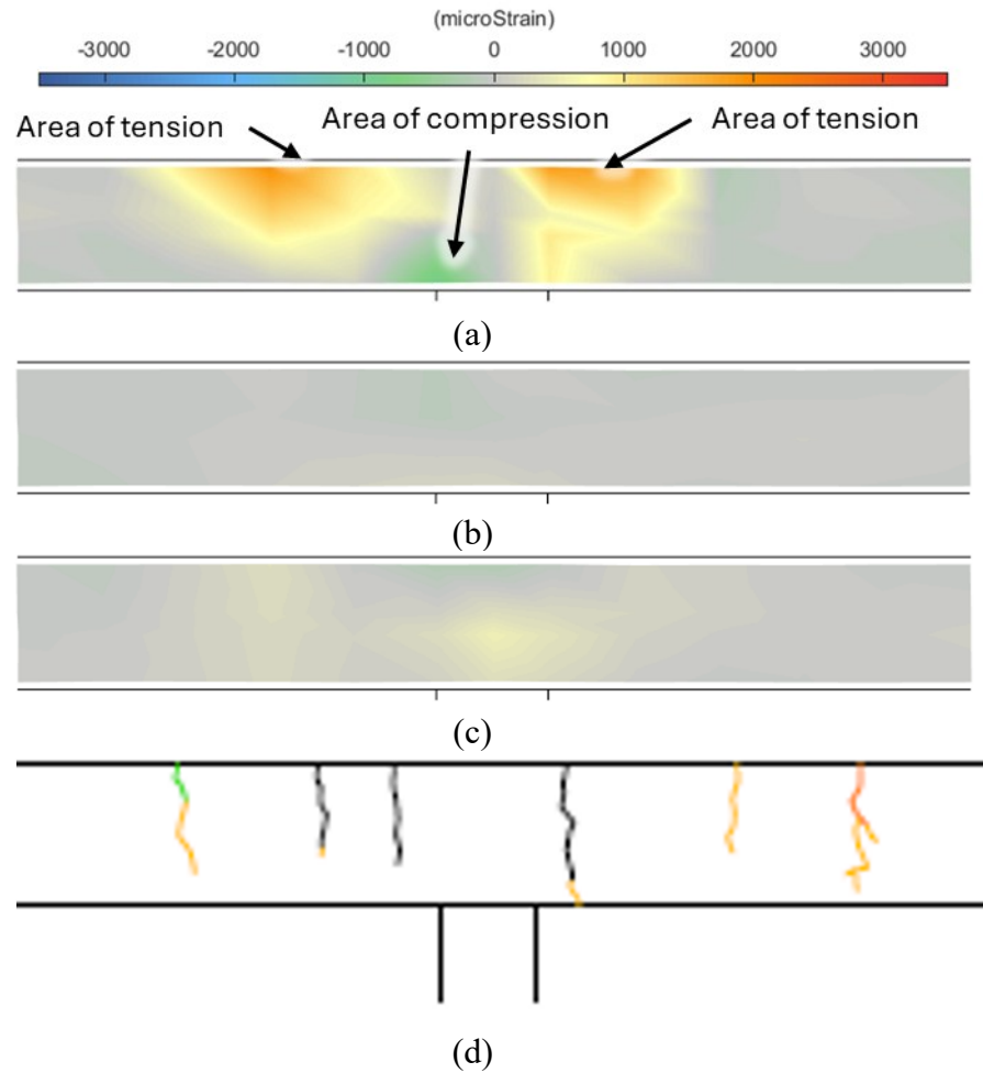
Figure 10.27. Optotrak strains for PBJ-CP1 Pattern All: (a) horizontal, (b) vertical, (c) shear strain, and (d) crack pattern.
