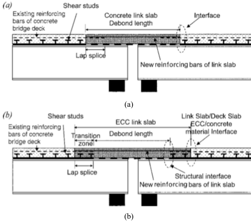
Figure 2.68. Link slab design for (a) normal concrete and (b) ECC with a reinforced transition zone to protect the discontinuity between materials; reprinted from Qian et al. (2009).
