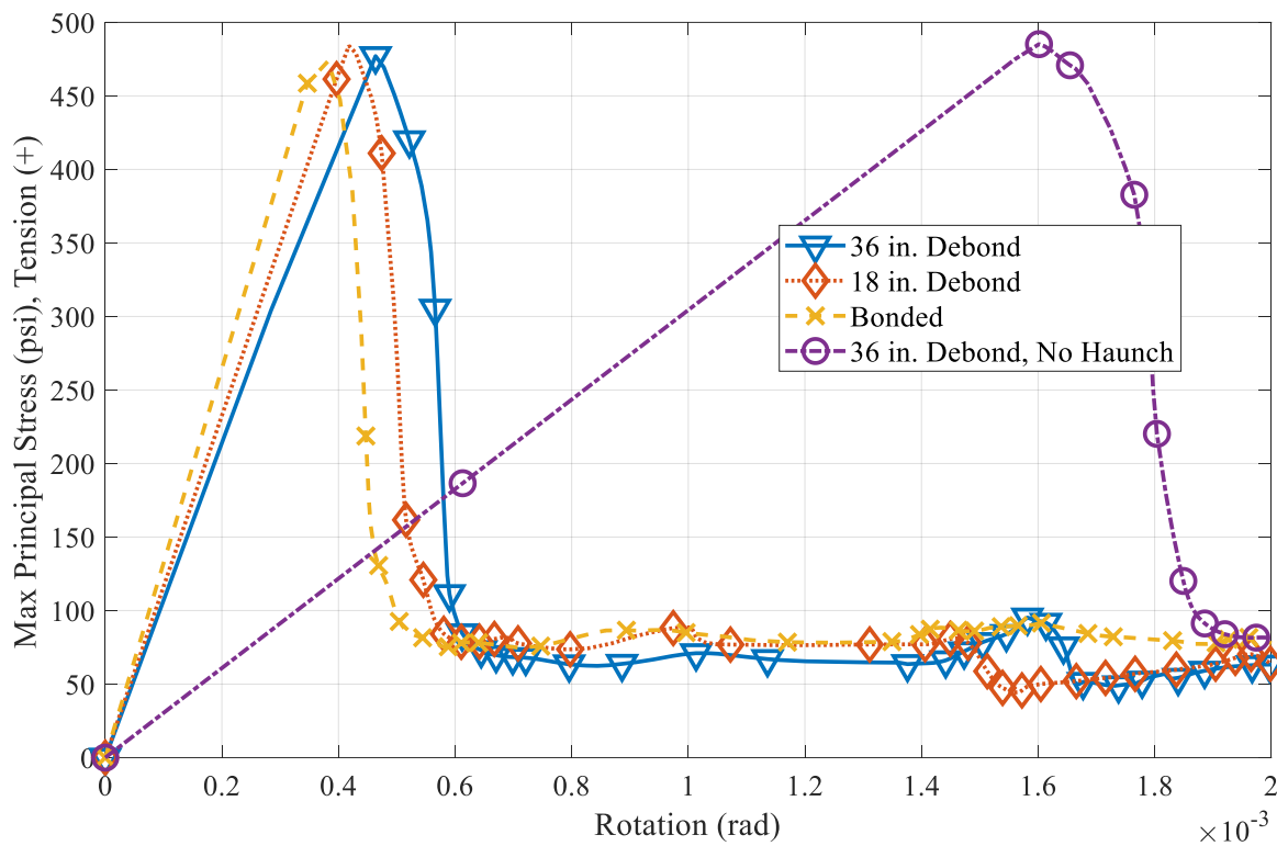
Figure 8.45. Maximum principal stress for various offset precast panel models at the location of first cracking.
