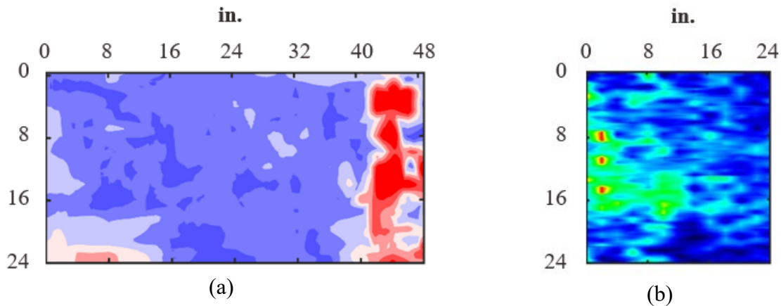
Figure 4.65. LUB4 results for the secondary NDE area for (a) GPR and (b) UST of the PMDF in the overhang at depth 8.5 in.
