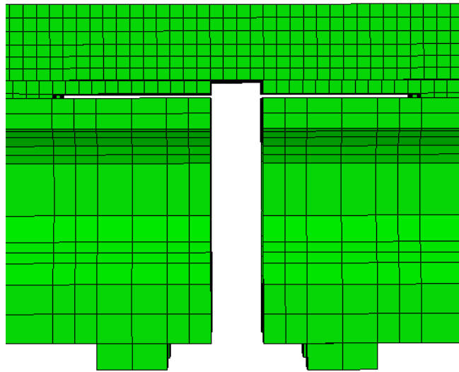
Figure 8.56. Side view of the DLS for the continuous panel models, showing the 0.5-in. gap between the slab and top faces of the girders.
