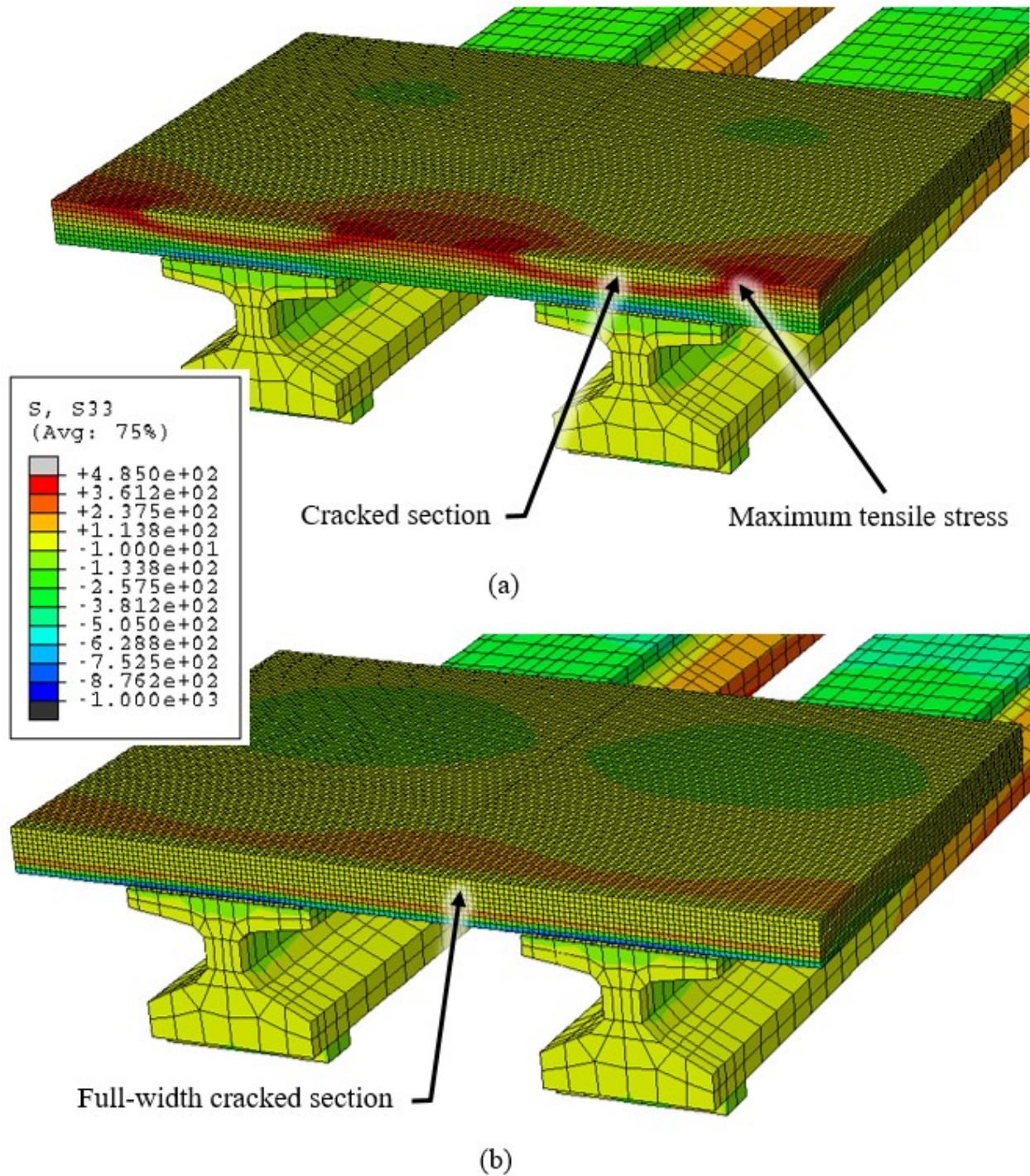
Figure 8.22. Longitudinal stresses in CIP deck concrete (psi), showing (a) initial crack propagation over the girders, which (b) continues until the entire deck width is cracked.
