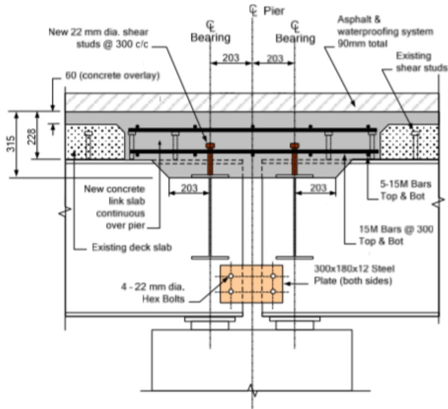
Figure 2.41. Trent Canal Bridge link slab detail, reprinted from Lam et al. (2008).
