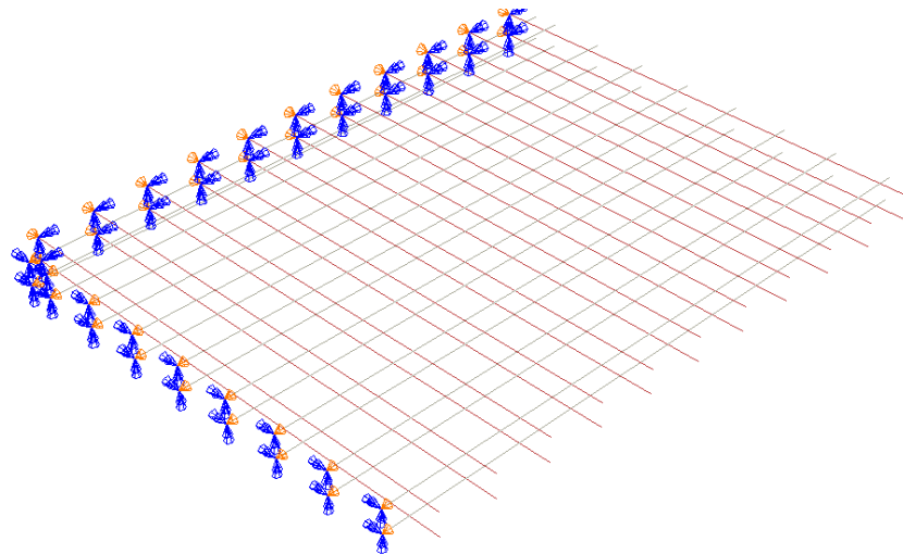
Figure 8.15. Rebar cage showing the mirrored end constraints on the reinforcement in two directions.
