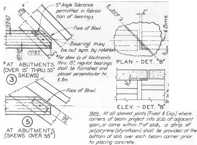
Figure 6.4. Prestressed concrete beam span details, AASHTO Type IV standard detail of 1968.
