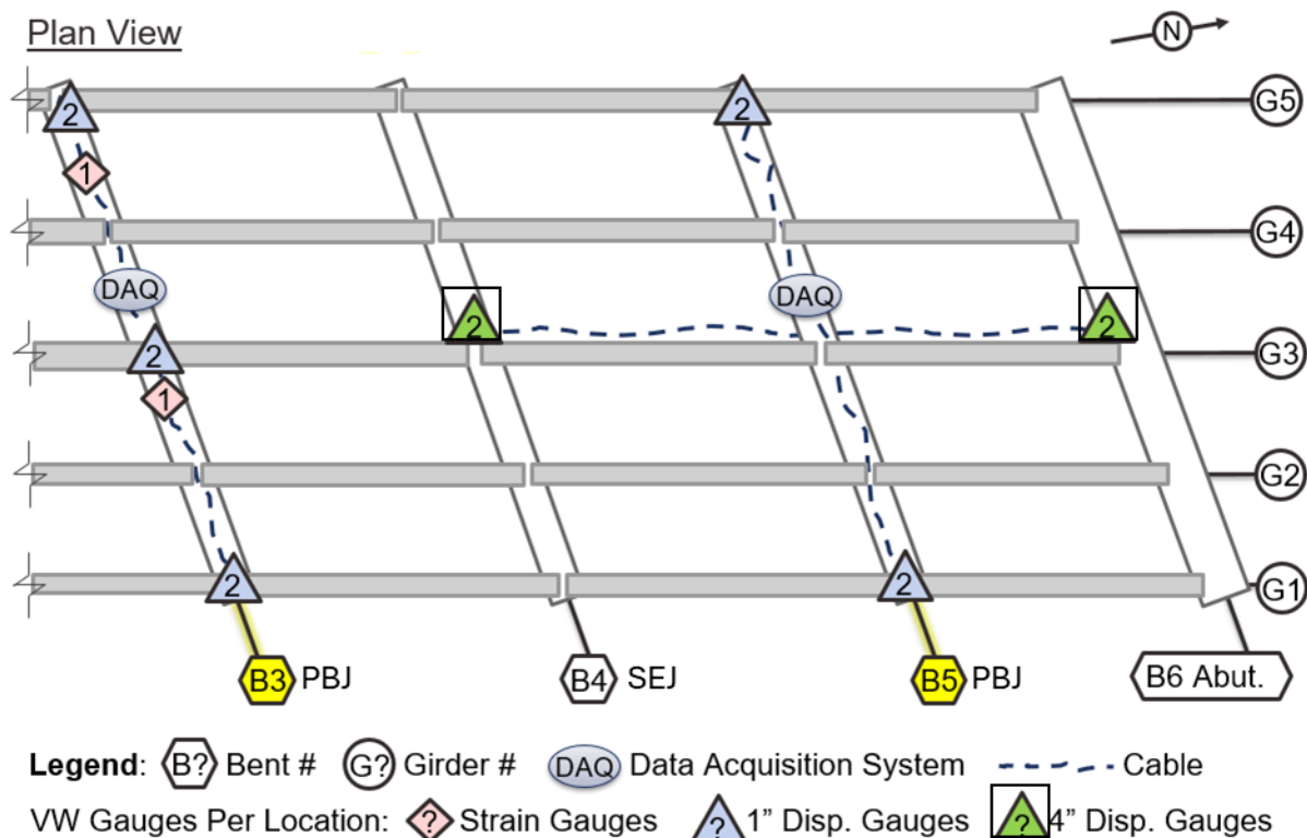
Figure 5.9. Instrumentation plan for Bridge BRY2 (FM 60 over Old River).
