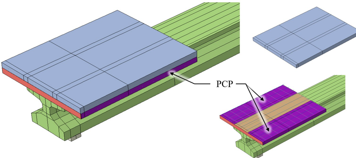
Figure 8.7. Partial-depth debonded model used with flush panel configuration.
