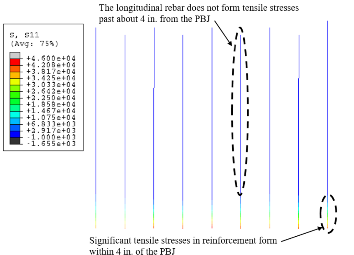
Figure 8.30. Close-up of embedded longitudinal steel reinforcement showing that tensile stresses are focused near the PBJ.
