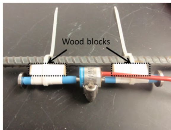
Figure 2.22. Vibrating wire strain gage installation on rebar, reprinted from Bayrak et al. (2013).
