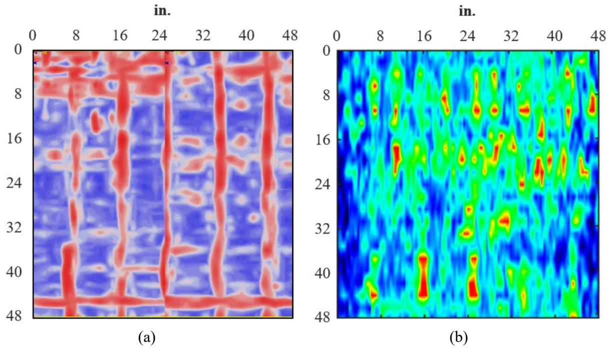
Figure 4.22. ATL3 results for (a) GPR and (b) UST of bottom longitudinal reinforcement at depth 5.98 in.
