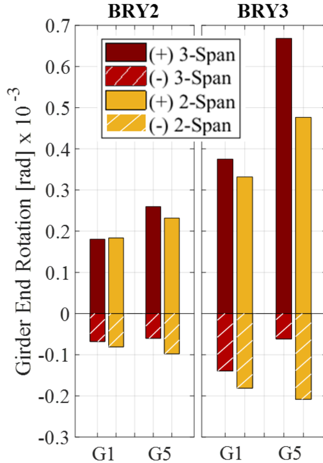
Figure 5.27. Thermal rotations for BRY2 and BRY3, with bars indicating number of continuous spans in a unit.
