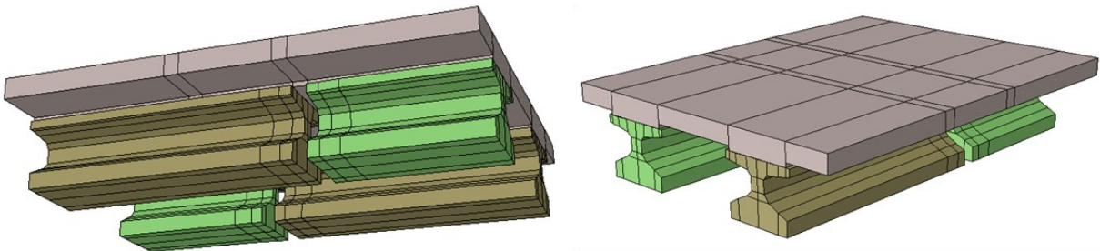
Figure 8.3. Dual-girder model for skewed girder configuration without clipped girders.
