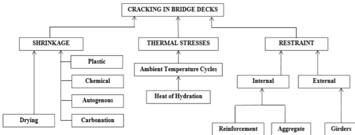
Figure 2.11. Bridge deck cracking sources, reprinted from Pesek et al. (2013).
