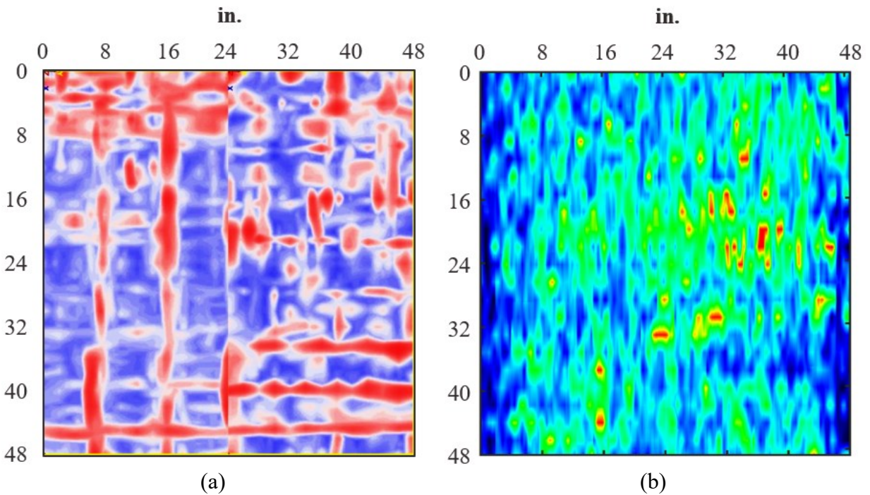
Figure 4.23. ATL3 results for (a) GPR and (b) UST of bottom transverse reinforcement at depth 5.48 in.
