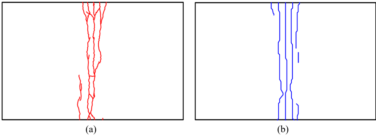
Figure 8.95. Crack patterns of model OP2 for (a) the experimental test and (b) the FEM.
