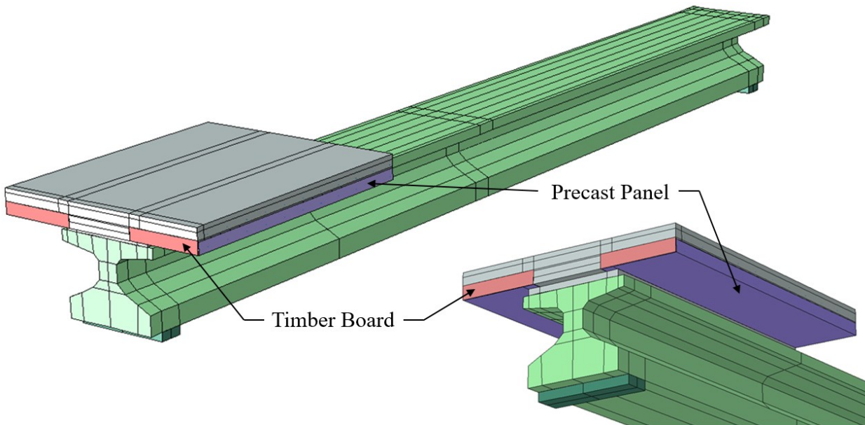
Figure 8.4. Flush panel model with timber board.
