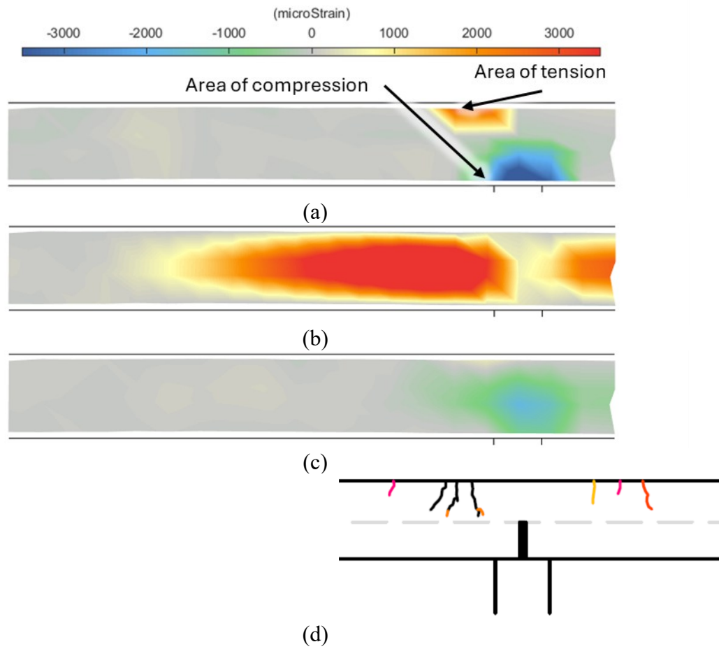
Figure 10.23. Optotrak strains for PBJ-FP1R Pattern All: (a) horizontal, (b) vertical, (c) shear strain, and (d) crack pattern.
