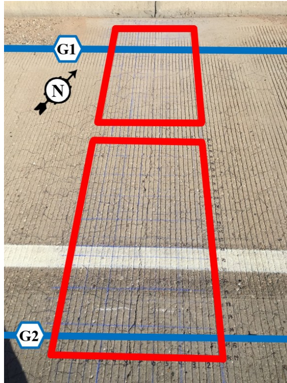
Figure 4.35. Primary NDE regions (Region 1 and 2) at Bent 3 for Bridge LUB1 (SB Loop 289 over Slide Rd./4th St.).
