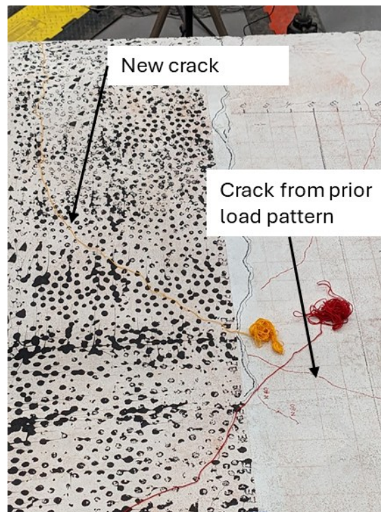
Figure 9.51. PBJ-OP1: North overhang cracks formed during Pattern NW-1 (red sharpie) and Pattern NE-1 (gold string) (right edge of speckled region is center of link slab).
