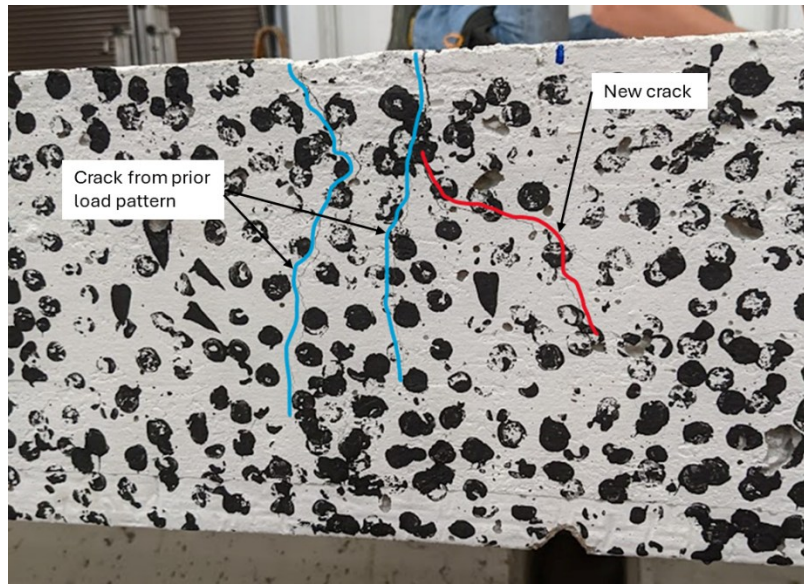
Figure 9.52. PBJ-OP1: East offset crack on north edge of deck at 430 kips in Pattern All-Yield (cracks at prior load steps shown in blue, new crack shown in red).
