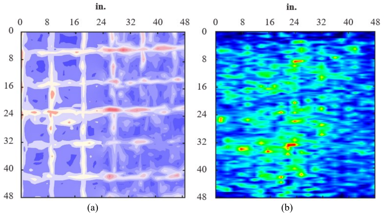
Figure 4.60. LUB4 results for the primary NDE area for (a) GPR and (b) UST of bottom reinforcement at depth 6.5 in.
