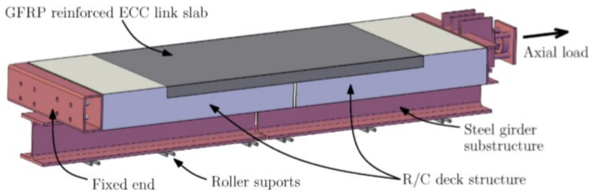
Figure 2.72. ECC link slab specimen characteristics, reprinted from Lárusson et al. (2013).
