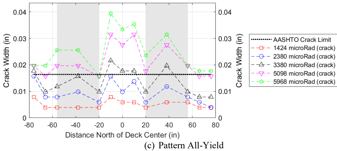
Figure 10.2. PBJ-FP1: Crack width profiles for select patterns.
