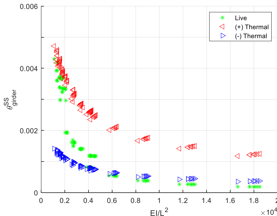
Figure 7.2. Girder end rotations for live and thermal loading.
