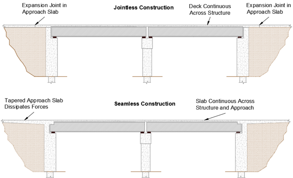
Figure 2.2. Bridge system nomenclature diagram.
