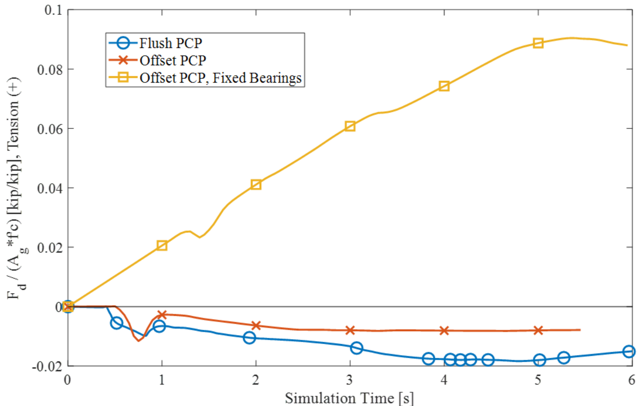
Figure 8.66. Longitudinal force in the deck, F_d , across the PBJ normalized by the gross section area at the PBJ and concrete compressive strength ( A_g * f'_c ) for models with flush PCP, offset PCP, and offset PCP with fixed bearings.
