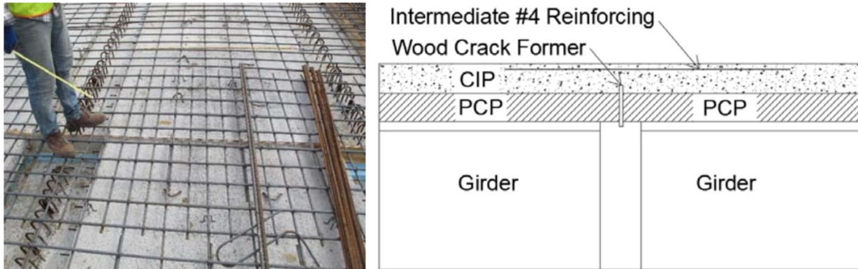
Figure 2.35. Added reinforcement over supports and crack-forming detail, reprinted from Munsterman (2017).
