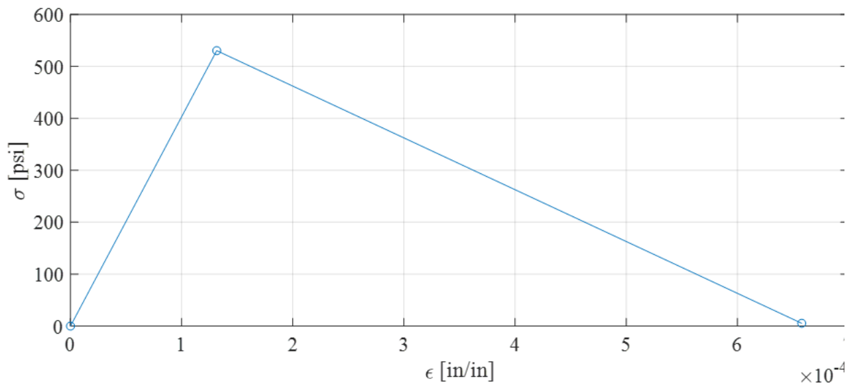
Figure 8.14. Bilinear tension model for concrete.
