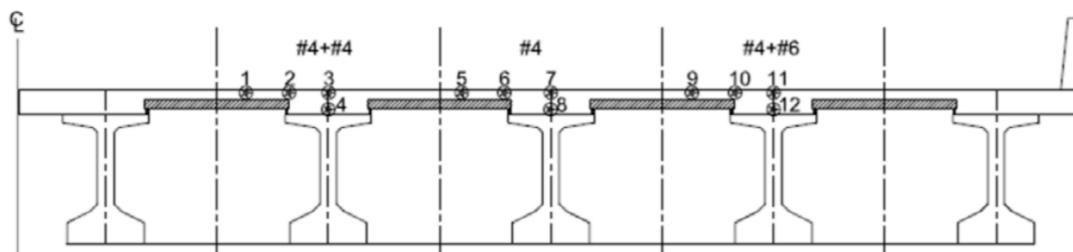
Figure 2.32. Gage placement diagram, reprinted from Munsterman (2017).
