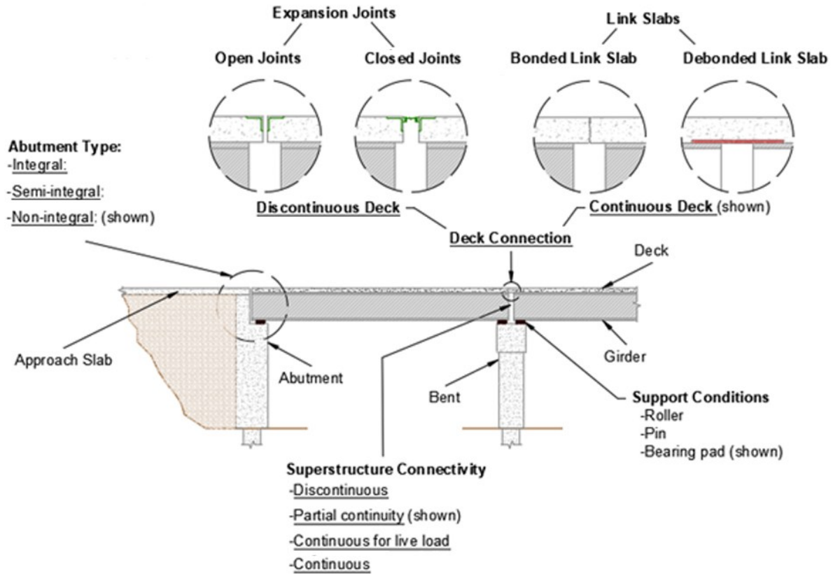
Figure 2.1. Nomenclature diagram for bridge components.
