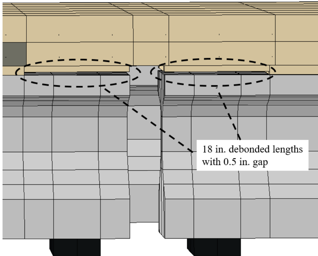
Figure 8.80. Debonded regions of the skewed model, with an 18-in. debonded length and a 0.5-in. gap between the girder face and the bottom of the deck.
