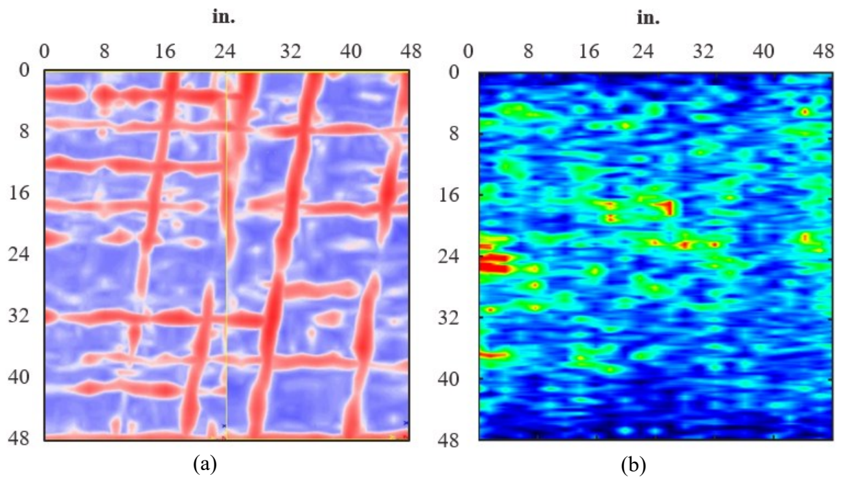
Figure 4.45. LUB2 results for (a) GPR and (b) UST of bottom reinforcement at depth 5.73 in.
