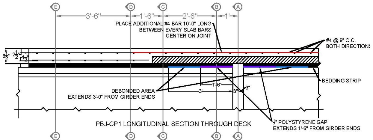
Figure 9.13. PBJ-CP1 details—elevation view.
