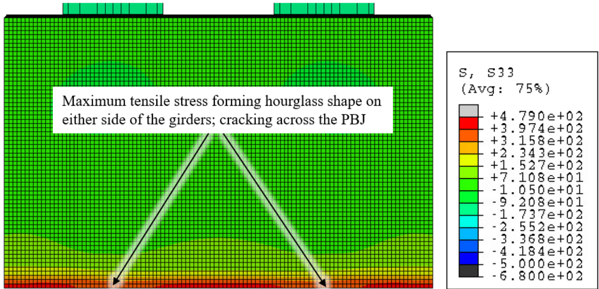
Figure 8.28. Initial cracking of the PBJ with the use of a control joint detail for a flush PCP model.
