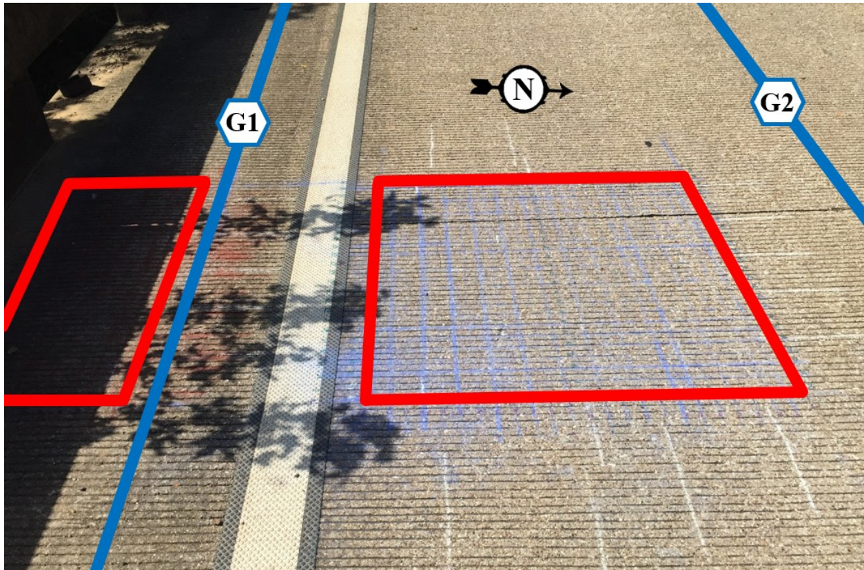
Figure 4.27. NDE region at Bent 3 for Bridge ATL4 (FM 968 over Clarks Creek).
