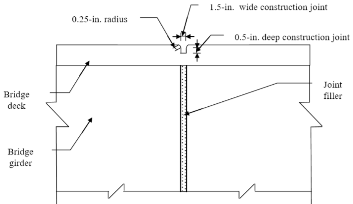
Figure 2.46. Construction joint and girder joint filler, reprinted from Snedeker et al. (2011).
