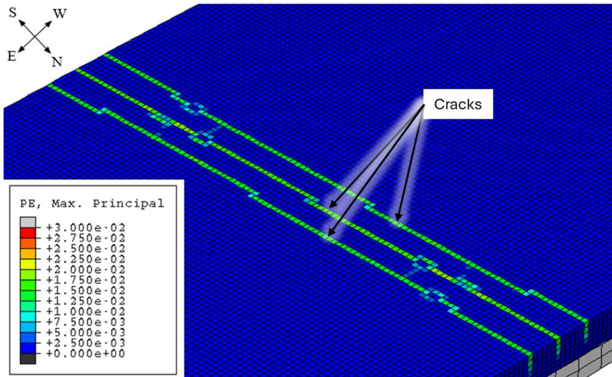
Figure 8.52. Offset precast panel model with longitudinal reinforcement added over the girders to provide 4.5-in. spacing.
