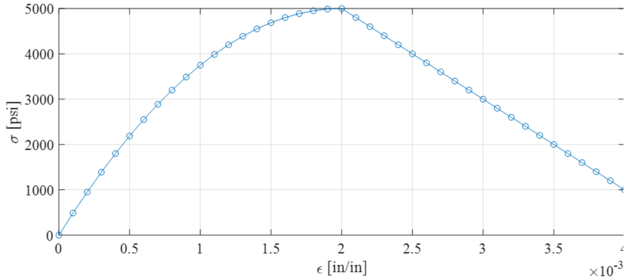
Figure 8.13. Unconfined Kent-Park concrete model for ultimate compressive strength of 5000 psi.
