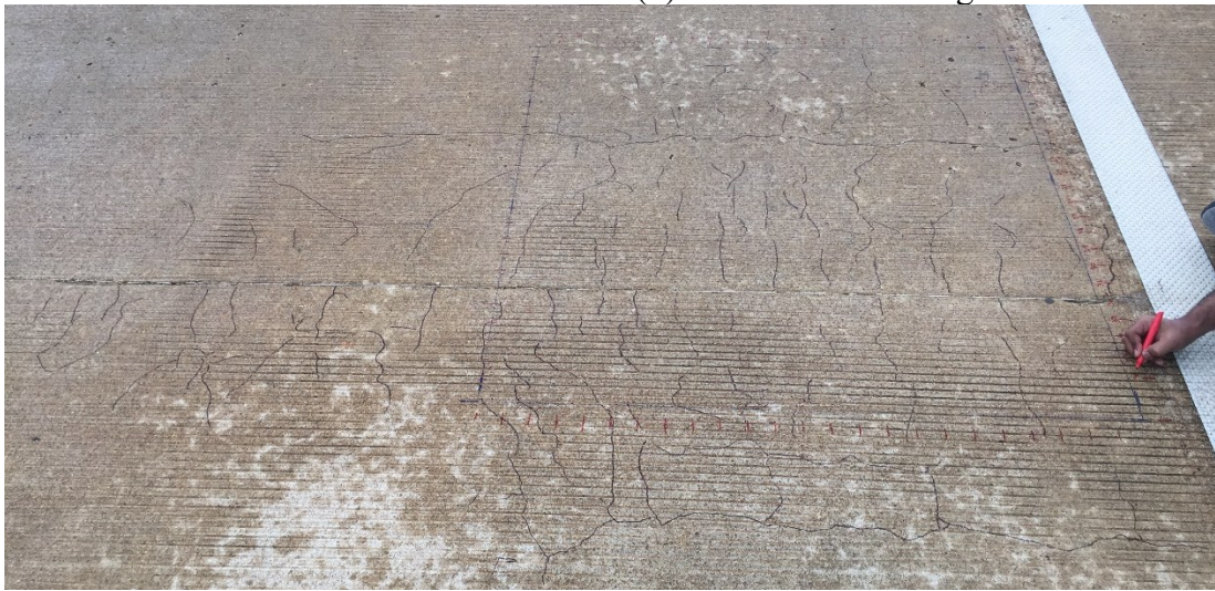
(c) Marked cracks in the NDE region at Bent 2
