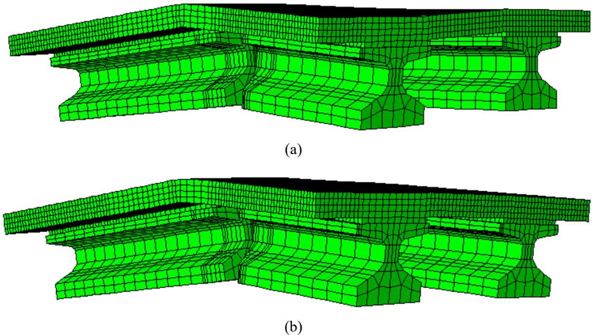
Figure 8.20. Deformation of girder stub model, at 20 times scale, showing deformation of (a) one girder line and (b) both girder lines.
