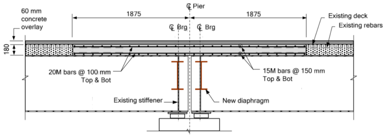
Figure 2.54. Orford Road Underpass link slab detail, reprinted from Lam et al. (2008).
