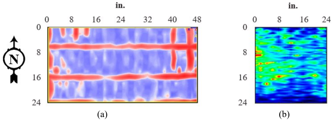
Figure 4.62. LUB4 results for the secondary NDE area for (a) GPR and (b) UST of the top longitudinal reinforcement in the overhang at depth 2.73 in.
