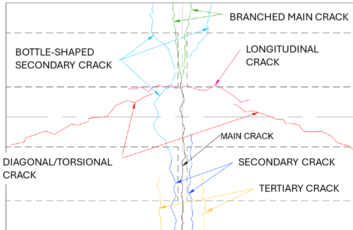
Figure 9.42. Examples of crack types used in describing damage in the link slabs.
