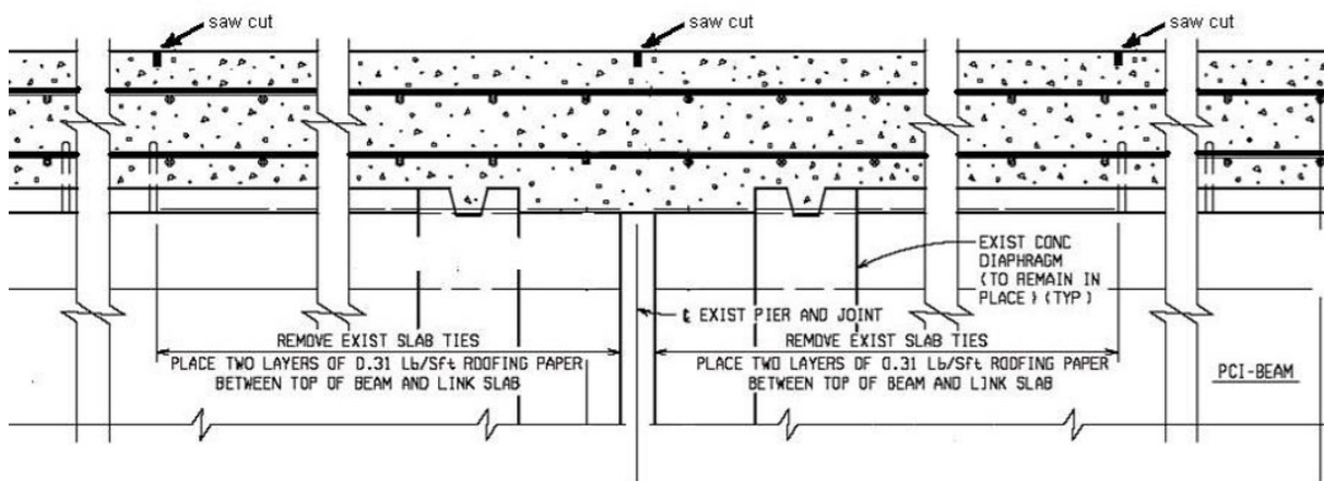
Figure 2.53. Debonded link slab design, reprinted from Aktan et al. (2008).
