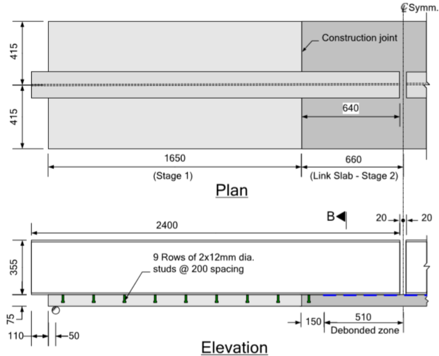
Figure 2.58. Diagram of test specimen, reprinted from Au et al. (2013).
