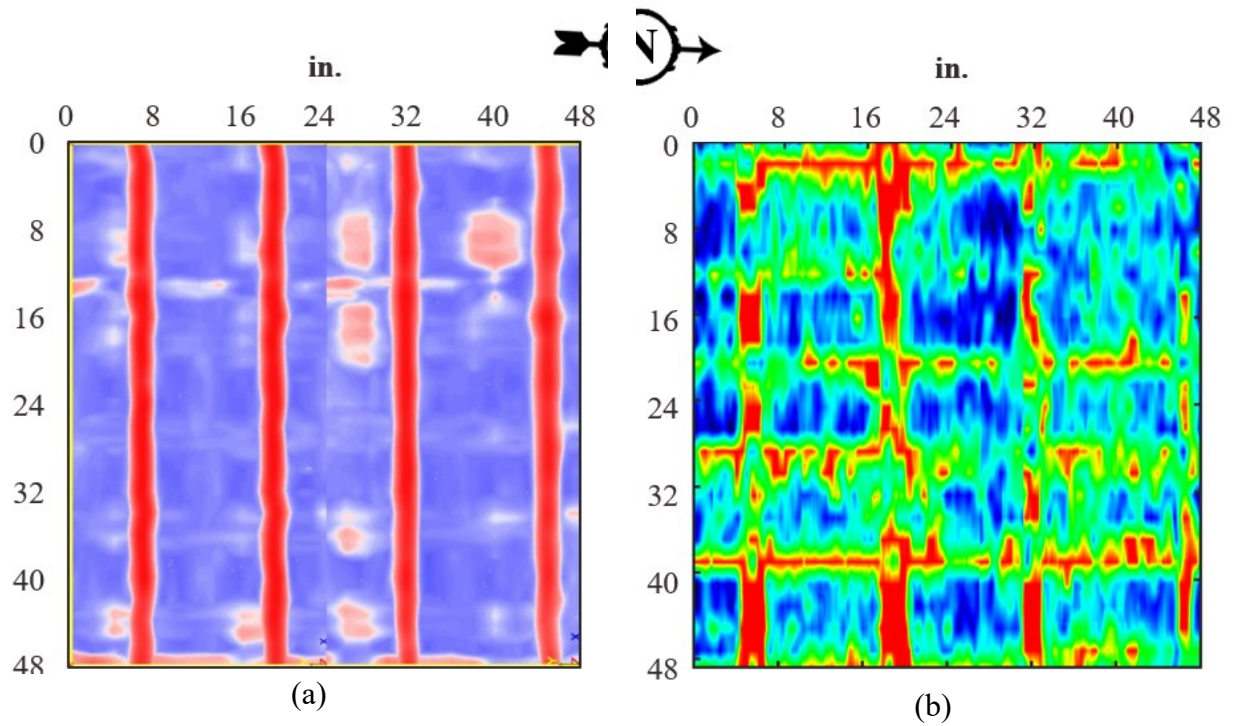
Figure 4.28. ATL4 results for (a) GPR and (b) UST of top longitudinal reinforcement between the girders at depth 4.95 in.
