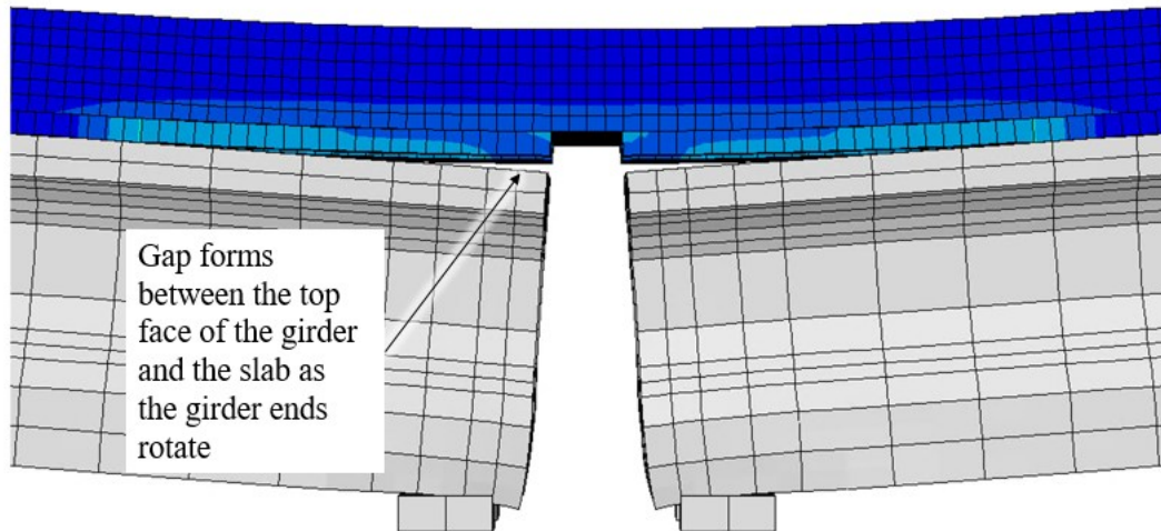
Figure 8.63. Exaggerated deformation of the girder ends for the 36-in. debonded model, causing a natural gap between the bottom of the DLS and the top face of the girder.
