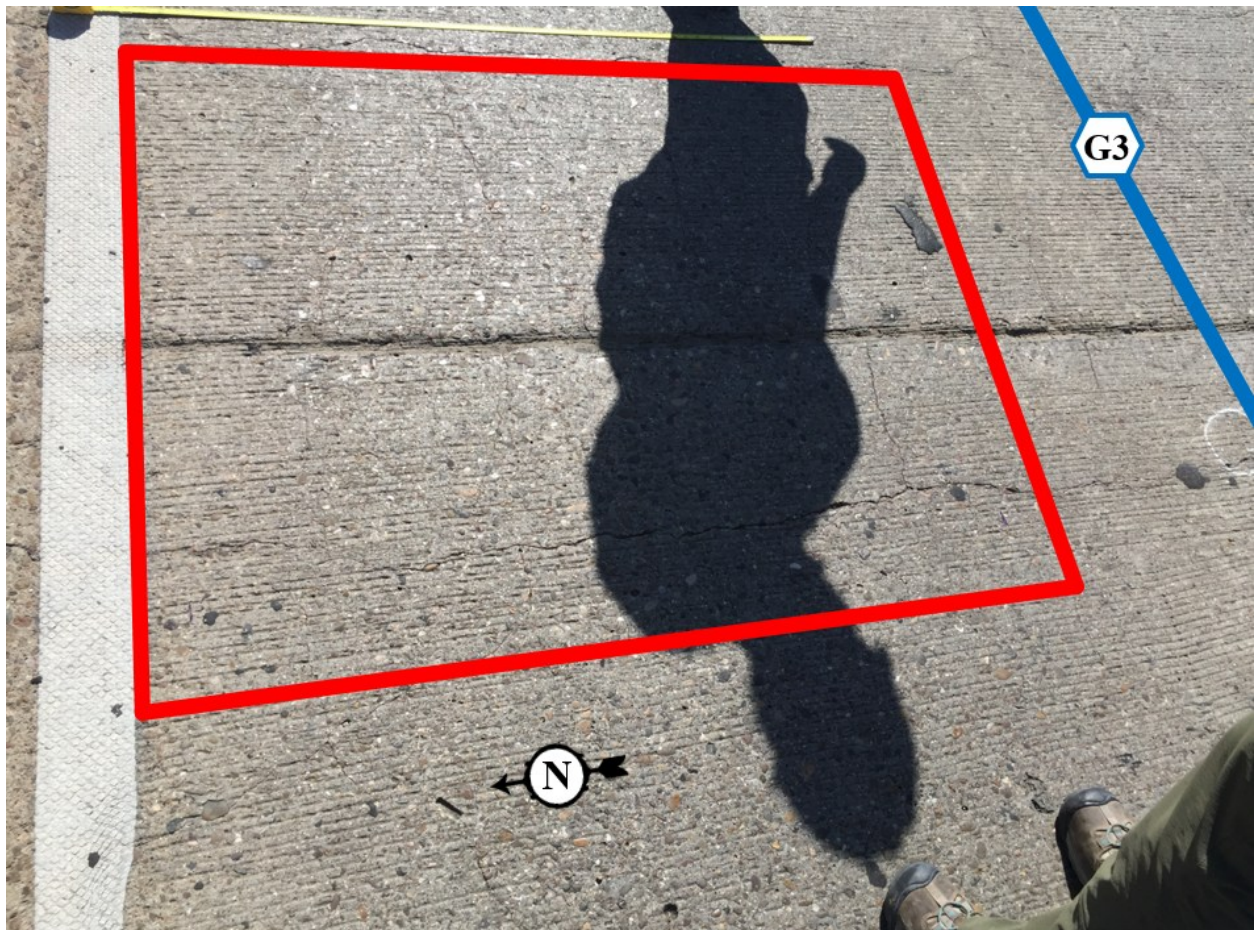
Figure 4.55. Primary NDE region at Bent 3 between G2 and G3 at Bridge LUB4 (WB Loop 289 over University Ave.).
