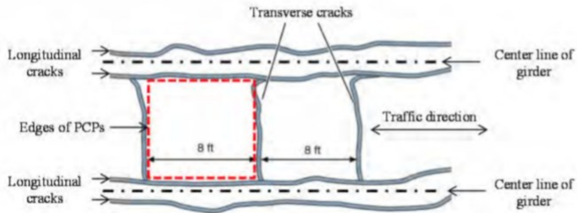
Figure 2.20. Crack pattern for CIP-PCP bridge deck, reprinted from Folliard et al. (2003).
