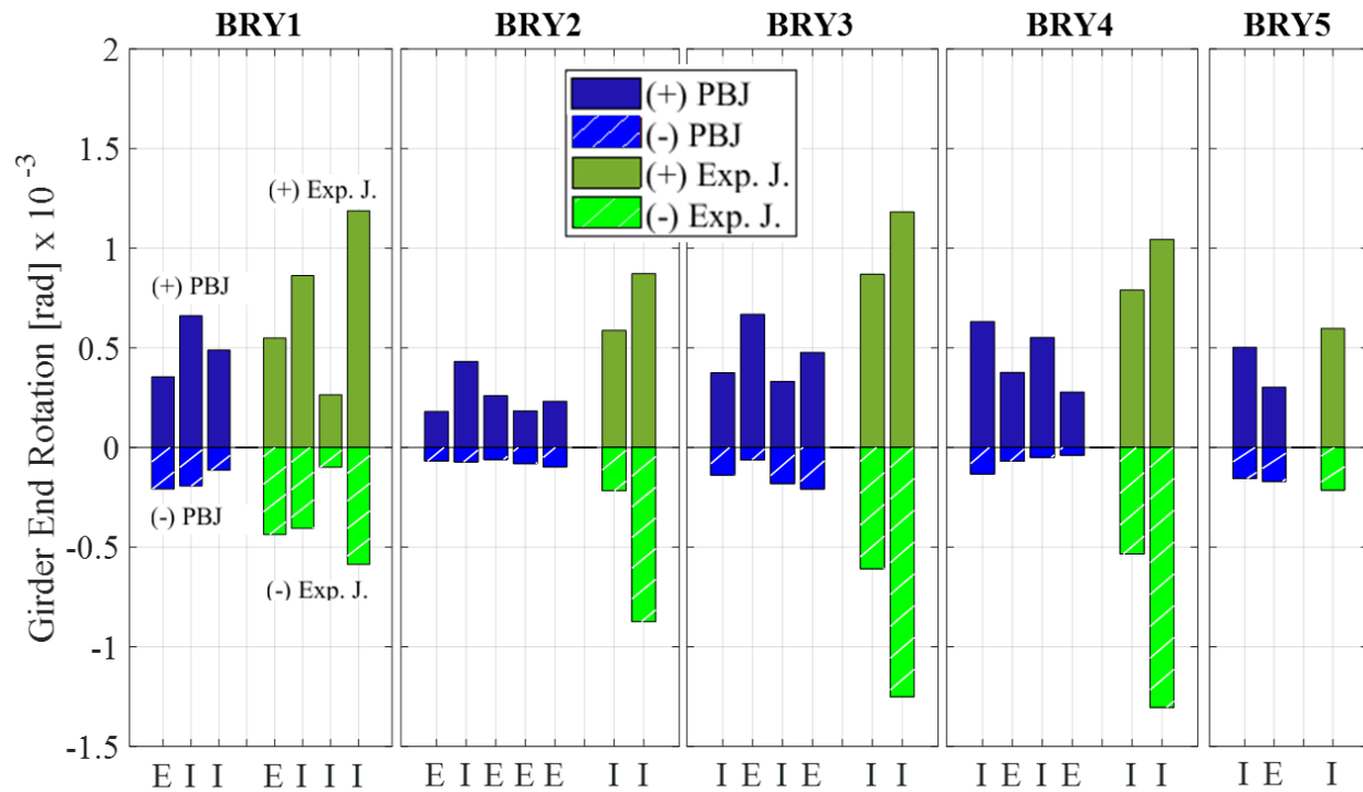
Figure 5.26. Maximum positive and negative live load rotations.
