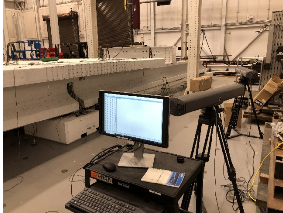
Figure 9.40. Setup of Optotrak cameras (shown for PBJ-FP1).
