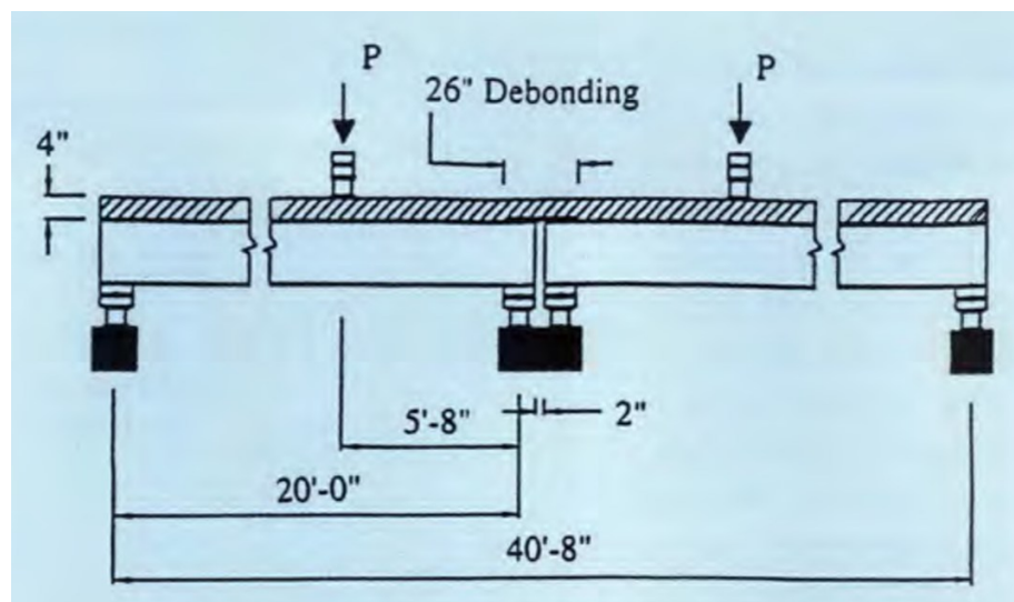
Figure 2.50. Elevation view of specimens, reprinted from Caner and Zia (1998).
