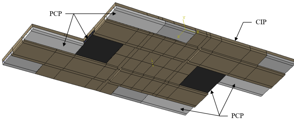
Figure 8.75. Bottom view of the deck for the dual-girder skewed model with the offset panel detail.
