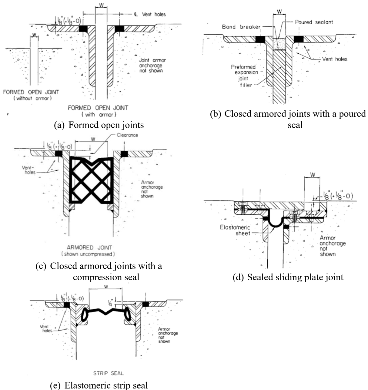
Figure 2.3. Examples of joints in discontinuous decks, reprinted from Burke Jr. (1989).
