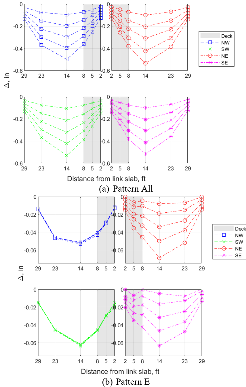
Figure 10.1. PBJ-FP1: Girder displacement profiles at select loads.
