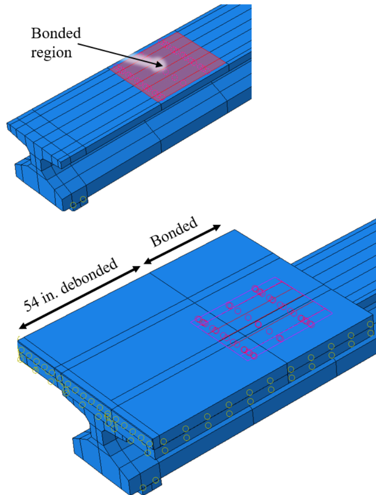
Figure 8.31. Flush precast panel model debonded from the top face of the girder for a length of 54 in.
