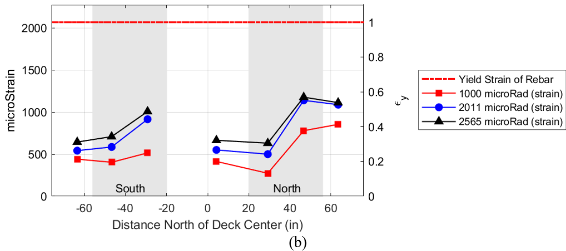
Figure 10.11. PBJ-CP1: Pattern All comparison of (a) crack width profiles and (b) strain width profiles.
