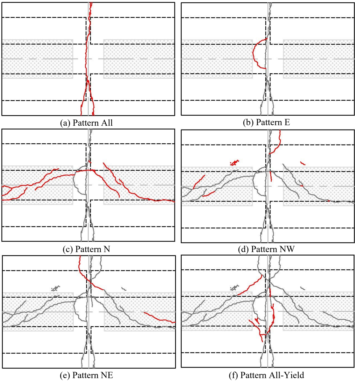
Figure 9.49. PBJ-OP1: Cracks for all load patterns.
