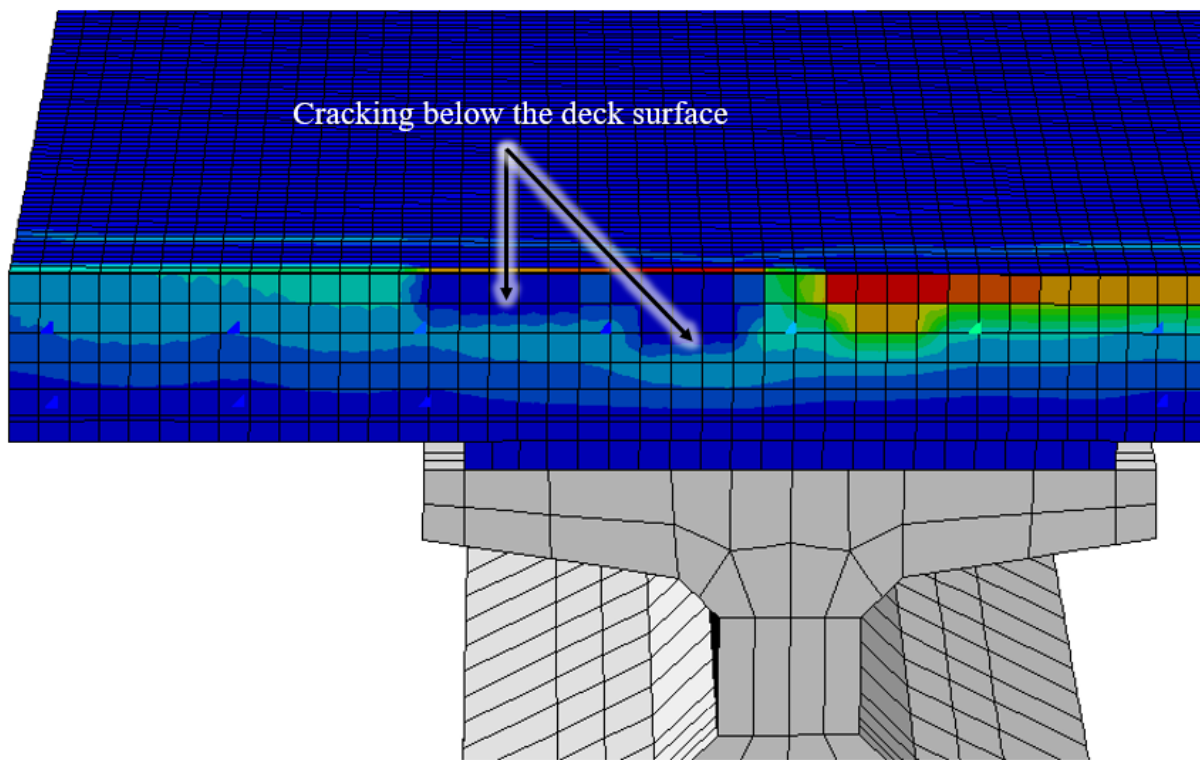
Figure 8.97. Angled section cut of the deck revealing cracking behavior below the deck surface similar to the behavior observed in laboratory testing.
