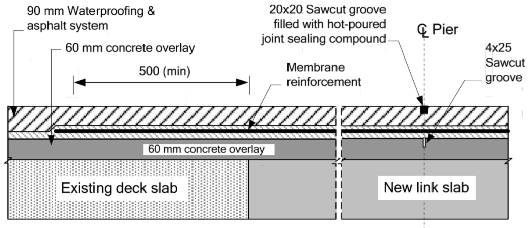
Figure 2.55. Water protection and crack-control details, reprinted from Lam et al. (2008).
