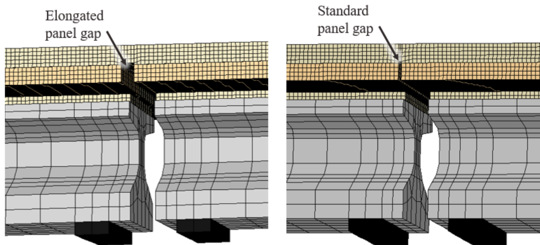
Figure 8.39. Flush precast panel models with a standard 0.75-in. end gap width (right) and an elongated 3-in. end gap width (left).
