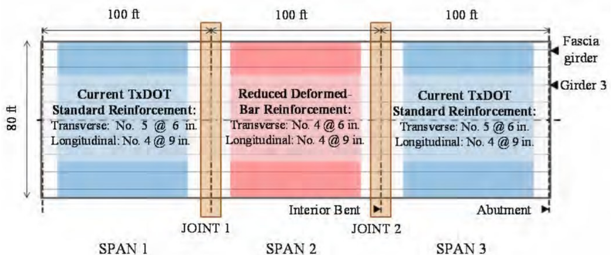
Figure 2.21. Deck reinforcement scheme on Wharton-Weems Overpass, reprinted from Bayrak et al. (2013).
