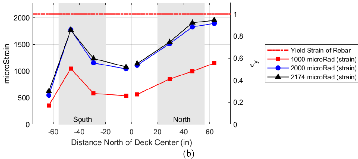
Figure 10.9. PBJ-OP1: Pattern All comparison of (a) crack width profiles and (b) strain width profiles.
