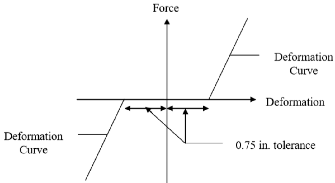
Figure 2.47. Bearing pad force-deformation behavior, reprinted from Snedeker et al. (2011).
