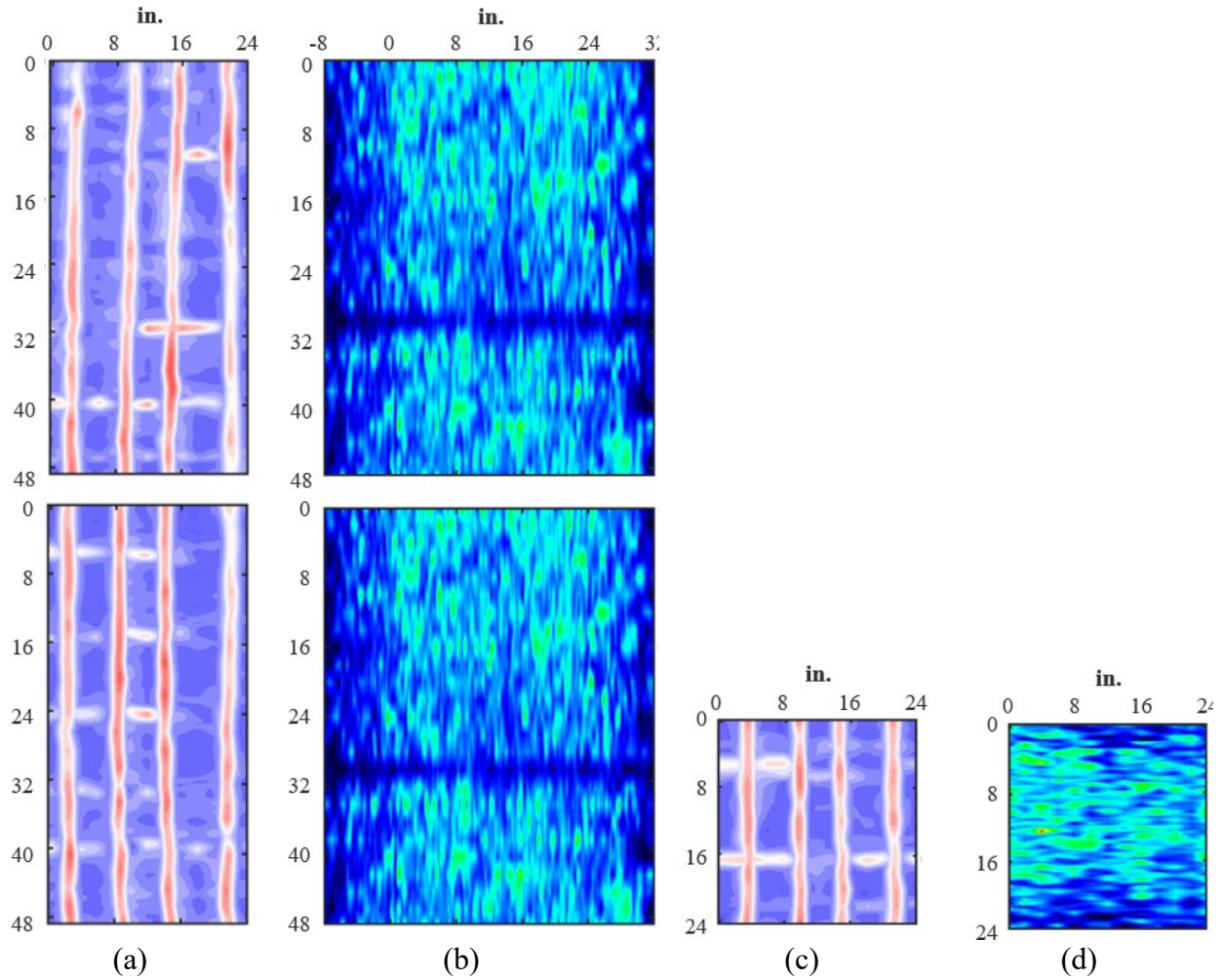
Figure 4.38. LUB1 results for top transverse reinforcement at depth 2.73 in. for (a) GPR in NDE Regions 1 and 2, (b) UST in Regions 1 and 2, (c) GPR in Region 3, and (d) UST in Region 3.
