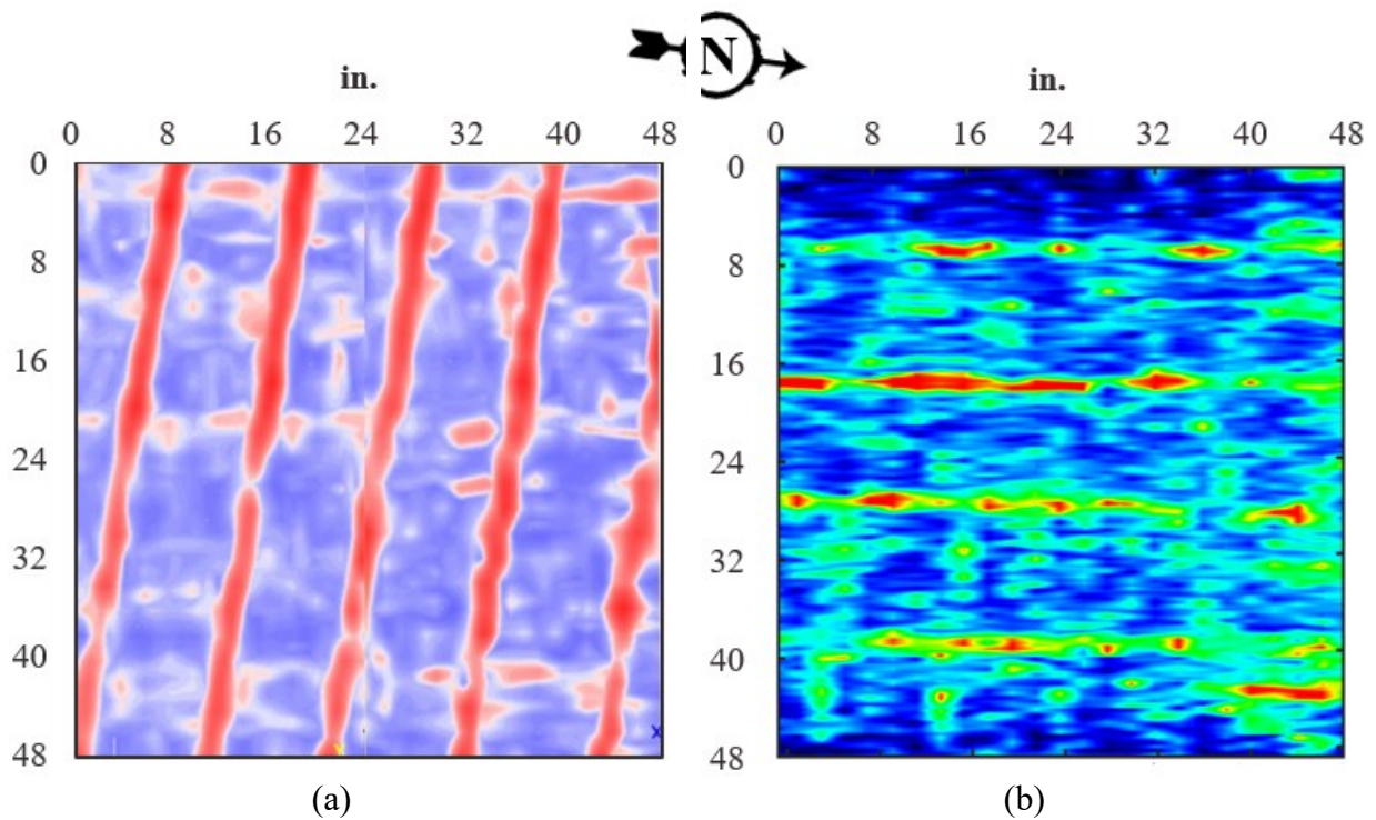
Figure 4.43. LUB2 results for (a) GPR and (b) UST of top longitudinal reinforcement at depth 3.48 in.
