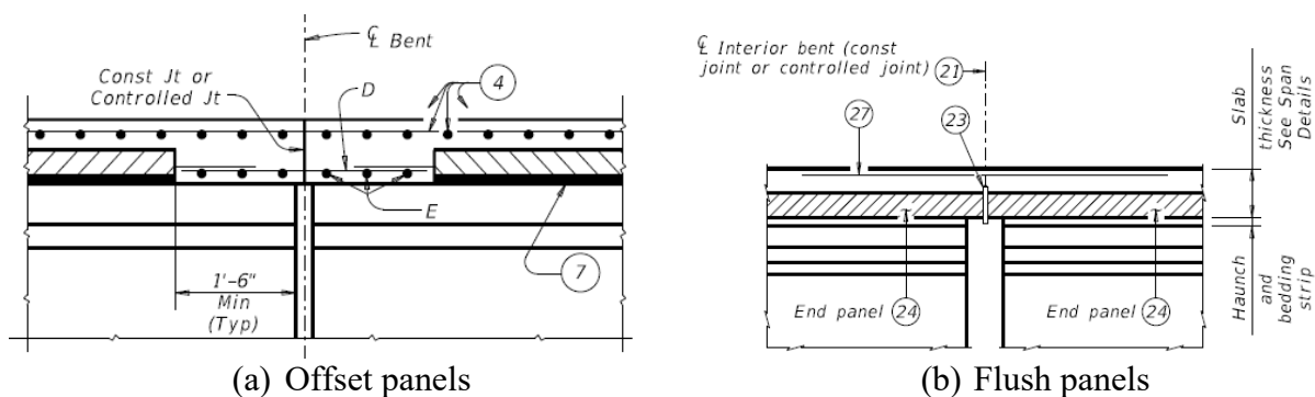
Figure 9.6. TxDOT standard drawing options for continuous deck details.
