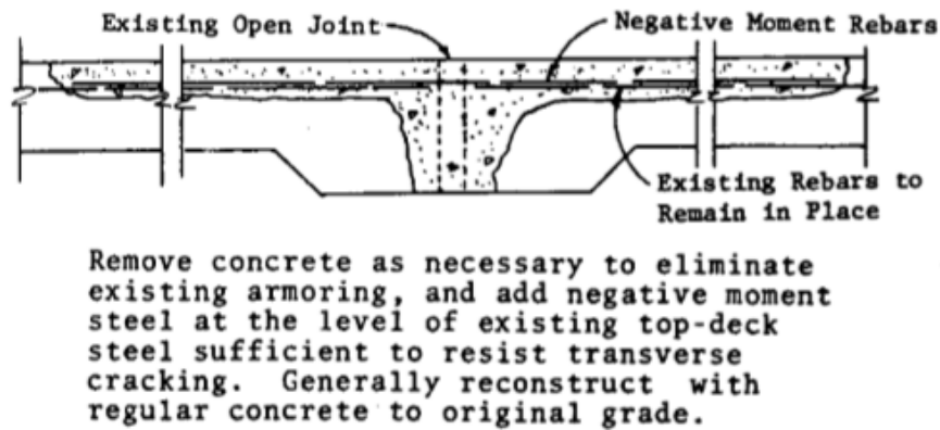
Figure 2.13. 1980s TxDOT expansion joint retrofit to continuous deck, reprinted from Burke Jr. (1989).
