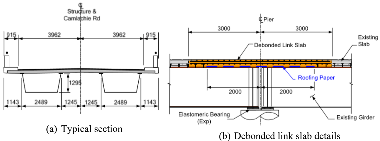
Figure 2.61. Bridge details, reprinted from Au et al. (2013).
