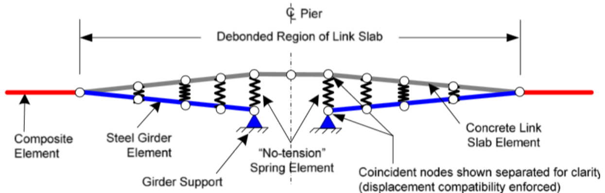
Figure 2.62. Spring model of link slab, reprinted from Au et al. (2013).
