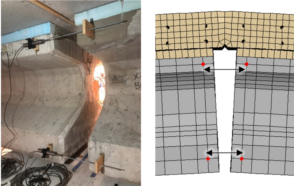
Figure 8.89. LVDTs recording deformation at the girder ends (left) and nodes of matching LVDT connection points on the FEM (right).
