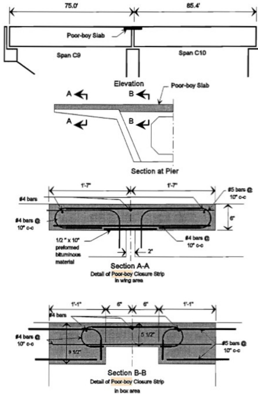
Figure 2.14. Poor boy continuous slab details, reprinted from Roberts et al. (1993).
