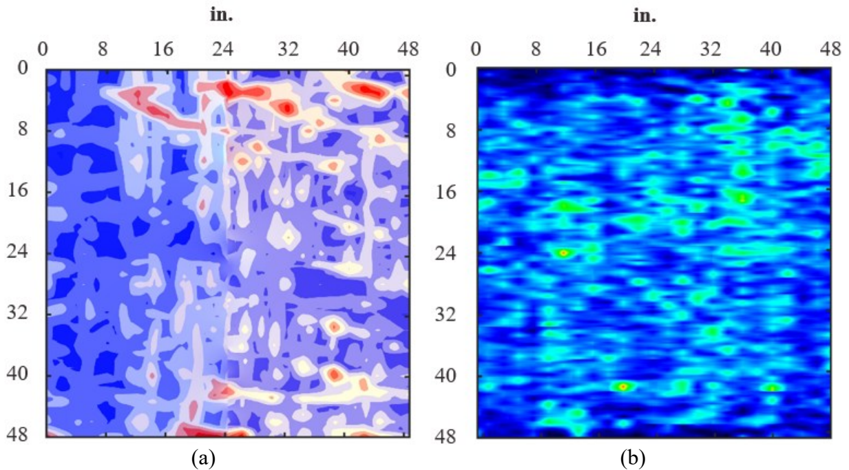
Figure 4.52. LUB3 results for (a) GPR and (b) UST of the PCP end gap at depth 8.5 in.
