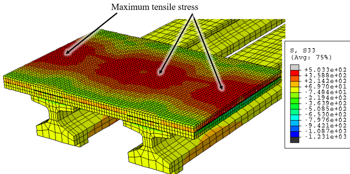
Figure 8.60. Longitudinal concrete stresses formed by uniform shrinkage in the deck, causing potential cracking within the section.
