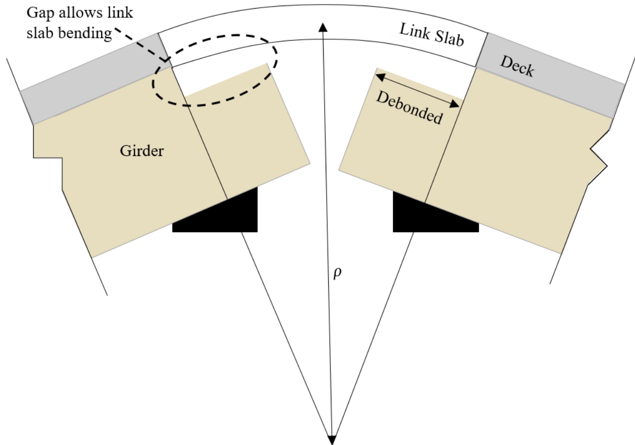
Figure 8.11. DLS diagram showing that the girder ends do not interfere with link slab deformation when a gap is provided along the debonded length, causing a longer radius of curvature, \rho , for the link slab.
