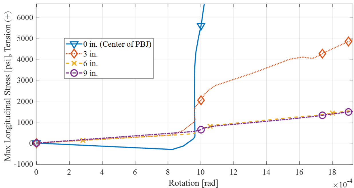
Figure 8.36. Top longitudinal steel stresses for the partial-depth debonded model showing that the bars at the center of the PBJ develop compressive stress prior to cracking.
