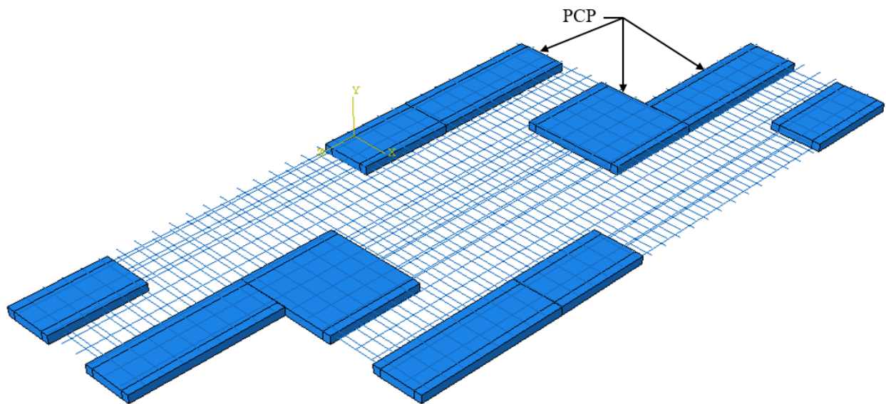
Figure 8.74. Top view of the PCPs and reinforcement for the dual-girder skewed model with the offset panel detail.
