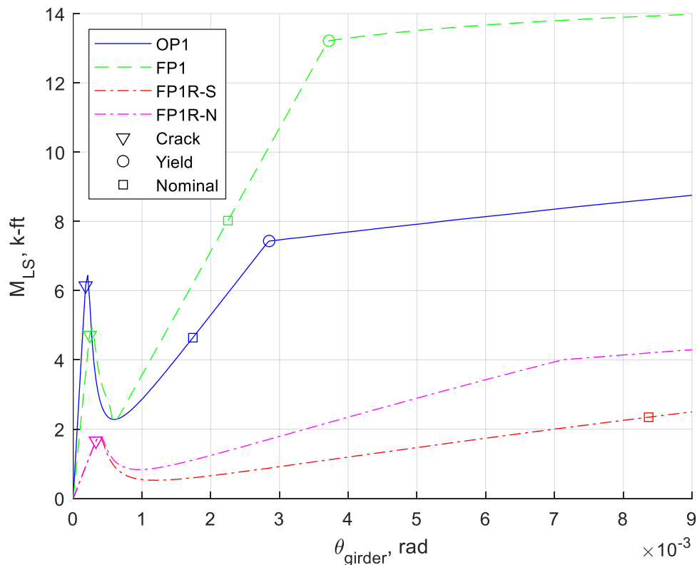
Figure 9.35. Moment-rotation response of link slab for design material properties and assumed link slab length of 12 in.
