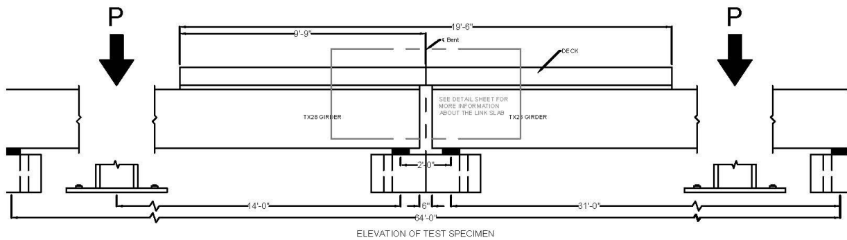
Figure 9.5. Generic elevation of specimens showing geometry.
