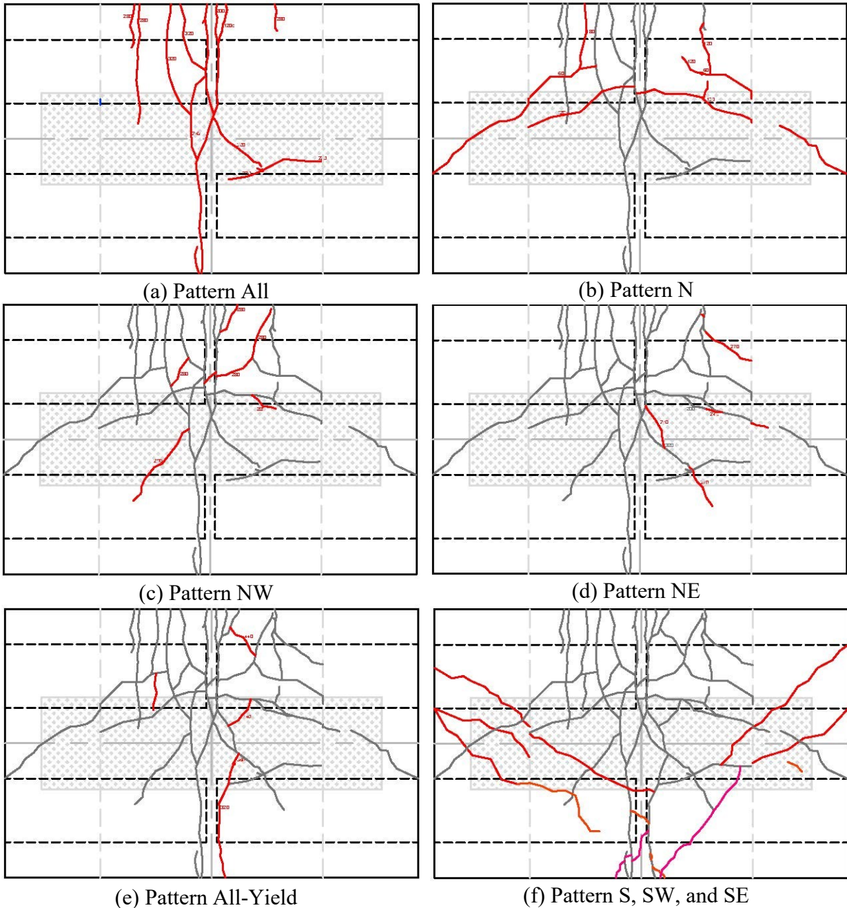
Figure 9.48. PBJ-FP1R: Cracks for all load patterns.
