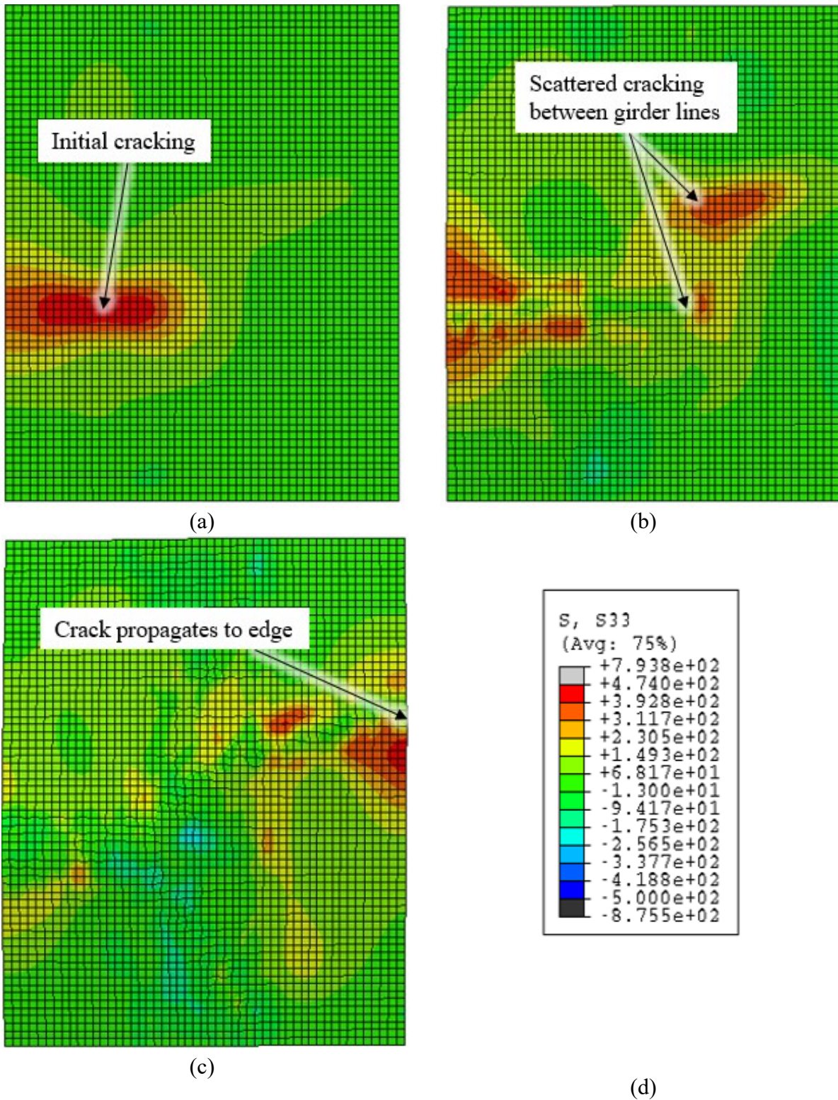
Figure 8.69. Longitudinal stress propagation in the deck of the non-skewed girder end model.
