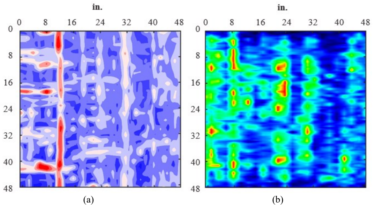
Figure 4.9. ATL1 results for (a) GPR and (b) UST of PMDF at depth 8.5 in.
