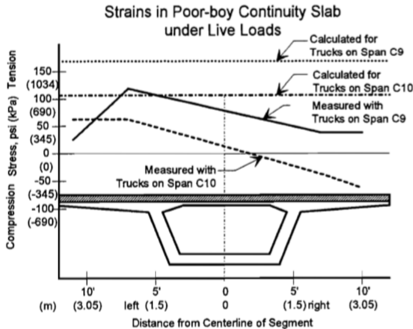
Figure 2.15. Link slab stresses, reprinted from Roberts et al. (1993).
