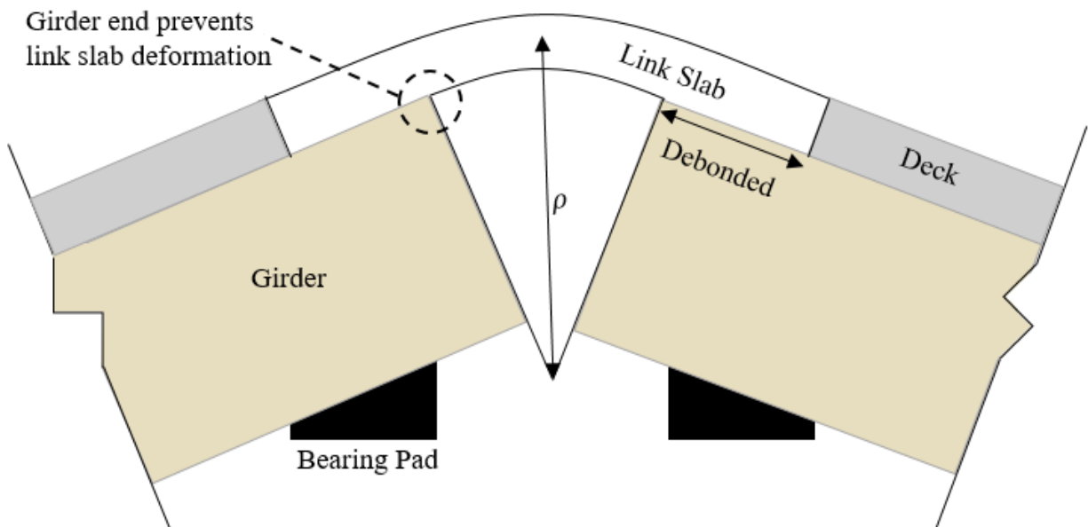
Figure 8.9. DLS diagram showing the girder ends interfering with intended link slab deformation, causing a short radius of curvature, \rho , for the link slab.
