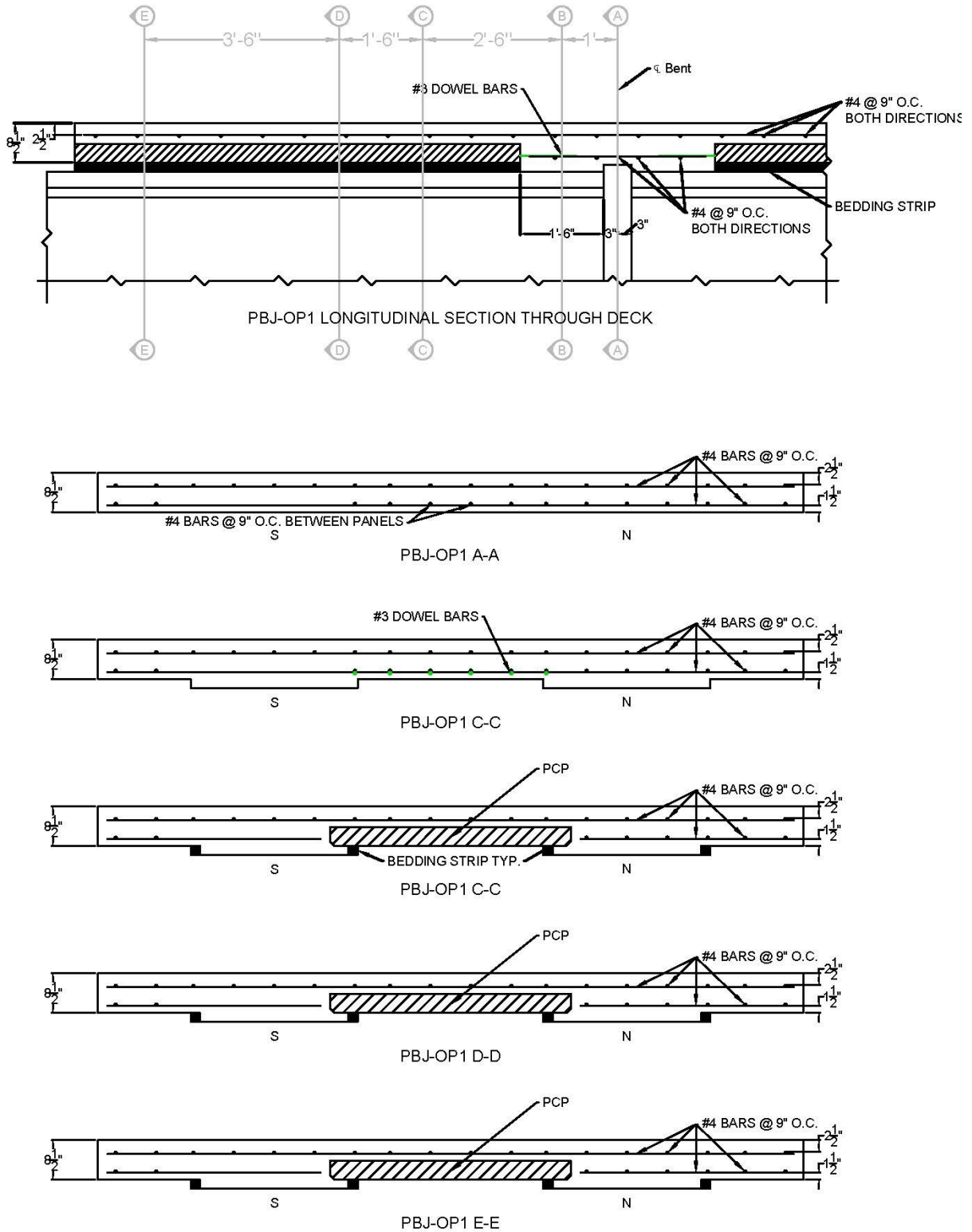
Figure B.3. PBJ-OP1: construction drawings.
