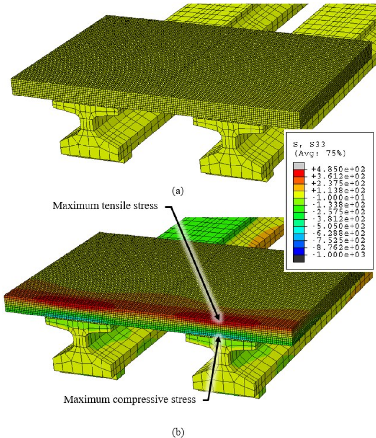
Figure 8.21. Longitudinal stresses in CIP deck concrete (psi), showing (a) the unloaded condition and (b) the formation of a force couple in the deck, concentrated over the girders.
