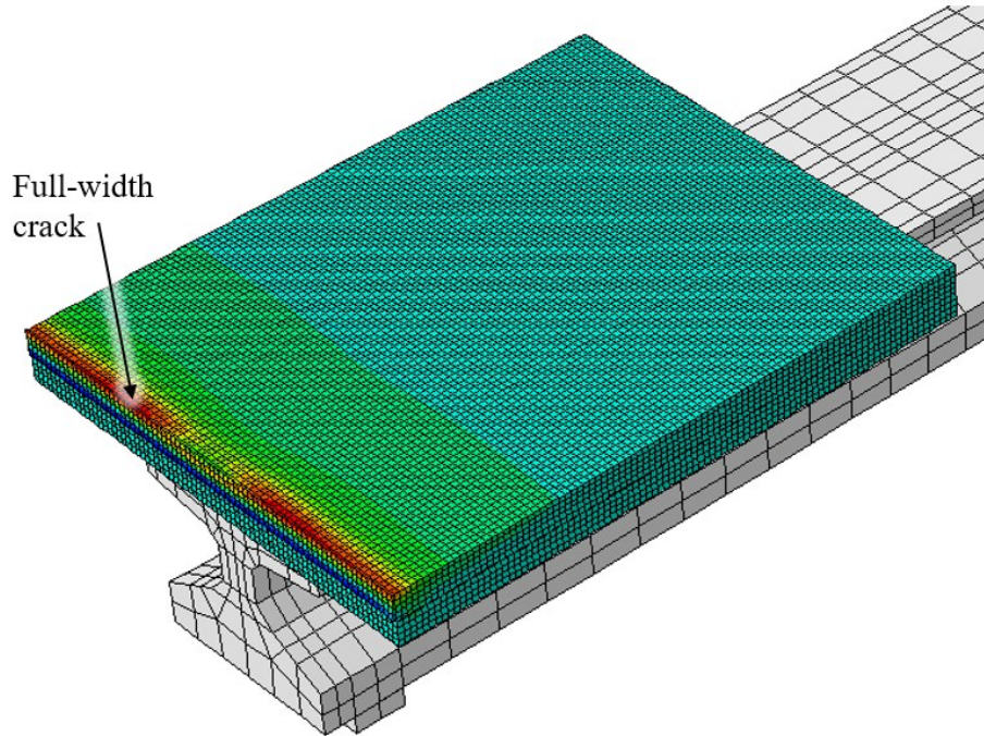
Figure 8.32. Debonded flush precast panel model with cracks across the full width of the deck above the panel gap.
