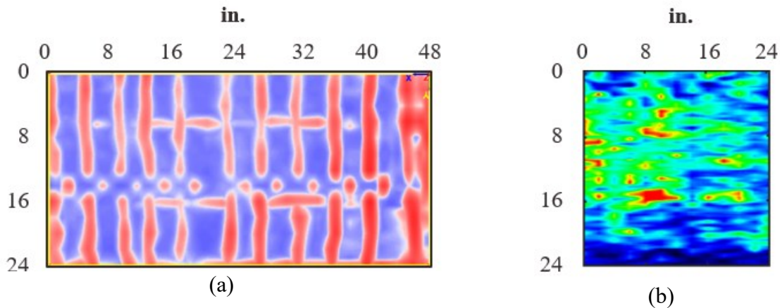
Figure 4.63. LUB4 results for the secondary NDE area for (a) GPR and (b) UST of the top transverse reinforcement in the overhang at depth 3.48 in.
