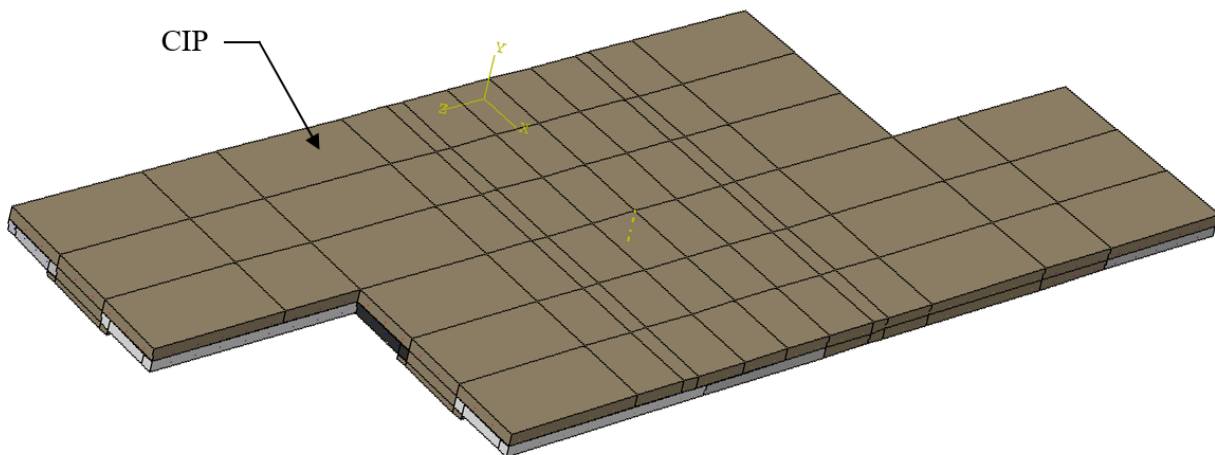
Figure 8.73. Top view of the deck for the dual-girder skewed model.
