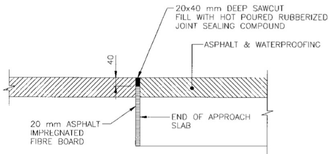
Figure 2.74. Approach slab expansion joint detail, reprinted from Husain and Bagnariol (2000).
