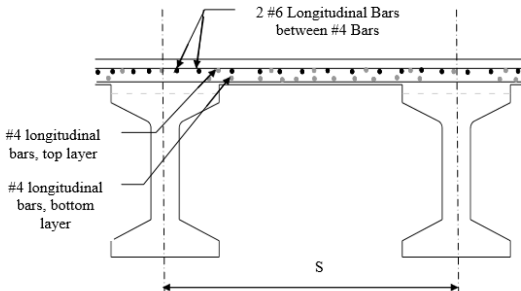
Figure 2.44. Reinforcement placement at continuous deck detail, reprinted from Snedeker et al. (2011).
