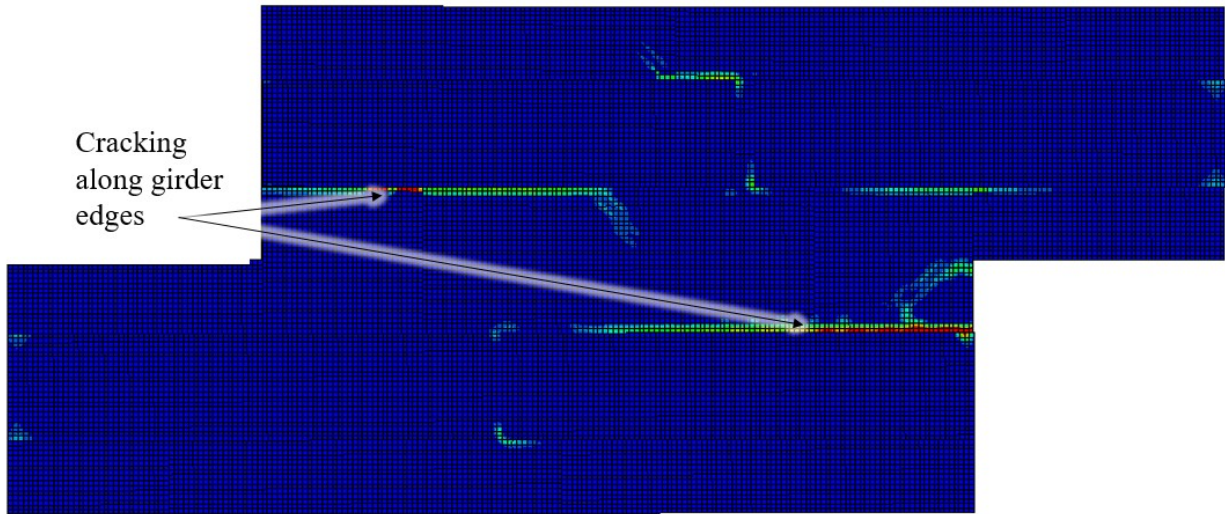
Figure 8.77. Cracking in the bottom of the deck for the dual-girder skewed model, primarily along the girder edges.
