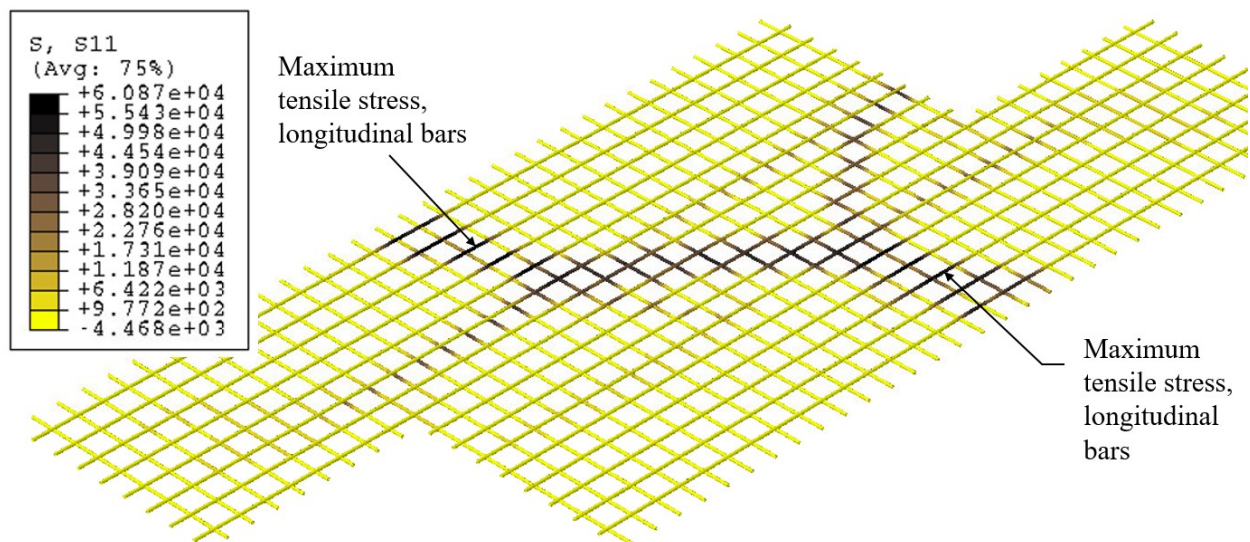
Figure 8.78. Stress in the top longitudinal and transverse bars for the skewed model, showing maximum tensile stresses forming over the girder, with stresses extending diagonally between girder lines following the cracking pattern.
