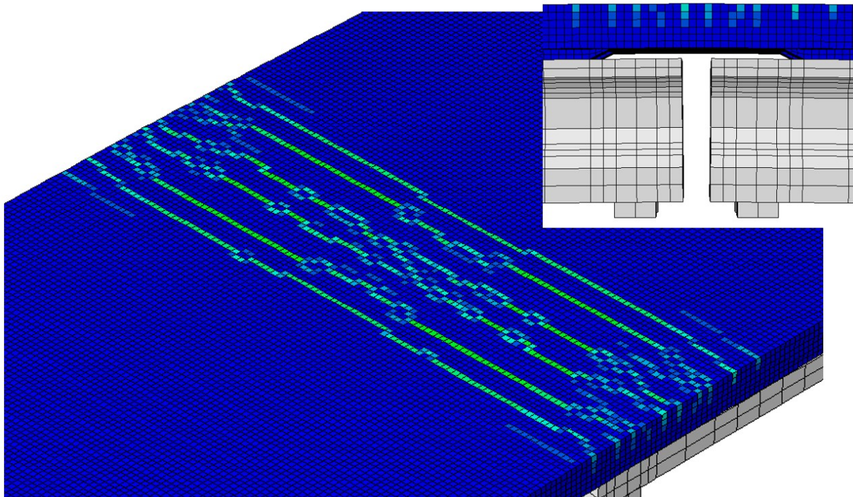
Figure 8.48. Cracking pattern for an offset precast panel model, debonded for 18 in. with a vertical gap along the debonded length, and tapered ends of the debonded region.
