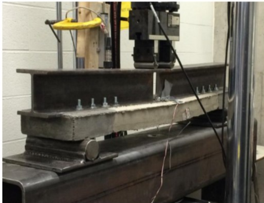
Figure 2.70. ECC link slab specimen under load test, reprinted from Samani (2015).
