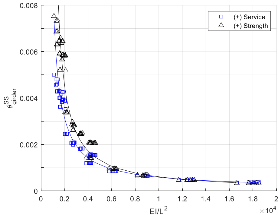
Figure 9.45. Girder end rotations for design of TxDOT standard I-girder bridges (only positive bending shown).
