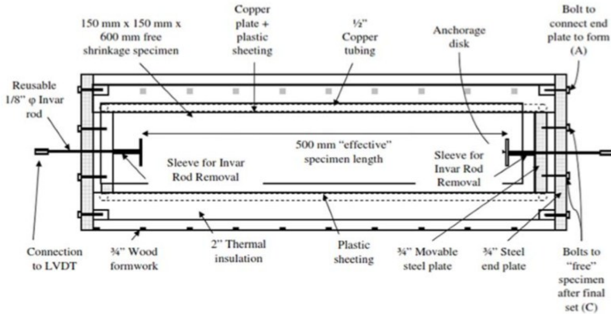
Figure 2.12. Diagram of shrinkage test setup, reprinted from Pesek et al. (2013).
