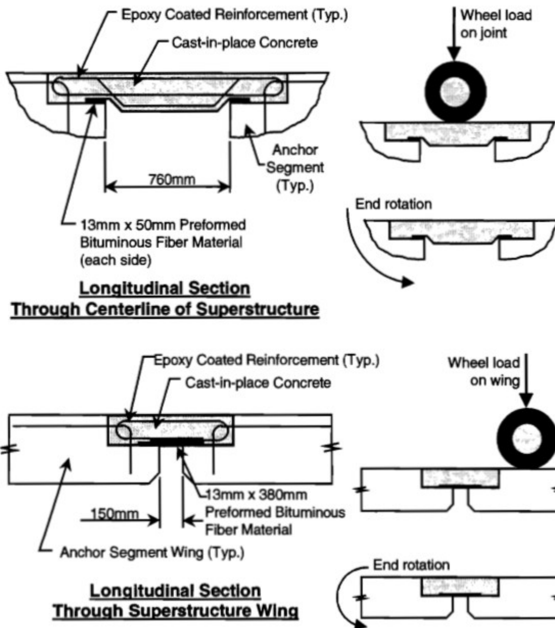
Figure 2.18. Link slab sections, reprinted from Davis et al. (1999).
