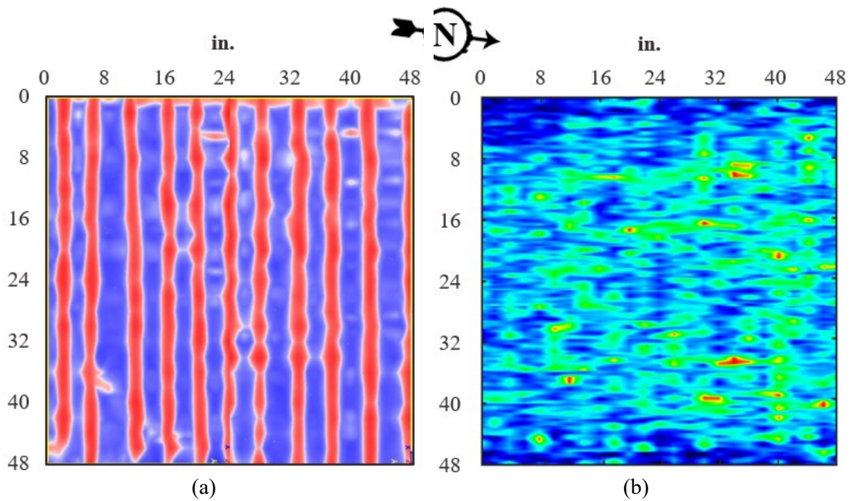
Figure 4.50. LUB3 results for (a) GPR and (b) UST of top longitudinal reinforcement at depth 4.73 in.
