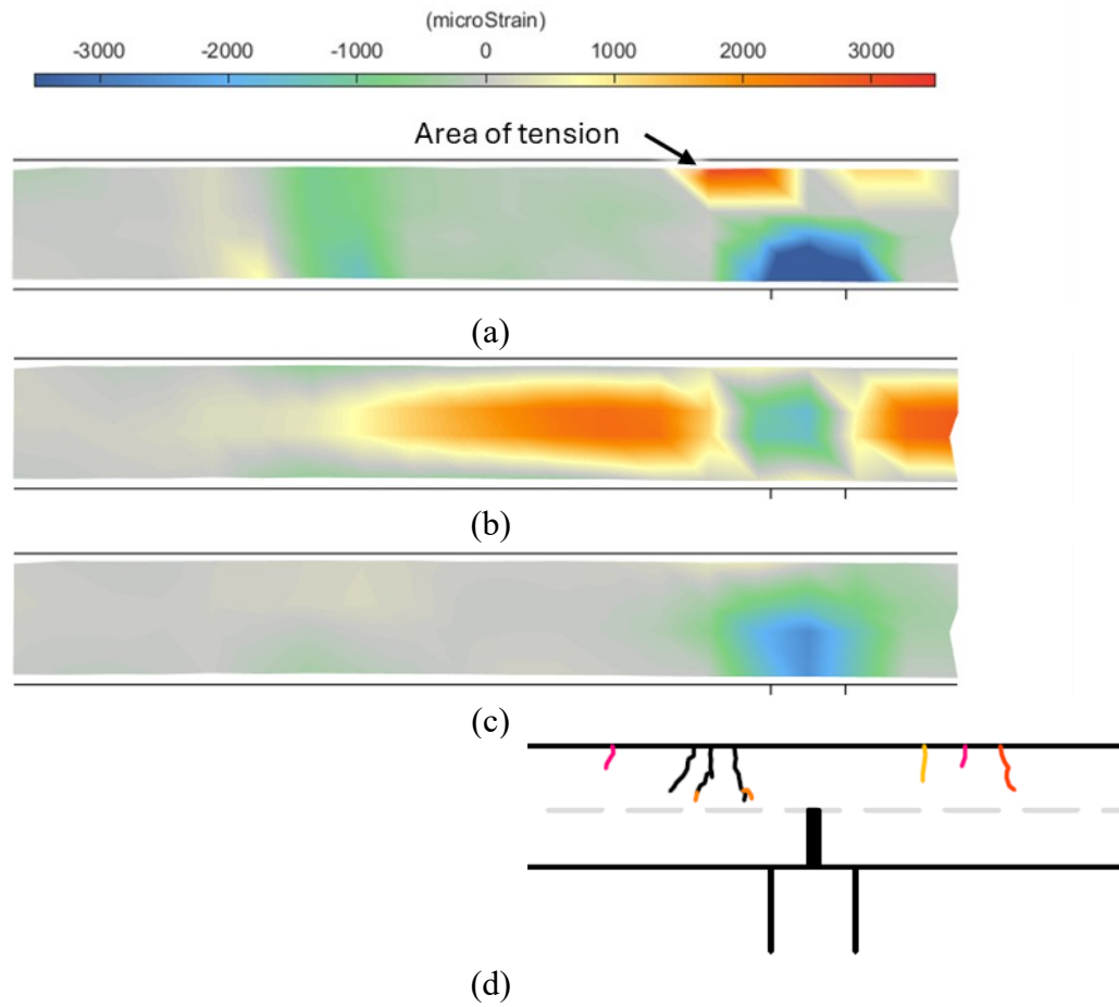
Figure 10.29. Optotrak strains for PBJ-FP1R Pattern All-Yield: (a) horizontal, (b) vertical, (c) shear strain, and (d) crack pattern.
