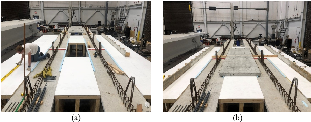
Figure 9.16. Installation of bottom formwork and placement of PCPs (shown for PBJ-FP1).
