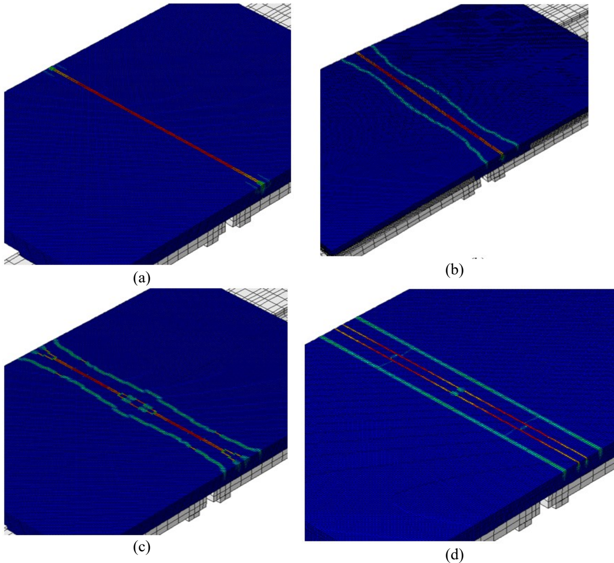
Figure 8.43. Crack patterns for different offset precast panel models: (a) bonded, (b) debonded, (c) debonded without a bottom notch, and (d) debonded without a bottom notch and with additional top longitudinal rebar.
