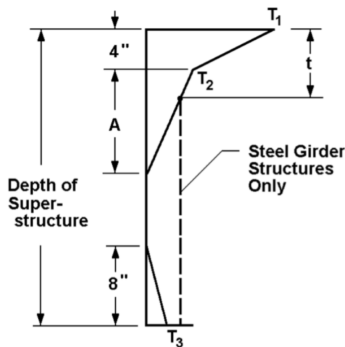
Figure 2.4. Girder temperature gradient, reprinted from AASHTO (2017).
