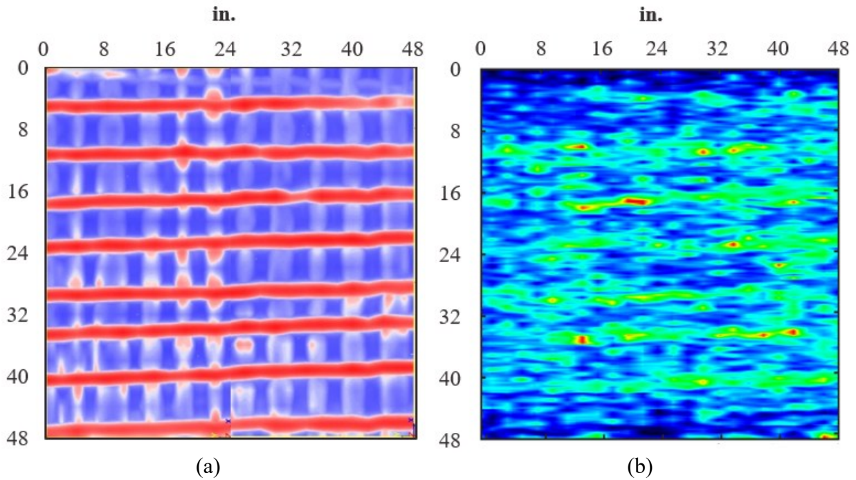
Figure 4.51. LUB3 results for (a) GPR and (b) UST of top transverse reinforcement at depth 3.73 in.
