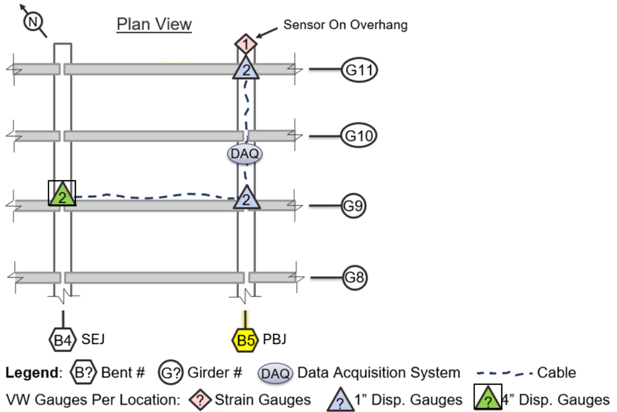
Figure 5.15. Instrumentation plan for Bridge BRY5 (SH 6 over Nantucket Dr.).
