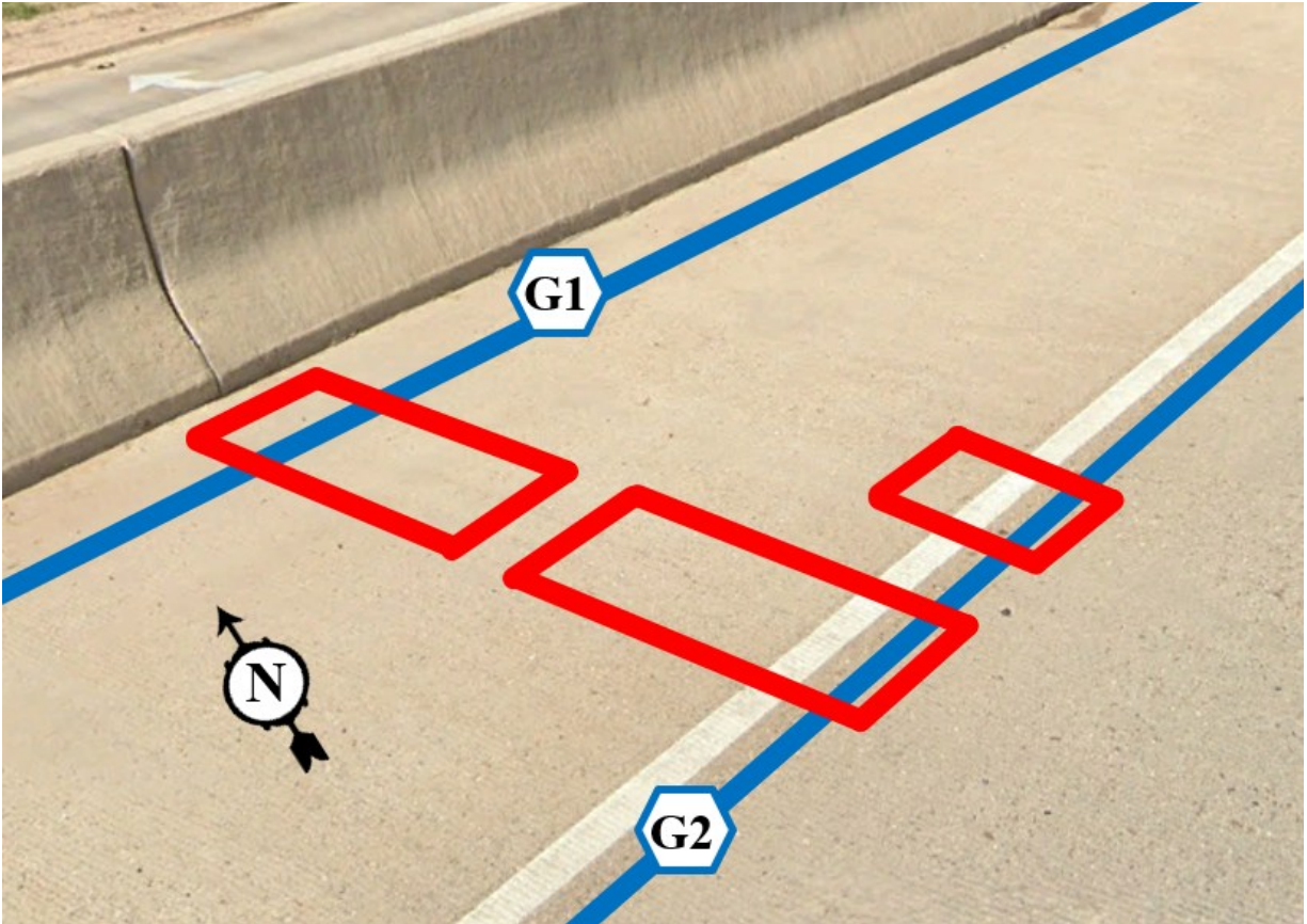
Figure 4.36. Primary NDE regions (1 and 2) at Bent 3 for Bridge LUB1 (SB Loop 289 over Slide Rd./4th St.) with the smaller secondary NDE region (Region 3) east of the primary regions adjacent to G2.
