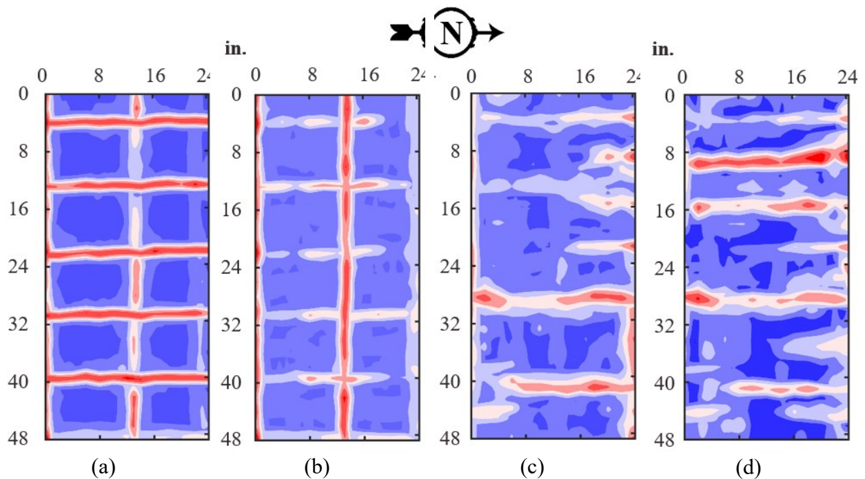
Figure 4.32. ATL4 GPR results in the overhang for (a) top transverse reinforcement at depth 4.23 in., (b) top longitudinal reinforcement at depth 4.98 in., (c) bottom reinforcement at 8.23 in., and (d) bottom reinforcement at 8.73 in.
