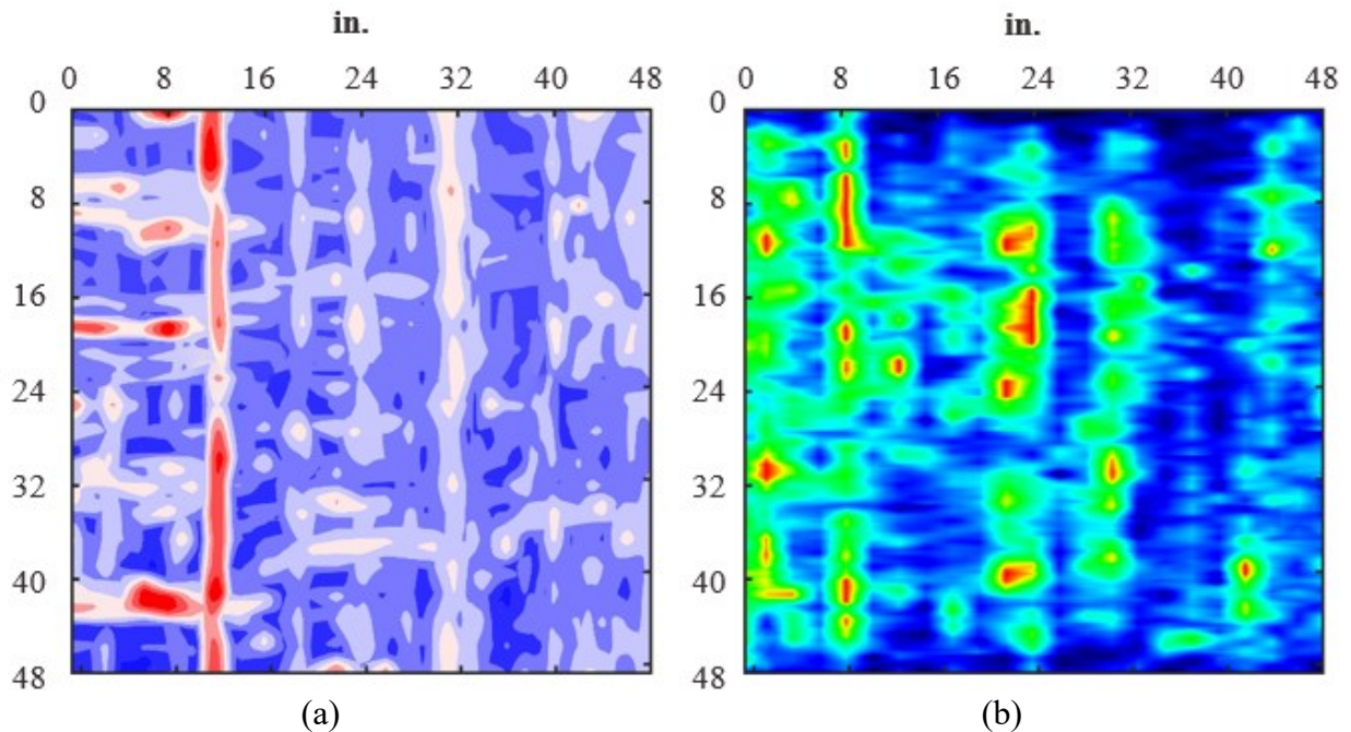
Figure 4.8. ATL1 results for (a) GPR and (b) UST of bottom reinforcement at depth 7.48 in.
