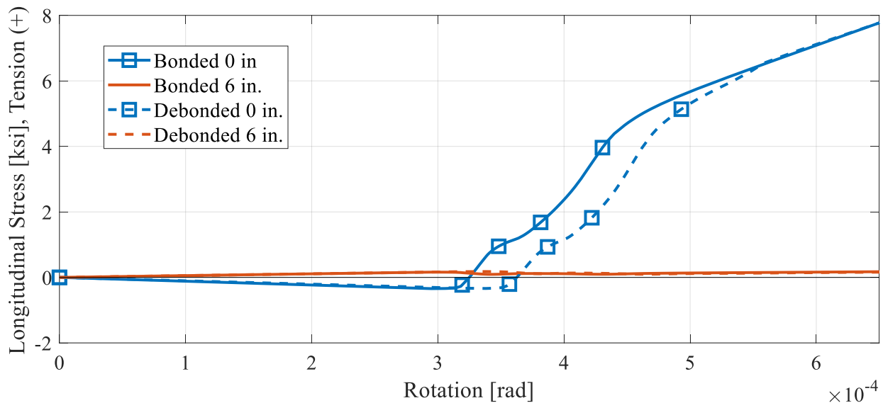
Figure 8.34. Bonded and debonded flush precast panel model steel stresses at the center of the PBJ (0 in.) and at 6 in. away longitudinally from the PBJ.
