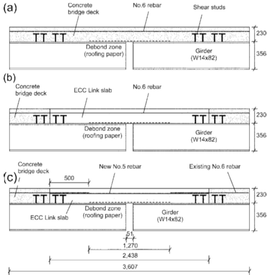
Figure 2.65. Diagrams of the three link slab specimens, dimensions in mm (1 in. = 25.4), reprinted from Kim et al. (2004).
