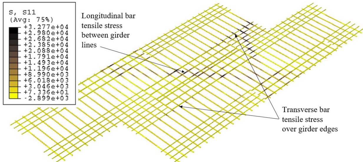
Figure 8.84. Stress in the bottom longitudinal and transverse bars for the debonded skewed model, showing tensile stresses forming over the girder edges, with stresses extending diagonally between girder lines following the cracking pattern.
