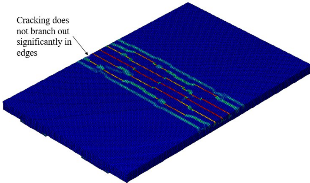
Figure 8.58. 36-in. debonded continuous panel model crack behavior, showing crack propagation at high rotations.
