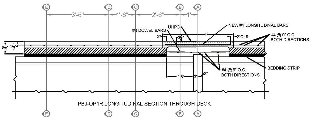
Figure 9.10. PBJ-OP1R elevation view.
