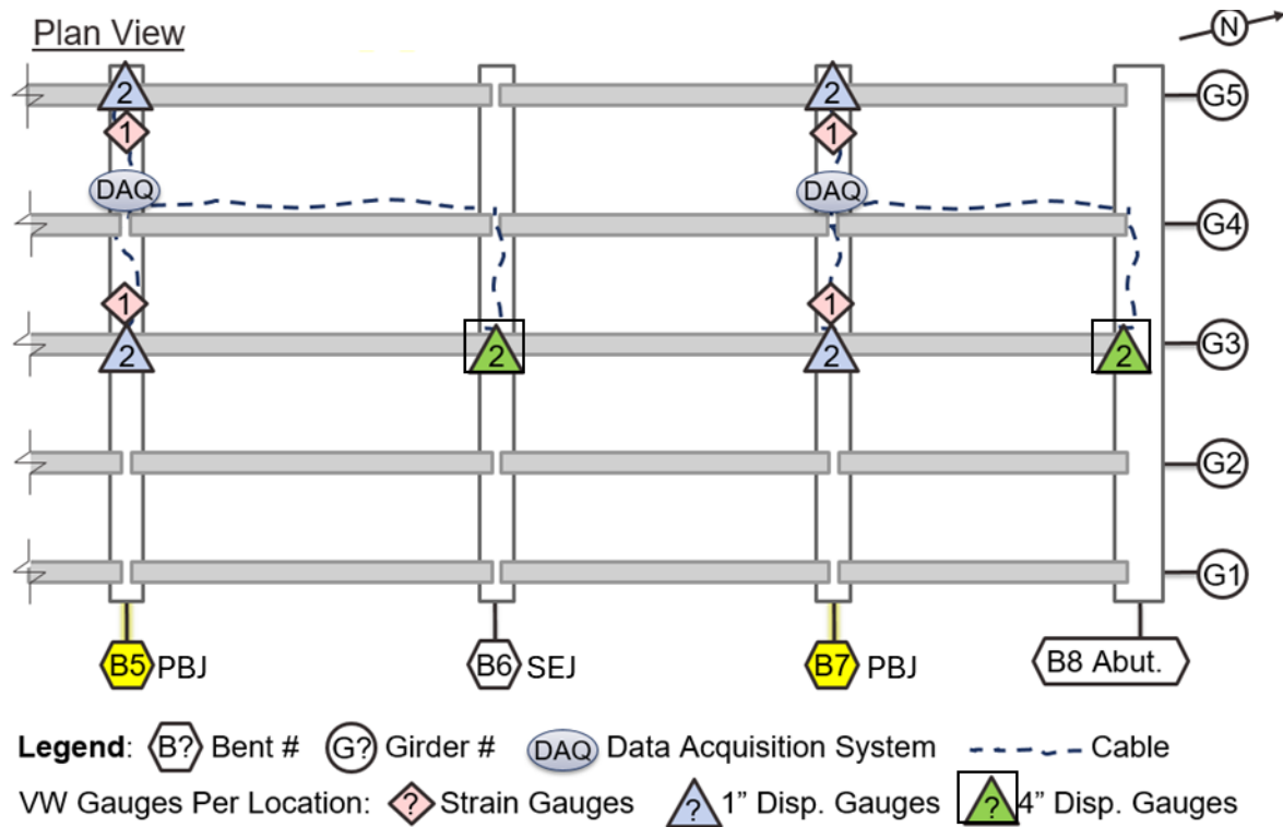
Figure 5.11. Instrumentation plan for Bridge BRY3 (SH 21/US 190 over Old Cedar Creek).
