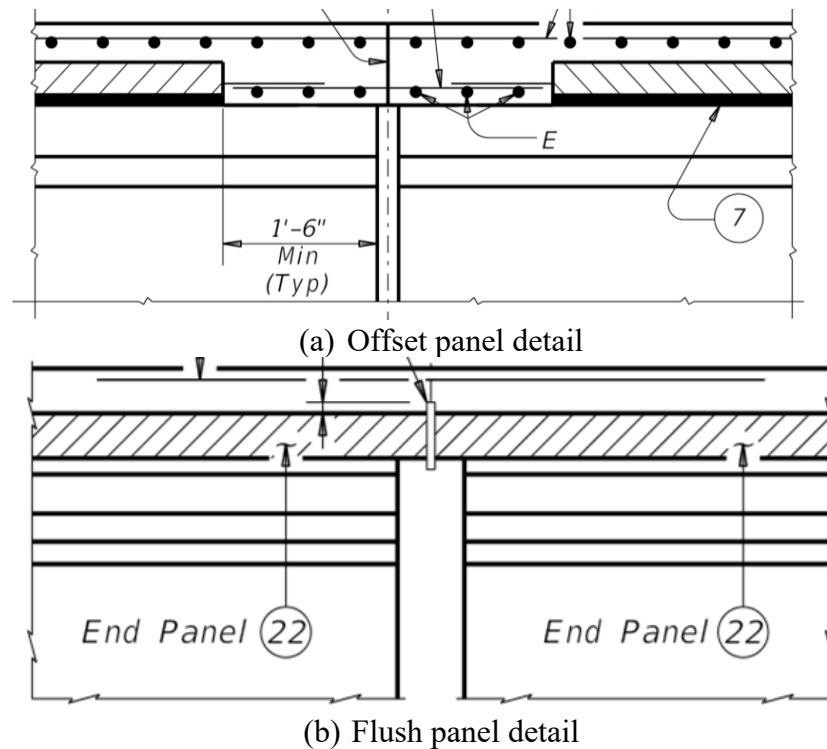
Figure 6.1. TxDOT PBJ detailing with partial-depth PCPs.
