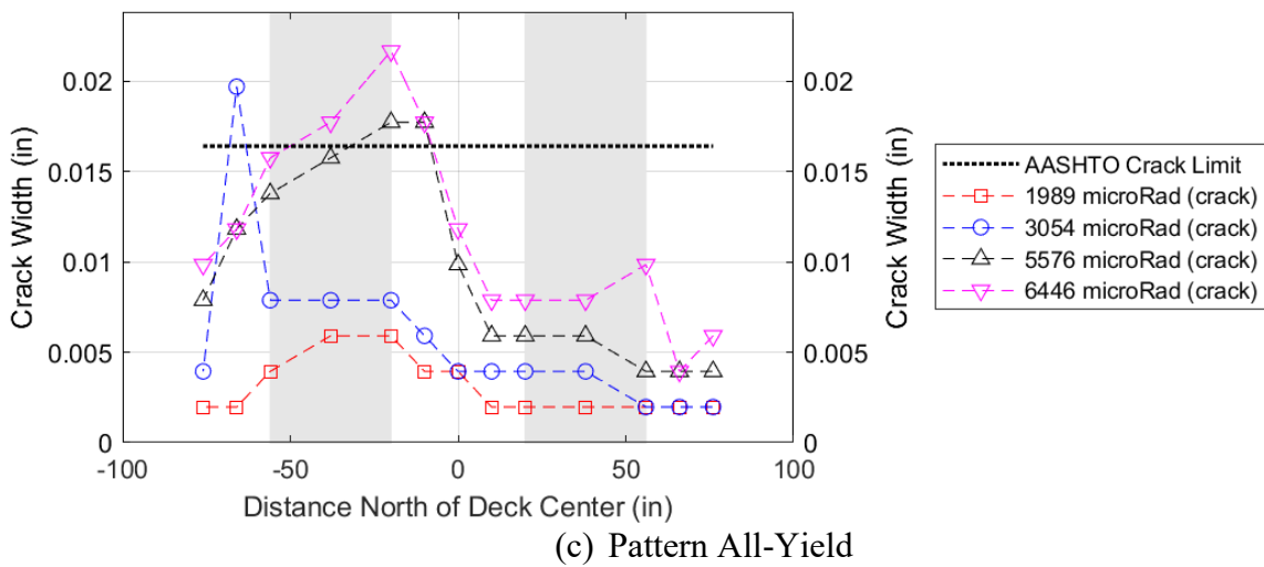
Figure 10.6. PBJ-FP1R: Crack width profiles for select patterns.
