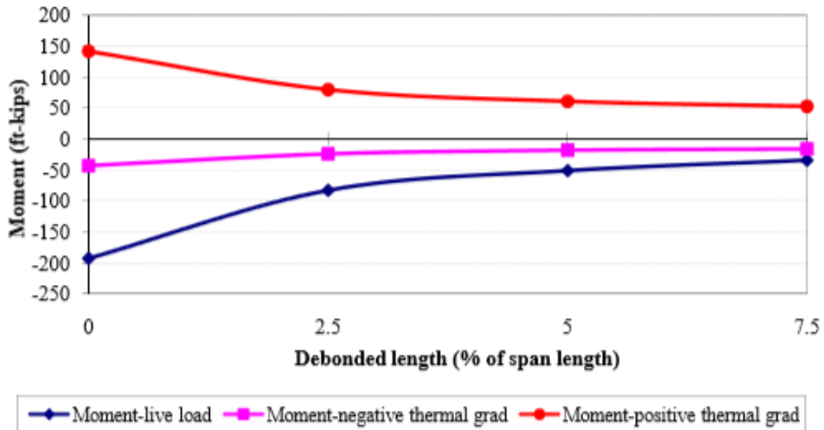
Figure 2.52. Moment demand for different debonded lengths, reprinted from Aktan et al. (2008).
