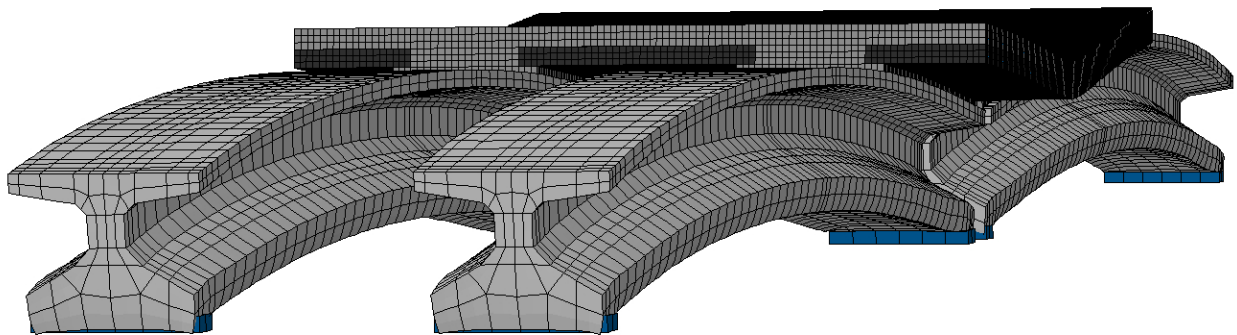
Figure 8.19. Negative bending due to thermal gradient with deformation exaggerated to show girder curvature.
