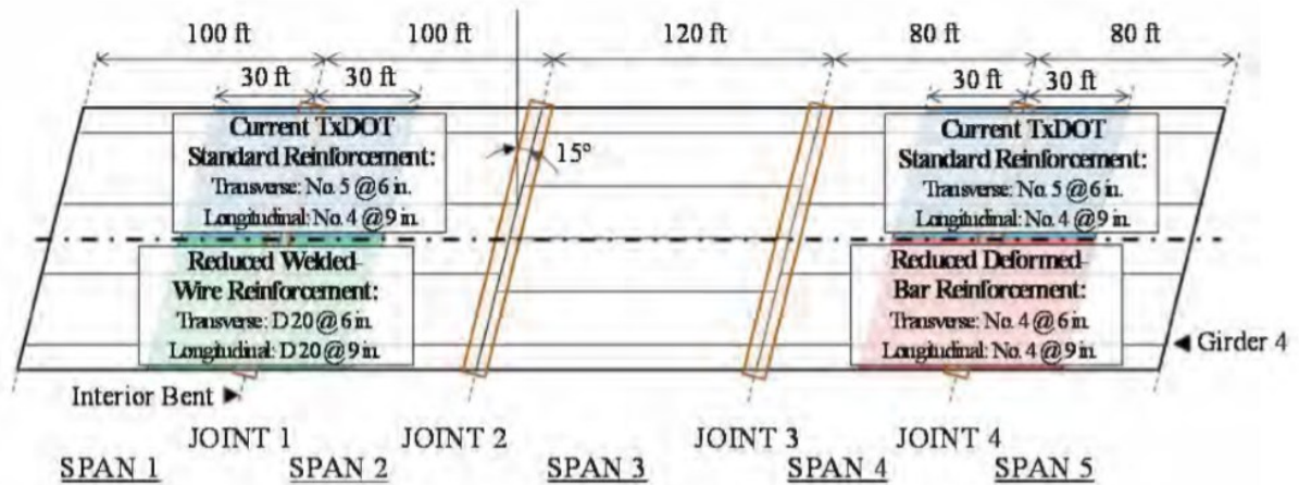
Figure 2.27. Deck reinforcement scheme on Lampasas River Bridge, reprinted from Bayrak et al. (2013).
