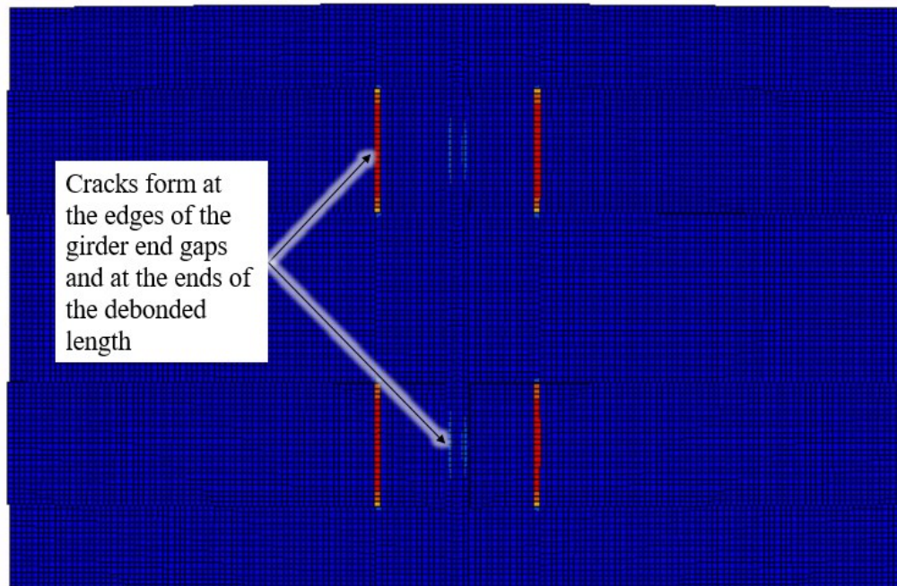
Figure 8.64. Crack pattern in the bottom of the slab for an 18-in. debonded offset precast panel model loaded with negative temperature gradient.
