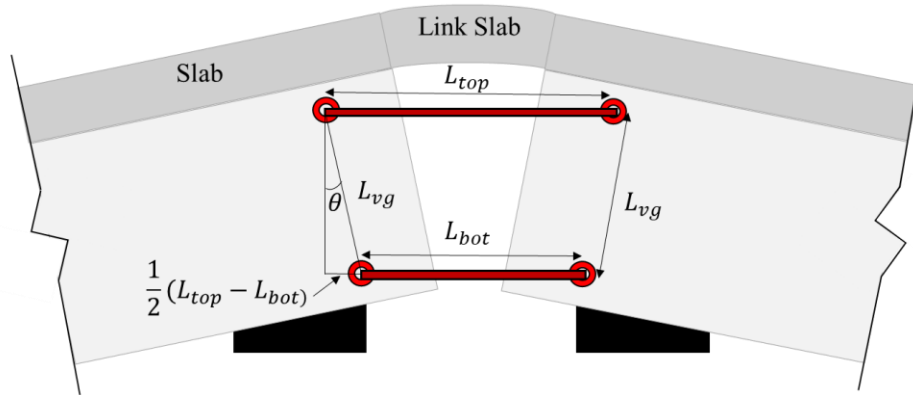
Figure 5.4. Variables used for the calculation of girder end rotations from displacement gages.
