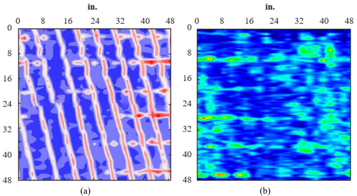
Figure 4.14. ATL2 results for (a) GPR and (b) UST of top transverse reinforcement at depth 2.98 in.
