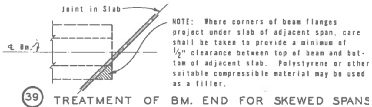
Figure 6.5. Prestressed concrete beam span details of 1971.
