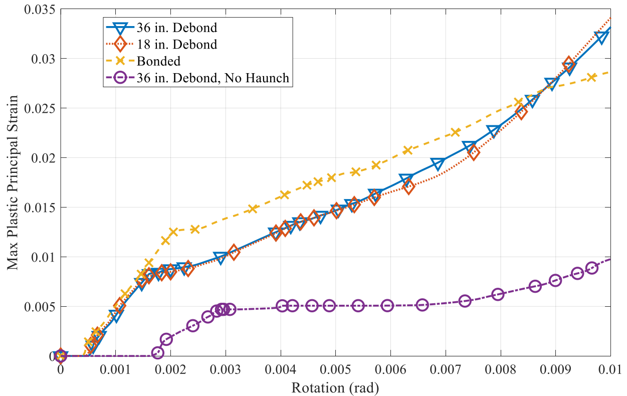
Figure 8.46. Maximum plastic principal strains for different offset panel models at the location of first cracking.
