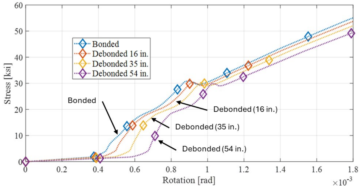
Figure 8.27. Comparison of top longitudinal steel stresses at different lengths of debonded slab, showing that debonding delays steel stress and crack formation.
