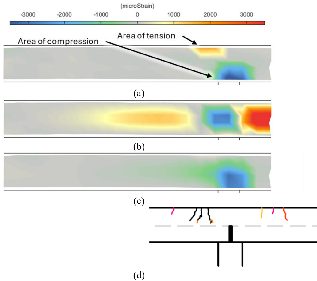
Figure 10.30. Optotrak strains for PBJ-FP1R Pattern East(a) horizontal, (b) vertical, (c) shear strain, and (d) crack pattern.
