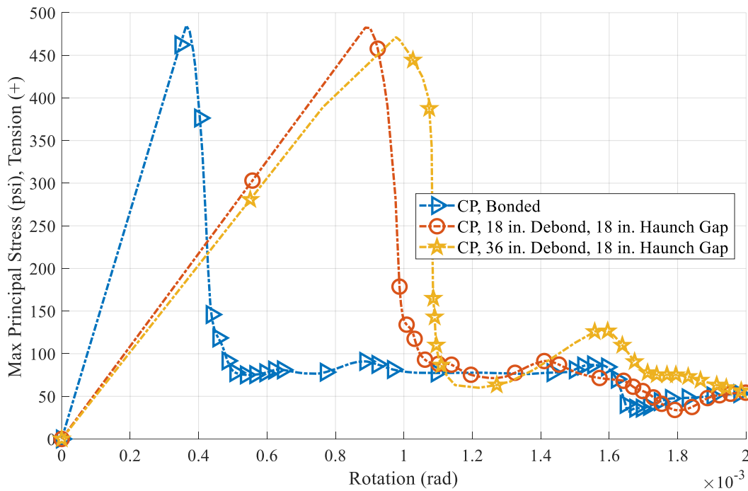
Figure 8.59. Comparison of first cracking behavior for continuous panel models.
