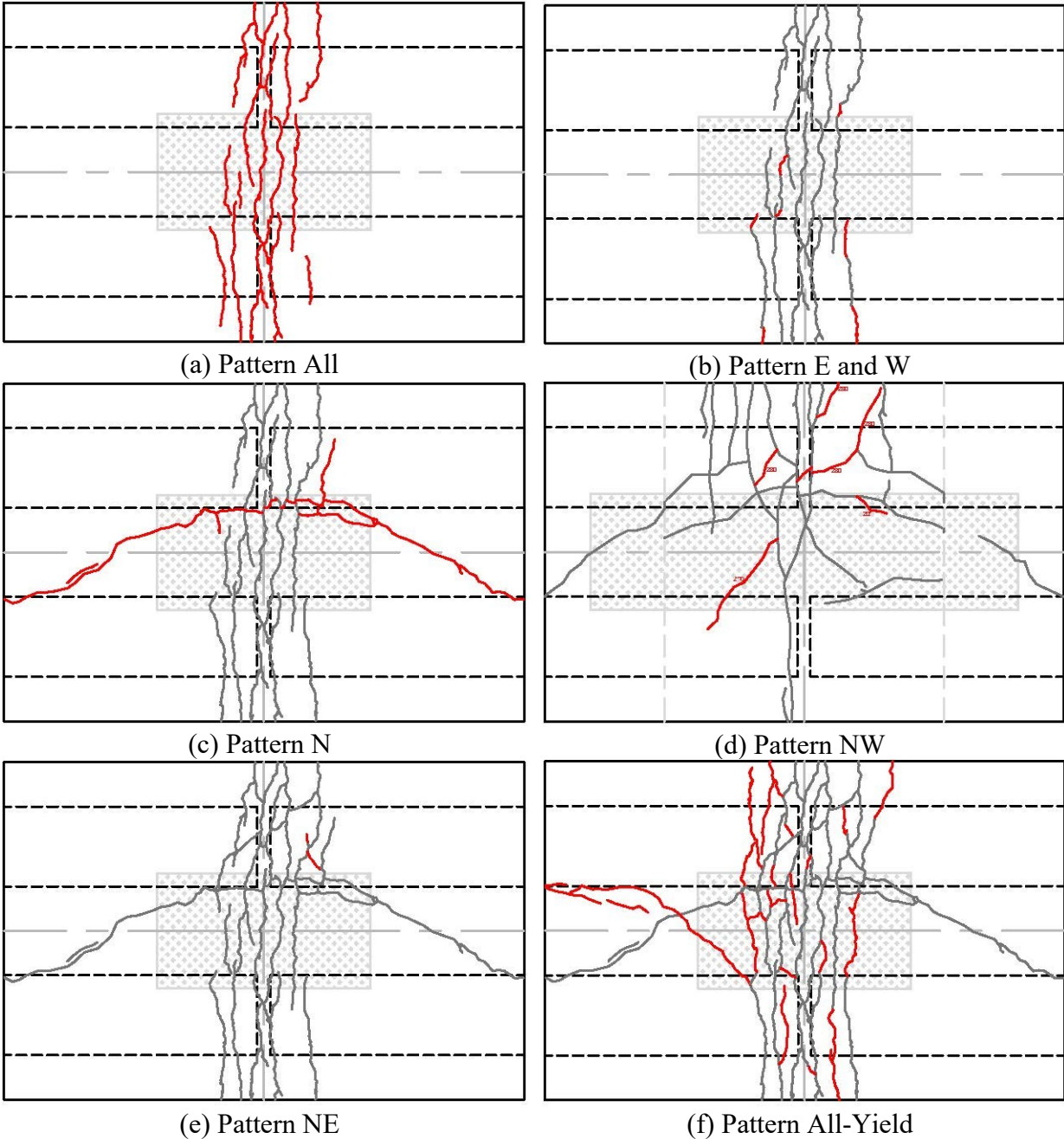
Figure 9.58. PBJ-CP1: Cracks for all load patterns.
