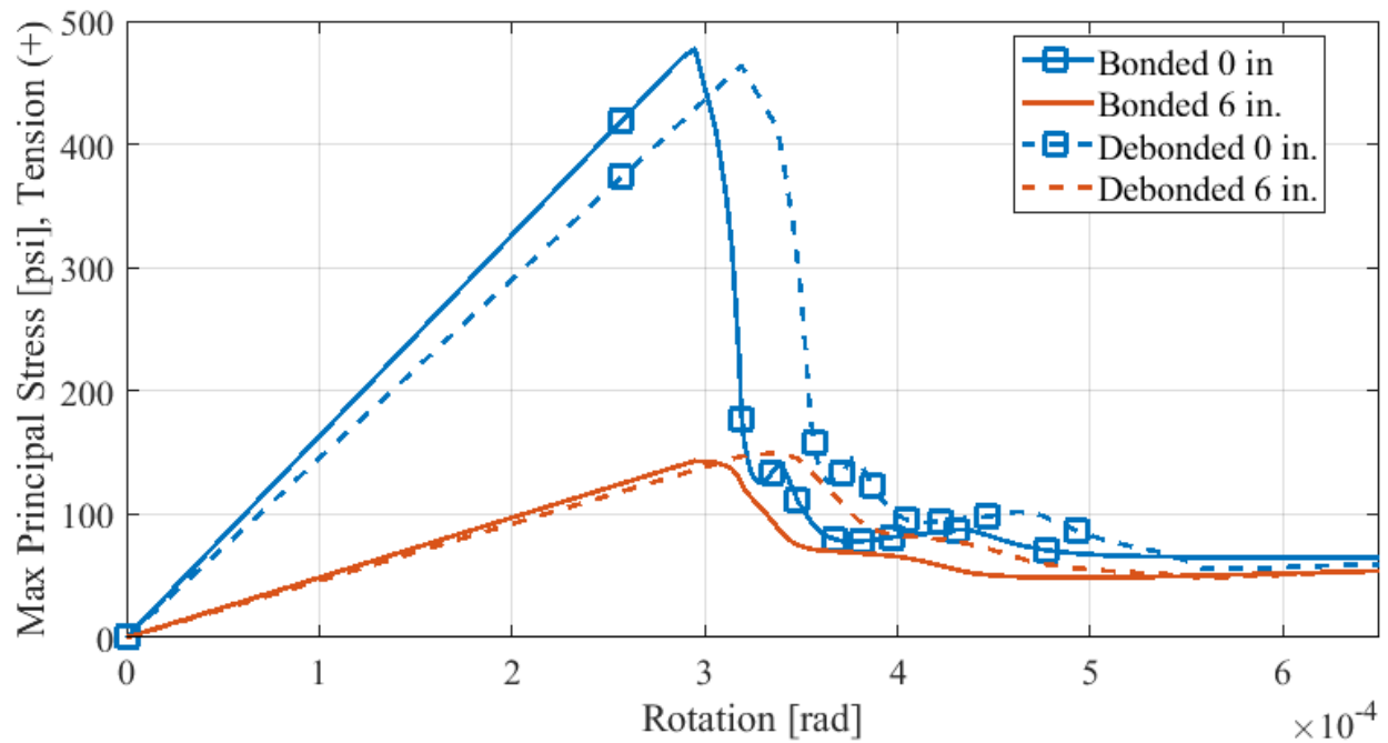
Figure 8.33. Bonded and 54-in. debonded flush precast panel model concrete stresses at the center of the PBJ (0 in.) and at 6 in. away longitudinally from the PBJ.
