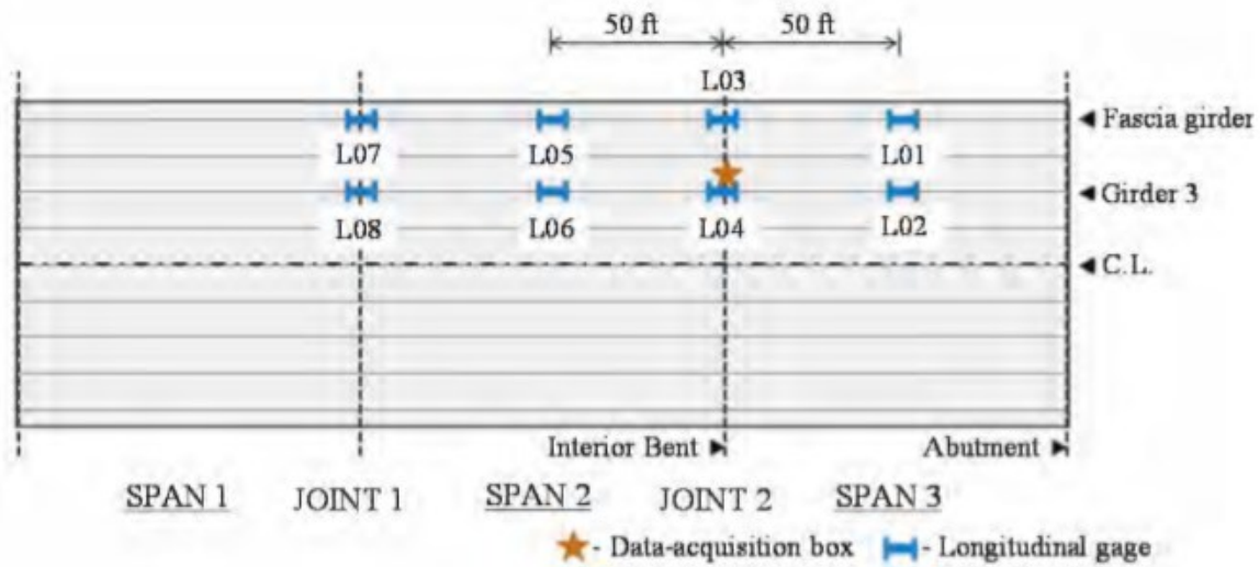
Figure 2.23. Longitudinal bar VW gage layout for the Wharton-Weems Overpass, reprinted from Bayrak et al. (2013).
