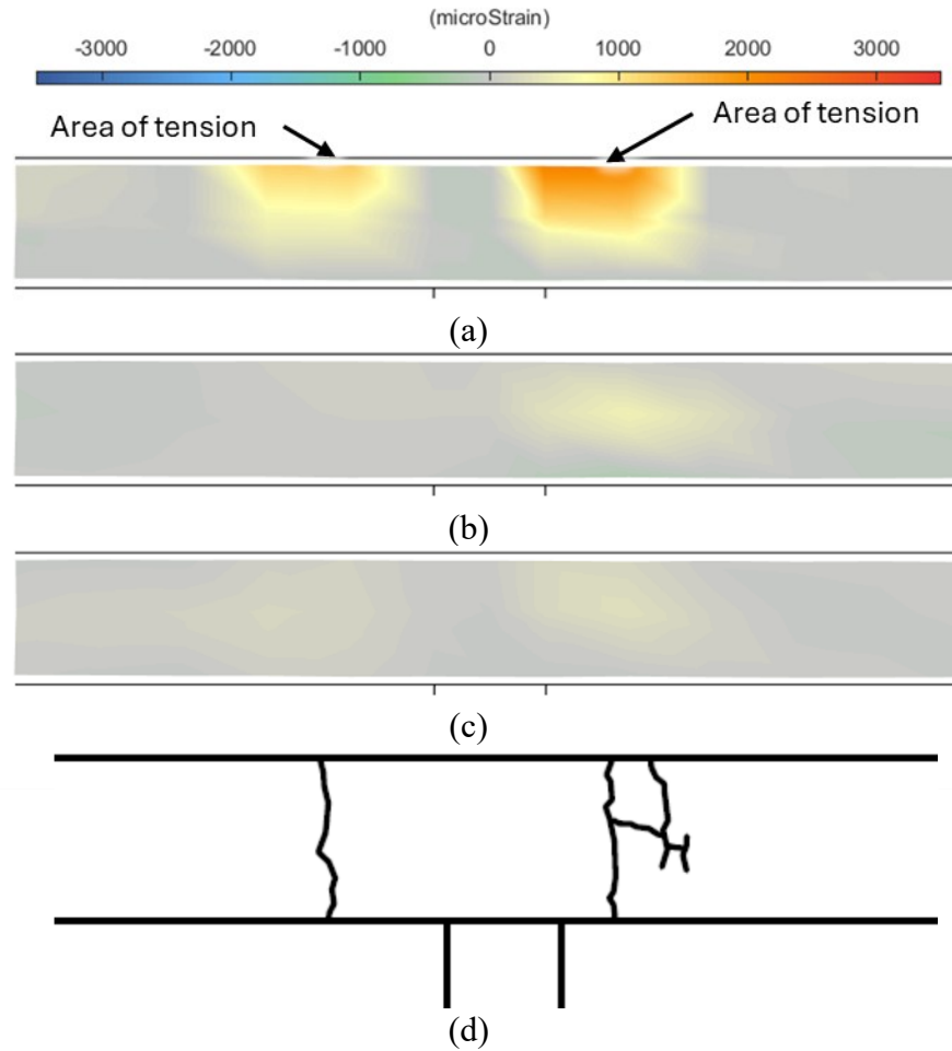
Figure 10.24. Optotrak strains for PBJ-OP1 Pattern All: (a) horizontal, (b) vertical, (c) shear strain, and (d) crack pattern.
