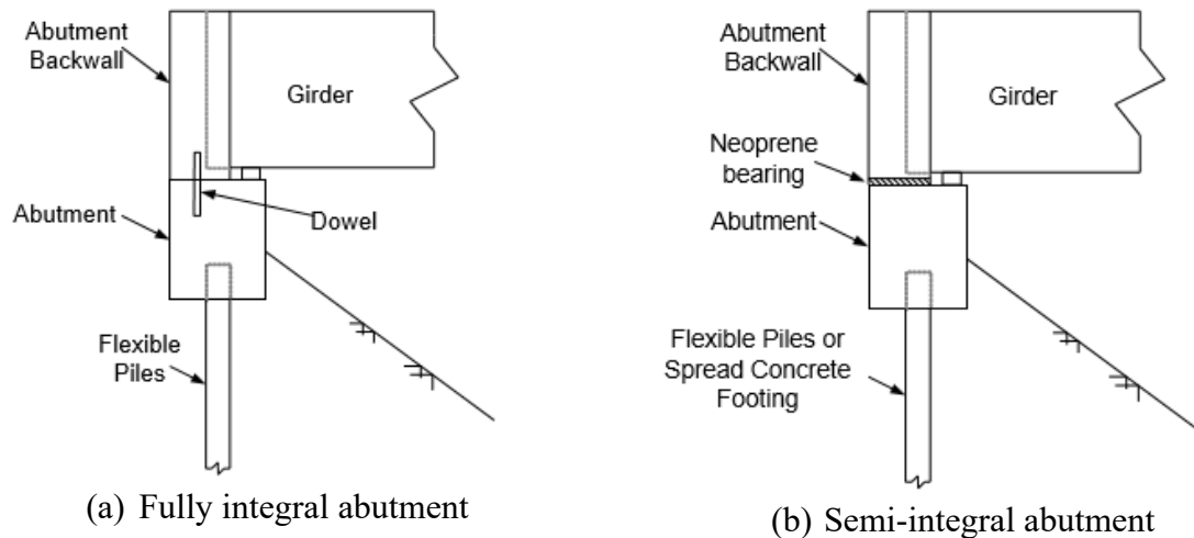
Figure 2.76. Abutment types in integral bridges, reprinted from Stringer and Burgueño (2012).
