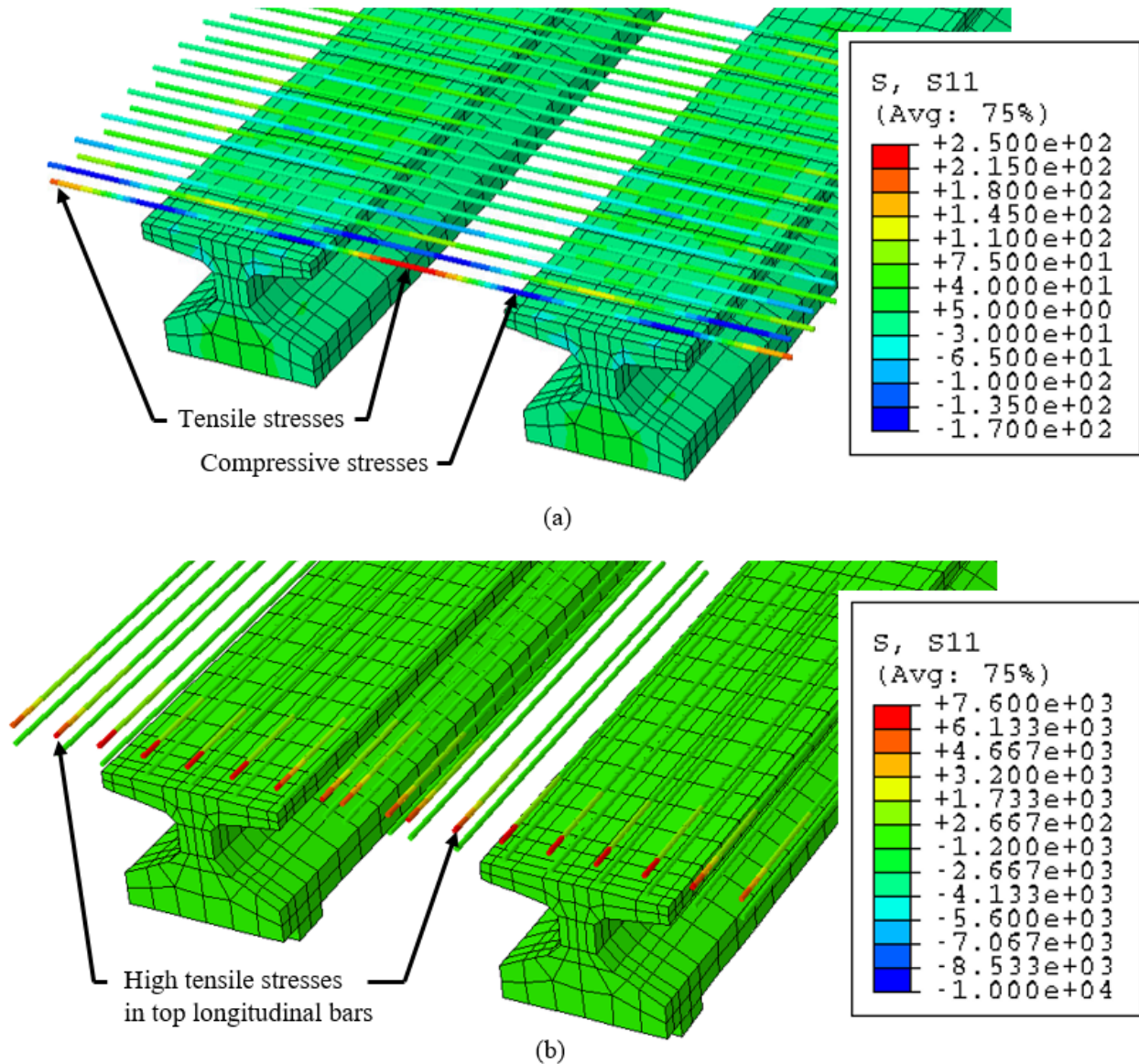
Figure 8.24. Longitudinal stresses (psi) in the reinforcement when the deck is cracked across the width of the section for (a) transverse bars and (b) longitudinal bars.
