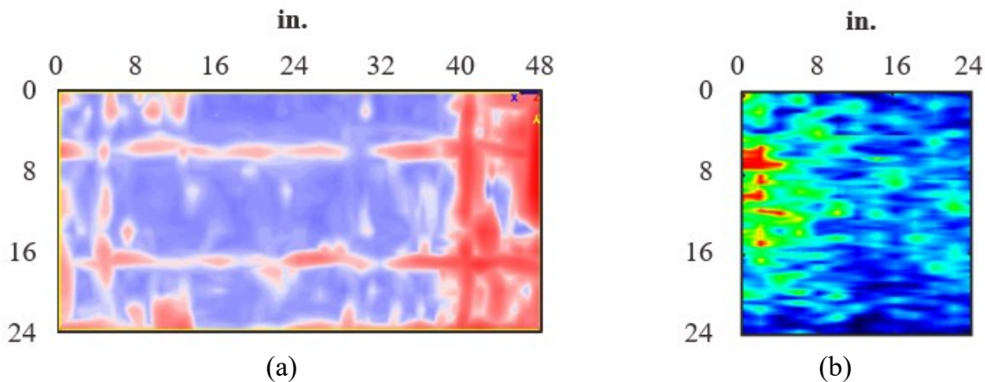
Figure 4.64. LUB4 results for the secondary NDE area for (a) GPR and (b) UST of the bottom reinforcement in the overhang at depth 5.98 in.
