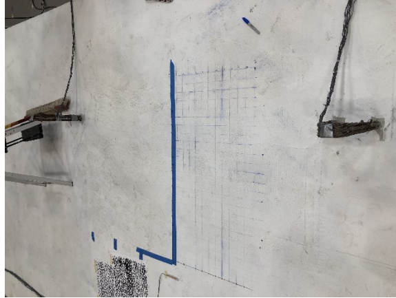
Figure 9.44. Locations of NDE grids.
