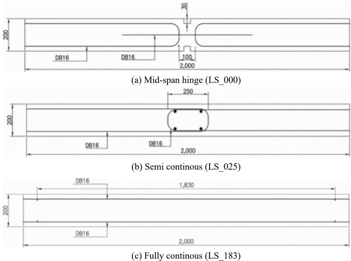
Figure 2.39. Tested reinforcement details, reprinted from Charuchaimontri et al. (2008).
