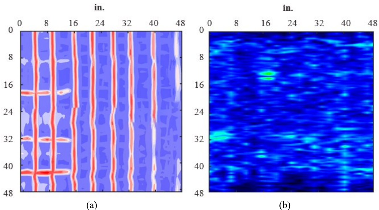
Figure 4.6. ATL1 results for (a) GPR and (b) UST of top longitudinal reinforcement at depth 1.48 in.
