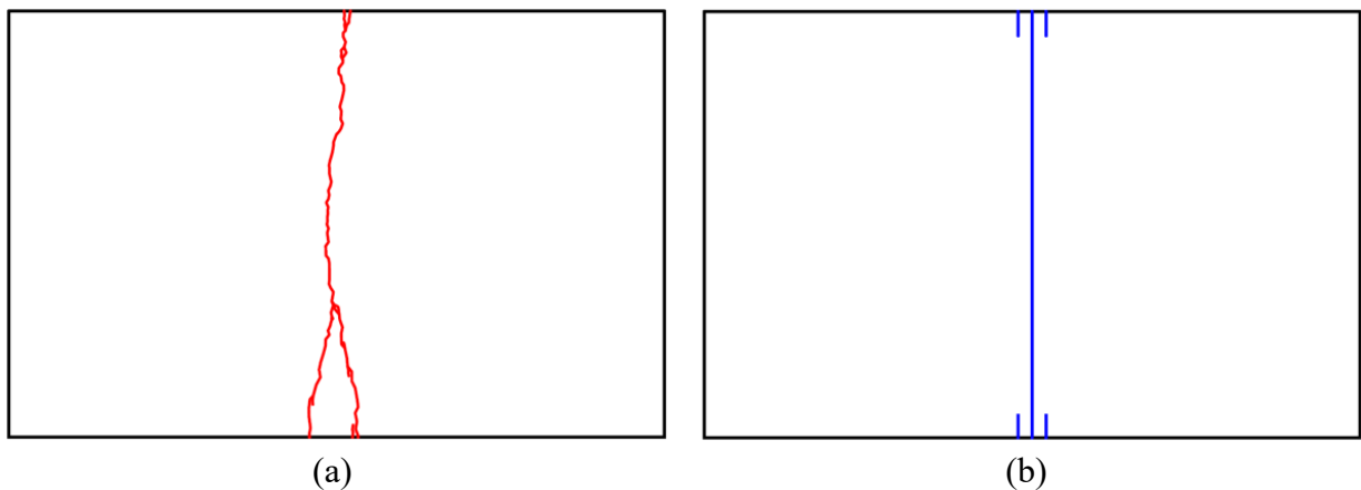
Figure 8.94. Crack patterns of model OP1 for (a) the experimental test and (b) the FEM.
