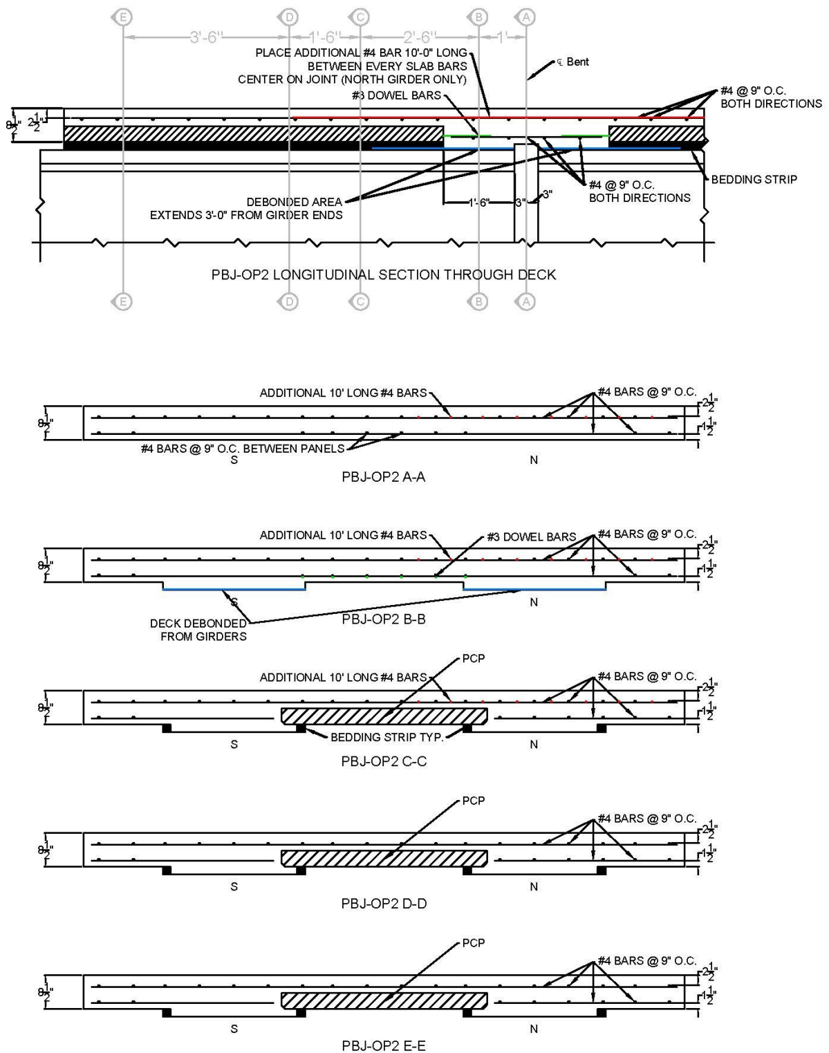
Figure B.5. PBJ-OP2: construction drawings.
