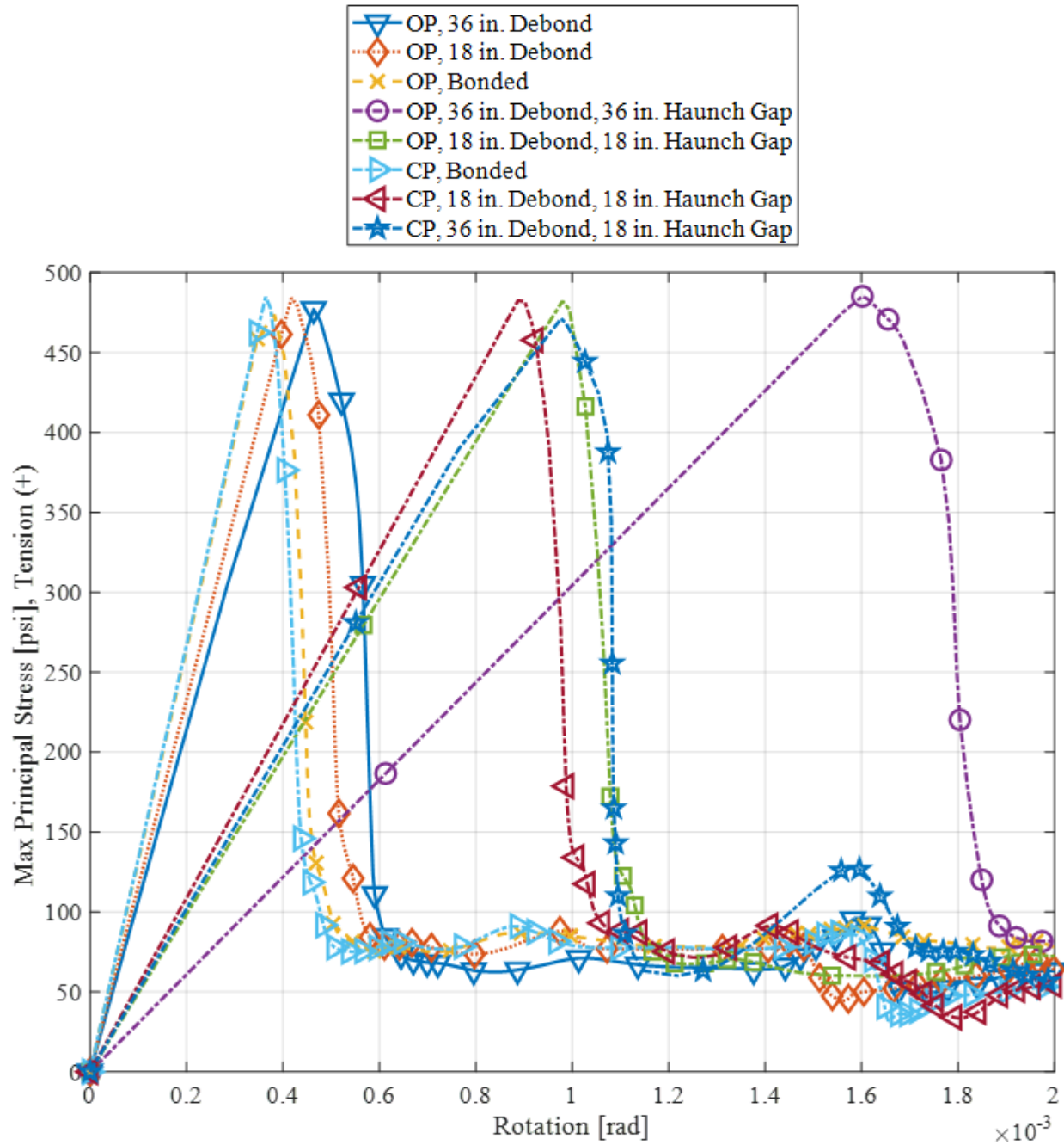
Figure 8.87. Comparison of cracking behavior between offset and continuous panel models, bonded and debonded, with differing haunch gap details.
