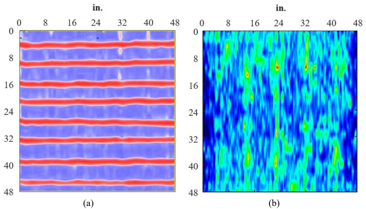
Figure 4.21. ATL3 results for (a) GPR and (b) UST of top transverse reinforcement at depth 1.98 in.
