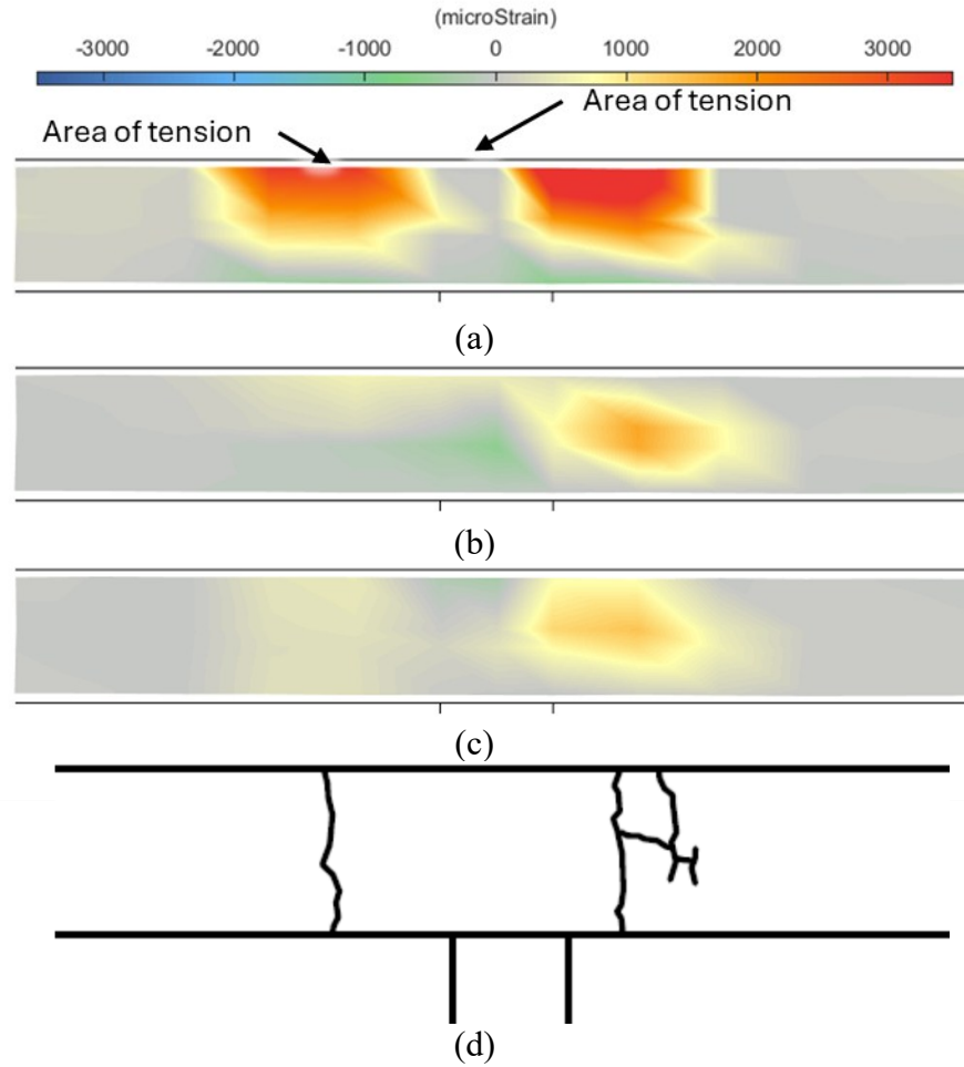
Figure 10.28. Optotrak strains for PBJ-OP1 Pattern All-Yield: (a) horizontal, (b) vertical, (c) shear strain, and (d) crack pattern.
