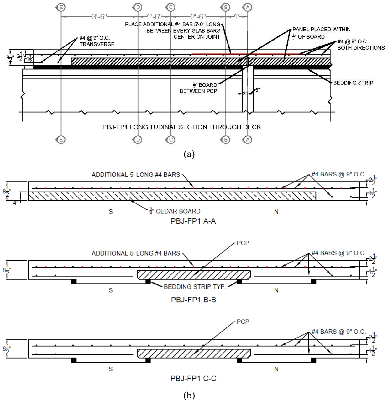
Figure 9.7. PBJ-FP1 geometry and reinforcement: (a) elevation view and (b) select cross-sections.
