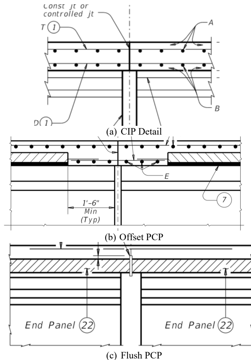
Figure 1.1. TxDOT poor boy joint continuous deck details (TxDOT bridge standards).
