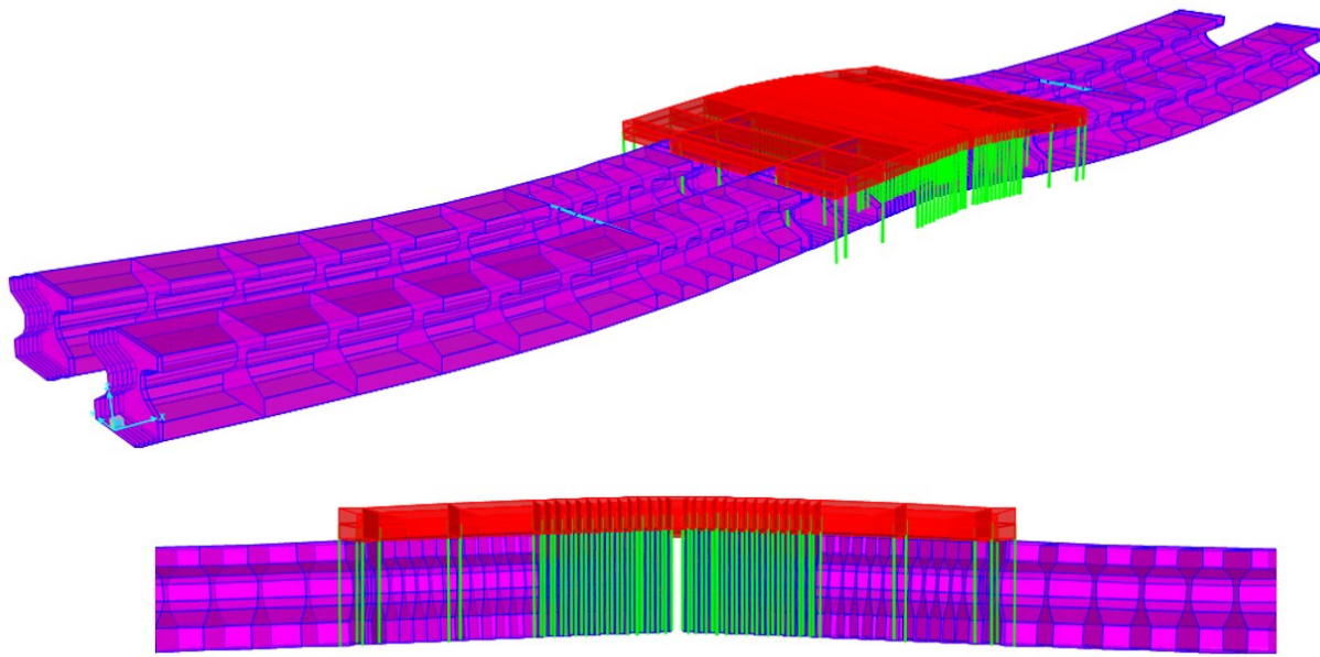
Figure 8.100. Deformed shape of the dual-girder and shell model used to investigate torsional effects.
