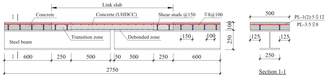
Figure 2.73. UHDC link slab design, reprinted from Hou et al. (2018).
