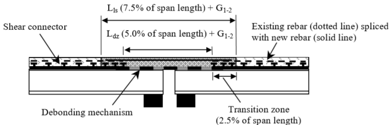
Figure 2.66. Debonded ECC link slab diagram.
