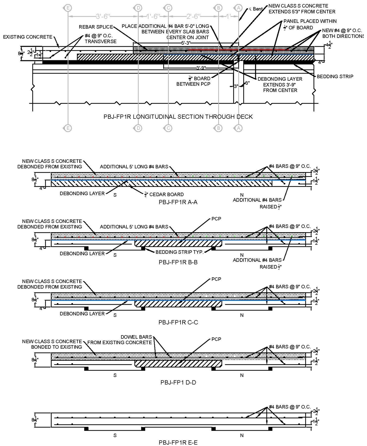
Figure B.2. PBJ-FP1R: construction drawings.
