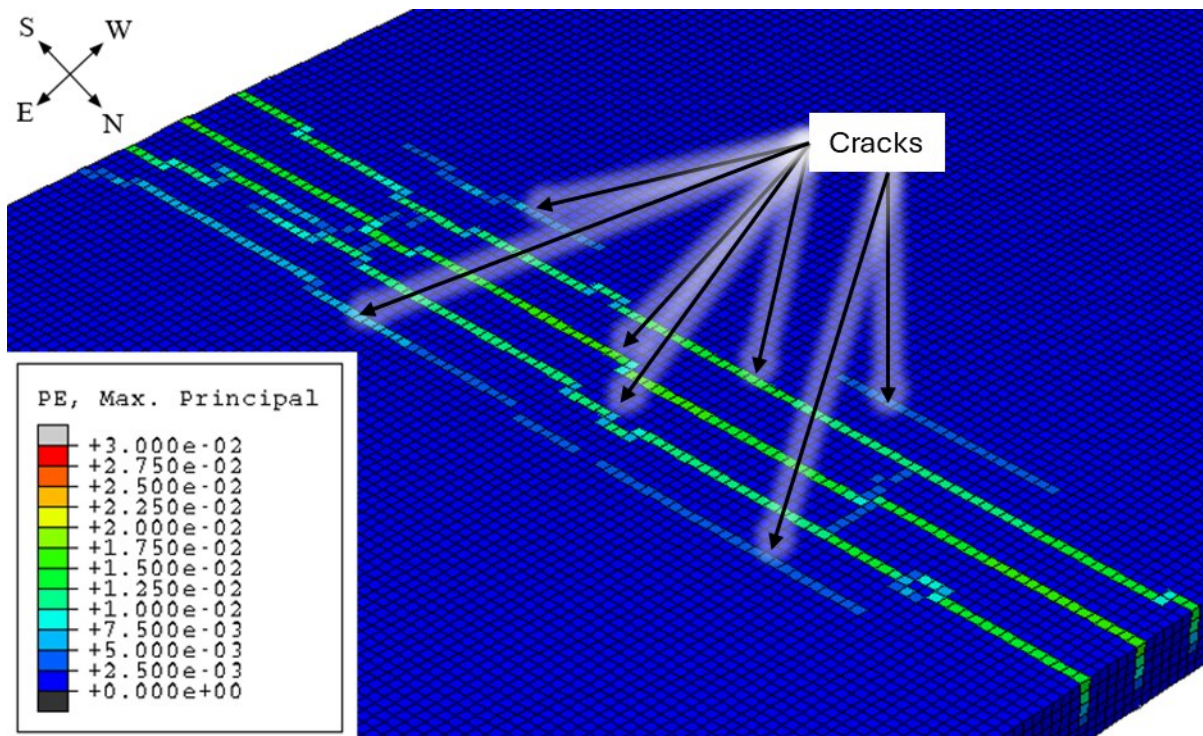
Figure 8.53. Offset precast panel model with longitudinal reinforcement added over the north girder to provide 2.25-in. spacing and over the south girder to provide 3-in. spacing.
