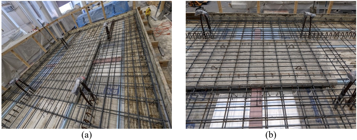
Figure 9.33. PBJ-CP1 prior to concrete pour: (a) overall view and (b) close-up of link slab region.
