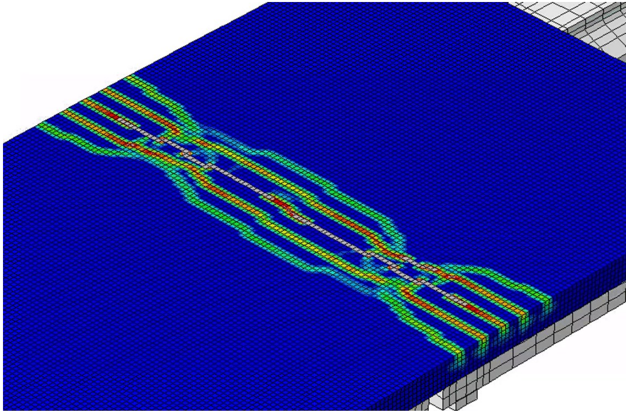
Figure 8.42. Cracking pattern for a bonded offset precast panel model, without a transverse notch in the bottom of the deck and with double the amount of top longitudinal reinforcement at the PBJ.
