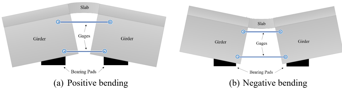
Figure 5.5. Sign convention for rotations.
