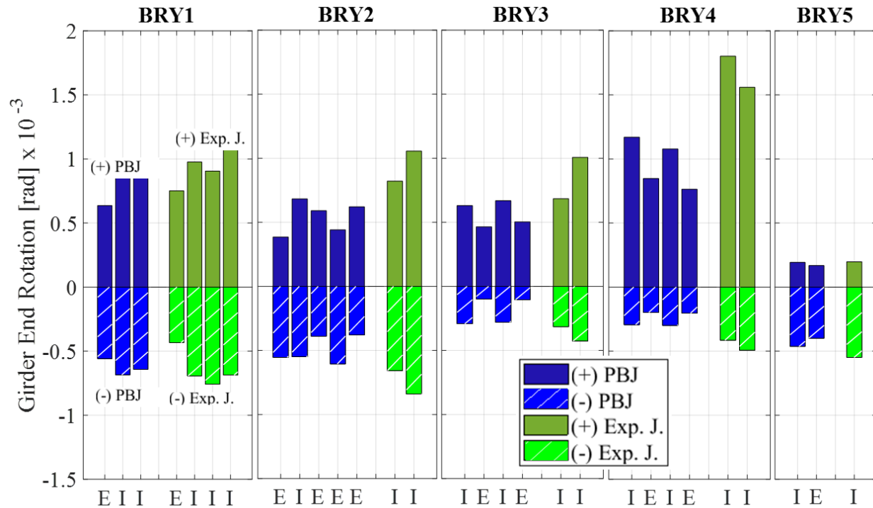
Figure 5.22. Maximum positive and negative thermal rotations.
