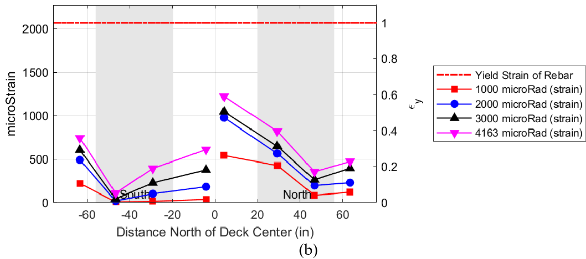
Figure 10.12. PBJ-FP1R: Pattern All comparison of (a) crack width profiles and (b) strain width profiles.
