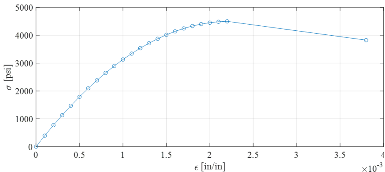
Figure 8.12. Hognestad concrete model for ultimate compressive strength of 4500 psi.
