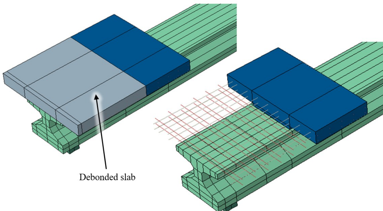
Figure 8.8. Full-depth debonded model.
