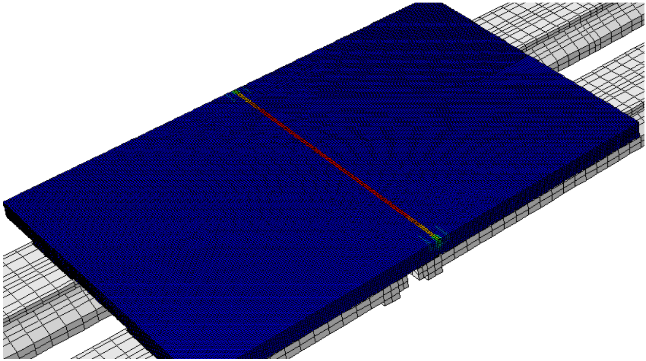
Figure 8.41. Cracking pattern for single-girder offset panel model, mirrored to show four girder lines and secondary cracking in the overhangs.
