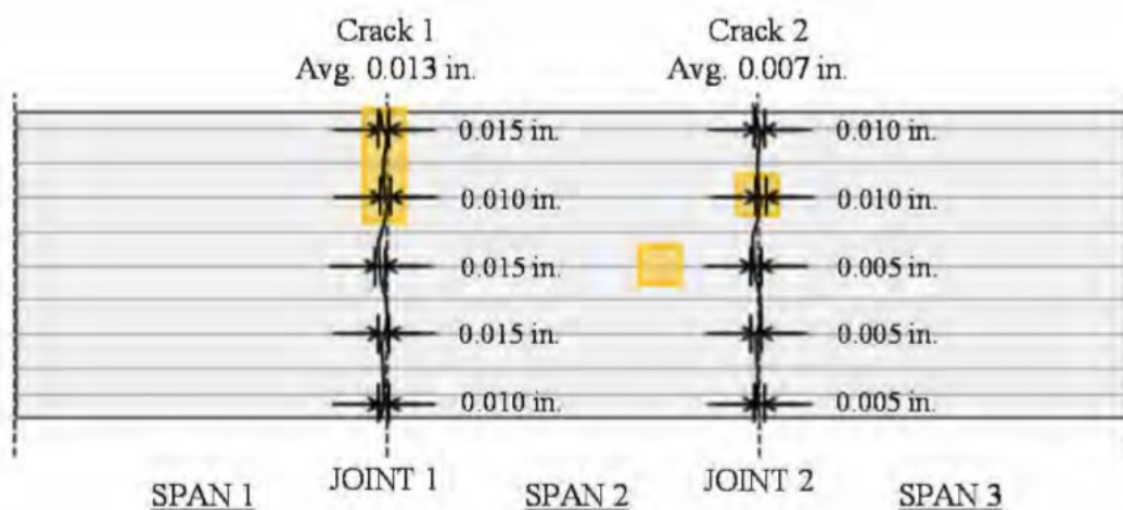
Figure 2.25. Crack widths found in the first inspection of the Wharton-Weems Overpass, reprinted from Bayrak et al. (2013).
