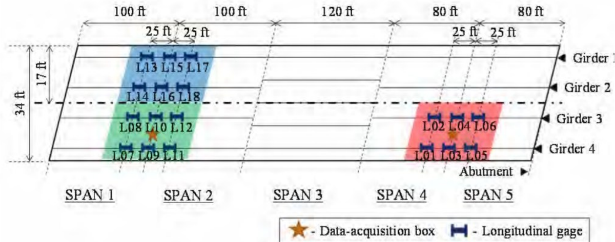
Figure 2.29. Longitudinal bar VW gage layout for the Lampasas River Bridge, reprinted from Bayrak et al. (2013).
