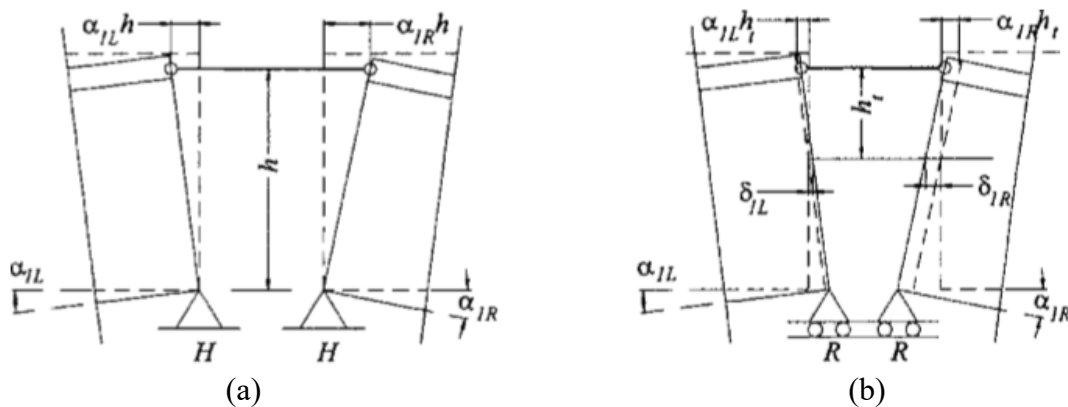
Figure 2.6. Deformation of the link slab system with (a) pin supports and (b) roller supports; reprinted from Okeil and ElSafty (2005).
