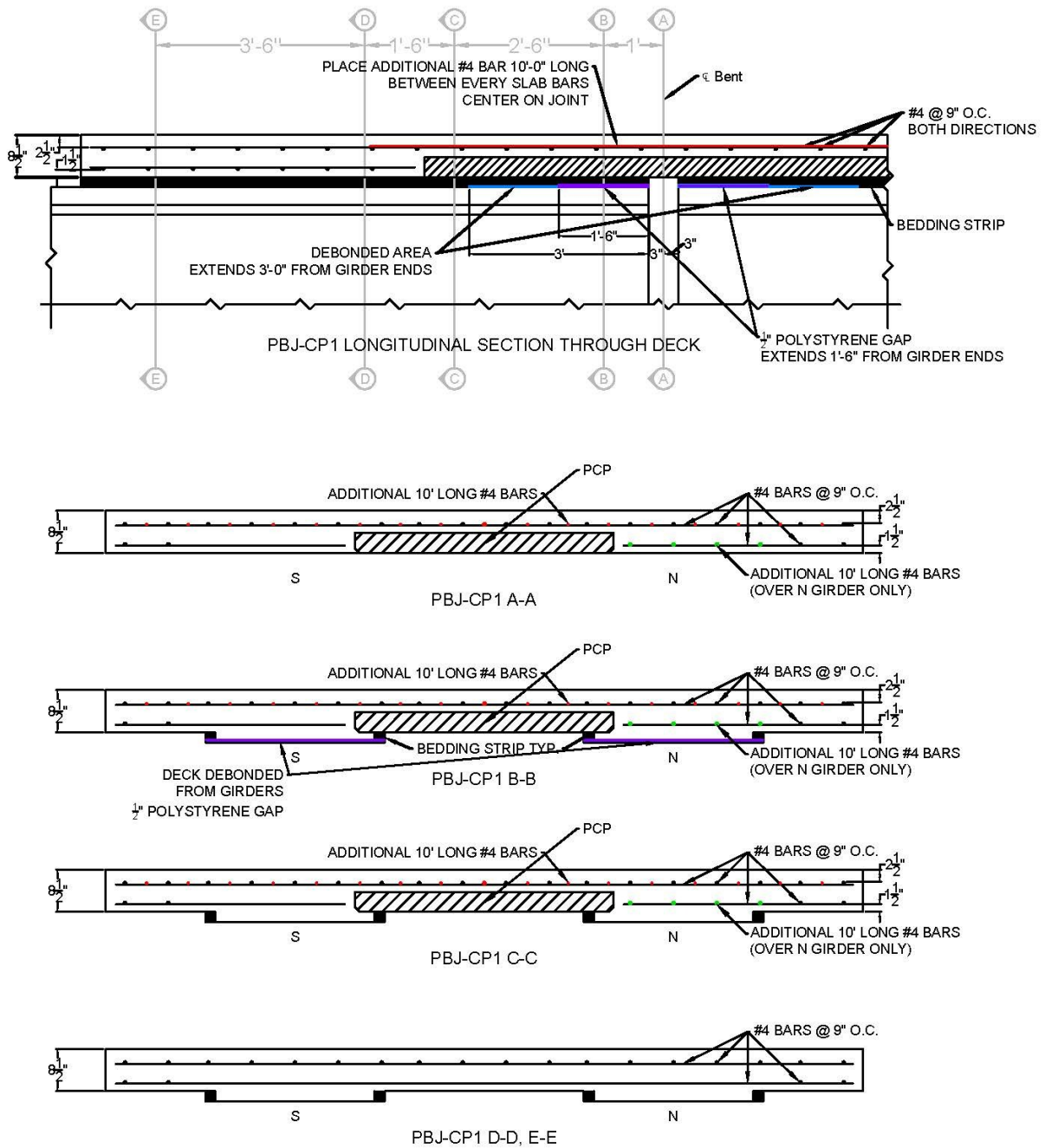
Figure B.6. PBJ-CP1: construction drawings.
