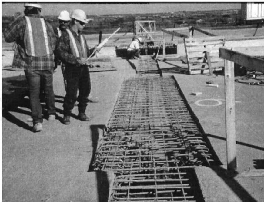
Figure 2.17. Poor boy continuous joint pour, reprinted from Davis et al. (1999).
