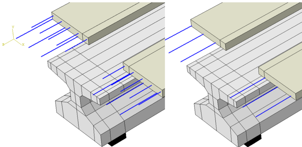
Figure 8.50. Offset panel models with bars protruding from the panels (left) and without bars protruding from the panels (right).
