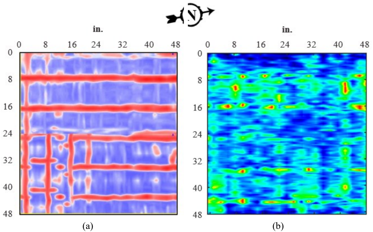
Figure 4.5. ATL1 results for (a) GPR and (b) UST of top longitudinal reinforcement at depth 2.73 in.
