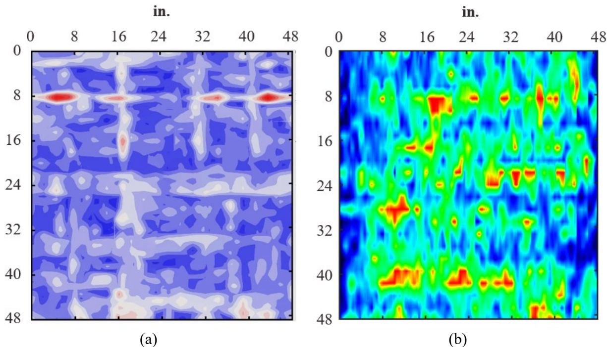
Figure 4.24. ATL3 results for (a) GPR and (b) UST of the PMDF at depth 8.5 in.
