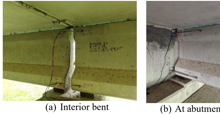
Figure 5.3. Example of gage attachment (shown installed on Bridge BRY3).
