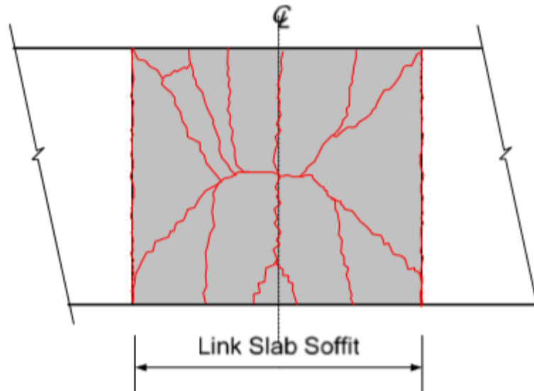
Figure 2.60. Slab crack pattern, reprinted from Au et al. (2013).
