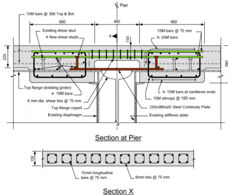
Figure 2.42. HwY 401 Underpass link slab detail, reprinted from Lam et al. (2008).
