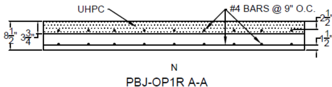
Figure 9.11. PBJ-OP1R cross-section at center of link slab (Section A-A).
