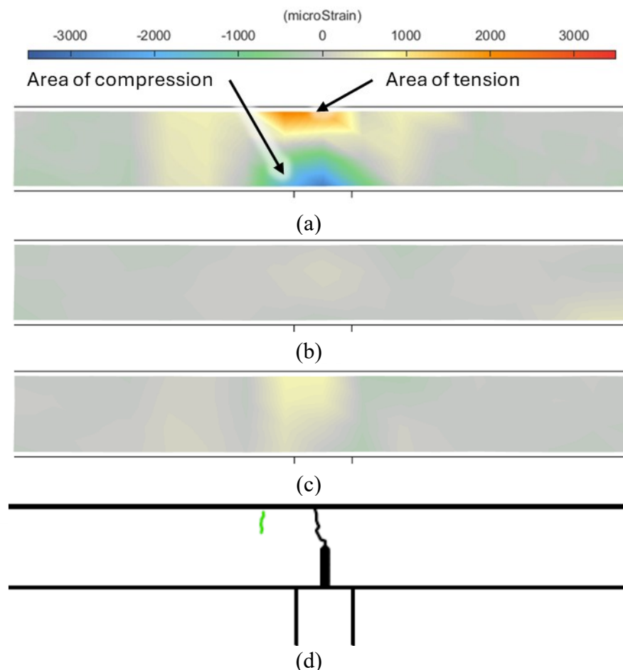
Figure 10.22. Optotrak strains for PBJ-FP1 Pattern All: (a) horizontal, (b) vertical, (c) shear strain, and (d) crack pattern.
