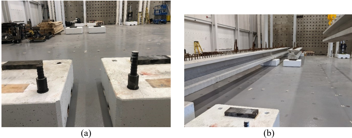
Figure 9.15. Placement of pedestals, bearing pads, and girders (shown for PBJ-FP1).
