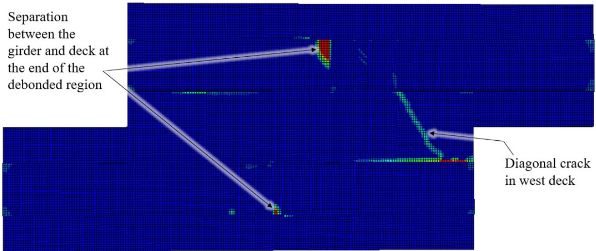
Figure 8.82. Cracking in the bottom of the deck for the debonded dual-girder skewed model, including a full-depth diagonal crack in the west deck, with separation between the girder and deck occurring at the end of the debonded regions.
