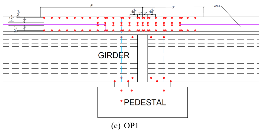
Figure 9.41. Optotrak grid of targets for each test.
