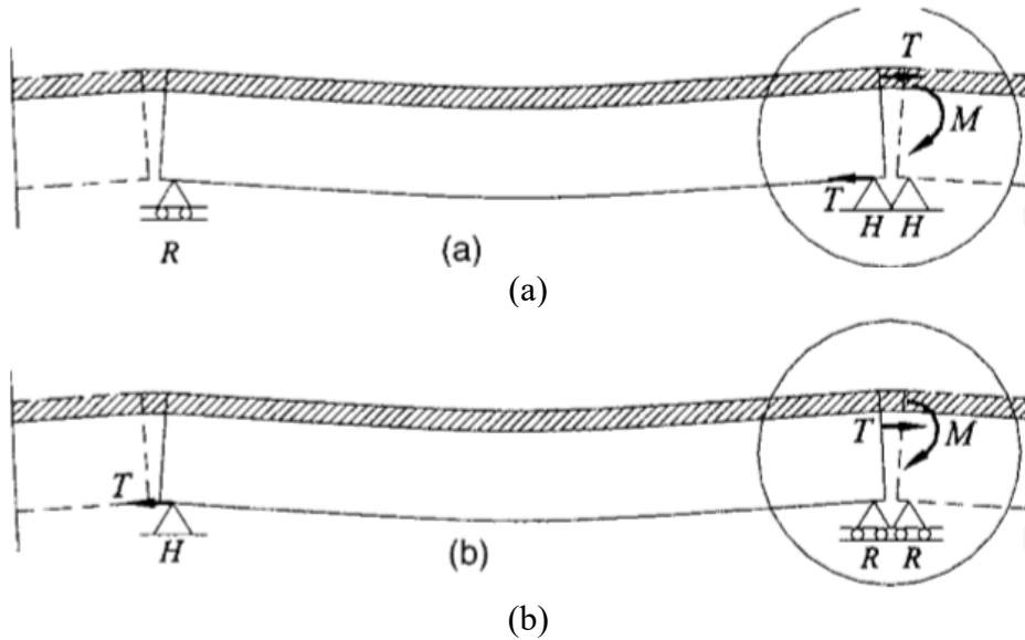
Figure 2.5. (a) Hinge supports causing a couple moment and tension in the link slab, and (b) roller supports preventing the formation of a couple moment, reducing the tension in the link slab; reprinted from Okeil and ElSafty (2005).
