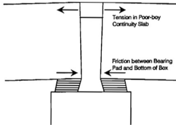
Figure 2.16. Couple moment causing link slab tension, reprinted from Roberts et al. (1993).
