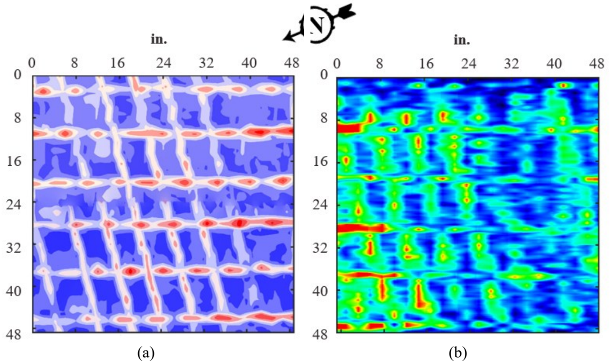
Figure 4.13. ATL2 results for (a) GPR and (b) UST of top longitudinal reinforcement at depth 3.73 in.
