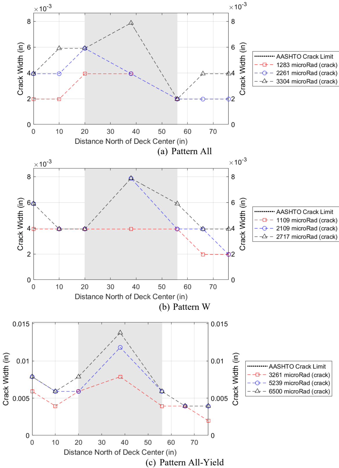
Figure 10.7. PBJ-OP1R: Crack width profiles for select patterns.
