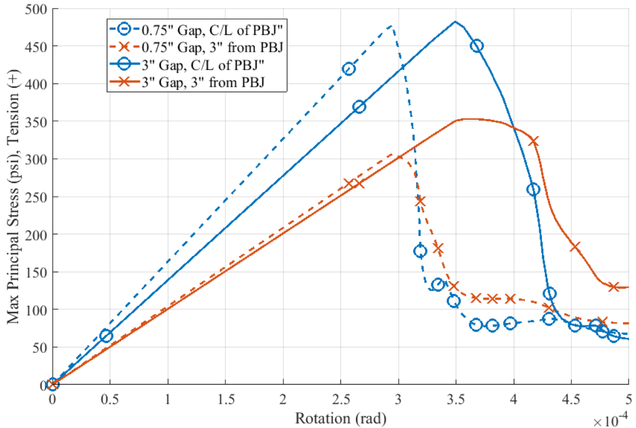
Figure 8.40. Concrete principal stress for flush precast panel models, comparing details of the standard 0.75-in. end gap with a longer 3-in. end gap.
