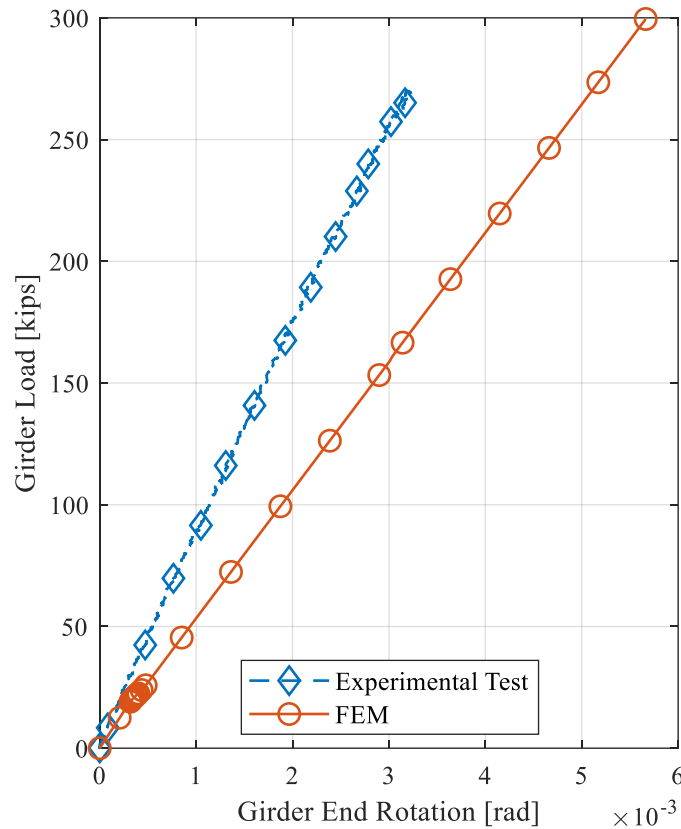
Figure 8.88. FP1 girder end rotation versus girder loading for the experimental test and FEM.
