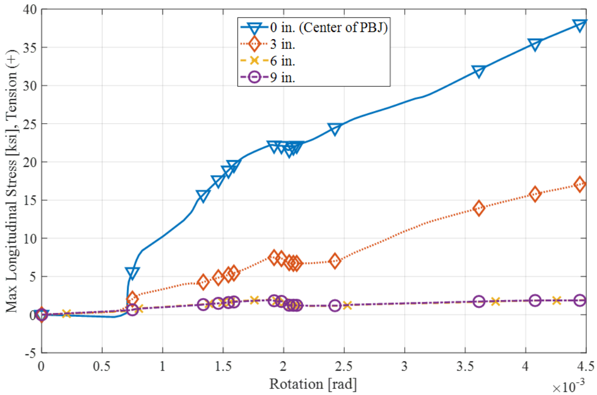
(b) Rebar stress (5 ft supplemental bars)
