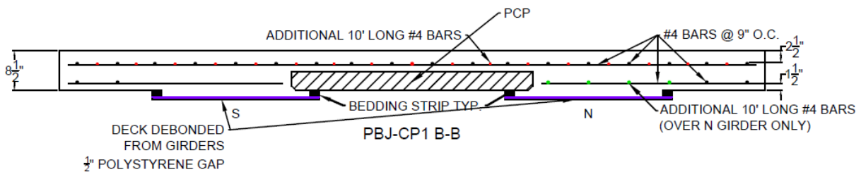
Figure 9.14. PBJ-CP1 details—cross-section (B-B) showing details where gap is present at end of girders.
