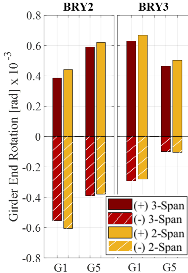
Figure 5.23. Thermal rotations for BRY2 and BRY3, with bars indicating number of continuous spans in a unit (red bars indicate three-span units and yellow bars indicate two-span units).
