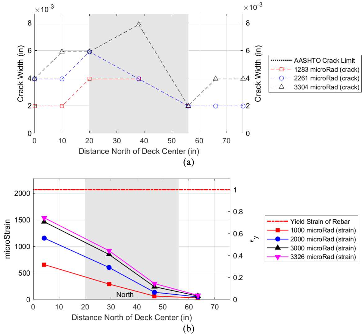
Figure 10.13. PBJ-OP1R: Pattern All comparison of (a) crack width profiles and (b) strain width profiles.
