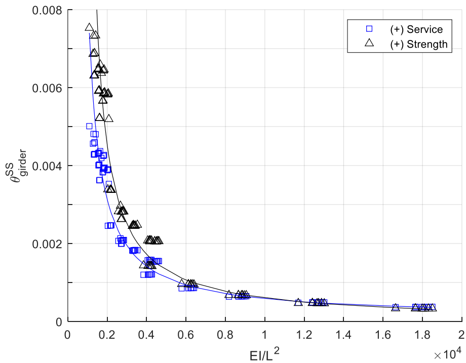
Figure 7.4. Girder end rotations for design of TxDOT standard I-girder bridges (only positive bending shown).
