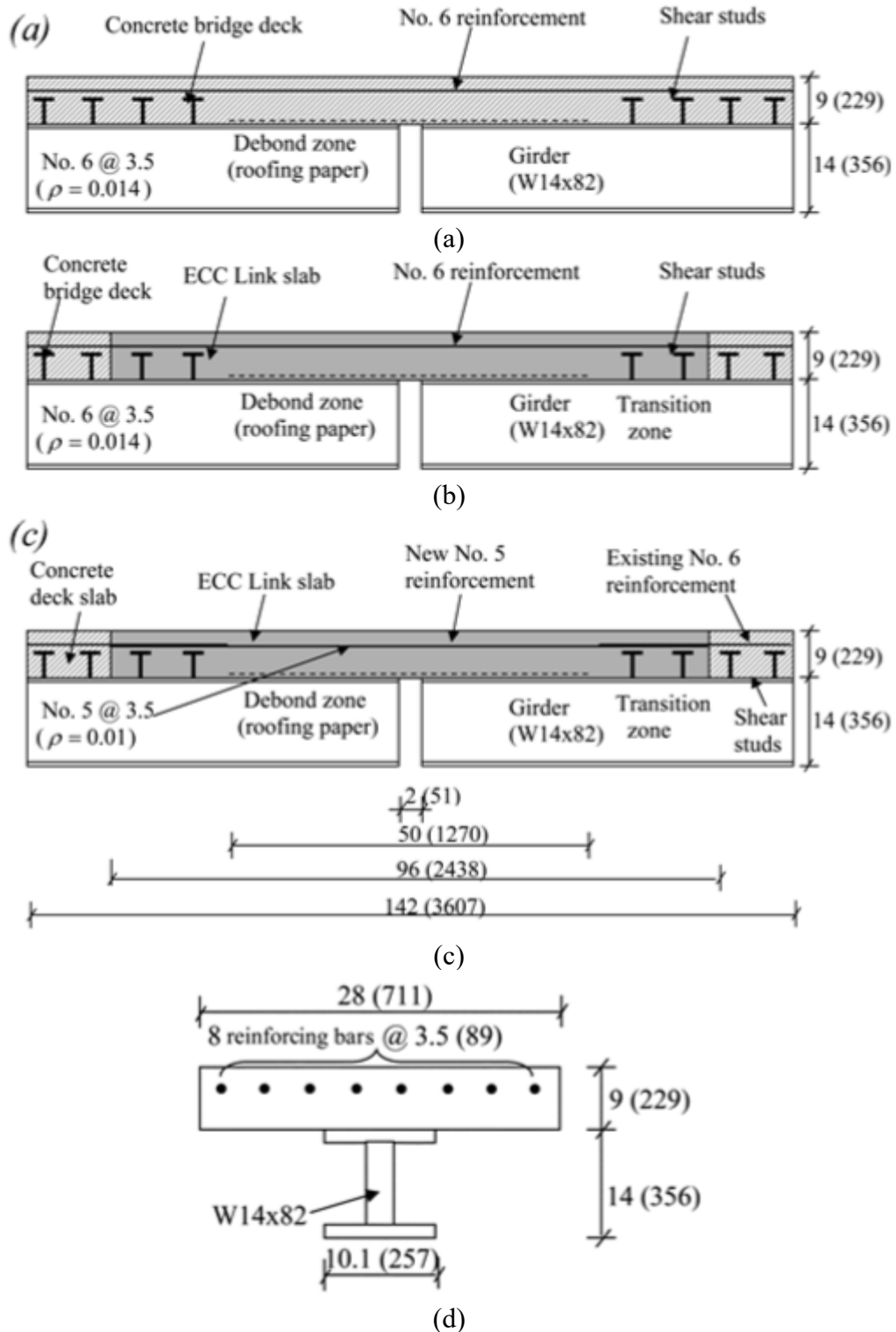
Figure 2.69. The three experimental link slab specimens (a, b, c) and a section view of the specimens (d), reprinted from Qian et al. (2009).
