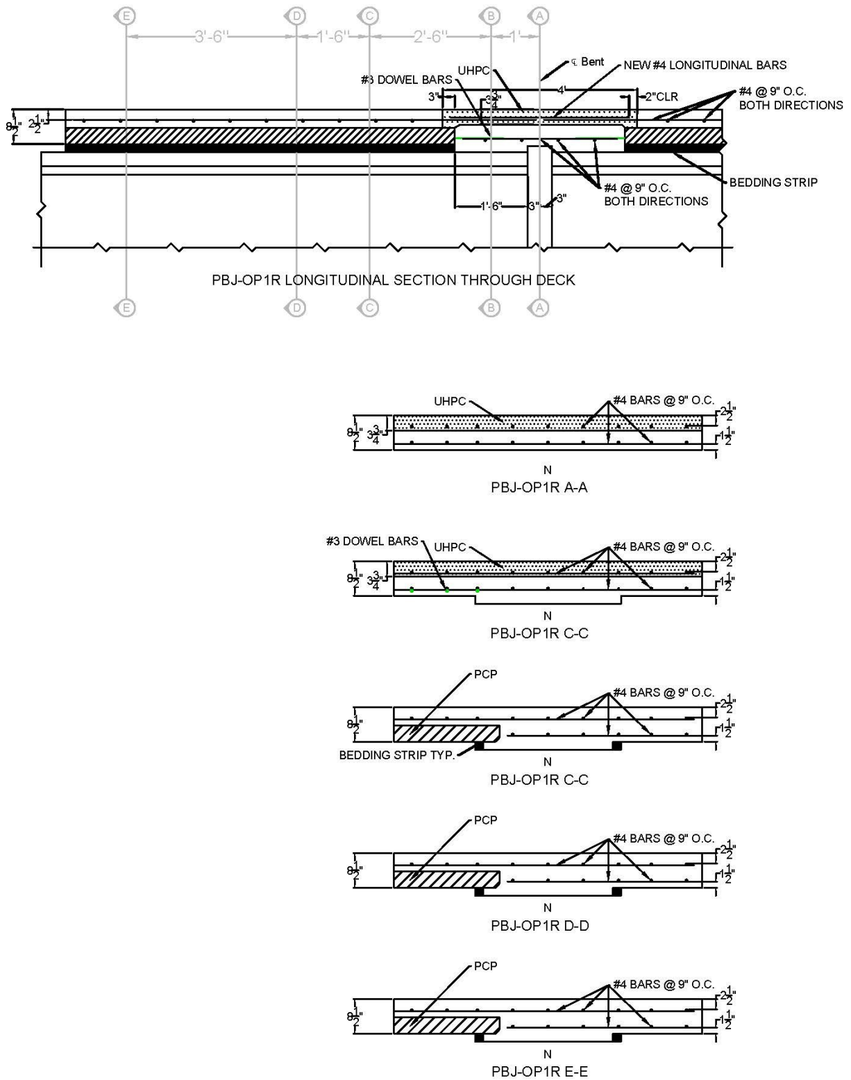
Figure B.4. PBJ-OP1R: construction drawings.
