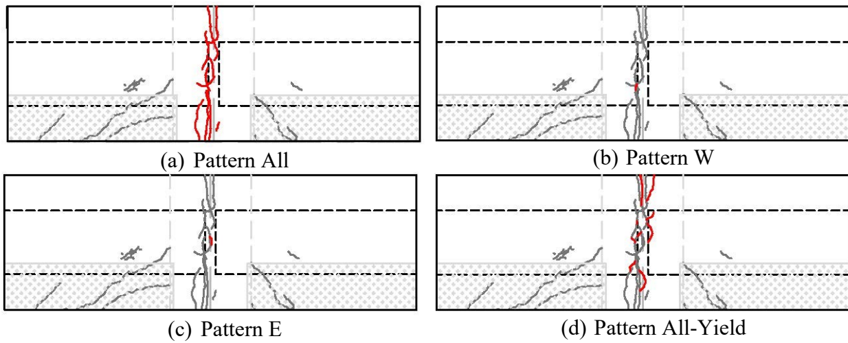
Figure 9.53. PBJ-OP1R: Cracks for all tests, with hatched region not tested (gray cracks are from prior test [PBJ-OP1]).
