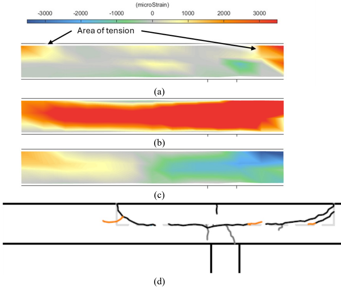
Figure 10.25. Optotrak strains for PBJ-OP1R Pattern All: (a) horizontal, (b) vertical, (c) shear strain, and (d) crack pattern.
