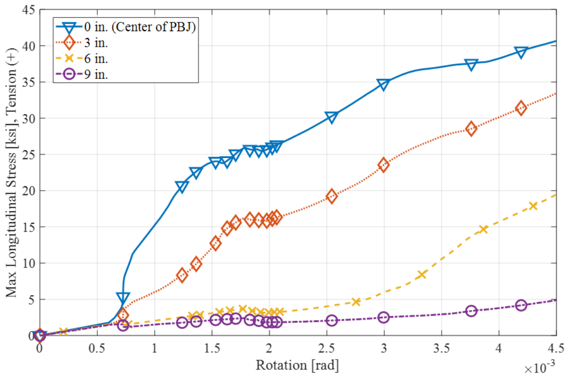
(b) Rebar stress (raised 5-ft supplemental bars)
