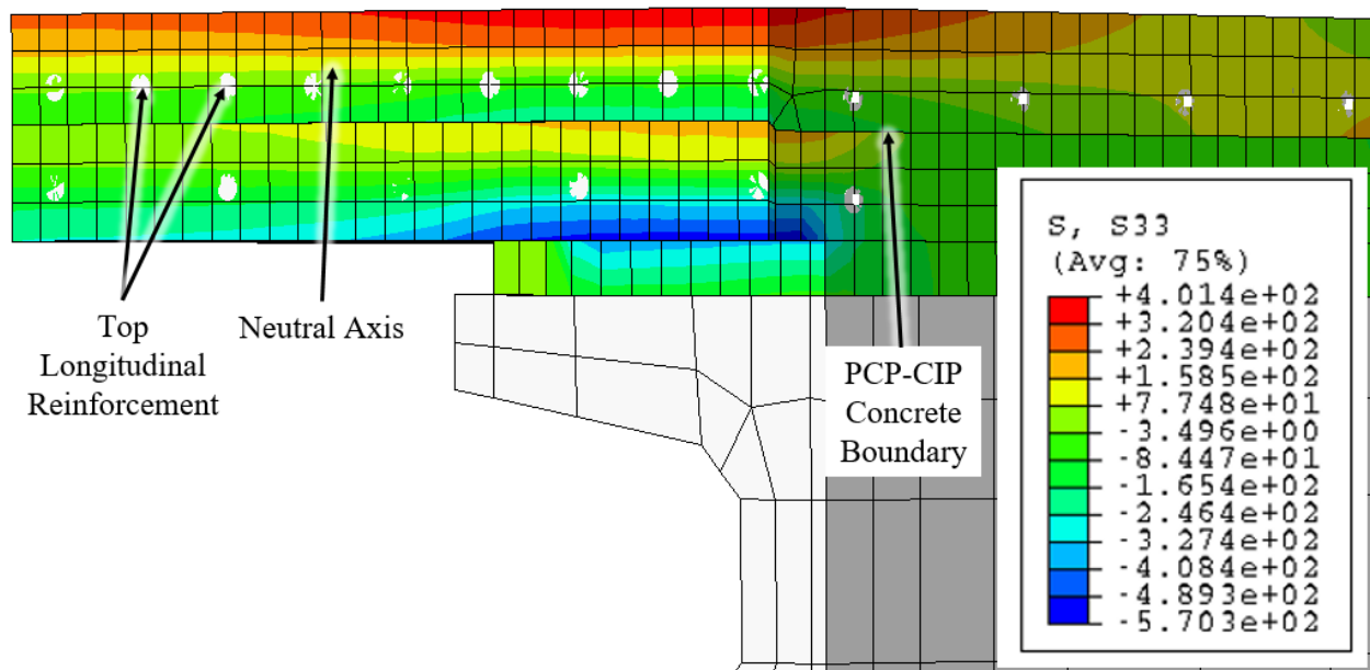
Figure 8.35. Cross-section of the slab for the partial-depth debonded model showing that the top longitudinal steel reinforcement is below the tension zone in the concrete prior to cracking.
