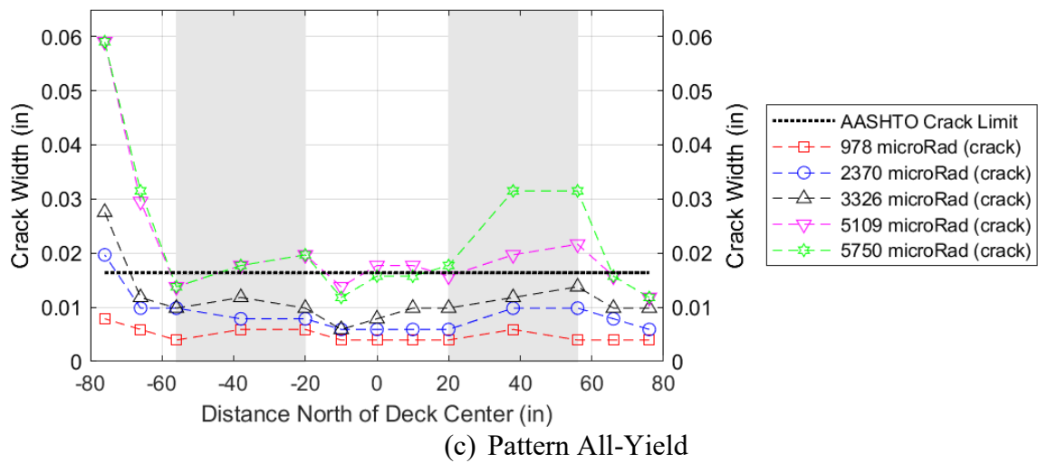
Figure 10.4. PBJ-OP2: Crack width profiles for select patterns.
