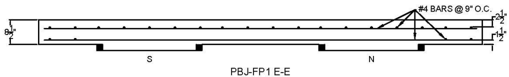
Figure B.1. PBJ-FP1: construction drawings.
