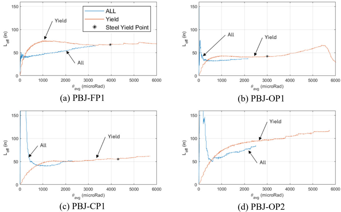
Figure 10.32. Effective link slab lengths calculated with Method 2 for Pattern All and Pattern All-Yield.
