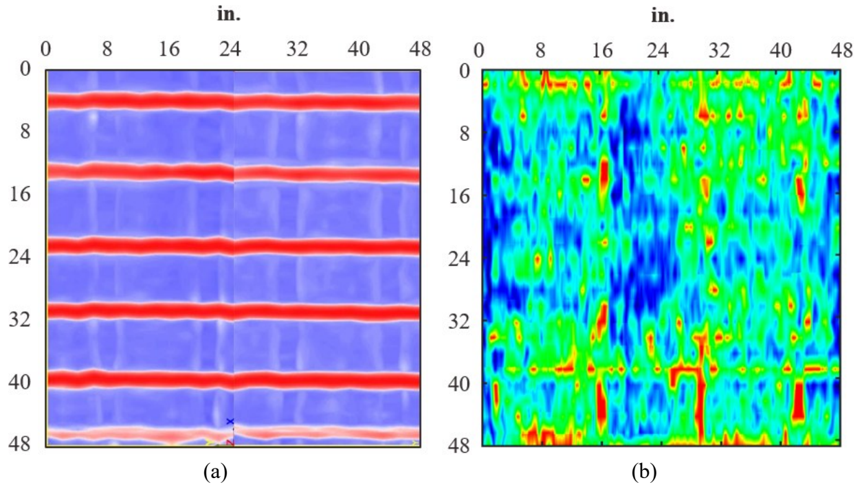
Figure 4.29. ATL4 results for (a) GPR and (b) UST of top transverse reinforcement between the girders at depth 3.95 in.
