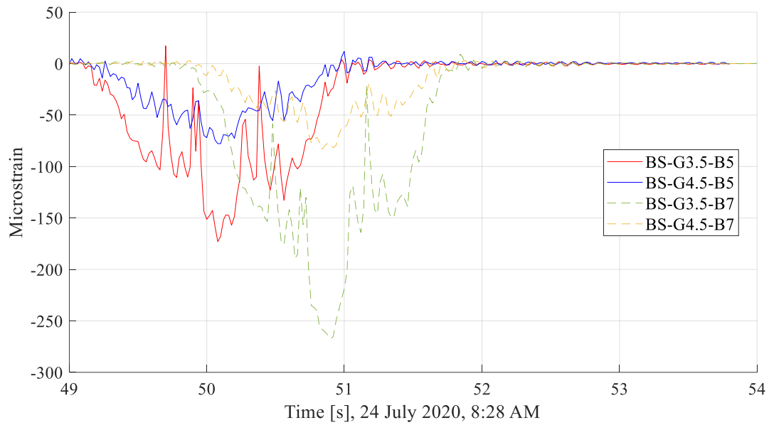
Figure 5.25. Strain data for sample live load event for truck on BRY3 above G3.
