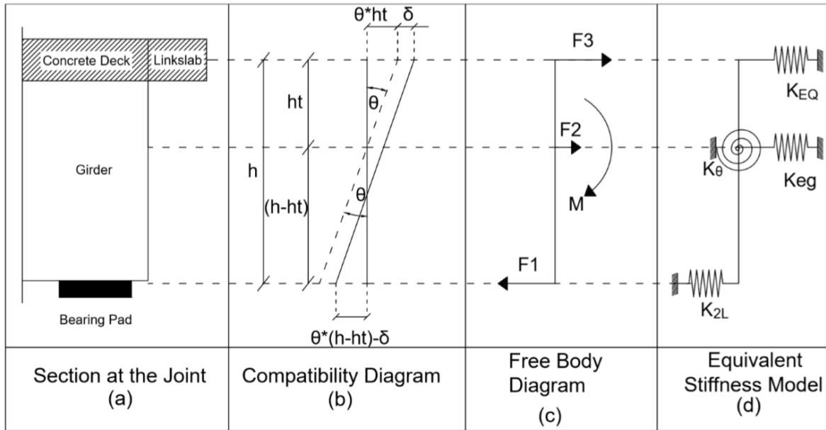
Figure 2.8. Parameter calculation for equivalent stiffness model, reprinted from Canales and Okeil (2019).
