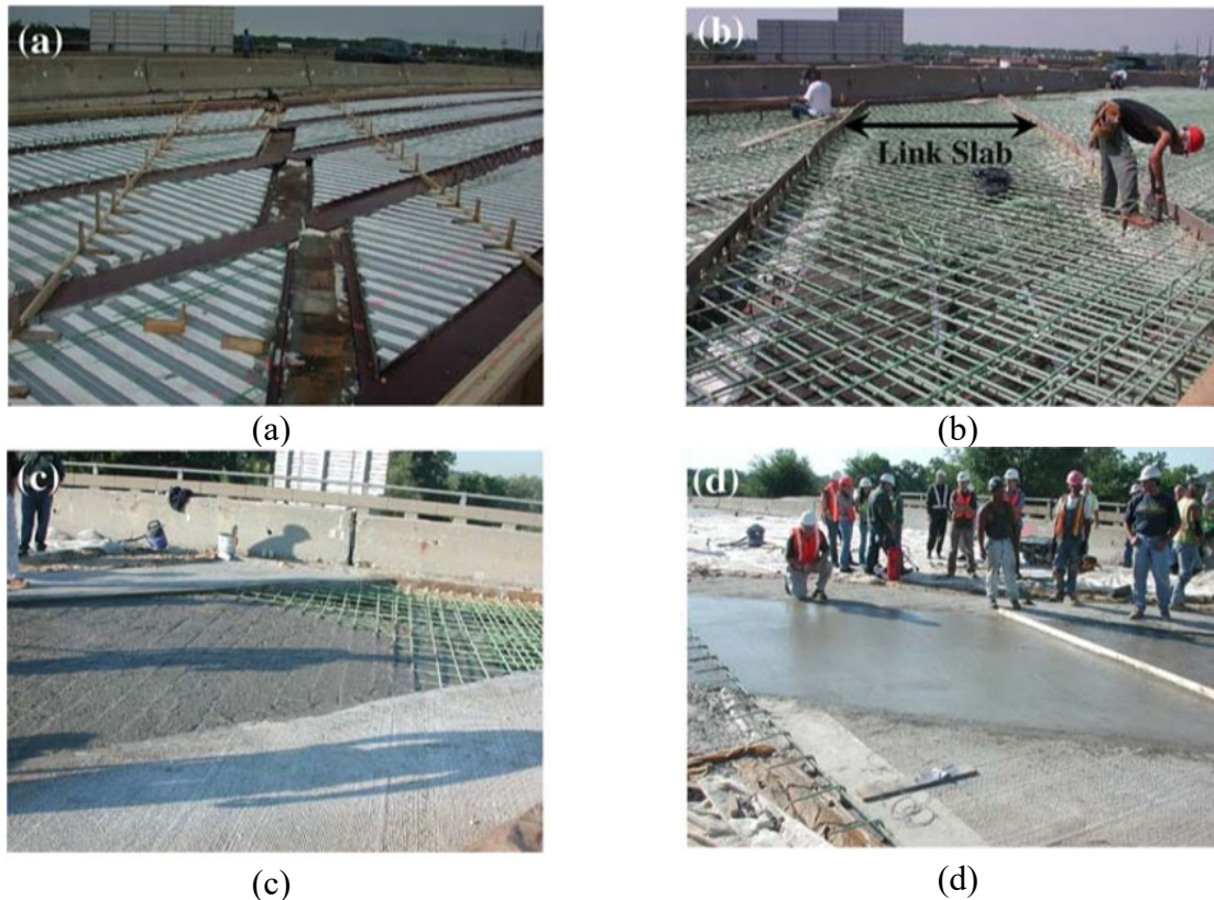
Figure 2.67. Construction of the ECC link slab, showing the (a) girder ends beneath, (b) placement of reinforcement, (c) ECC pour, and (d) ECC finishing; reprinted from Lepech and Li (2009).
