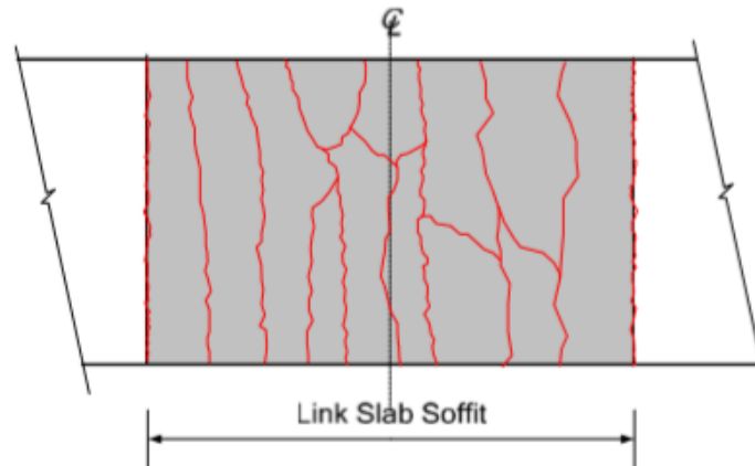
Figure 2.59. Slab crack pattern, reprinted from Au et al. (2013).
