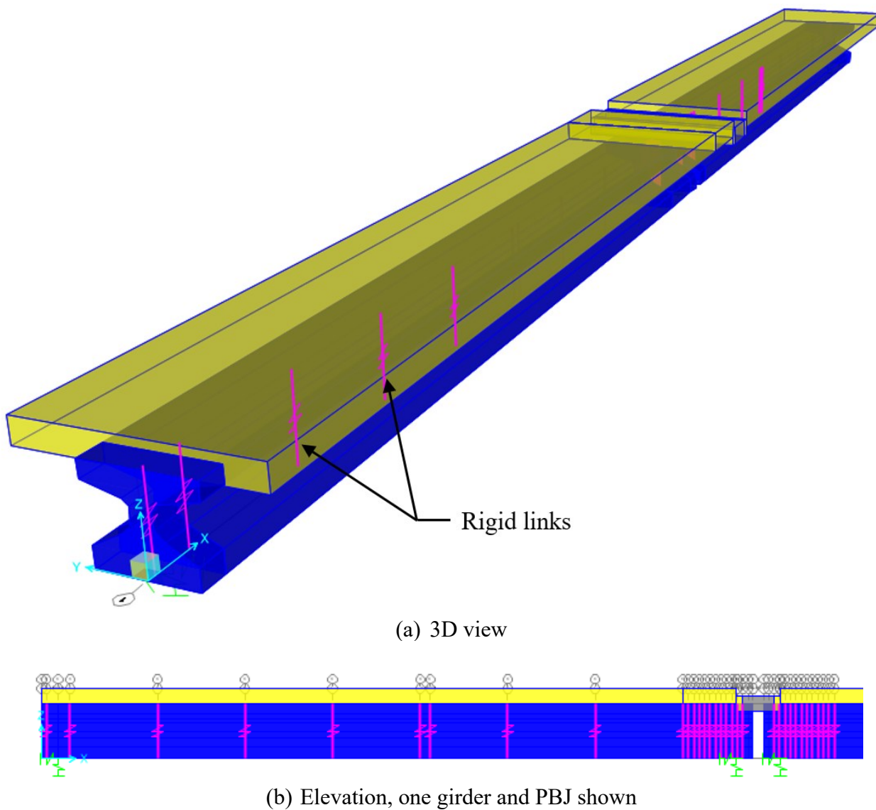
Figure 8.98. Simplified SAP2000 model using a single girder line with offset beam elements connected with rigid links.
