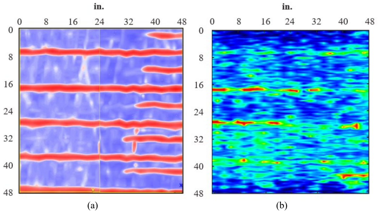
Figure 4.44. LUB2 results for (a) GPR and (b) UST of top transverse reinforcement at depth 2.73 in.
