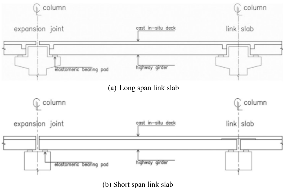
Figure 2.38. Short- and long-span link slabs, reprinted from Charuchaimontri et al. (2008).
