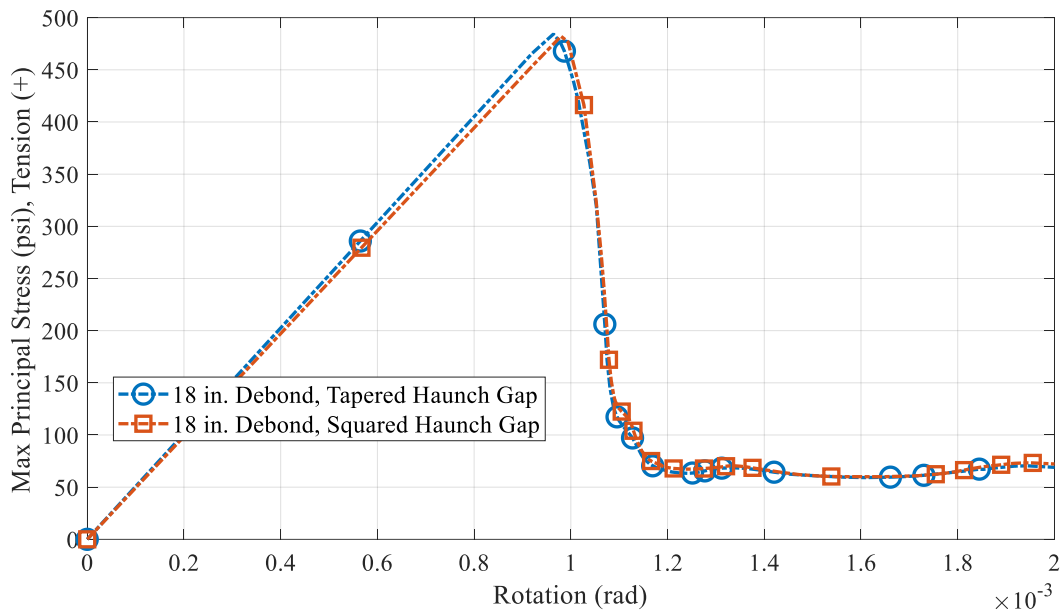
Figure 8.49. Comparison of concrete principal stress at the location of first cracking for debonded offset precast panel models with different haunch gap end conditions.
