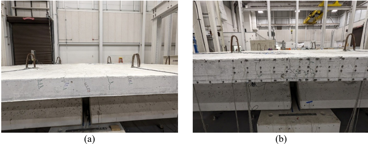
Figure 9.57. PBJ-OP2: Deck edge cracks following Pattern All-Yield on (a) north half of deck and (b) south half of deck.
