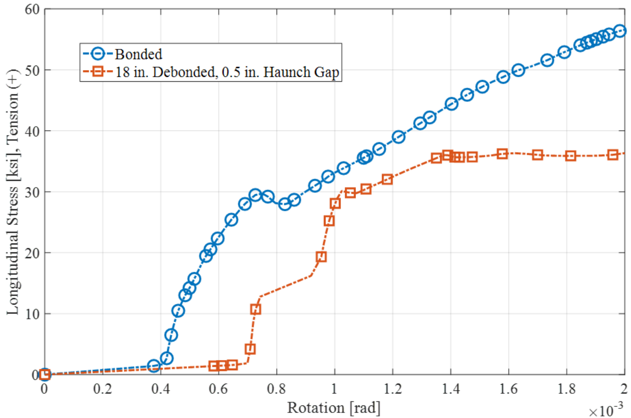
Figure 8.86. Bonded and debonded comparison of dual-girder skewed models, showing longitudinal stress in the top longitudinal reinforcement at the location of first cracking in each deck.
