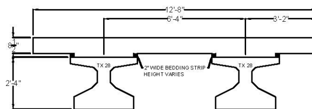
Figure 9.3. Generic cross-section of specimen.
