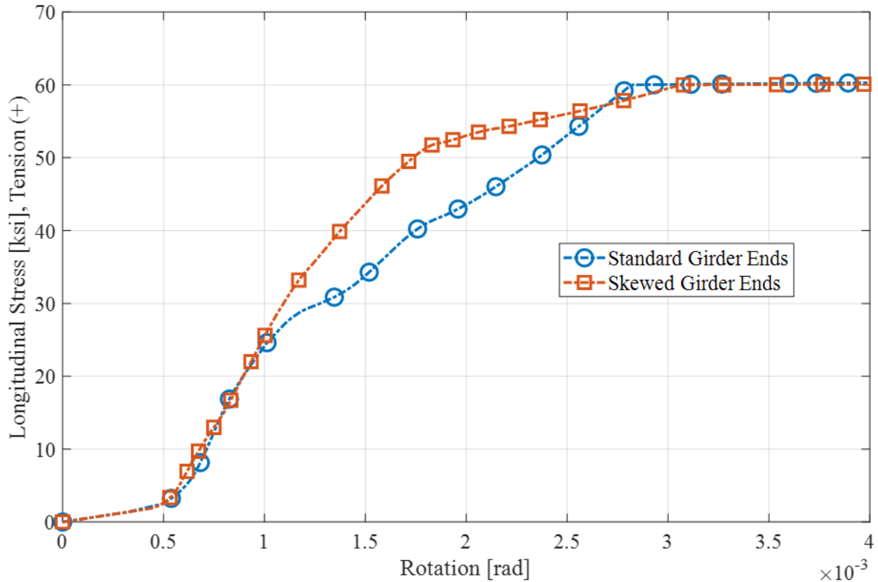
Figure 8.71. Comparison of longitudinal stress in the top longitudinal reinforcement adjacent to the point of first cracking in the deck for the skewed girder stub models with standard girder ends and skewed girder ends.
