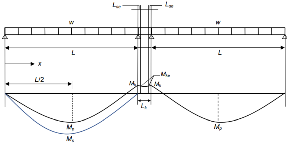
Moment diagram due to a uniformly distributed load w applied continuously
