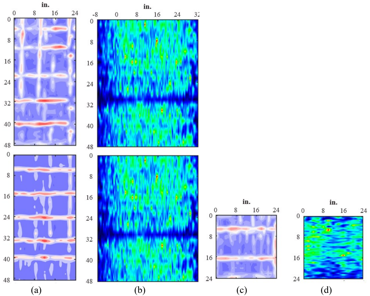
Figure 4.37. LUB1 results for top longitudinal reinforcement at depth 3.73 in. for (a) GPR in NDE Regions 1 and 2, (b) UST in Regions 1 and 2, (c) GPR in Region 3, and (d) UST in Region 3.
