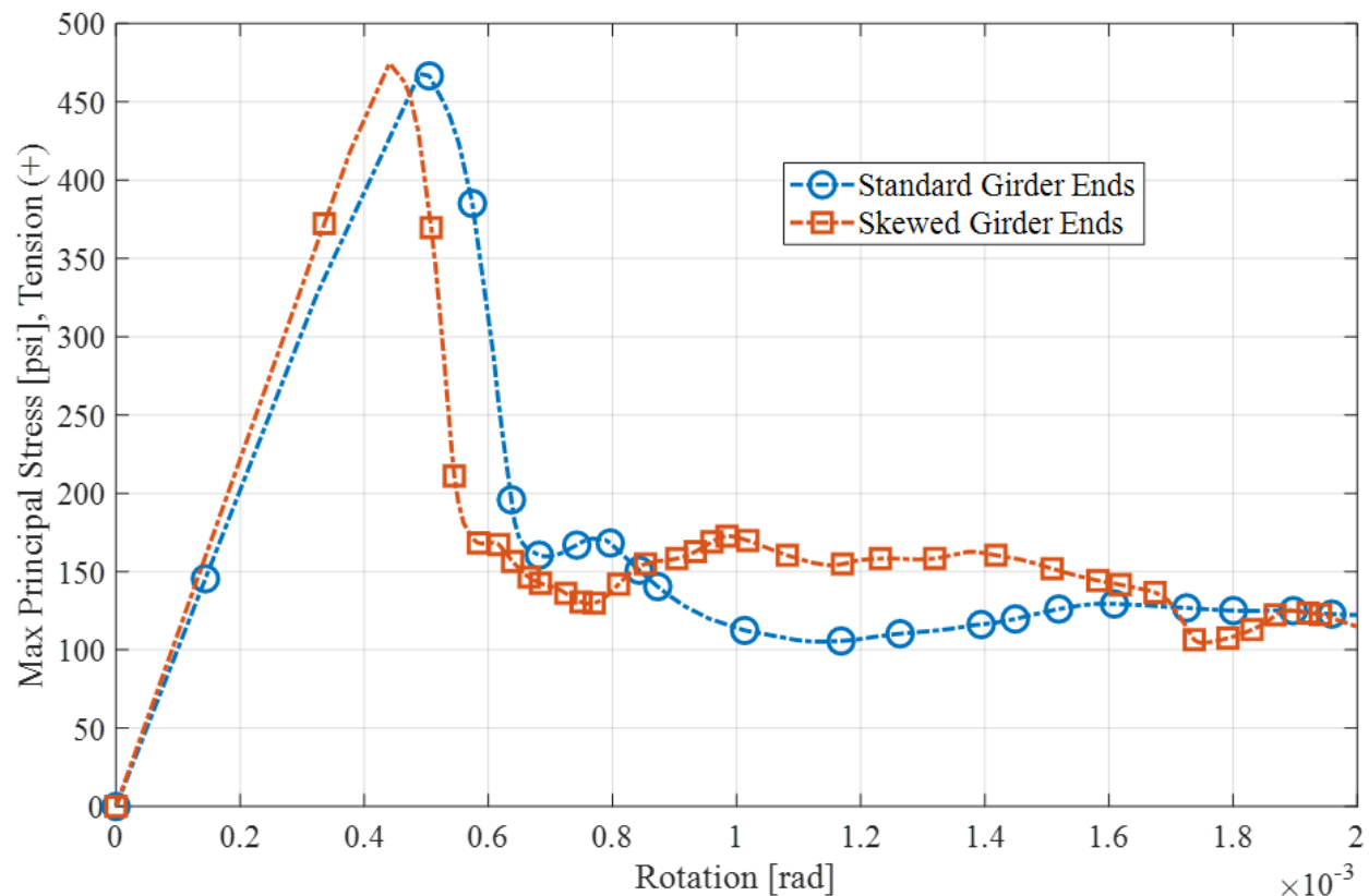
Figure 8.70. Comparison of maximum principal stresses at the point of first cracking for the skewed girder stub models with standard girder ends and skewed girder ends.
