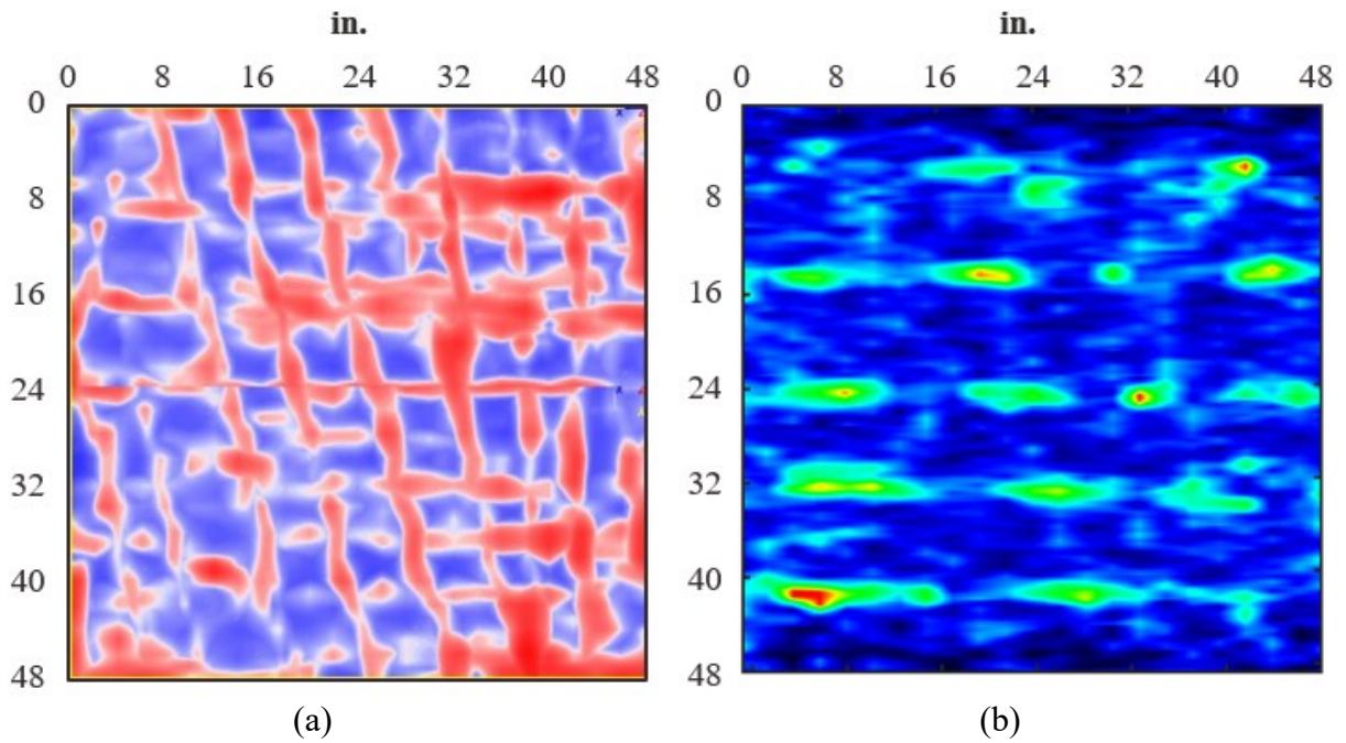
Figure 4.16. ATL2 results for (a) GPR and (b) UST of bottom transverse reinforcement at depth 6.73 in.
