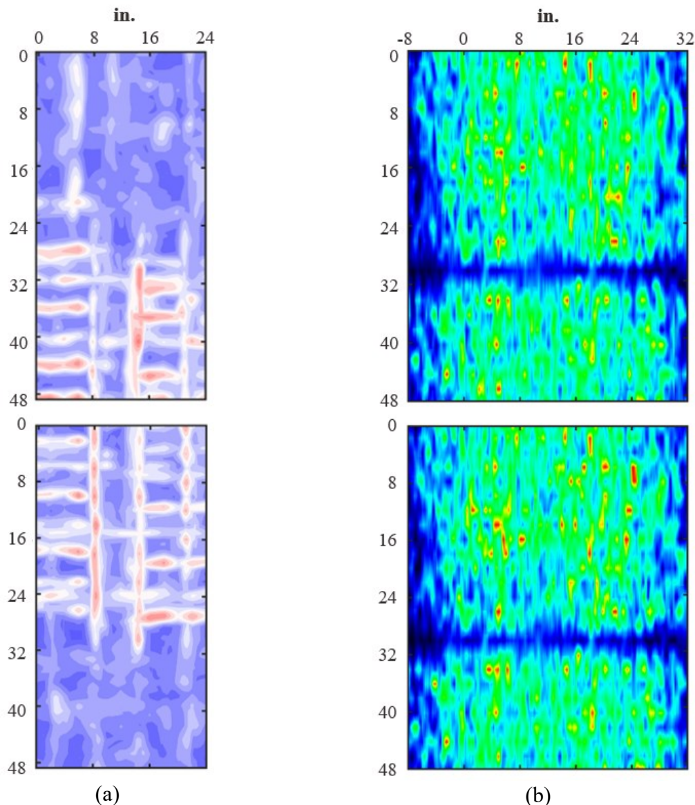
Figure 4.39. LUB1 results for bottom reinforcement at depth 6.98 in. for (a) GPR in NDE Regions 1 and 2, and (b) UST in Regions 1 and 2.
