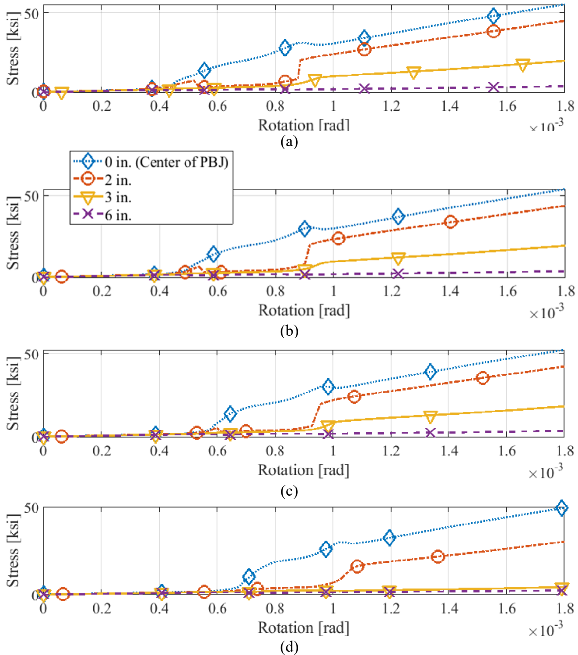
Figure 8.26. Effect of debonded length on top longitudinal reinforcing steel stresses, showing (a) a fully bonded slab, as well as a slab debonded at the girder-slab interface for (b) 16 in., (c) 35 in., and (d) 54 in.
