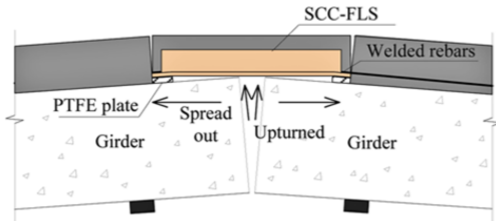
Figure 2.63. Composite link slab design, reprinted from Wang et al. (2019).
