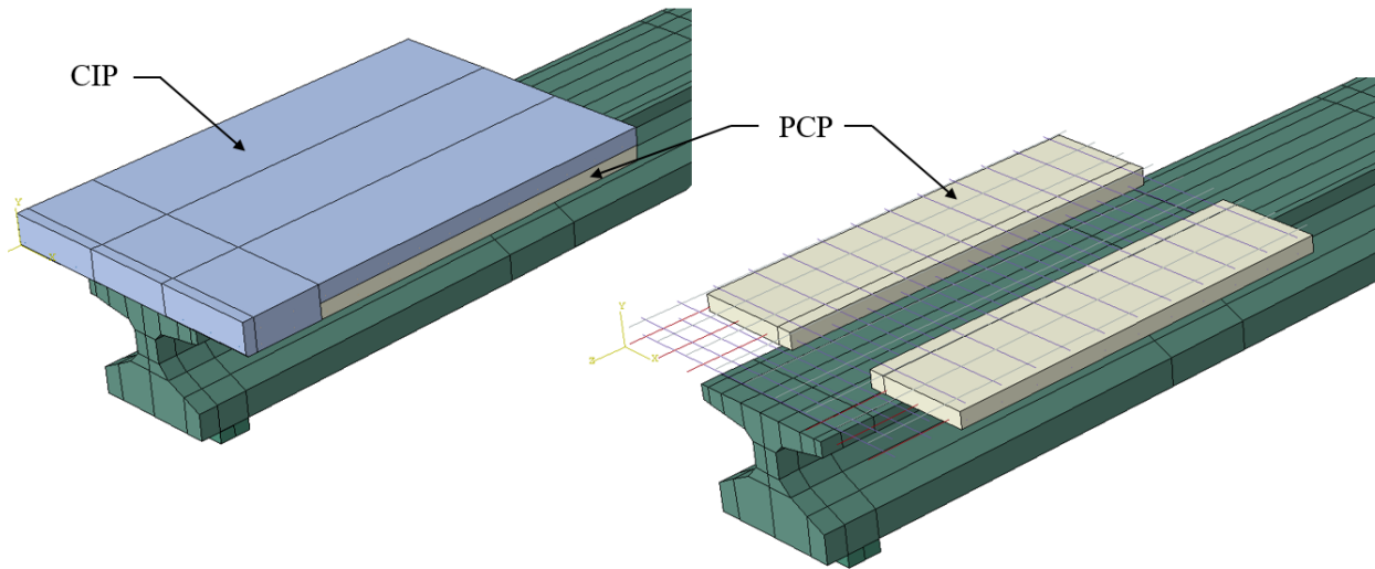
Figure 8.5. Single-girder offset precast panel model, showing the CIP topping slab (left) and without the CIP concrete, revealing the offset PCPs and reinforcement beneath (right).
