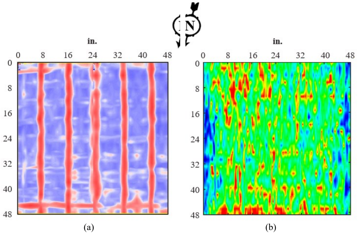
Figure 4.20. ATL3 results for (a) GPR and (b) UST of top longitudinal reinforcement at depth 2.72 in.
