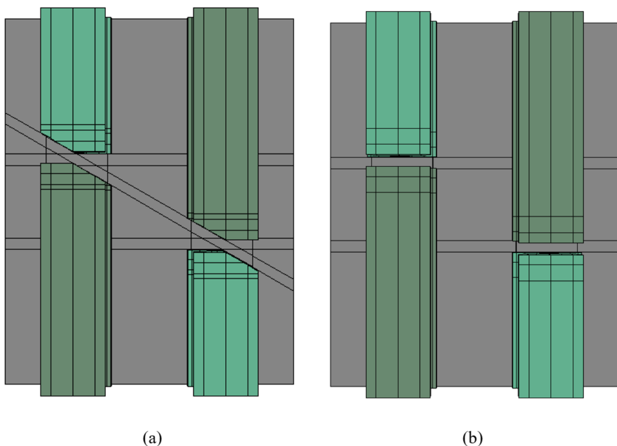
Figure 8.67. Underside of skewed stub models, showing (a) a skewed girder end condition and (b) a flat girder end condition.
