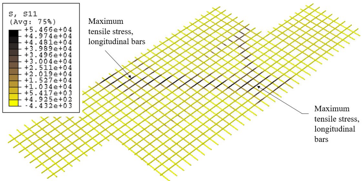
Figure 8.83. Stress in the top longitudinal and transverse bars for the debonded skewed model, showing maximum tensile stresses forming over the girder, with stresses extending diagonally between girder lines following the cracking pattern.
