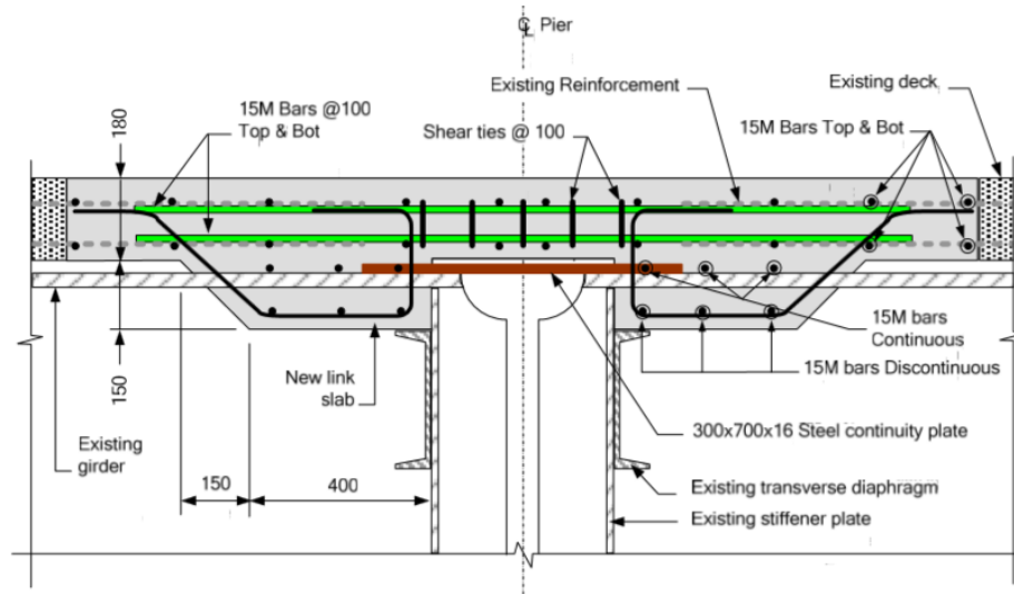
Figure 2.43. Dixon Road Overpass link slab detail, reprinted from Lam et al. (2008).
