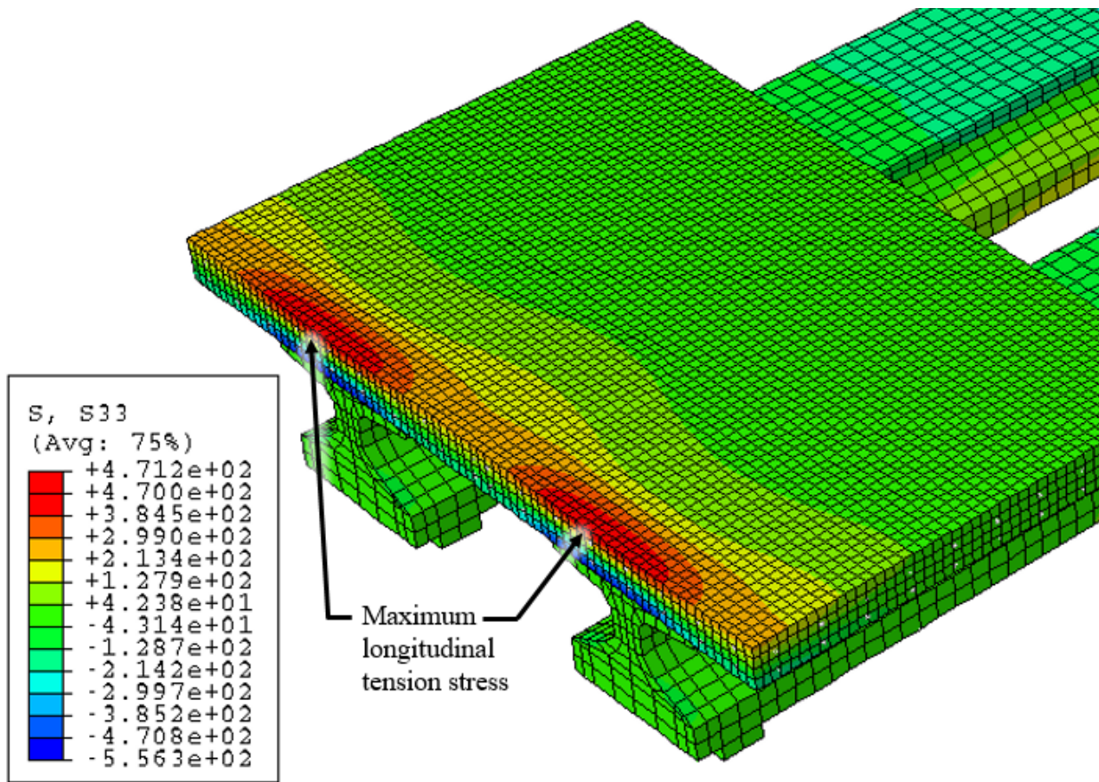
Figure 8.2. Shear lag effect shown by longitudinal stress distribution with hourglass shape over the girder ends.
