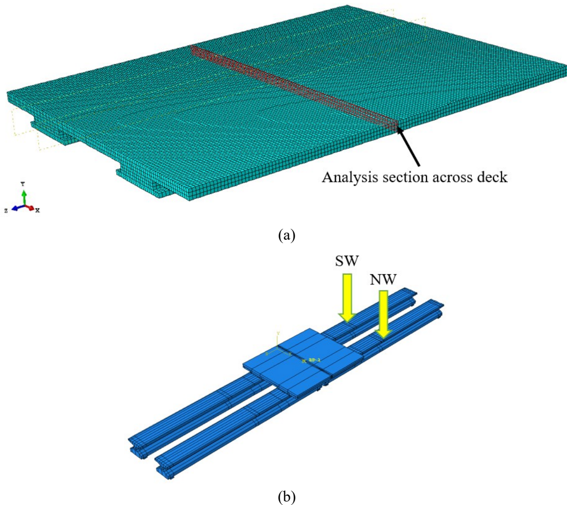
Figure 8.65. (a) Deck model used to analyze tensile forces across the PBJ, and (b) loading diagram for the flush PCP model.
