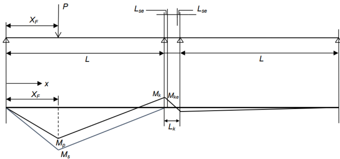
Moment diagram due to a concentrated load P applied at distance X_F
