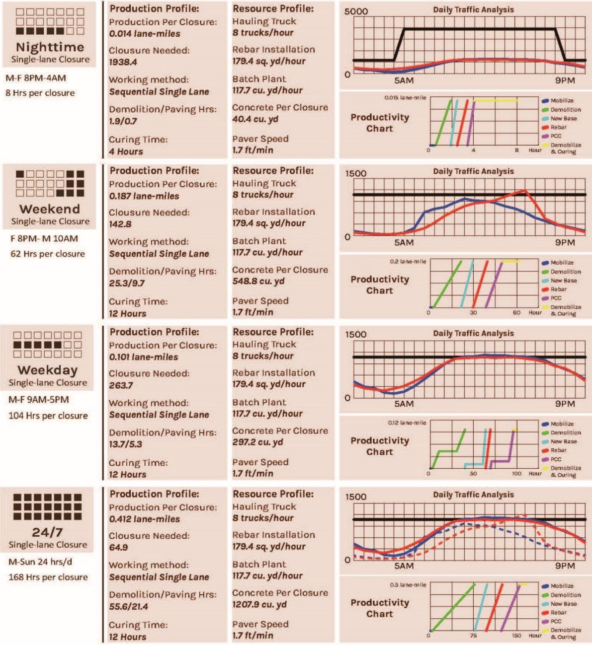
Figure 56. IH 45 Traffic Analysis Page 3.
