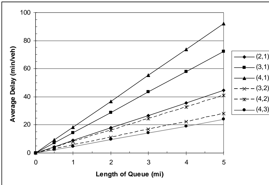
Figure 9. Effect of Queue Length on Average Delay (65-mph Roadways).
