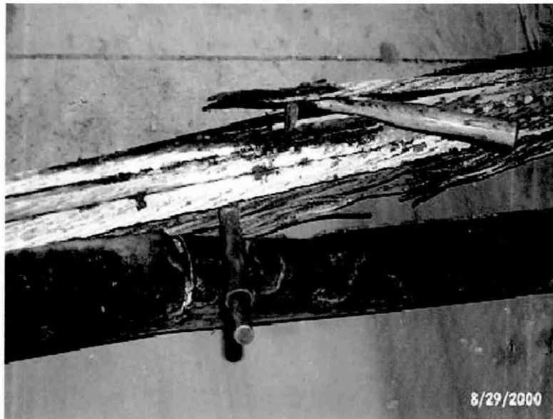
Figure 2.8 Failure of Tendon 28-6 on the Mid-Bay Bridge 16
