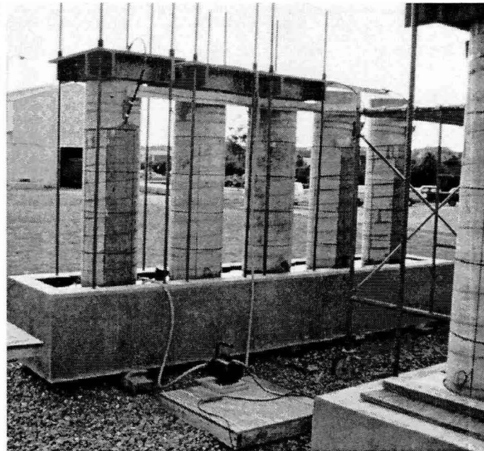
Figure 3.18 Column Test Setup 37
