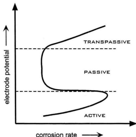
Figure 2.12 Passive-Active Behavior in Steel 34
