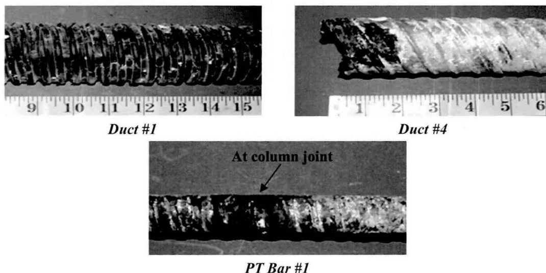
Figure 3.21 Duct and PT Bar Condition for Specimen PT-TC-S-PD
