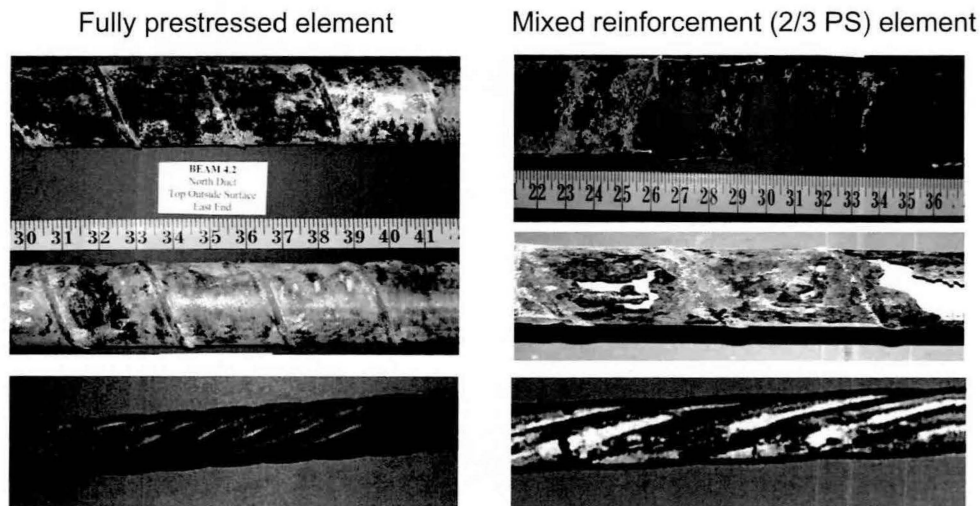
Figure 3.27 Corrosion in Galvanized Steel Duct in Beams with Different Levels of Post-Tensioning 37,38
