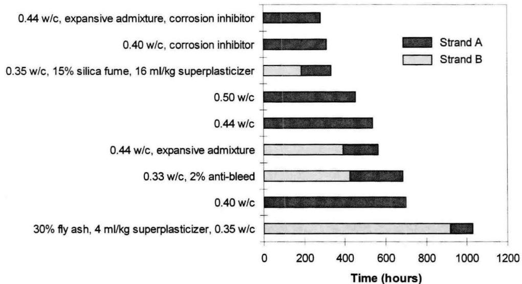
Figure 3.4 Comparison of ACTM Average Times to Corrosion 34
