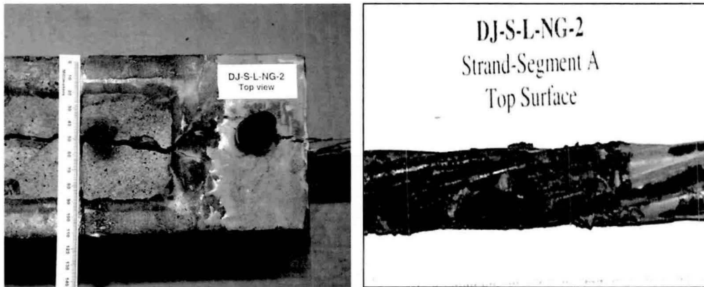
Figure 3.25 Example of Longitudinal (Splitting) Crack in Macrocell Specimen 83
