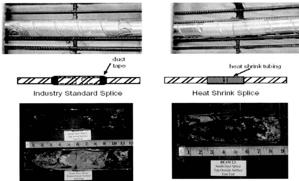
Figure 3.28 Duct Splice Performance 37
