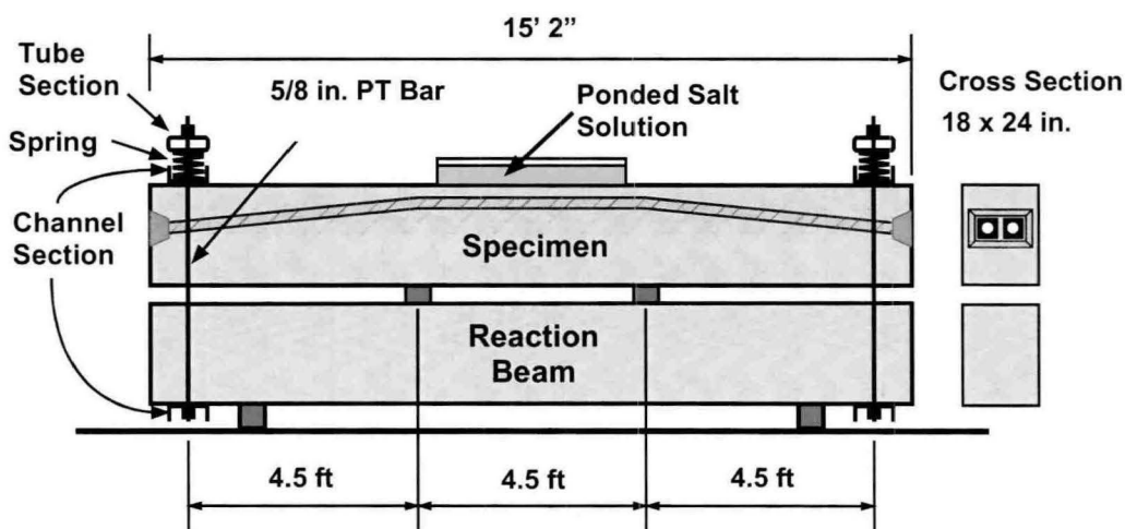
Figure 3.14 Test Setup 33
