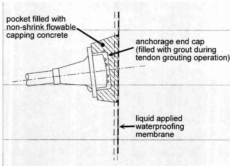
Figure 2.17 Multi-Layer Corrosion Protection for Buried Post-Tensioning Anchorages 22
