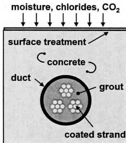
Figure 2.15 Multilayer Corrosion Protection for Bonded Post-Tensioned Systems 33
