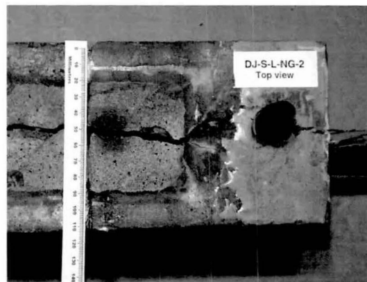
Figure 3.10 Example of Specimen Condition Prior to Autopsy Specimen DJ-S-L-NG-2 83
