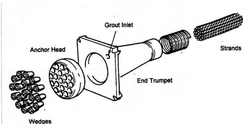
Figure 2.1 Post-Tensioning Anchorage Details (from T.Y. Lin, and N.H. Burns, 1981) 34
