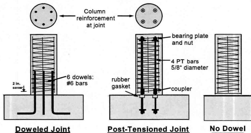
Figure 3.19 Column-Foundation Joint Configurations 37
