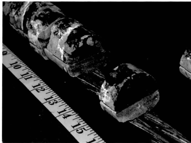
Figure 3.31 Effect of Grout Cracking 37
