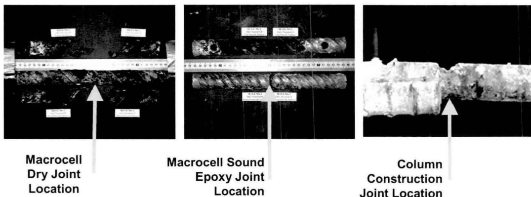
Figure 3.26 Segmental or Construction Joint Performance 37
