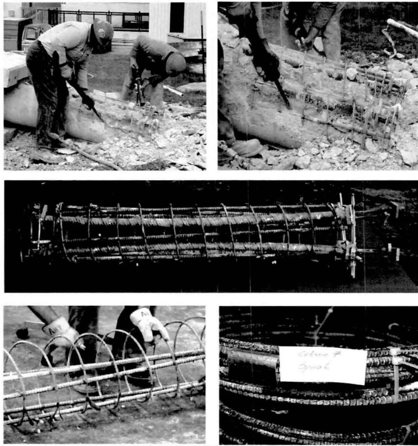
Figure 3.20 Column Concrete Removal and Reinforcement Dismantling 37
