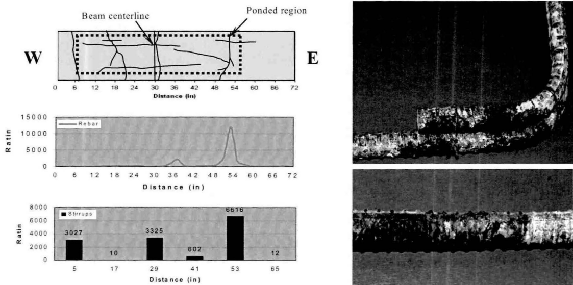
Figure 3.24 Effect of Transverse Concrete Cracking Due to Service Loading on Reinforcement Corrosion 37,38
