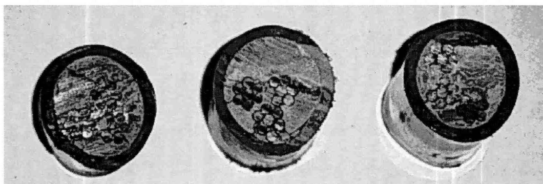
Figure 3.6 Beginning of Void Formation at Intermediate Crest 34
