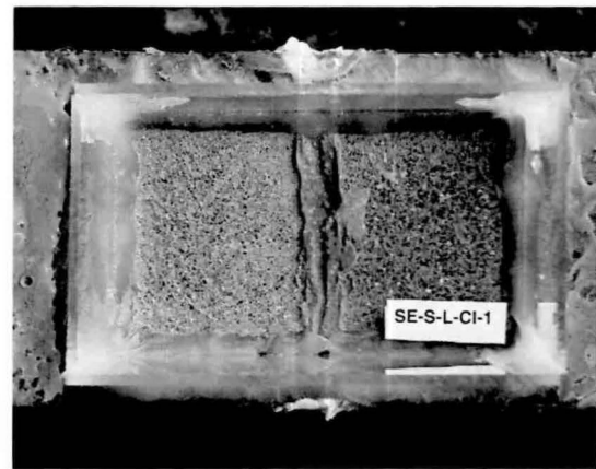
Figure 3.12 Top View of the Effect of a Faulty Epoxy Joint (SE-S-M-CI-1) Compared to a Sound Epoxy Joint (SE-S-L-CI-1)
