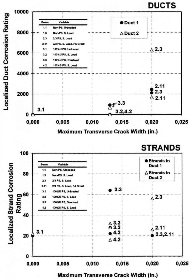
Figure 3.17 Localized Duct and Strand Corrosion Rating versus Maximum Crack Width for Phase I Autopsy Specimens
