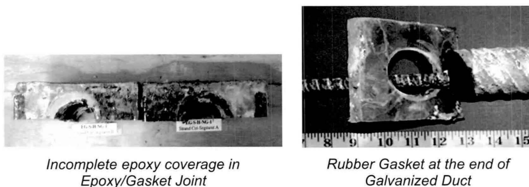
Figure 3.29 Effect of the Use of Rubber Gaskets 37
