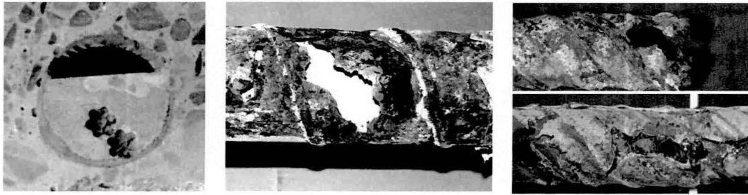
Figure 3.30 Bleed Water Voids and Duct Corrosion 37
