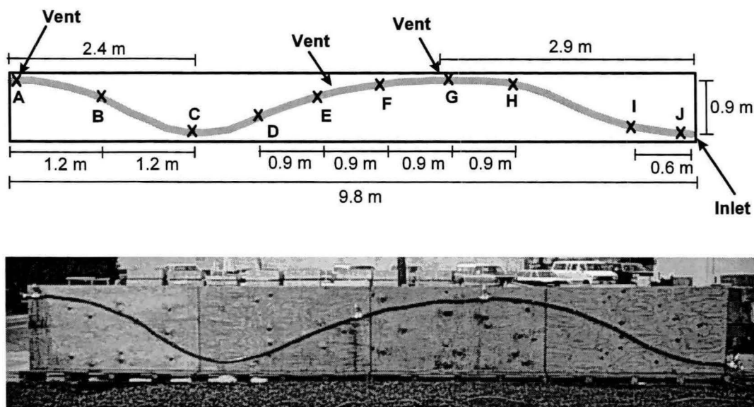
Figure 3.1 Large-Scale Clear Draped Parabolic Duct Test 34
