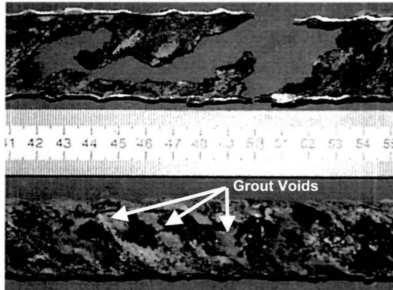
Figure 3.11 Hole in Duct Corresponding to Grout Void (Specimen DJ-S-M-NG-2) (From Autopsy at Eight Years of Exposure Testing)
