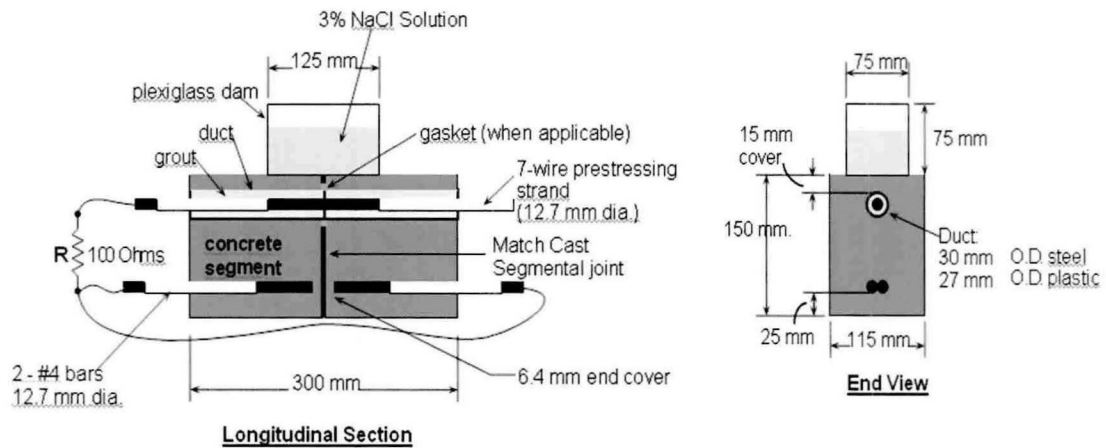
Figure 3.9 Macrocell specimen details 83
