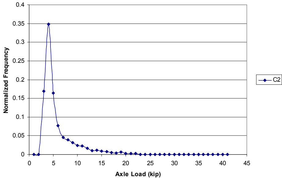
Figure 26. Axle Load Distribution for Single Axle at WIM Station D522 in Texas.
