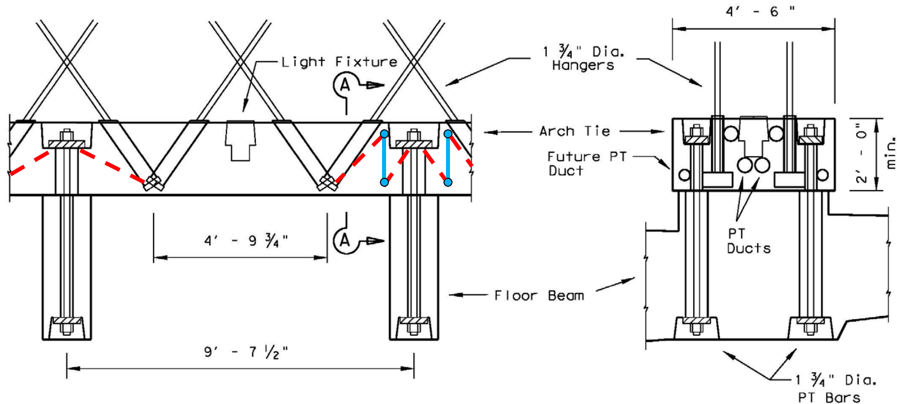
ARCH ELEVATION
